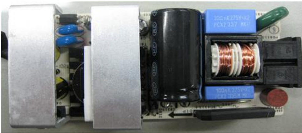
Back change AD-4014B front view
