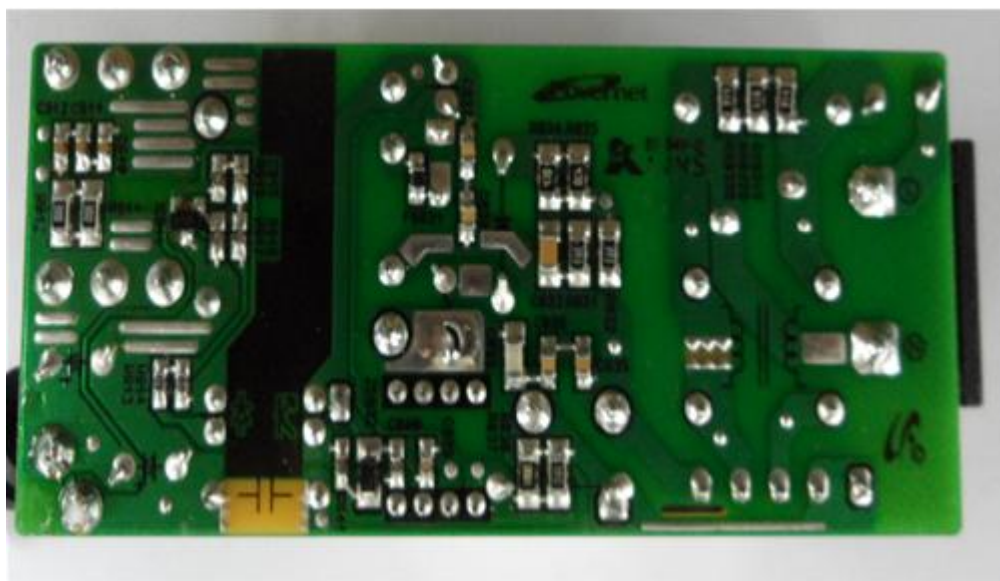
Before change PS30W-14J1 internal rear view
