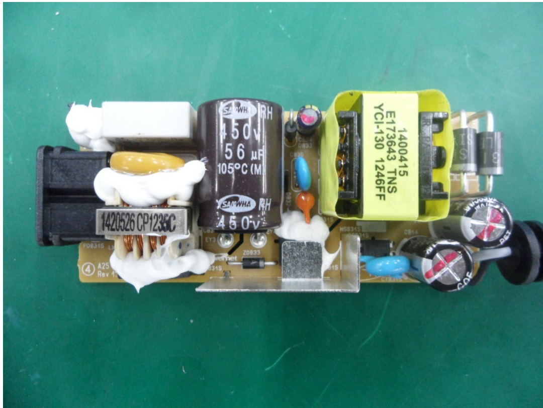
Back change A2514_DPN internal front view
