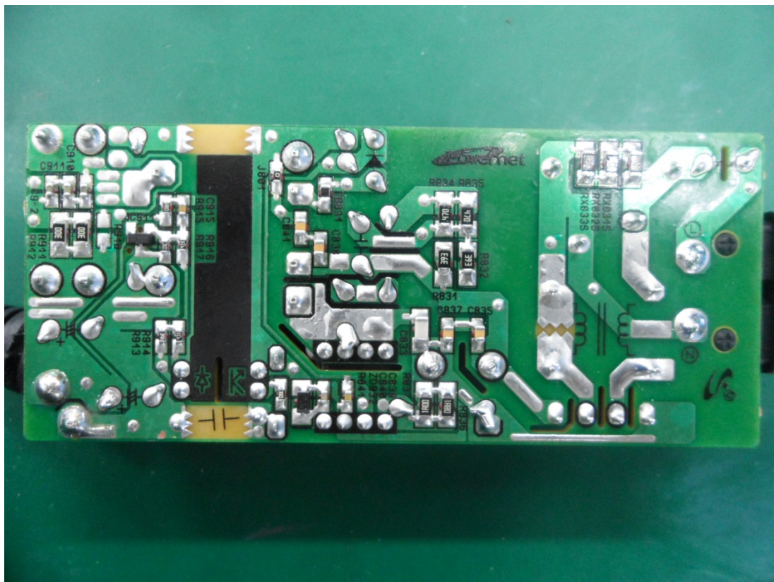
Back change A2514_DPN internal rear view
