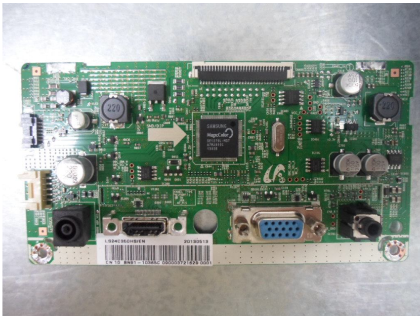
(Main Board )
