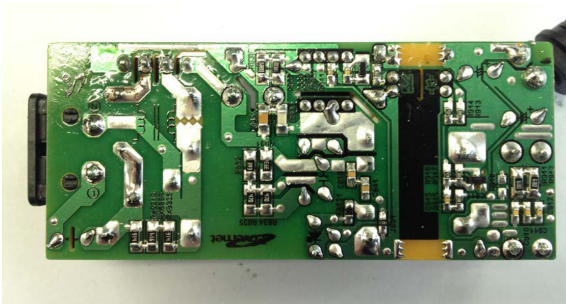
Before change A2514_DPN internal rear view
