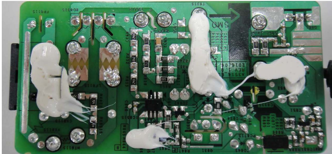
Back change A3514_DPN internal rear view
