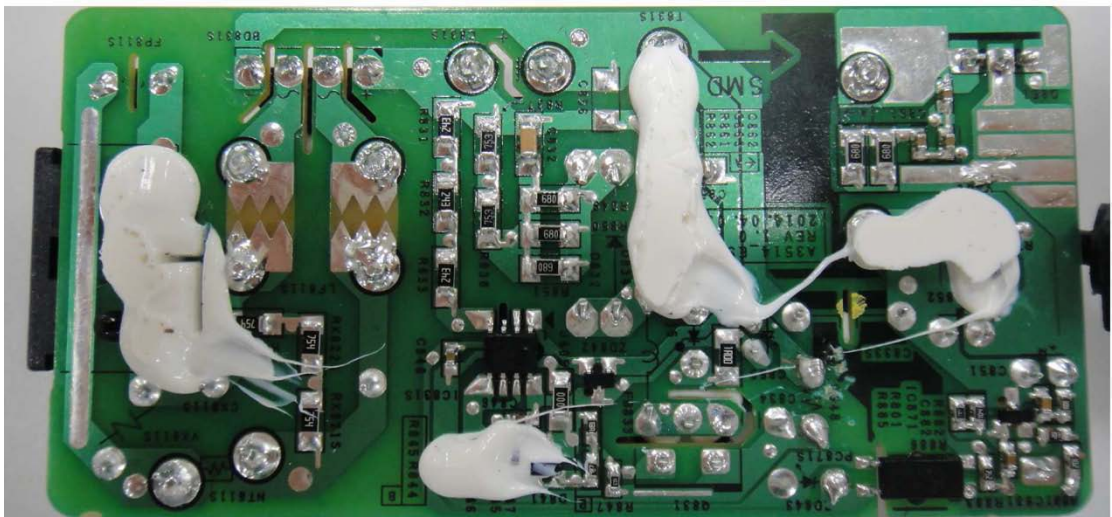
Before change A3514_ESM internal rear view
