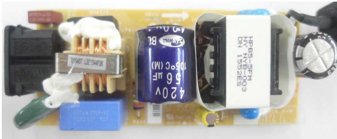
Back change A2514_KSM internal front view
