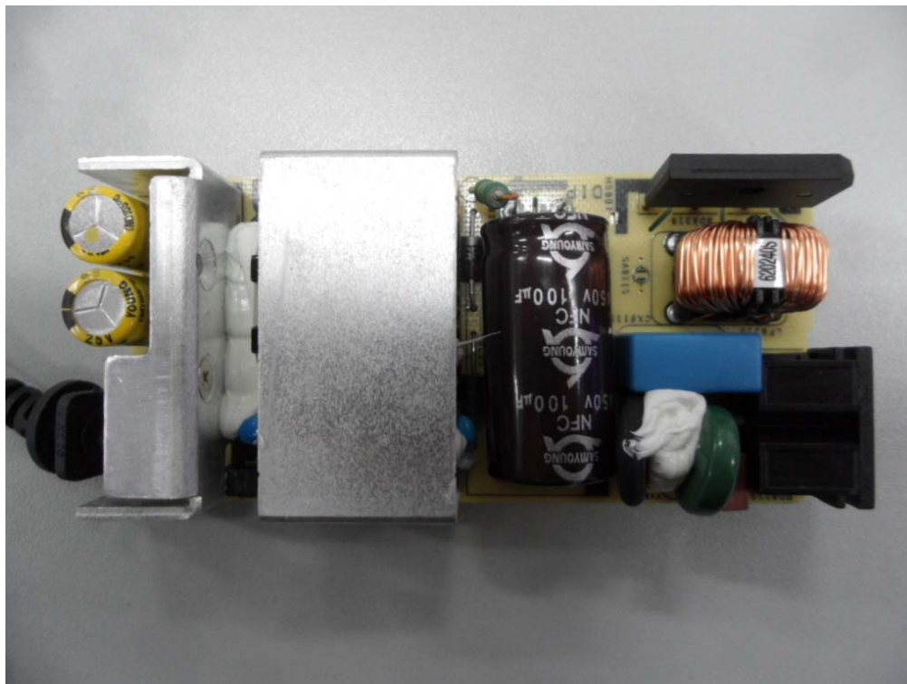
Before change A4514-DSM internal front view
