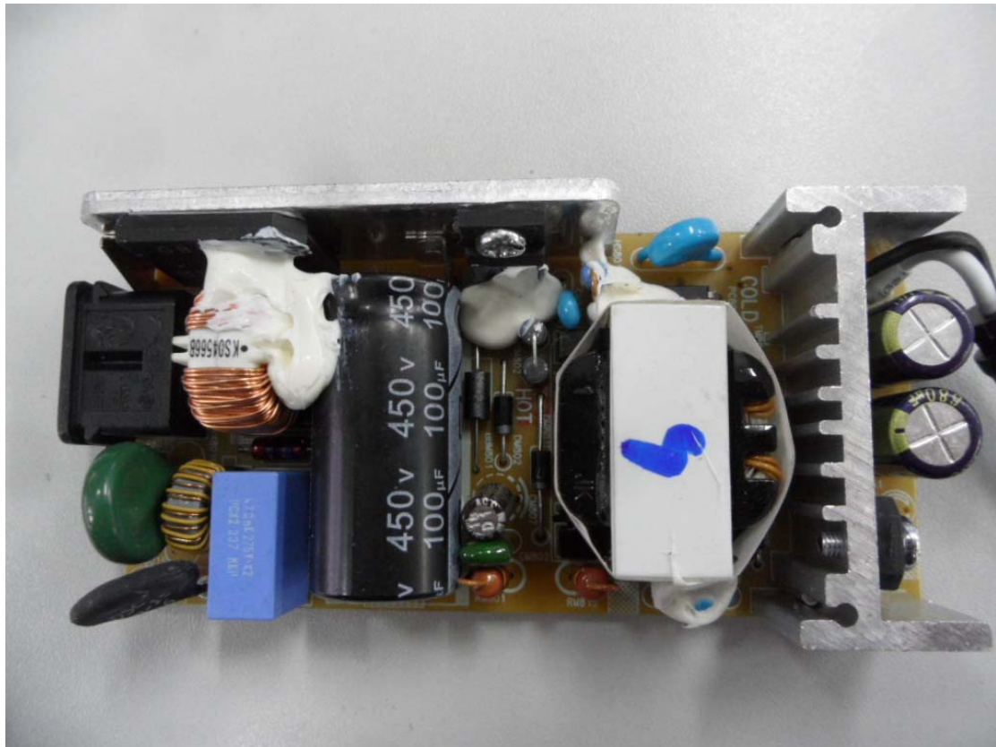
back change A4514-DDY internal front view
