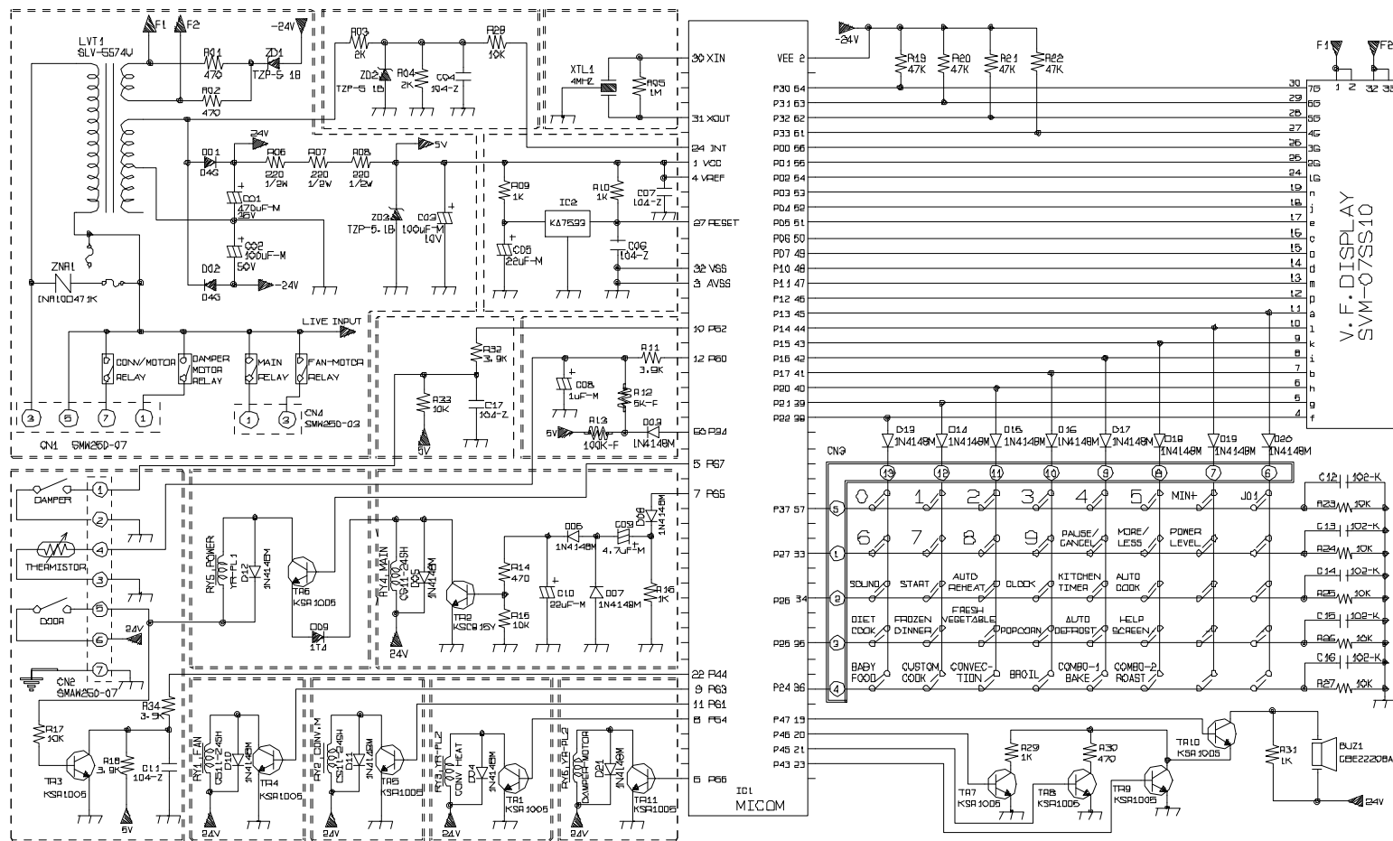
ELECTRIC-DIAGRAM MC5694
