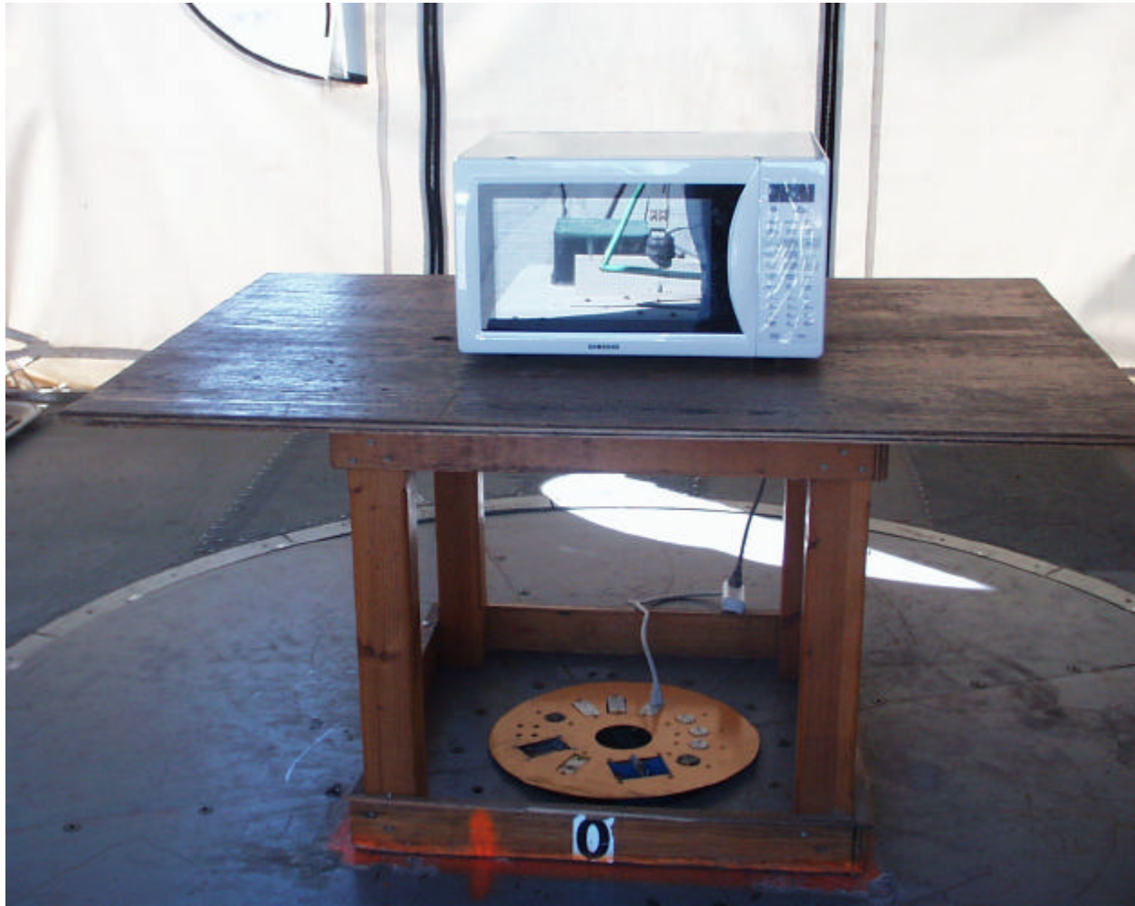
Below 1 GHz Radiated setup (Front Side)
