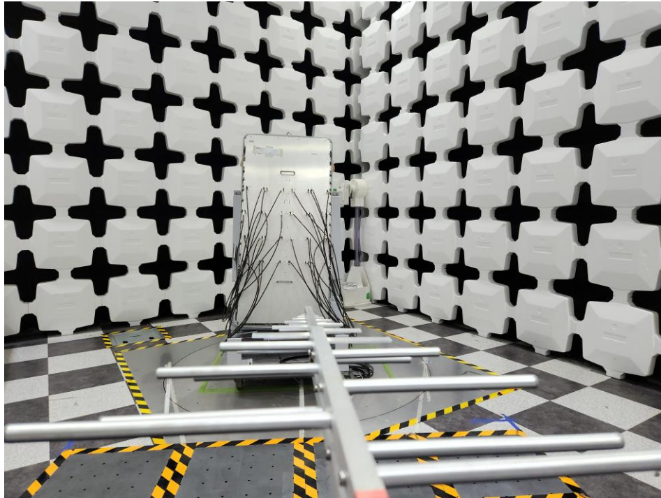
Below 1GHz Radiated spurious emission Test Measurement Setup
