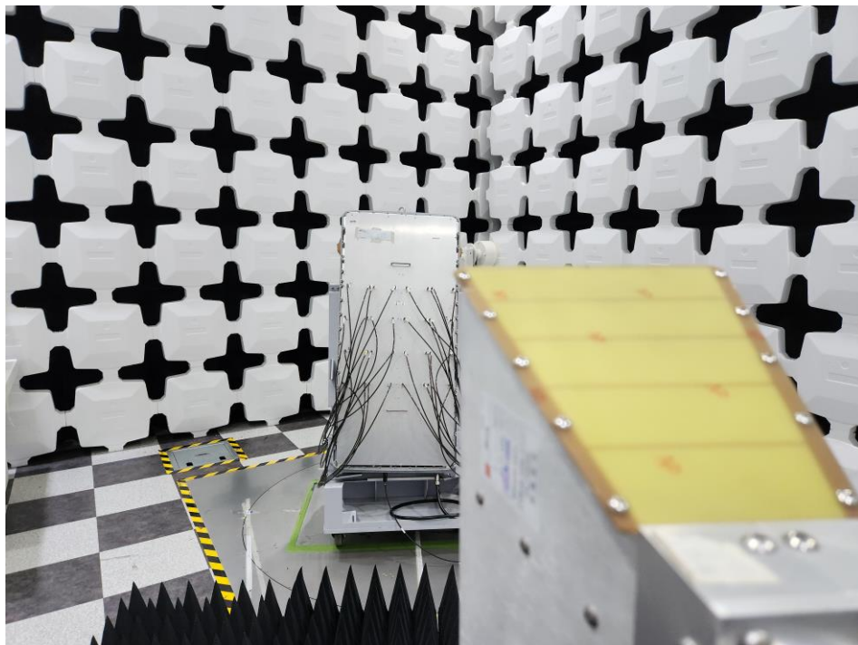
Above 1GHz Radiated spurious emission Test Measurement Setup
