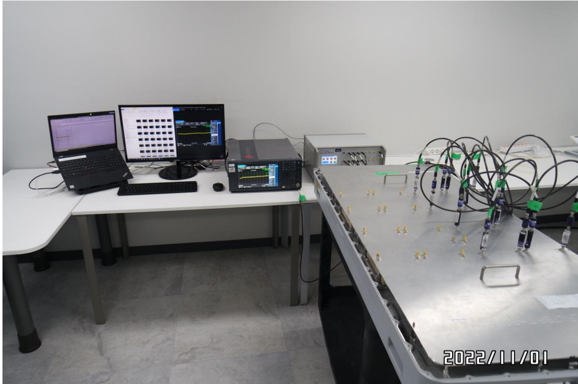
Conducted Test Measurement Setup
