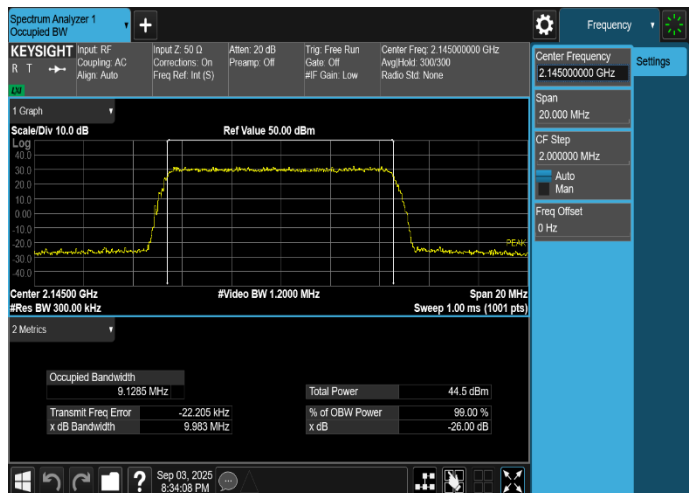
Plot 8-42. Occupied Bandwidth Plot (LTE_B66_1C_10M_256QAM - Mid Channel, Port 18)
