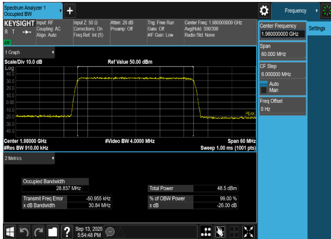
Plot 8-19. Occupied Bandwidth Plot (NR_n25_1C_30M_QPSK - High Channel, Port 3)
