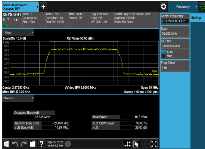
Plot 8-43. Occupied Bandwidth Plot (LTE_B66_1C_15M_QPSK - High Channel, Port 28)
