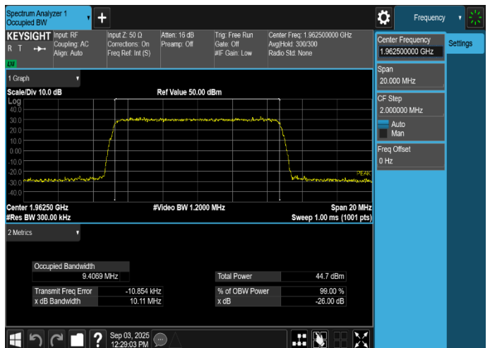
Plot 8-12. Occupied Bandwidth Plot (NR_n25_1C_10M_64QAM - Mid Channel, Port 6)
