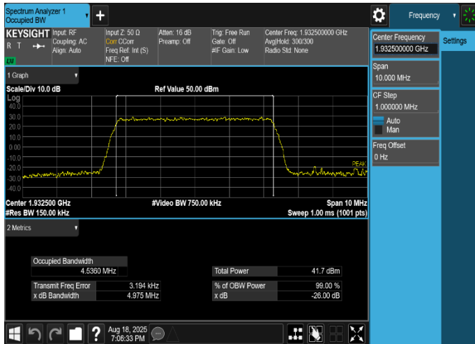
Plot 8-1. Occupied Bandwidth Plot (LTE_B25_1C_5M_QPSK - Low Channel, Port 28)
