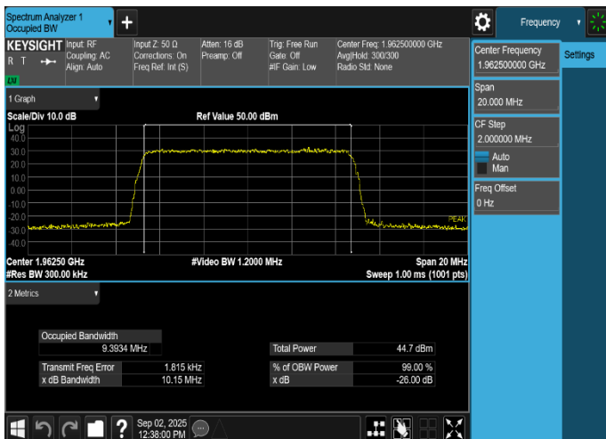
Plot 8-11. Occupied Bandwidth Plot (NR_n25_1C_10M_QPSK - Mid Channel, Port 9)
