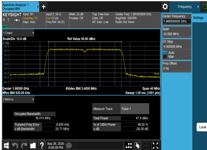
Plot 8-31. Occupied Bandwidth Plot (NR_n25_2C_10M+10M_QPSK - High Channel, Port 19)
