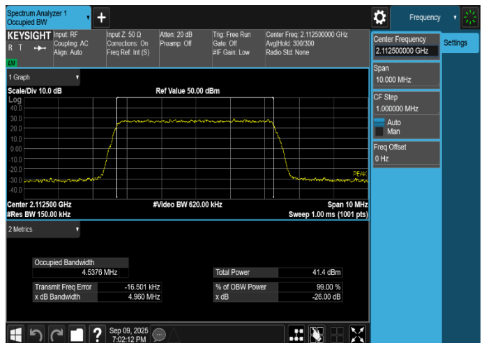
Plot 8-48. Occupied Bandwidth Plot (NR_n66_1C_5M_64QAM - Low Channel, Port 31)
