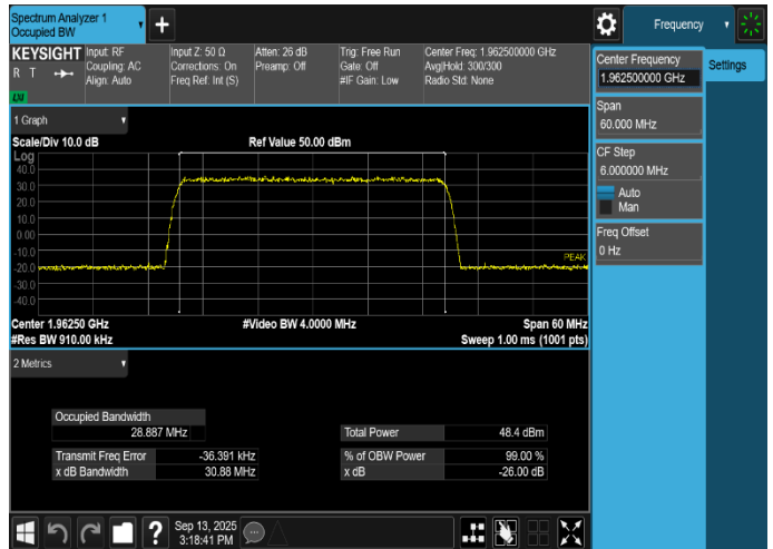
Plot 8-20. Occupied Bandwidth Plot (NR_n25_1C_30M_256QAM - Mid Channel, Port 20)
