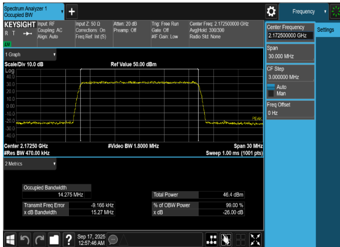
Plot 8-51. Occupied Bandwidth Plot (NR_n66_1C_15M_QPSK - High Channel, Port 2)
