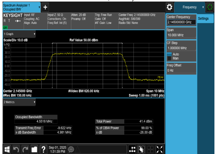
Plot 8-40. Occupied Bandwidth Plot (LTE_B66_1C_5M_256QAM - Mid Channel, Port 10)
