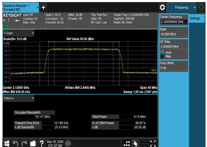
Plot 8-54. Occupied Bandwidth Plot (NR_n66_1C_20M_64QAM - Low Channel, Port 1)
