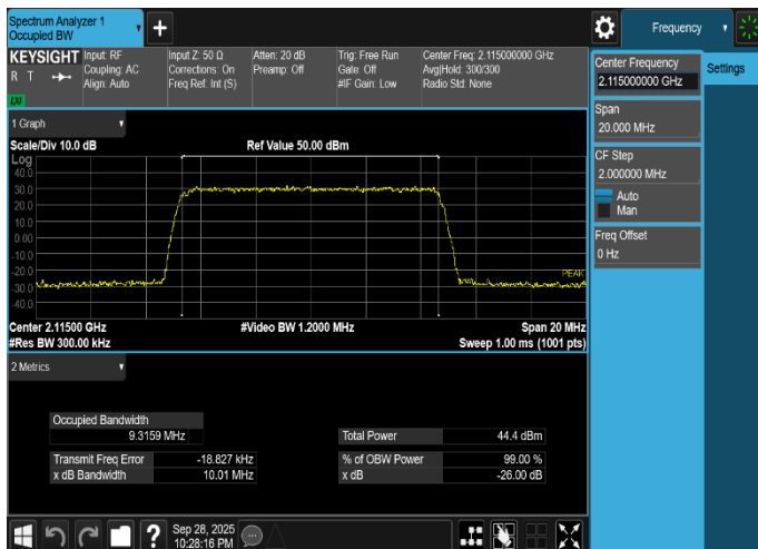
Plot 8-59. Occupied Bandwidth Plot (DSS_B/n66_1C_10M_QPSK - Low Channel, Port 26)
