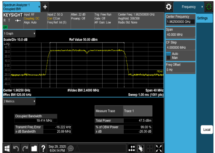
Plot 8-32. Occupied Bandwidth Plot (NR_n25_2C_10M+10M_16QAM - Mid Channel, Port 0)
