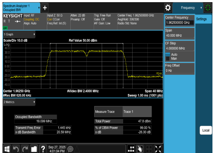
Plot 8-28. Occupied Bandwidth Plot (LTE_B25_2C_10M+10M_16QAM - Mid Channel, Port 8)
