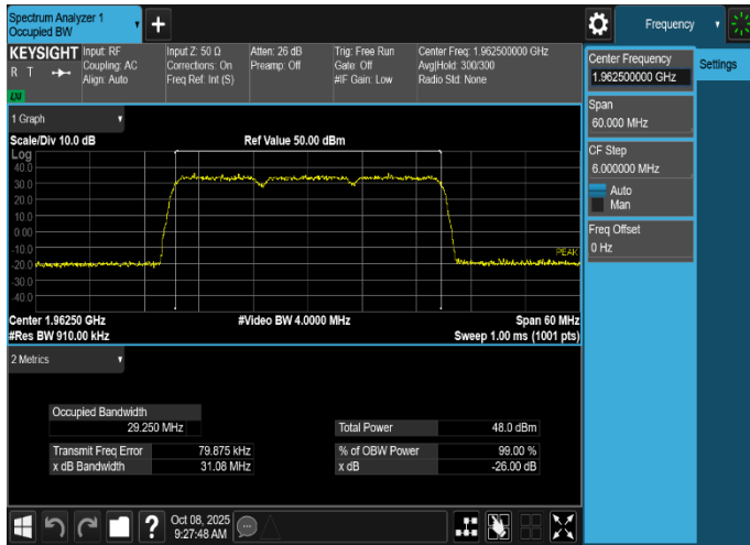
Plot 8-37. Occupied Bandwidth Plot (MSR_B/n25_3C_LTE 10M+NR 10M+DSS 10M_QPSK - Mid Channel, Port 30)
