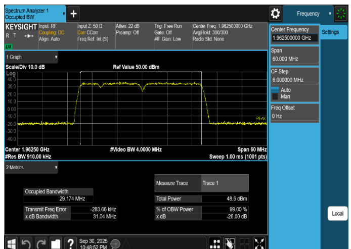
Plot 8-30. Occupied Bandwidth Plot (LTE_B25_3C_5M+10M+15M_16QAM - Mid Channel, Port 13)
