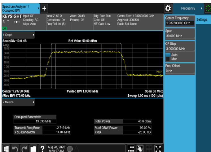
Plot 8-5. Occupied Bandwidth Plot (LTE_B25_1C_15M_QPSK - Low Channel, Port 11)
