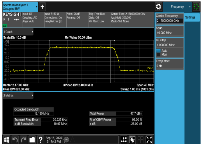
Plot 8-46. Occupied Bandwidth Plot (LTE_B66_1C_20M_256QAM - High Channel, Port 16)
