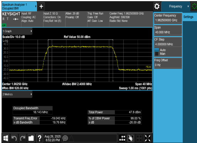
Plot 8-7. Occupied Bandwidth Plot (LTE_B25_1C_20M_QPSK - Mid Channel, Port 11)
