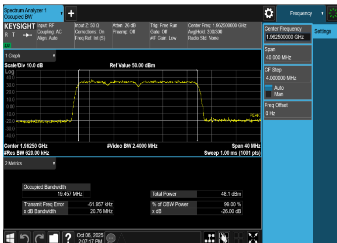
Plot 8-35. Occupied Bandwidth Plot (MSR_B/n25_3C_LTE 5M+NR 5M+DSS 10M_QPSK - Mid Channel, Port 9)
