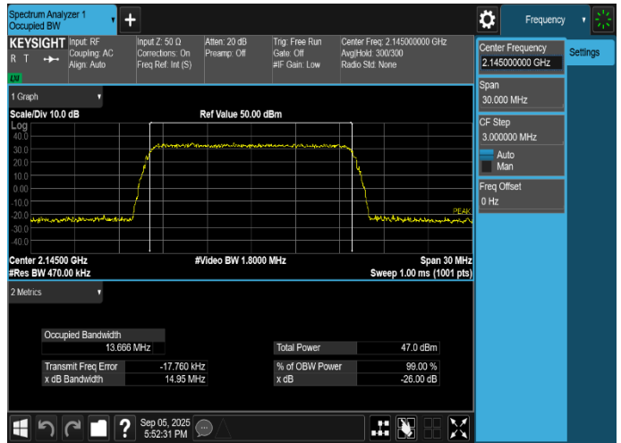
Plot 8-44. Occupied Bandwidth Plot (LTE_B66_1C_15M_64QAM - Mid Channel, Port 8)
