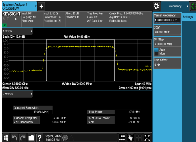
Plot 8-25. Occupied Bandwidth Plot (DSS_B/n25_1C_20M_QPSK - Low Channel, Port 14)
