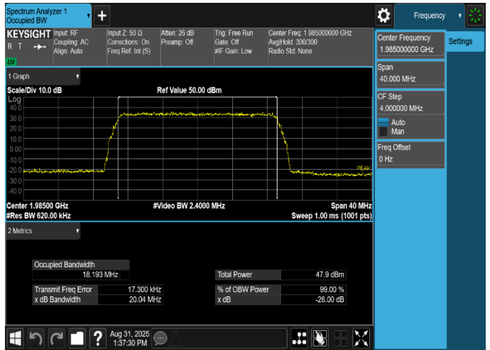
Plot 8-8. Occupied Bandwidth Plot (LTE_B25_1C_20M_256QAM - High Channel, Port 29)
