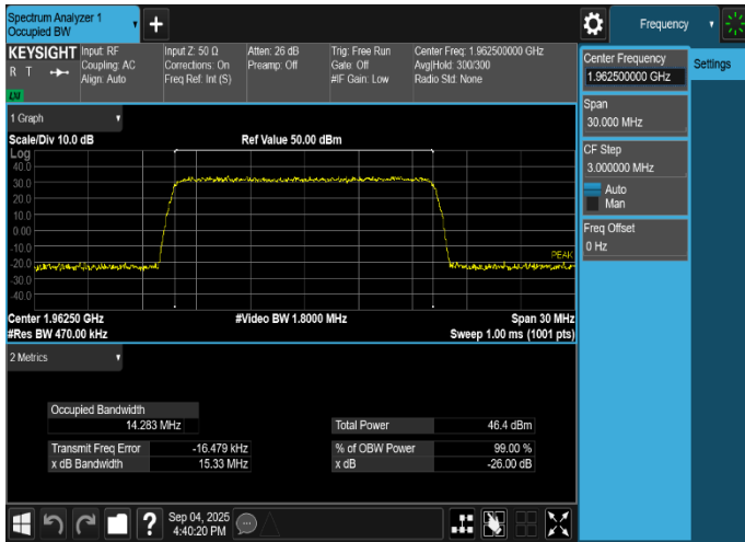
Plot 8-13. Occupied Bandwidth Plot (NR_n25_1C_15M_QPSK - Mid Channel, Port 5)
