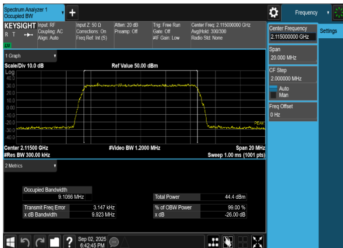
Plot 8-41. Occupied Bandwidth Plot (LTE_B66_1C_10M_QPSK - Low Channel, Port 20)
