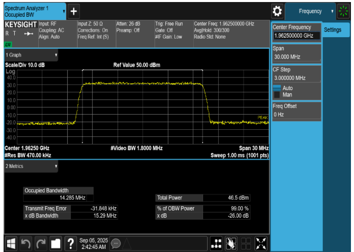
Plot 8-14. Occupied Bandwidth Plot (NR_n25_1C_15M_256QAM - Mid Channel, Port 17)
