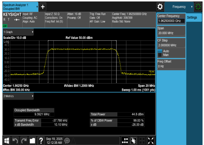
Plot 8-22. Occupied Bandwidth Plot (DSS_B/n25_1C_10M_64QAM - Mid Channel, Port 19)
