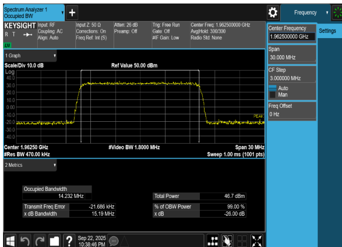
Plot 8-23. Occupied Bandwidth Plot (DSS_B/n25_1C_15M_QPSK - Mid Channel, Port 10)
