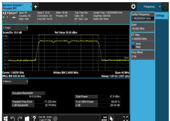
Plot 8-36. Occupied Bandwidth Plot (MSR_B/n25_3C_LTE 5M+NR 5M+DSS 10M_16QAM - Mid Channel, Port 5)
