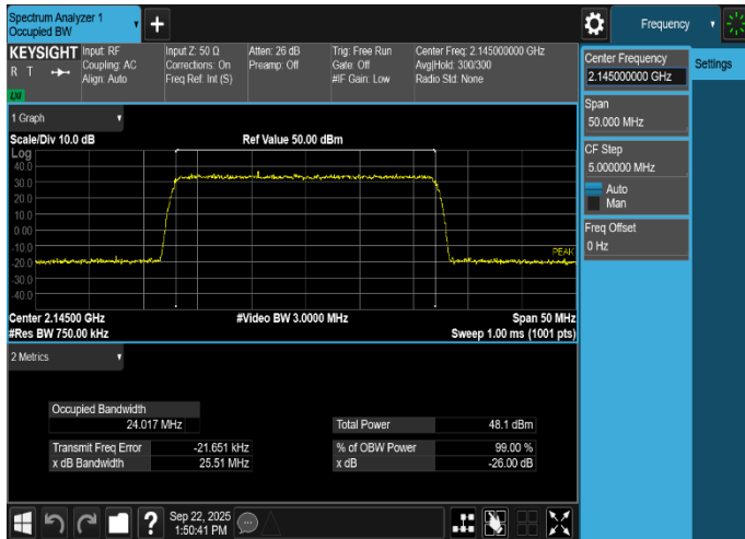
Plot 8-55. Occupied Bandwidth Plot (NR_n66_1C_25M_QPSK - Mid Channel, Port 5)
