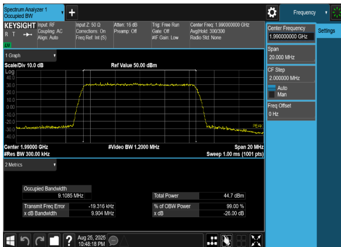
Plot 8-3. Occupied Bandwidth Plot (LTE_B25_1C_10M_QPSK - High Channel, Port 30)
