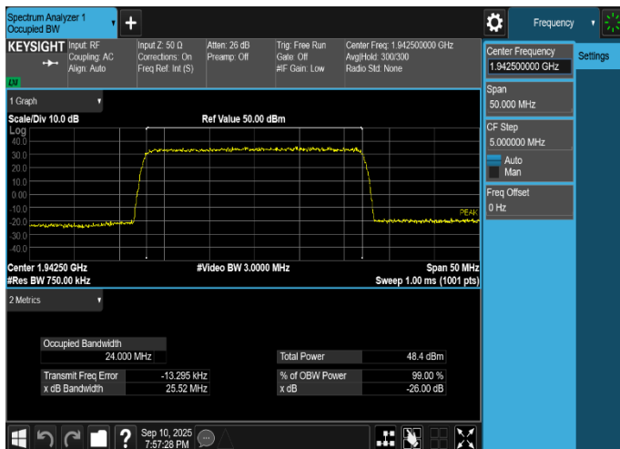
Plot 8-17. Occupied Bandwidth Plot (NR_n25_1C_25M_QPSK - Low Channel, Port 18)
