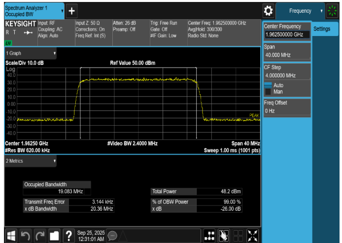
Plot 8-26. Occupied Bandwidth Plot (DSS_B/n25_1C_20M_256QAM - Mid Channel, Port 31)
