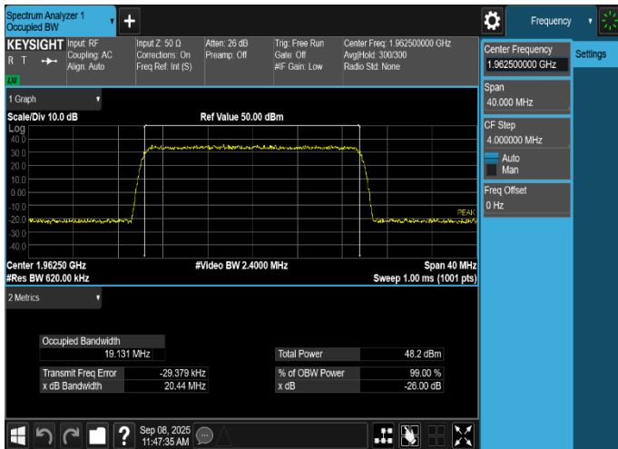
Plot 8-15. Occupied Bandwidth Plot (NR_n25_1C_20M_QPSK - Mid Channel, Port 19)
