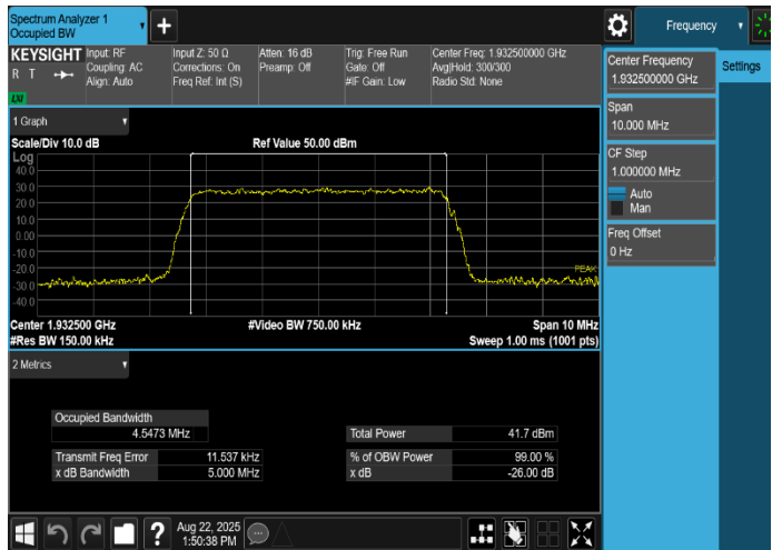
Plot 8-10. Occupied Bandwidth Plot (NR_n25_1C_5M_256QAM - Low Channel, Port 1)
