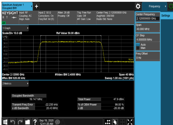
Plot 8-53. Occupied Bandwidth Plot (NR_n66_1C_20M_QPSK - Low Channel, Port 14)
