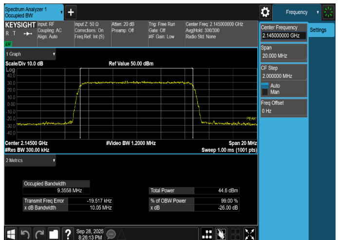
Plot 8-60. Occupied Bandwidth Plot (DSS_B/n66_1C_10M_64QAM - Mid Channel, Port 27)
