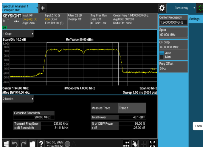
Plot 8-29. Occupied Bandwidth Plot (LTE_B25_3C_5M+10M+15M_QPSK - Low Channel, Port 10)
