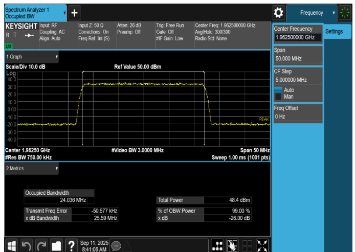
Plot 8-18. Occupied Bandwidth Plot (NR_n25_1C_25M_16QAM - Mid Channel, Port 18)
