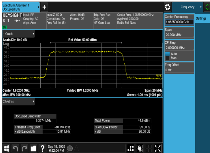
Plot 8-21. Occupied Bandwidth Plot (DSS_B/n25_1C_10M_QPSK - Mid Channel, Port 29)
