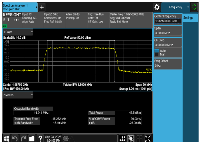
Plot 8-24. Occupied Bandwidth Plot (DSS_B/n25_1C_15M_16QAM - High Channel, Port 7)
