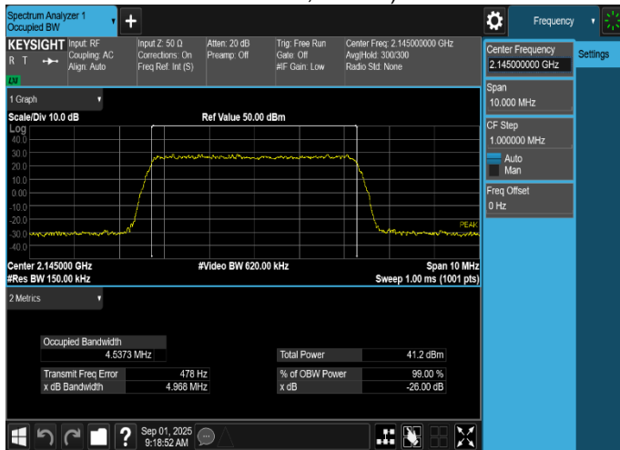
Plot 8-39. Occupied Bandwidth Plot (LTE_B66_1C_5M_QPSK - Mid Channel, Port 6)
