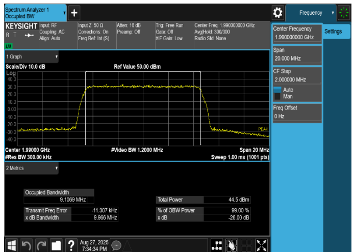
Plot 8-4. Occupied Bandwidth Plot (LTE_B25_1C_10M_64QAM - High Channel, Port 7)
