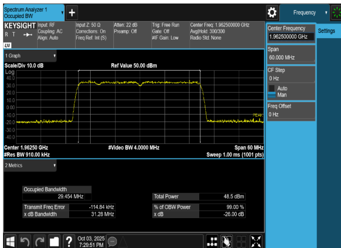
Plot 8-33. Occupied Bandwidth Plot (NR_n25_3C_5M+10M+15M_QPSK - Mid Channel, Port 10)
