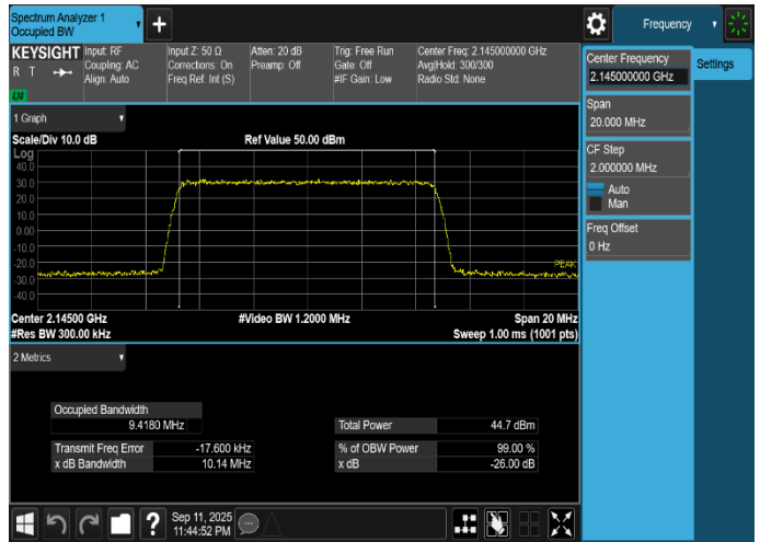
Plot 8-50. Occupied Bandwidth Plot (NR_n66_1C_10M_256QAM - Mid Channel, Port 9)
