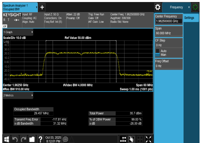
Plot 8-34. Occupied Bandwidth Plot (NR_n25_3C_5M+10M+15M_16QAM - Mid Channel, Port 19)
