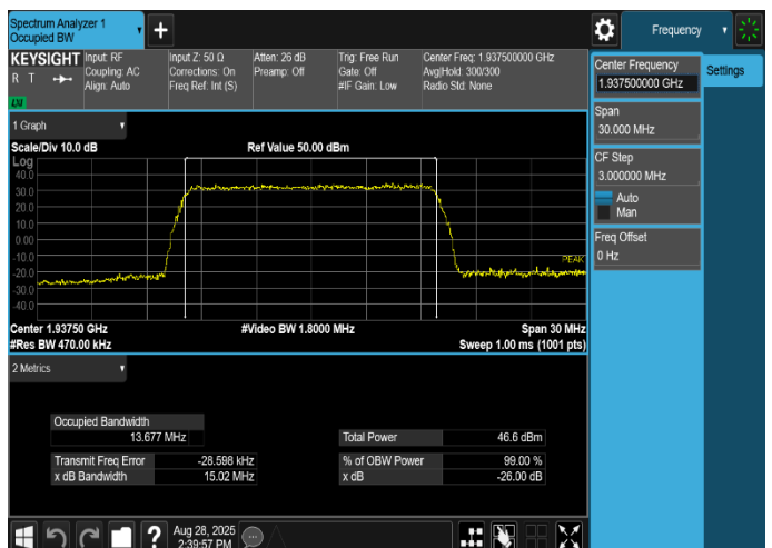
Plot 8-6. Occupied Bandwidth Plot (LTE_B25_1C_15M_256QAM - Low Channel, Port 1)
