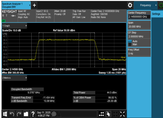
Plot 8-49. Occupied Bandwidth Plot (NR_n66_1C_10M_QPSK - Mid Channel, Port 3)
