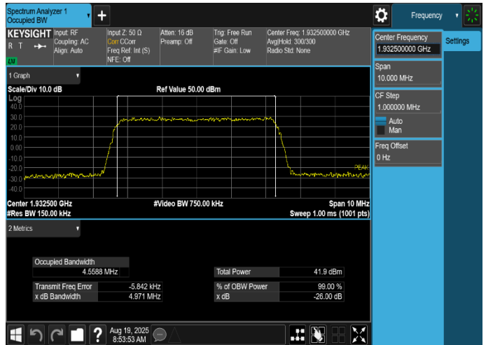
Plot 8-2. Occupied Bandwidth Plot (LTE_B25_1C_5M_64QAM - Low Channel, Port 13)
