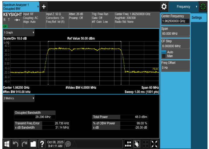
Plot 8-38. Occupied Bandwidth Plot (MSR_B/n25_3C_LTE 10M+NR 10M+DSS 10M_16QAM - Mid Channel, Port 5)
