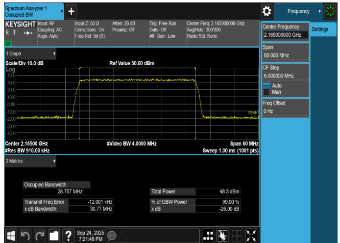
Plot 8-58. Occupied Bandwidth Plot (NR_n66_1C_30M_64QAM - High Channel, Port 0)
