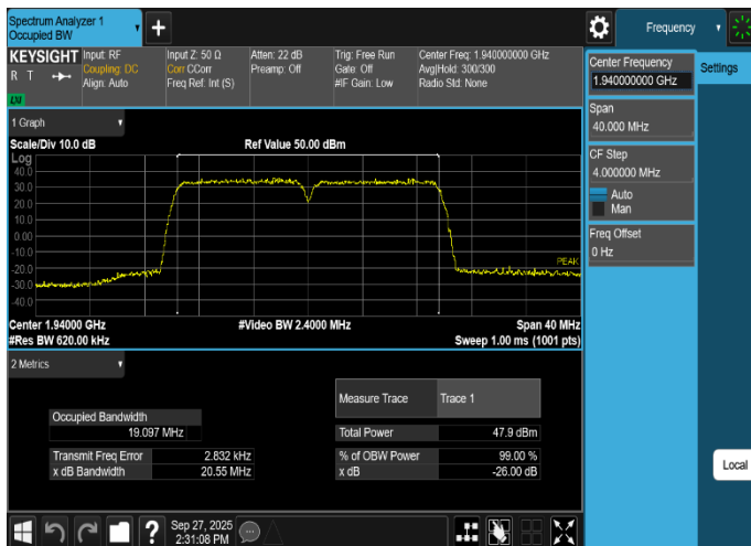
Plot 8-27. Occupied Bandwidth Plot (LTE_B25_2C_10M+10M_QPSK - Low Channel, Port 16)
