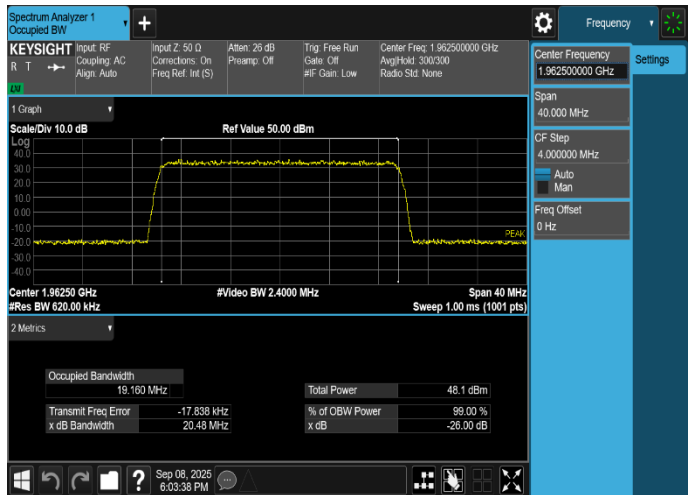
Plot 8-16. Occupied Bandwidth Plot (NR_n25_1C_20M_256QAM - Mid Channel, Port 23)
