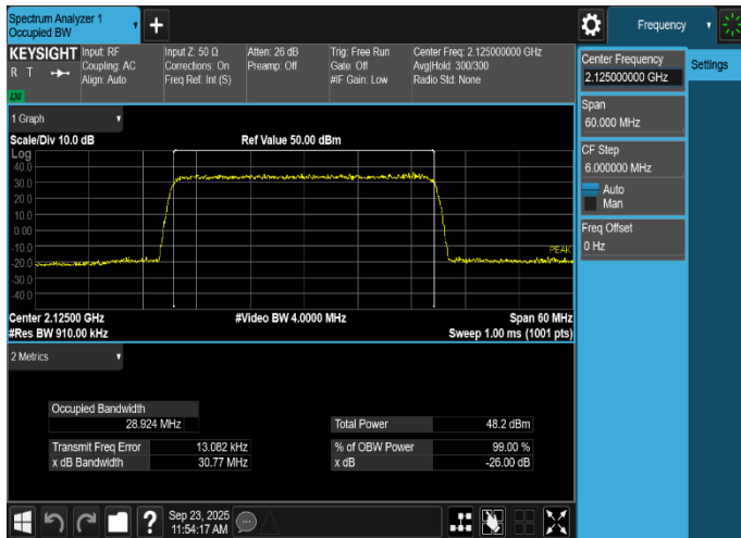
Plot 8-57. Occupied Bandwidth Plot (NR_n66_1C_30M_QPSK - Low Channel, Port 29)
