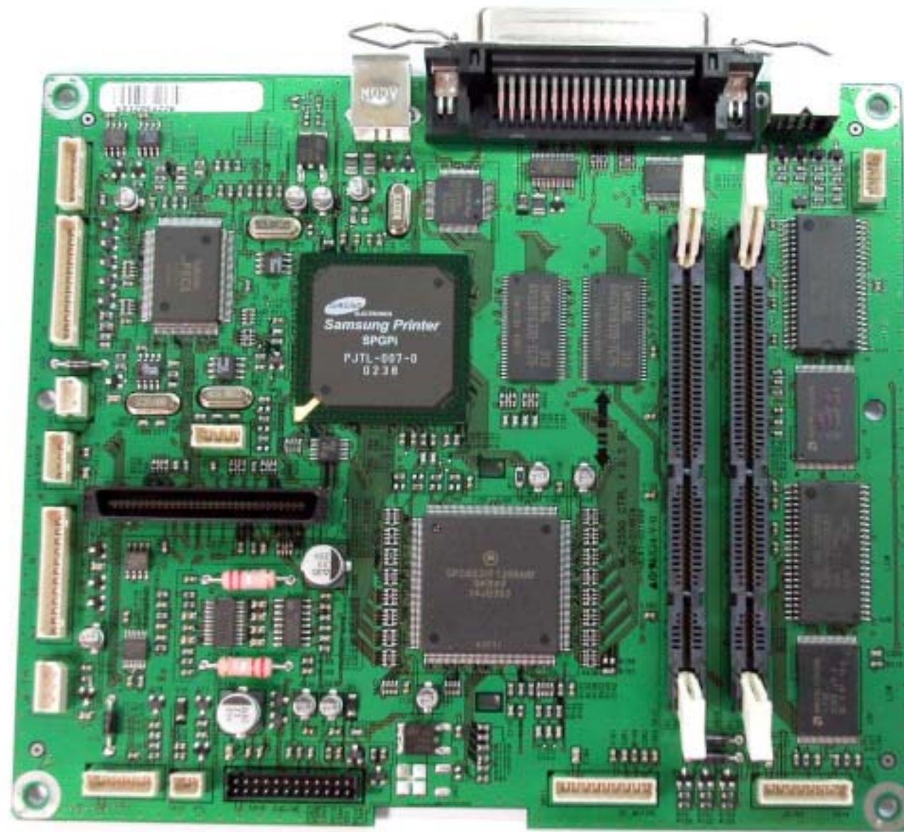
Top View of Main Controller
