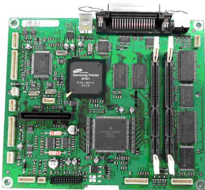
Mainboard Front (Before)
