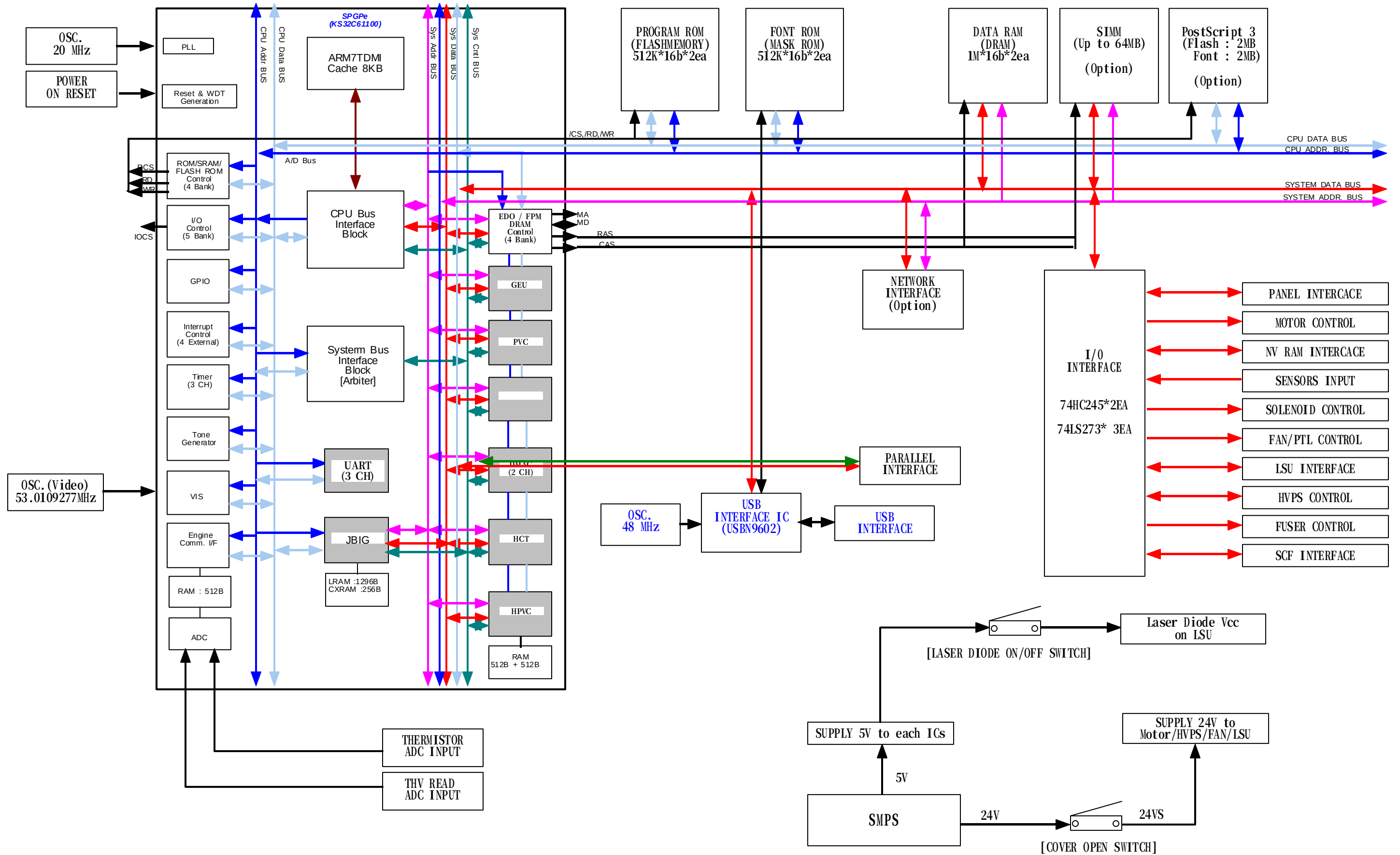
[ ML-1450/1451N Block Diagram ]
