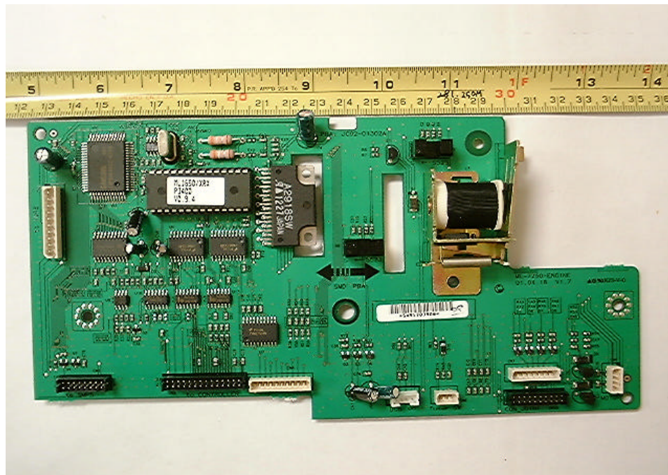
Solder view of Engine b'd
