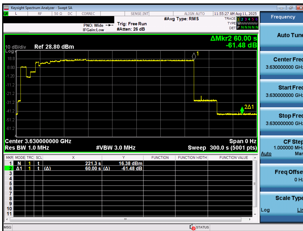
Plot 12. Conducted Measurement – RF transmission stops within 60s of SAS heartbeat response (Marker 1) (WINNF.FT.C.HBT.4)
