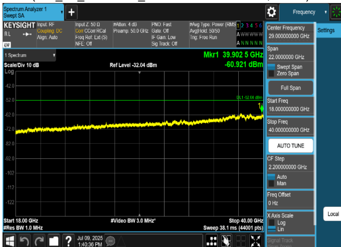
Plot 8-84. Conducted Spurious Emission Plot 18 GHz to 40 GHz (n48_2C_20M+30M_64QAM - Low Channel, Port 2)
