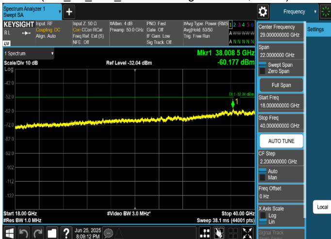
Plot 8-89. Conducted Spurious Emission Plot 18 GHz to 40 GHz (n48_1C_60M_256QAM - High Channel, Port 2)
