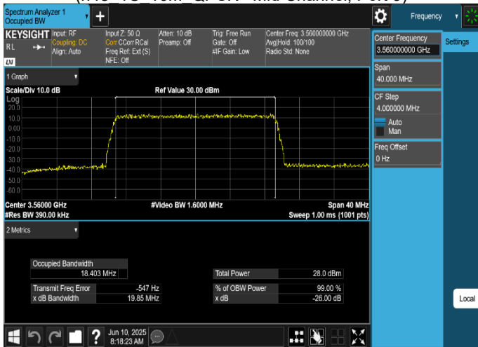
Plot 8-3. Occupied Bandwidth Plot (n48 1C 20M QPSK - Low Channel, Port 5)
