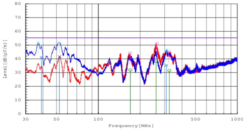
Plot 8-133. Radiated spurious emission Plot_30 MHz to 1000 MHz (Multi-Band_n48_4C_20M+20M+20M+20M+n77_2C_100M+100M)
