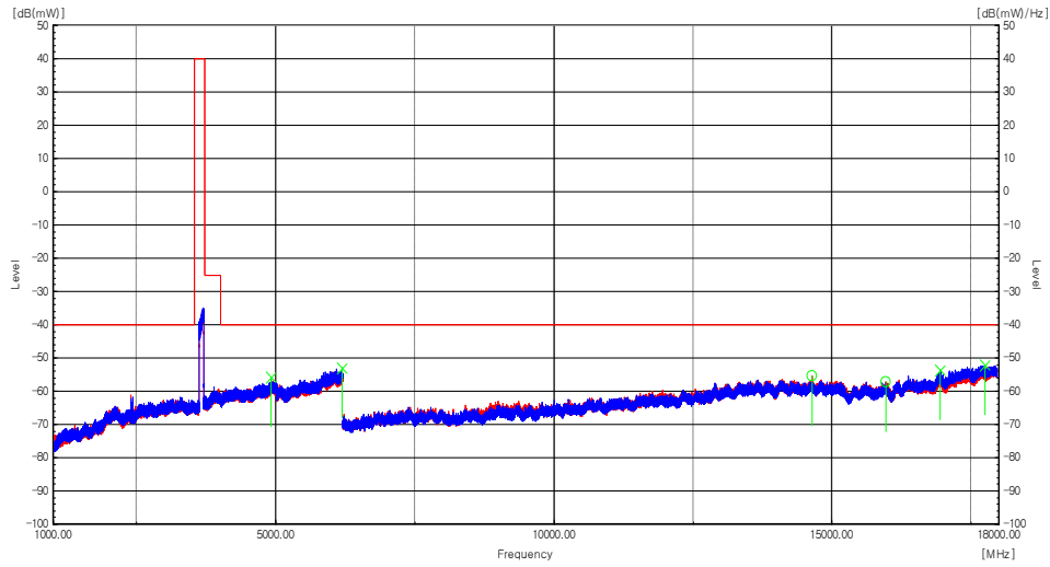
Plot 8-143. Radiated spurious emission Plot_1 GHz to 18 GHz (n48_1C_80M_High Channel)
