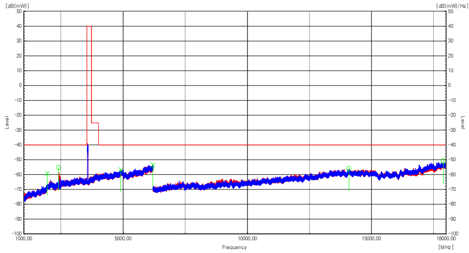
Plot 8-137. Radiated spurious emission Plot_1 GHz to 18 GHz (n48_1C_40M_Low Channel)
