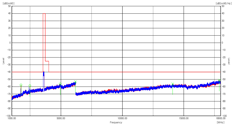
Plot 8-141. Radiated spurious emission Plot_1 GHz to 18 GHz (n48_1C_80M_Low Channel)
