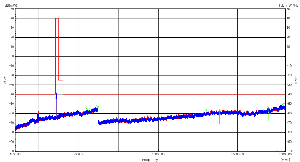
Plot 8-139. Radiated spurious emission Plot_1 GHz to 18 GHz (n48_1C_60M_Low Channel)
