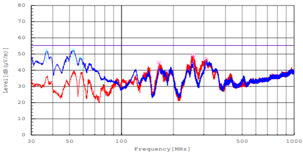
Plot 8-132. Radiated spurious emission Plot_30 MHz to 1000 MHz (n48_1C_80M_High Channel)
