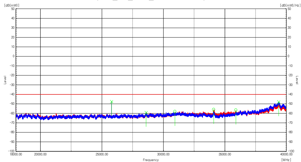
Plot 8-150. Radiated spurious emission Plot_18 GHz to 40 GHz (n48_1C_80M_High Channel)
