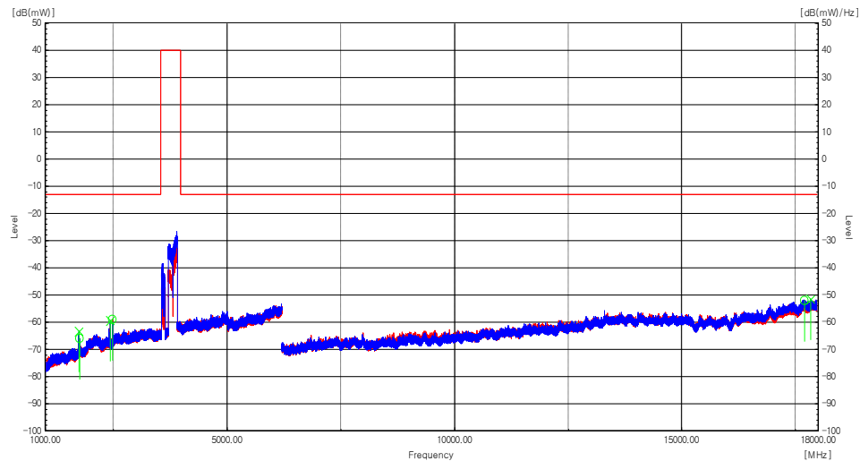
Plot 8-147. Radiated spurious emission Plot_1 GHz to 18 GHz (Multi -Band_n48_4C_20M+20M+20M+20M + n77_2C_100M+100M)
