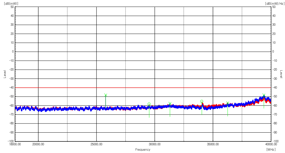
Plot 8-148. Radiated spurious emission Plot_18 GHz to 40 GHz (n48_1C_80M_Low Channel)
