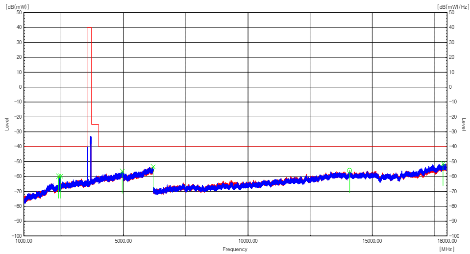
Plot 8-144. Radiated spurious emission Plot_1 GHz to 18 GHz (n48_2NC_20M+30M_Mid Channel)
