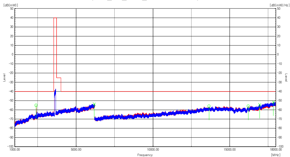
Plot 8-142. Radiated spurious emission Plot_1 GHz to 18 GHz (n48_1C_80M_Mid Channel)
