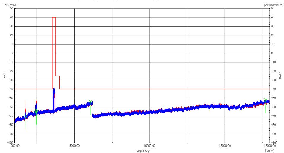
Plot 8-145. Radiated spurious emission Plot_1 GHz to 18 GHz (n48_4NC_10M+10M+10M+40M_Mid Channel)
