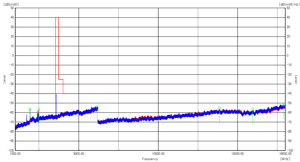
Plot 8-135. Radiated spurious emission Plot_1 GHz to 18 GHz (n48_1C_20M_Low Channel)
