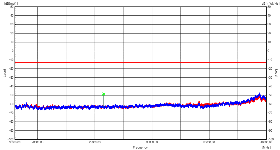
Plot 8-151. Radiated spurious emission Plot_18 GHz to 40 GHz (Multi-Band_n48_4C_20M+20M+20M+20M + n77_2C_100M+100M)
