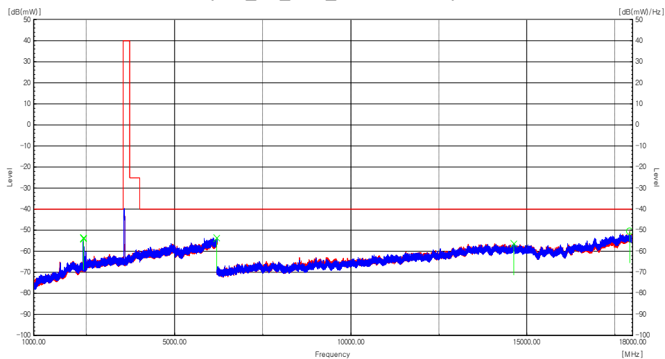
Plot 8-136. Radiated spurious emission Plot_1 GHz to 18 GHz (n48_1C_30M_Low Channel)
