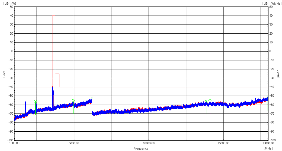
Plot 8-140. Radiated spurious emission Plot_1 GHz to 18 GHz (n48_4C_10M+10M+10M+40M_Low Channel)
