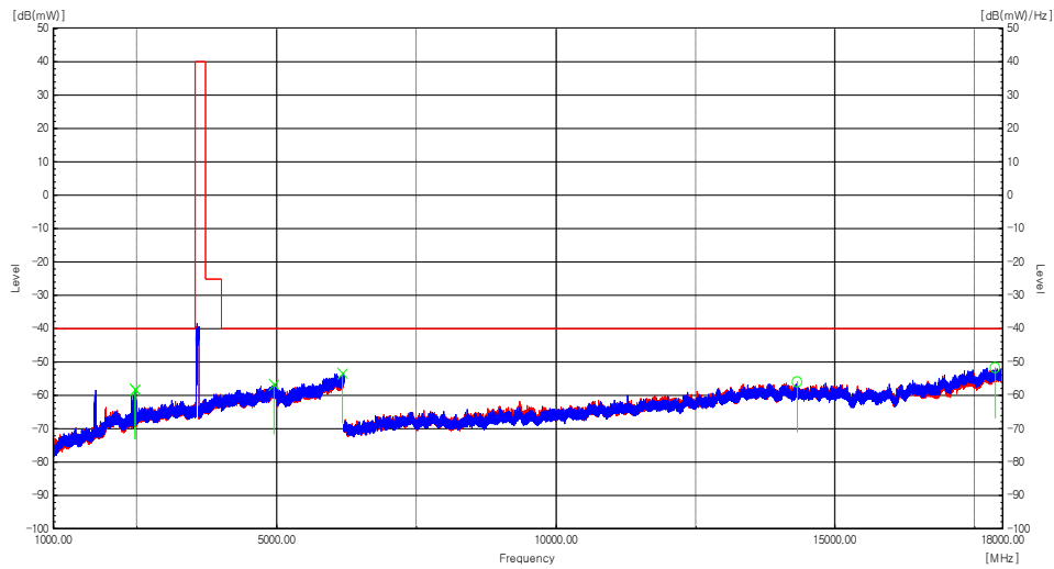
Plot 8-138. Radiated spurious emission Plot_1 GHz to 18 GHz (n48_2C_20M+30M_Low Channel)
