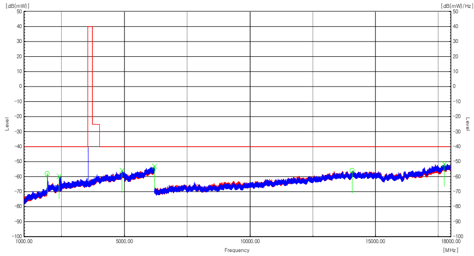
Plot 8-134. Radiated spurious emission Plot_1 GHz to 18 GHz (n48_1C_10M_Low Channel)
