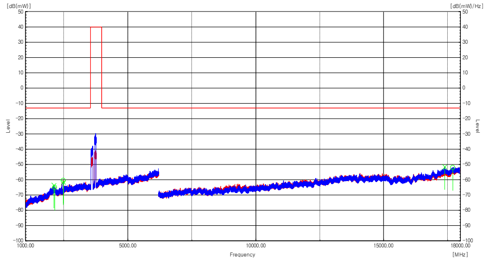
Plot 8-146. Radiated spurious emission Plot_1 GHz to 18 GHz (Multi -Band_n48_1C_80M + n77_1C_60M)
