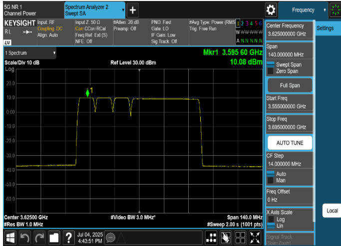
Plot 8-27. Power Spectral Density Plot (n48_4C_10M+10M+10M+40M_QPSK – Mid Channel, Port 6)
