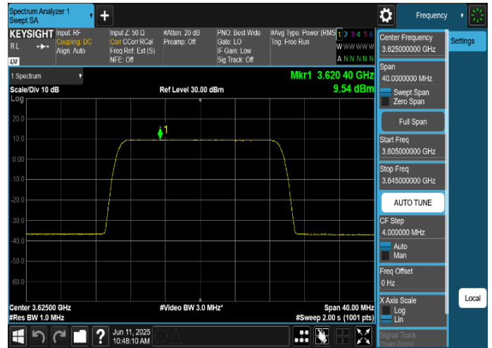
Plot 8-22. Power Spectral Density Plot (n48_1C_20M_16QAM – Mid Channel, Port 6)
