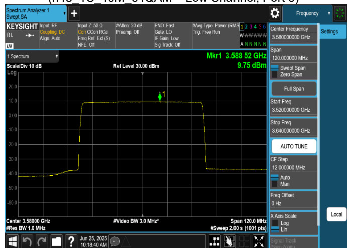
Plot 8-26. Power Spectral Density Plot (n48_1C_60M_64QAM – Low Channel, Port 6)
