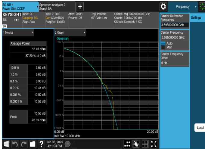
Plot 8-37. Peak To Average Power Ratio Plot (n48_1C_10M_16QAM - High Channel, Port 10)
