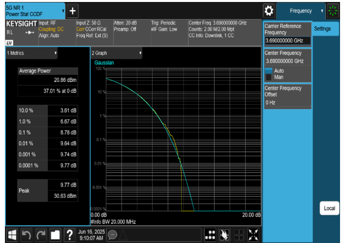
Plot 8-38. Peak To Average Power Ratio Plot (n48_1C_20M_16QAM - High Channel, Port 12)
