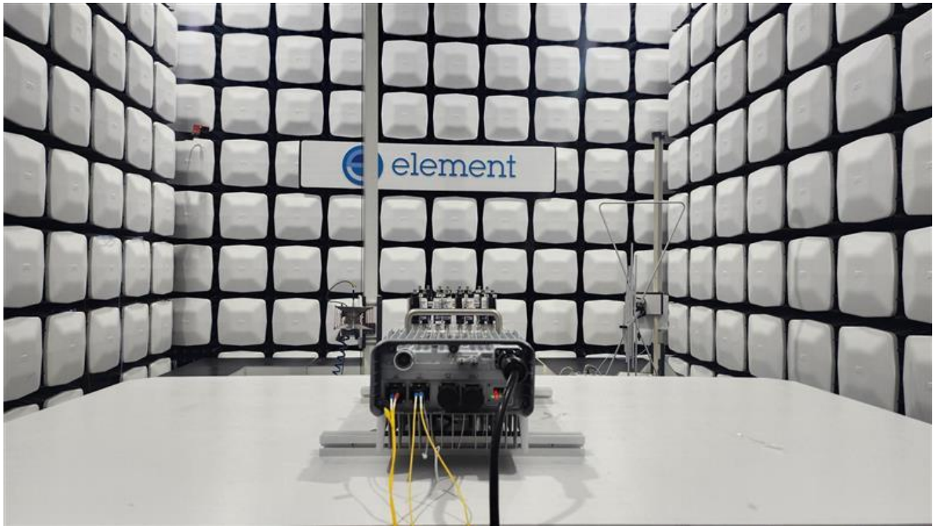
Above 1GHz radiated Test Instrument & Measurement Setup
