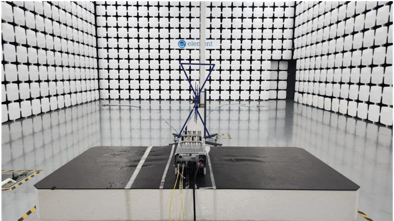
Below 1GHz radiated Test Instrument & Measurement Setup
