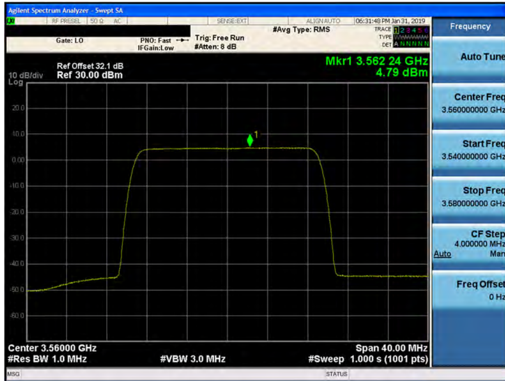
Plot 7-143. Peak Power Spectral Density Plot (1CC- 3560 MHz- 20.0MHz 256QAM- Low Channel) Port 26
