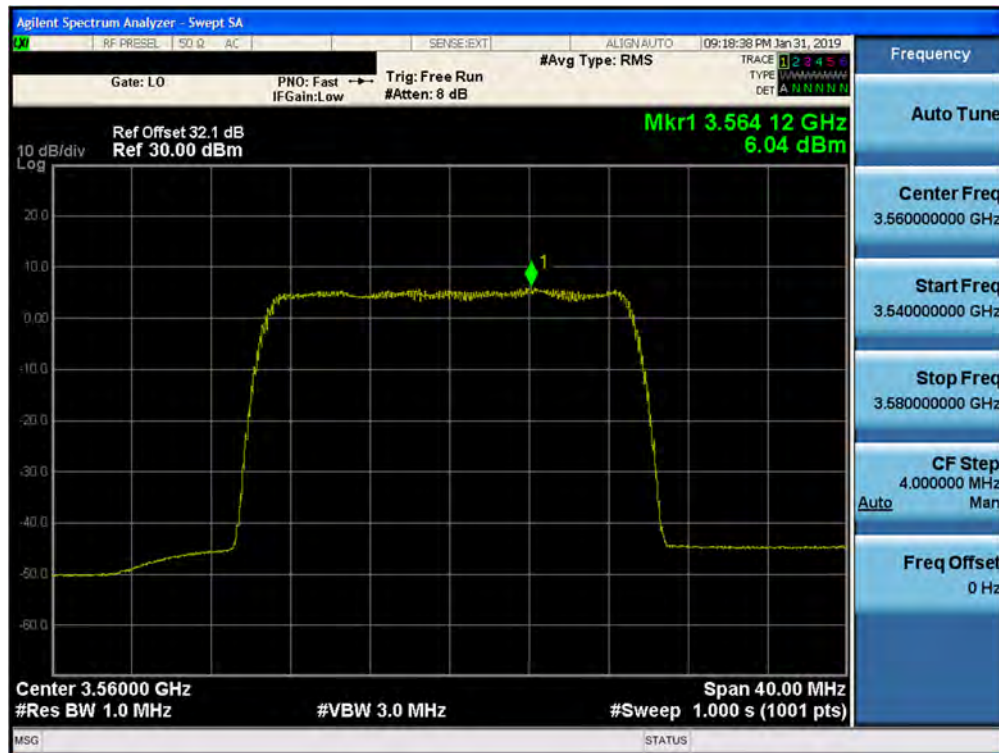
Plot 7-84. Peak Power Spectral Density Plot (1CC- 3560 MHz- 20.0MHz 16QAM- Low Channel) Port 12
