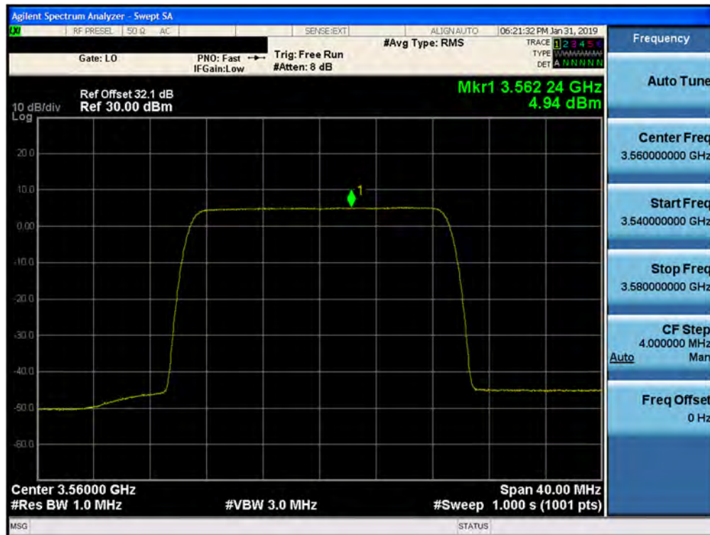
Plot 7-114. Peak Power Spectral Density Plot (1CC- 3560 MHz- 20.0MHz 64QAM- Low Channel) Port 14
