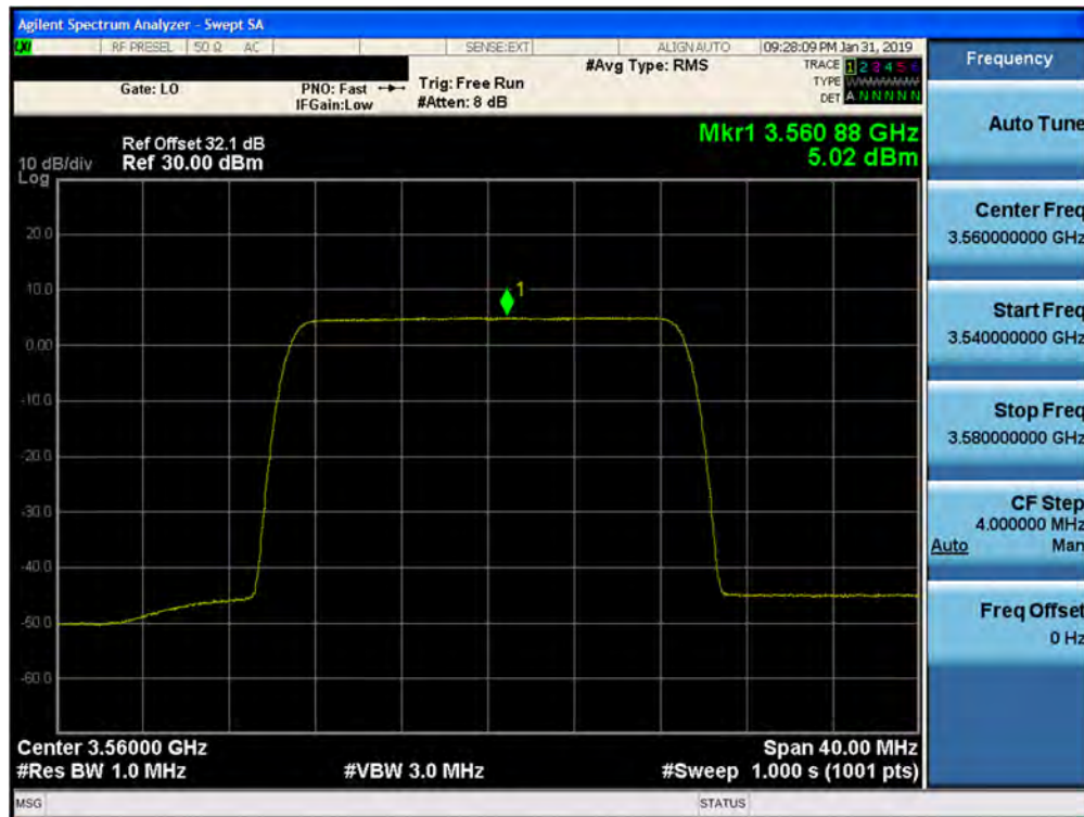
Plot 7-108. Peak Power Spectral Density Plot (1CC- 3560 MHz- 20.0MHz 64QAM- Low Channel) Port 08
