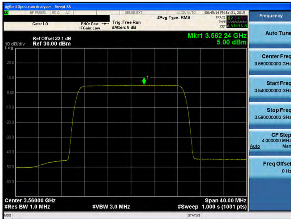
Plot 7-130. Peak Power Spectral Density Plot (1CC- 3560 MHz- 20.0MHz 256QAM- Low Channel) Port 06
