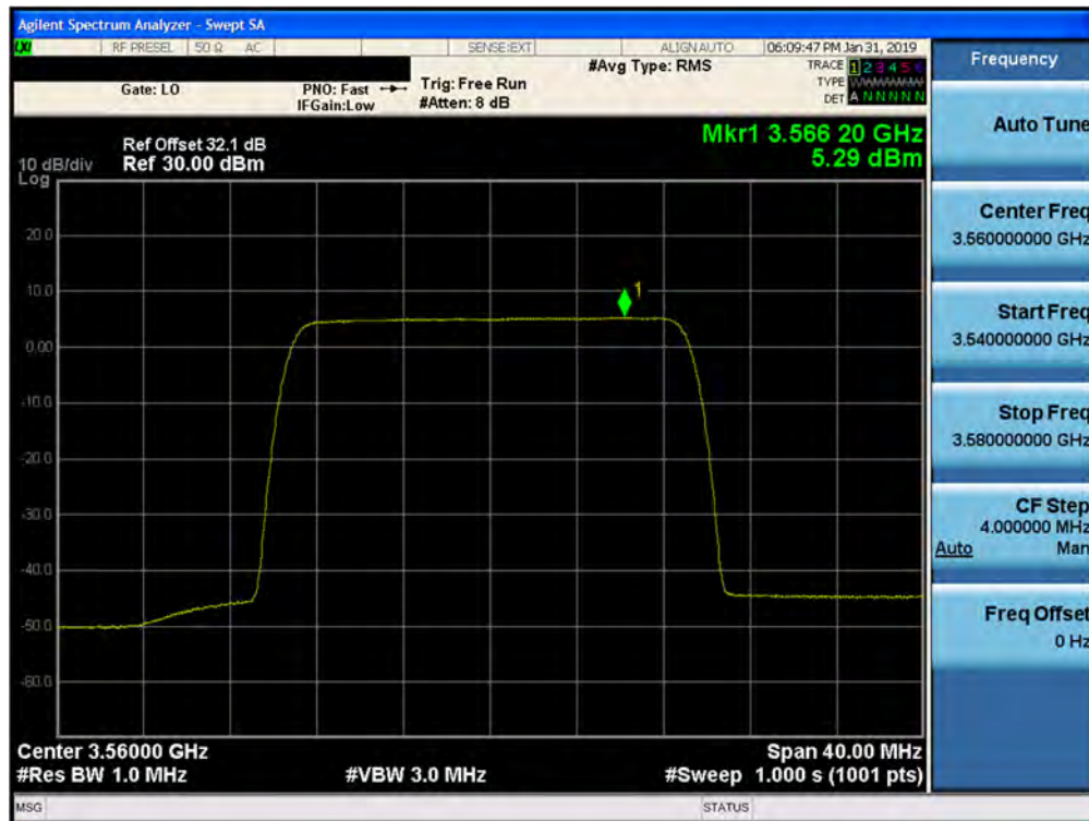
Plot 7-120. Peak Power Spectral Density Plot (1CC- 3560 MHz- 20.0MHz 64QAM- Low Channel) Port 31
