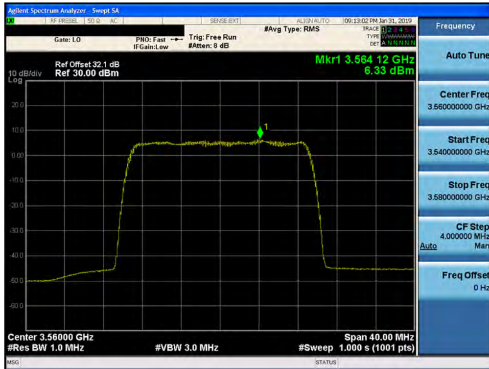
Plot 7-85. Peak Power Spectral Density Plot (1CC– 3560 MHz- 20.0MHz 16QAM- Low Channel) Port 28
