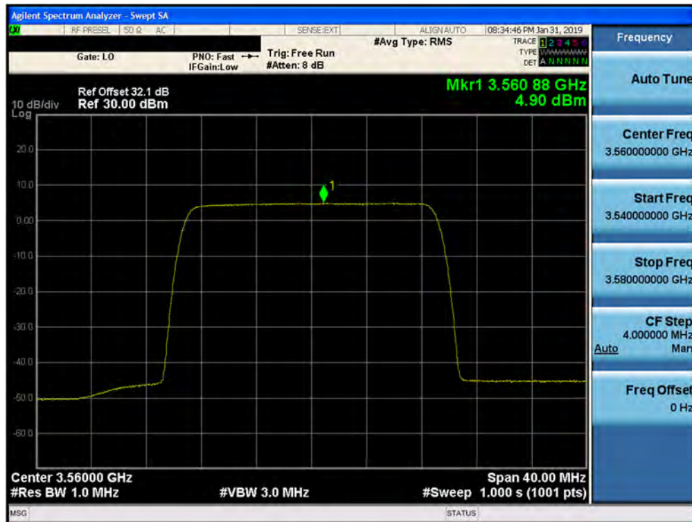
Plot 7-94. Peak Power Spectral Density Plot (1CC- 3560 MHz- 20.0MHz 64QAM- Low Channel) Port 17
