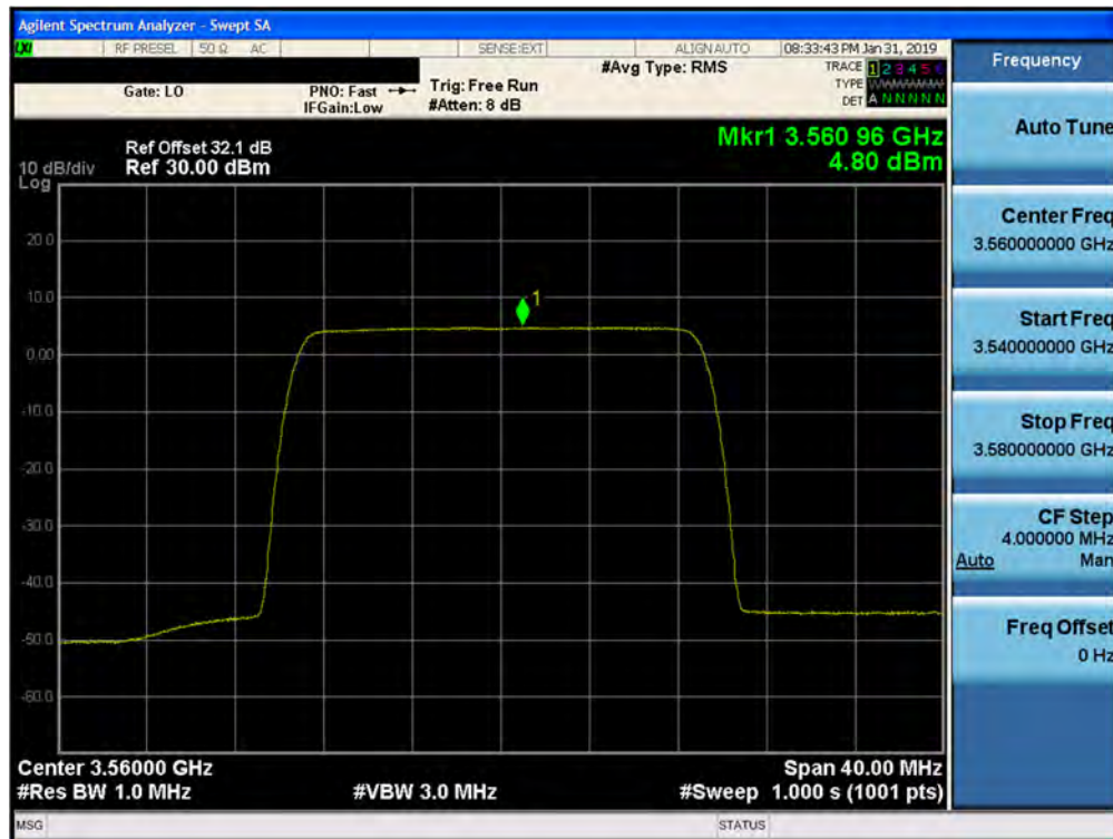
Plot 7-126. Peak Power Spectral Density Plot (1CC- 3560 MHz- 20.0MHz 256QAM- Low Channel) Port 17
