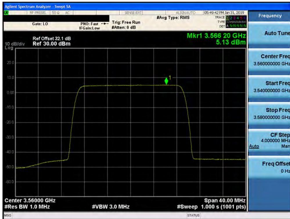
Plot 7-112. Peak Power Spectral Density Plot (1CC- 3560 MHz- 20.0MHz 64QAM- Low Channel) Port 27
