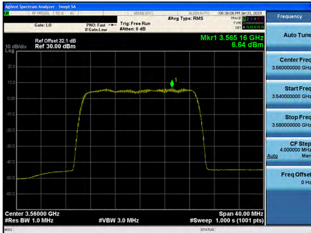
Plot 7-74. Peak Power Spectral Density Plot (1CC– 3560 MHz- 20.0MHz 16QAM- Low Channel) Port 10
