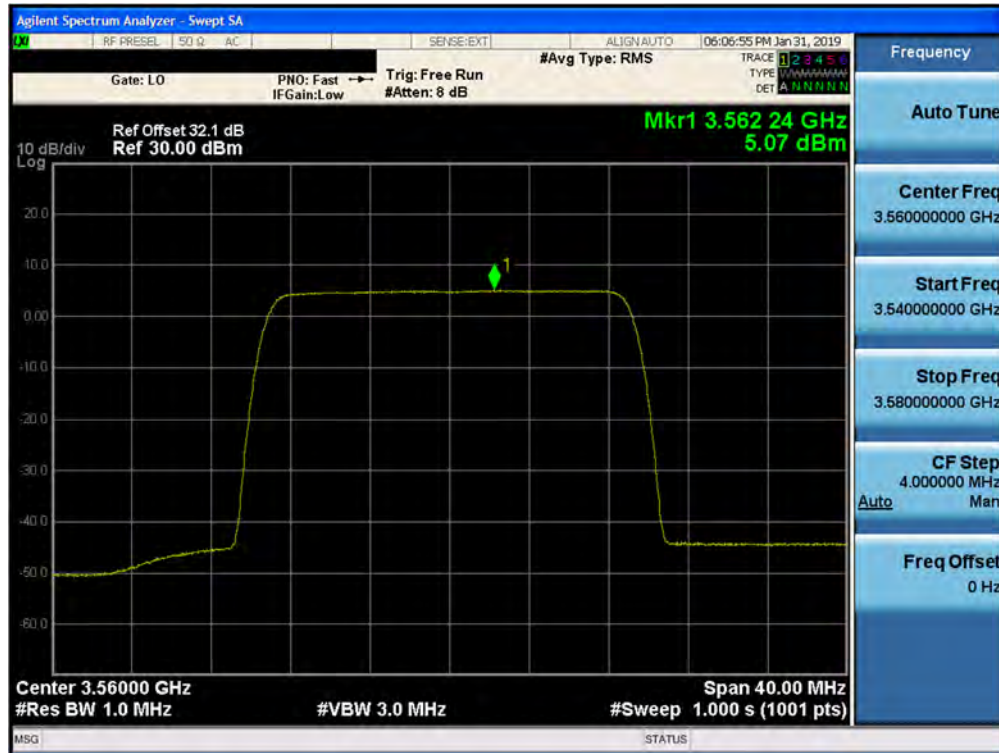
Plot 7-145. Peak Power Spectral Density Plot (1CC– 3560 MHz- 20.0MHz 256QAM- Low Channel) Port 15
