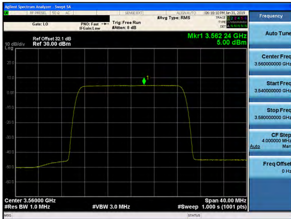
Plot 7-146. Peak Power Spectral Density Plot (1CC– 3560 MHz- 20.0MHz 256QAM- Low Channel) Port 14
