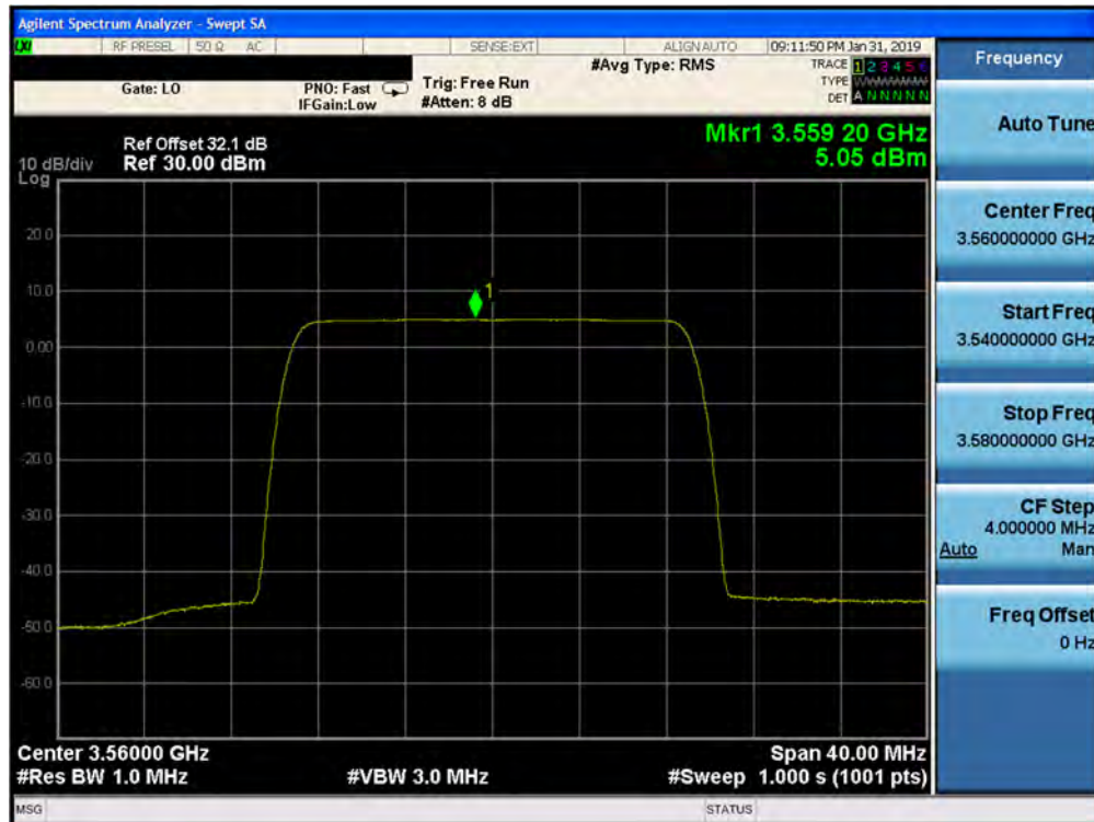
Plot 7-53. Peak Power Spectral Density Plot (1CC- 3560 MHz- 20.0MHz QPSK- Low Channel) Port 28
