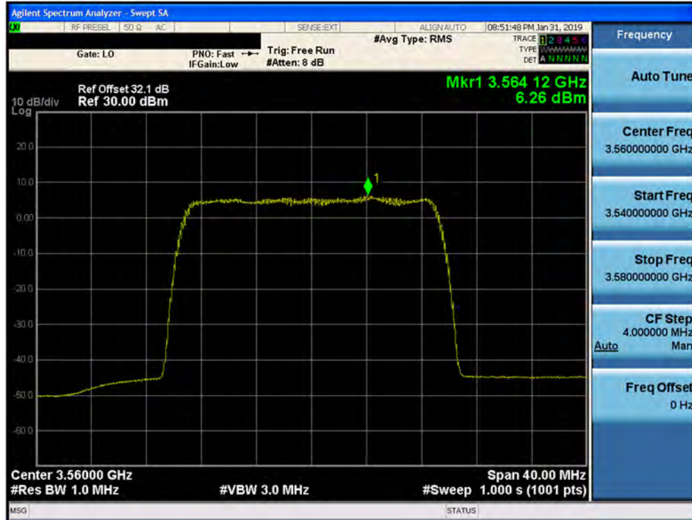
Plot 7-75. Peak Power Spectral Density Plot (1CC- 3560 MHz- 20.0MHz 16QAM- Low Channel) Port 09
