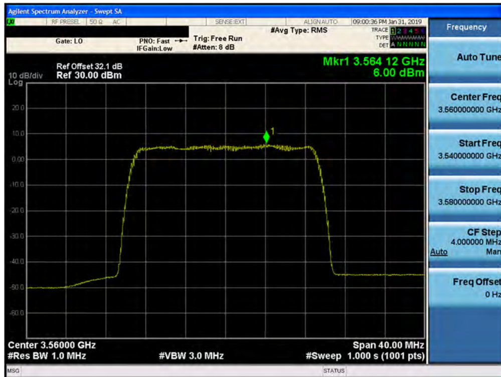
Plot 7-78. Peak Power Spectral Density Plot (1CC- 3560 MHz- 20.0MHz 16QAM- Low Channel) Port 25
