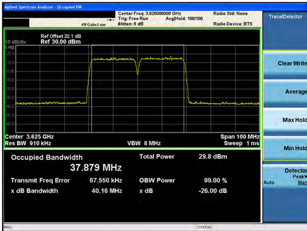
Plot 7-20. Occupied Bandwidth Plot(CC Configuration–3625 MHz - 40.0MHz 64QAM- Mid Channel)
