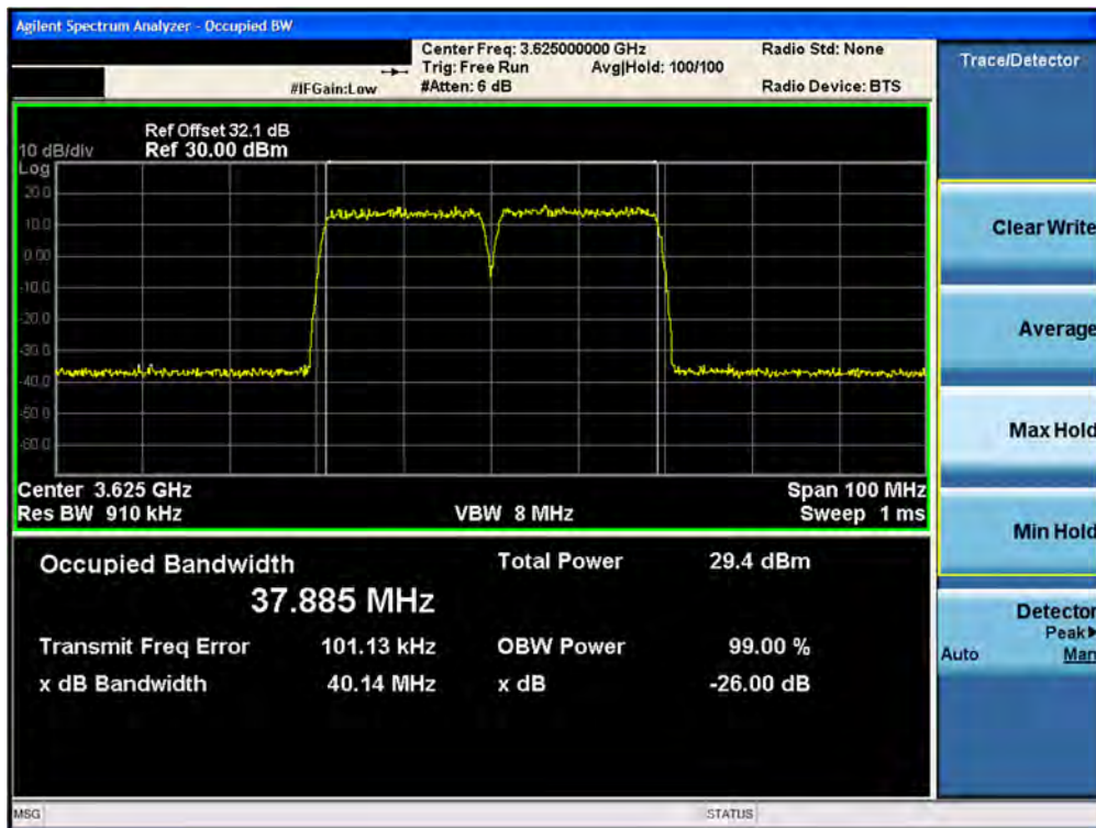
Plot 7-14. Occupied Bandwidth Plot (2CC Configuration– 3625 MHz - 40.0MHz QPSK- Mid Channel)
