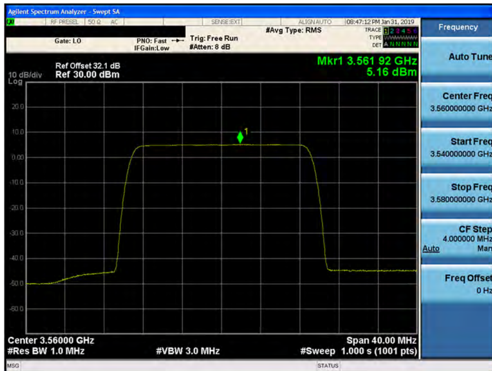
Plot 7-38. Peak Power Spectral Density Plot (1CC- 3560 MHz- 20.0MHz QPSK- Low Channel) Port 21
