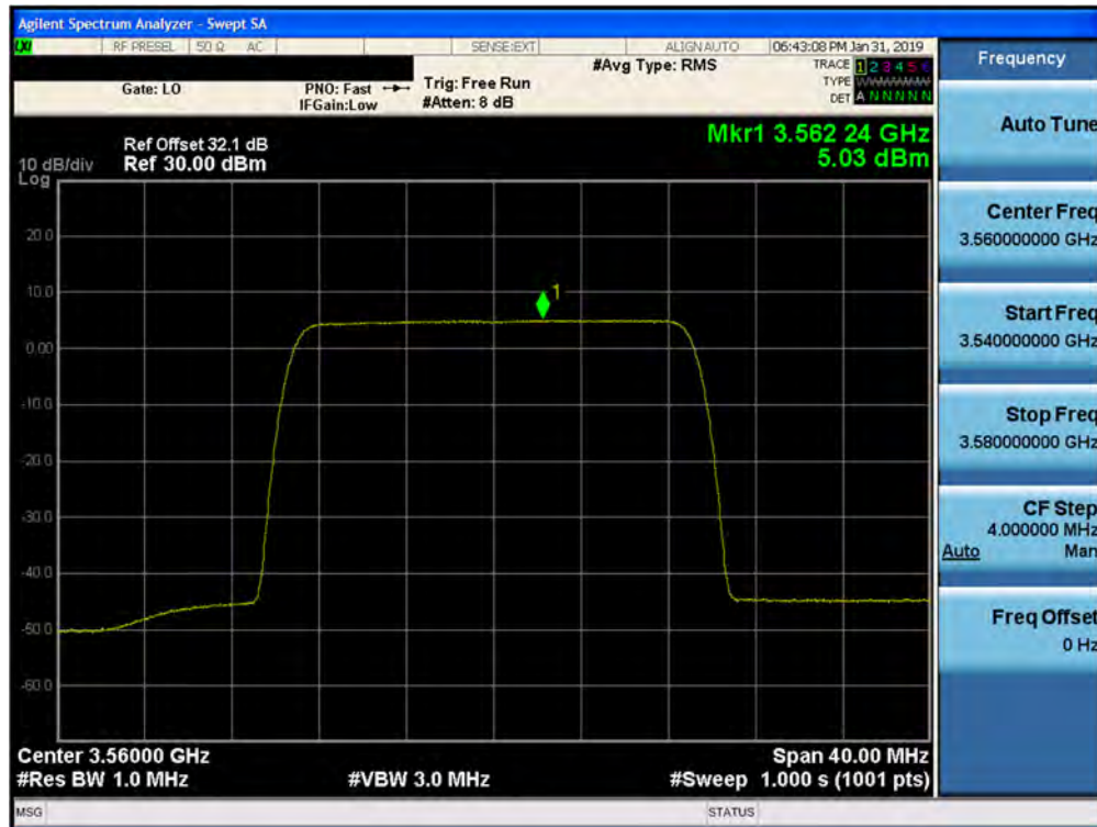
Plot 7-135. Peak Power Spectral Density Plot (1CC- 3560 MHz- 20.0MHz 256QAM- Low Channel) Port 22
