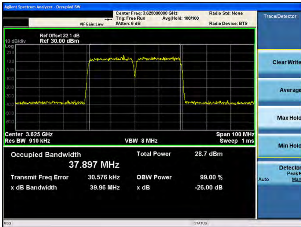
Plot 7-17. Occupied Bandwidth Plot(2CC Configuration– 3625 MHz- 40.0MHz 16QAM- Mid Channel)
