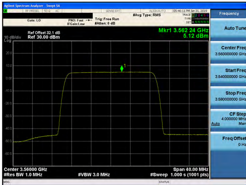
Plot 7-144. Peak Power Spectral Density Plot (1CC- 3560 MHz- 20.0MHz 256QAM- Low Channel) Port 27
