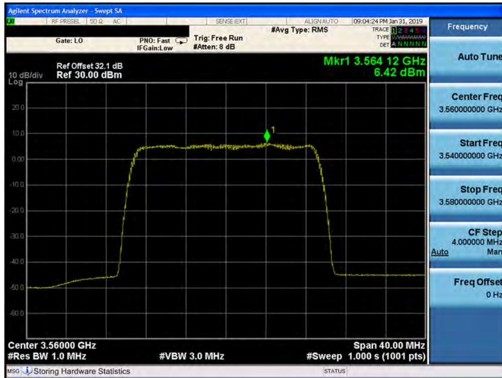
Plot 7-83. Peak Power Spectral Density Plot (1CC- 3560 MHz- 20.0MHz 16QAM- Low Channel) Port 13
