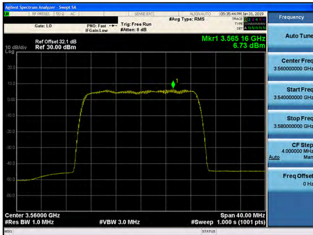
Plot 7-72. Peak Power Spectral Density Plot (1CC– 3560 MHz- 20.0MHz 16QAM- Low Channel) Port 23
