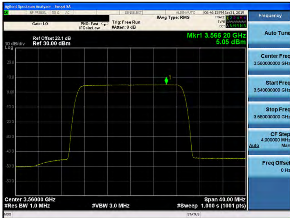
Plot 7-98. Peak Power Spectral Density Plot (1CC- 3560 MHz- 20.0MHz 64QAM- Low Channel) Port 06
