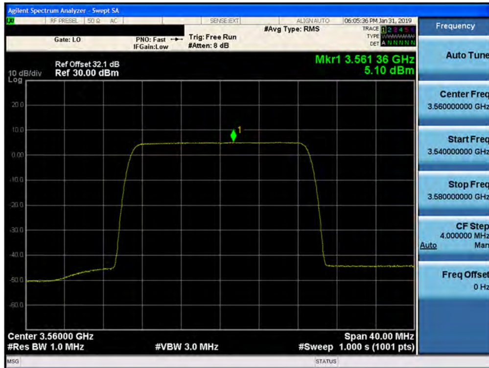
Plot 7-113. Peak Power Spectral Density Plot (1CC- 3560 MHz- 20.0MHz 64QAM- Low Channel) Port 15
