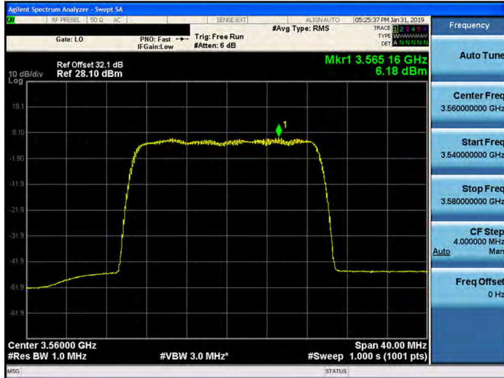
Plot 7-65. Peak Power Spectral Density Plot (1CC- 3560 MHz- 20.0MHz 16QAM- Low Channel) Port 07
