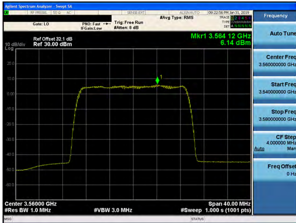
Plot 7-77. Peak Power Spectral Density Plot (1CC- 3560 MHz- 20.0MHz 16QAM- Low Channel) Port 24
