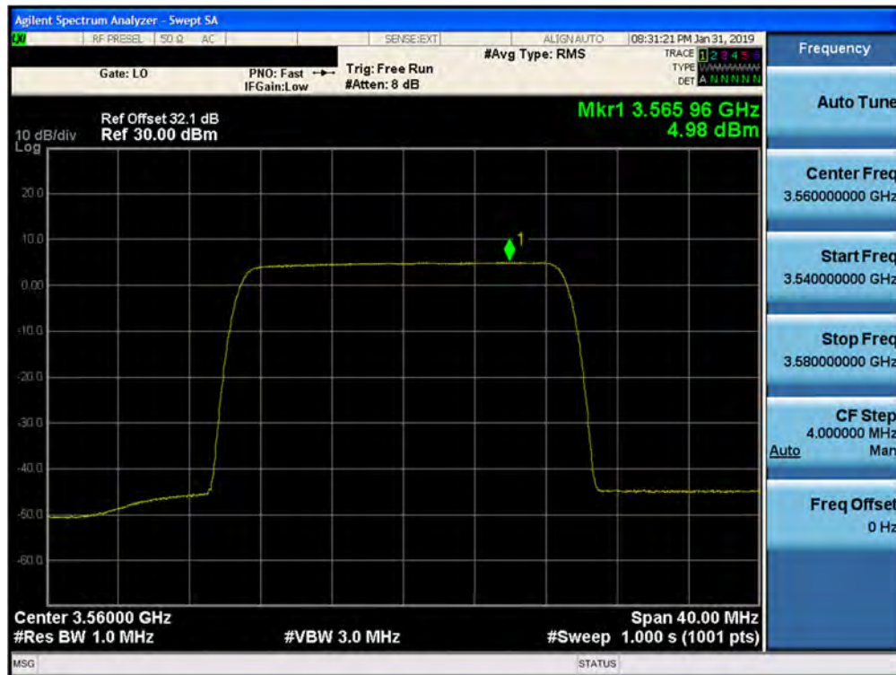
Plot 7-91. Peak Power Spectral Density Plot (1CC– 3560 MHz- 20.0MHz 64QAM- Low Channel) Port 01
