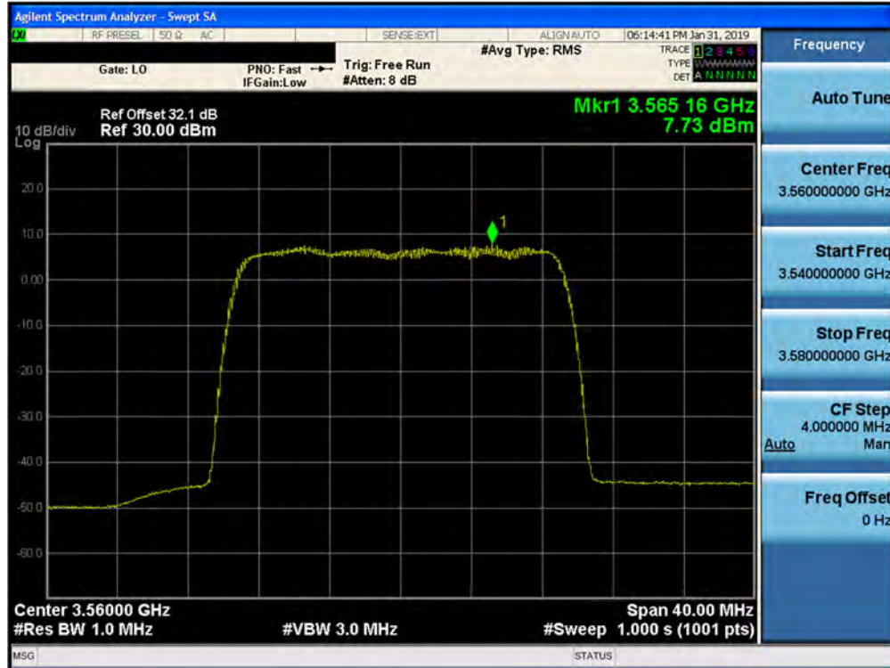
Plot 7-87. Peak Power Spectral Density Plot (1CC- 3560 MHz- 20.0MHz 16QAM- Low Channel) Port 30
