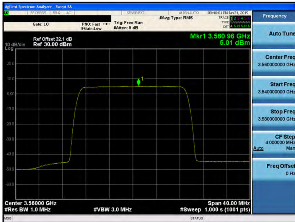
Plot 7-132. Peak Power Spectral Density Plot (1CC- 3560 MHz- 20.0MHz 256QAM- Low Channel) Port 04
