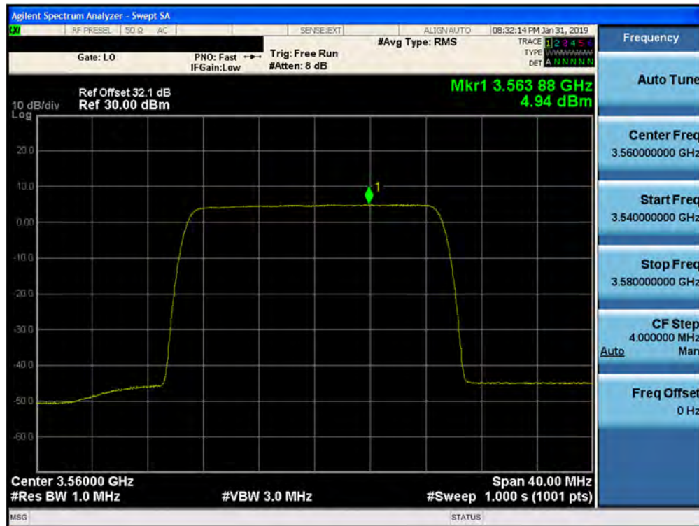
Plot 7-123. Peak Power Spectral Density Plot (1CC– 3560 MHz- 20.0MHz 256QAM- Low Channel) Port 01
