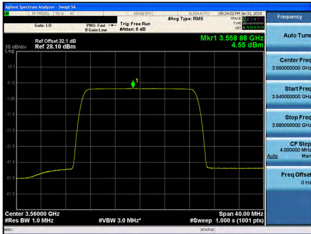
Plot 7-33. Peak Power Spectral Density Plot (1CC- 3560 MHz- 20.0MHz QPSK- Low Channel) Port 07
