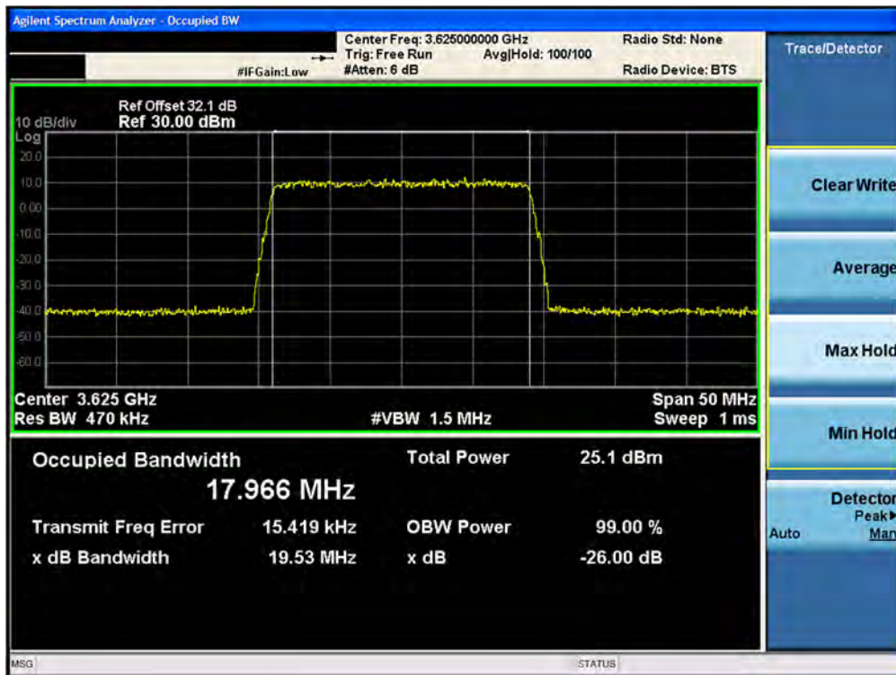
Plot 7-8. Occupied Bandwidth Plot(1CC Configuration–3625 MHz - 20.0MHz 64QAM- Mid Channel)
