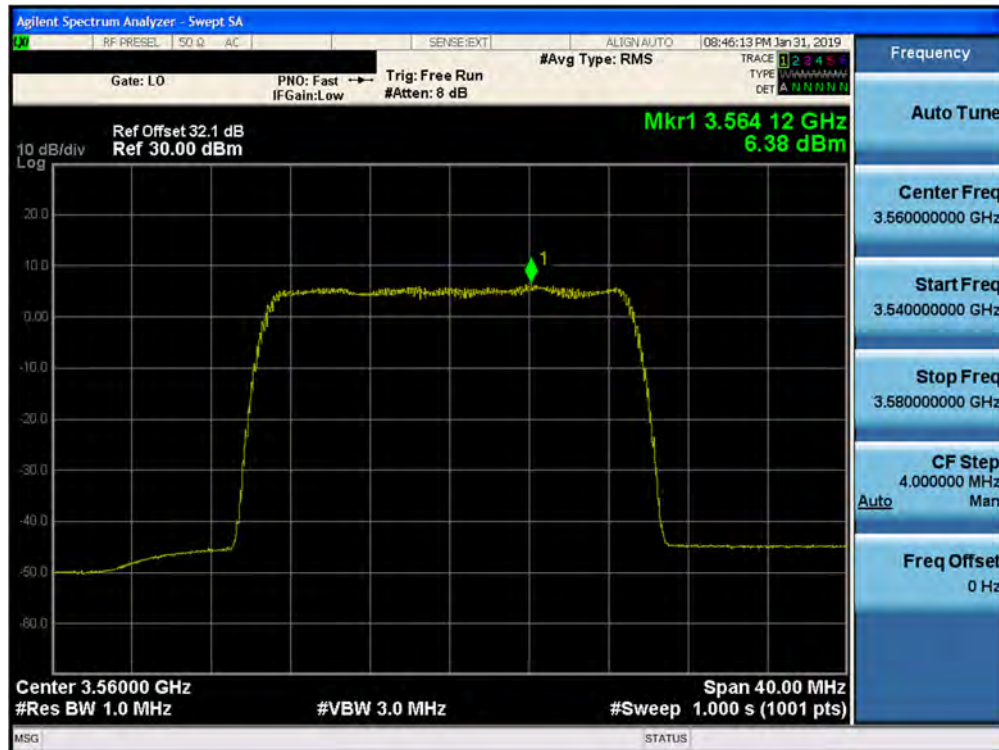
Plot 7-70. Peak Power Spectral Density Plot (1CC- 3560 MHz- 20.0MHz 16QAM- Low Channel) Port 21
