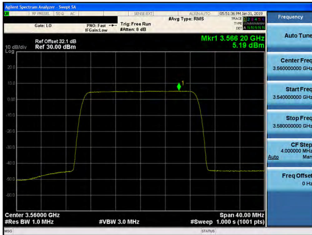
Plot 7-80. Peak Power Spectral Density Plot (1CC- 3560 MHz- 20.0MHz 16QAM- Low Channel) Port 27
