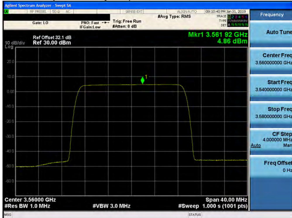
Plot 7-54. Peak Power Spectral Density Plot (1CC- 3560 MHz- 20.0MHz QPSK- Low Channel) Port 29
