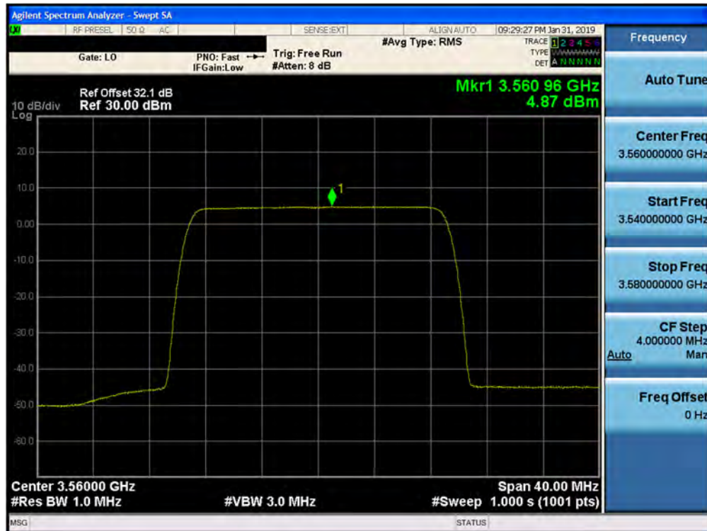
Plot 7-140. Peak Power Spectral Density Plot (1CC– 3560 MHz- 20.0MHz 256QAM- Low Channel) Port 08
