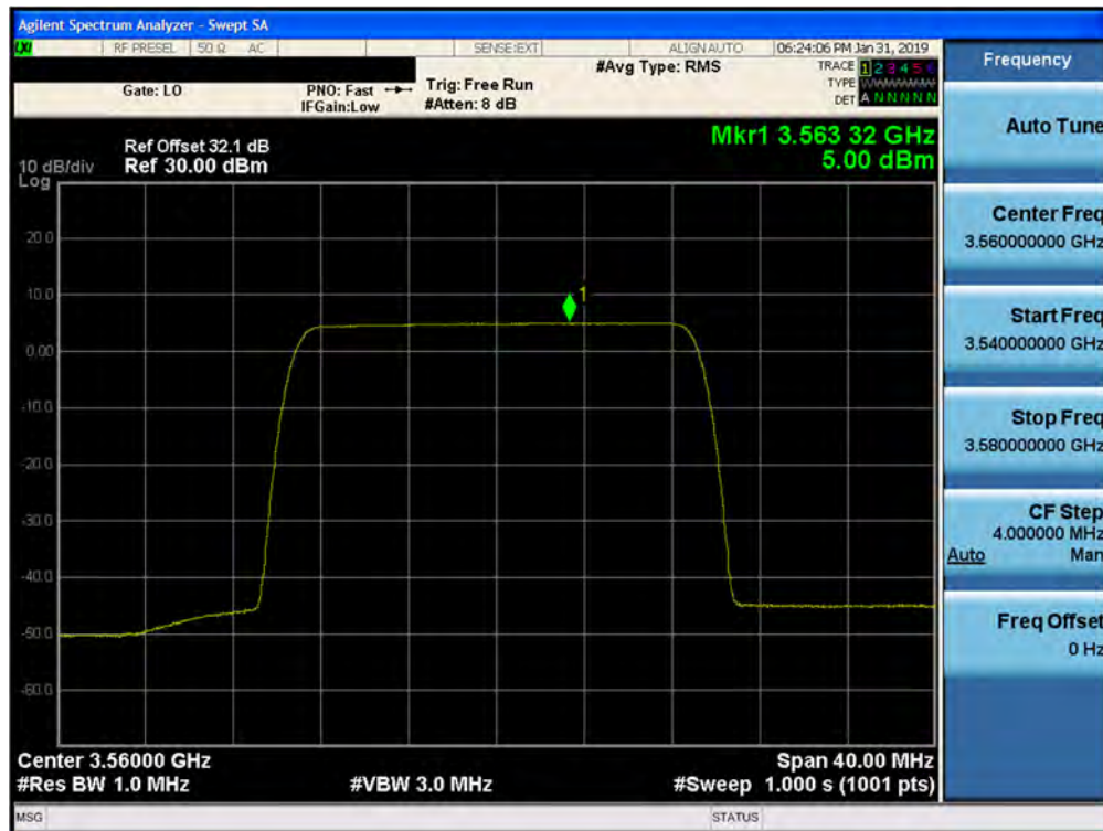
Plot 7-50. Peak Power Spectral Density Plot (1CC- 3560 MHz- 20.0MHz QPSK- Low Channel) Port 14
