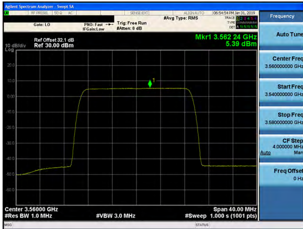
Plot 7-127. Peak Power Spectral Density Plot (1CC- 3560 MHz- 20.0MHz 256QAM- Low Channel) Port 18
