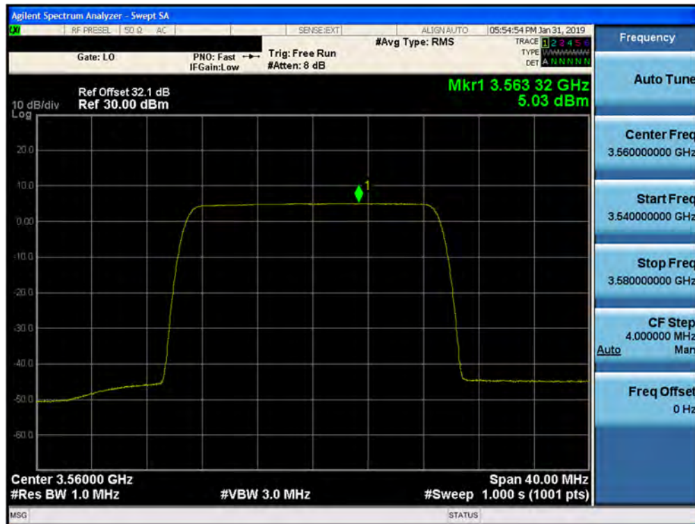
Plot 7-40. Peak Power Spectral Density Plot (1CC- 3560 MHz- 20.0MHz QPSK- Low Channel) Port 23
