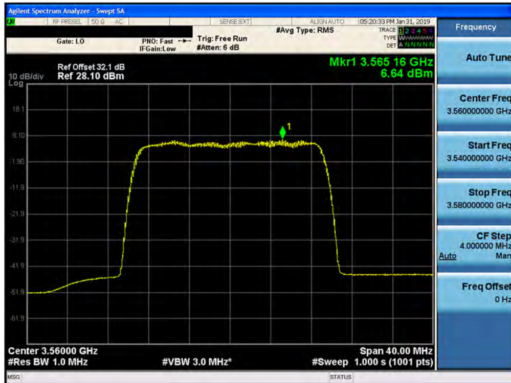
Plot 7-64. Peak Power Spectral Density Plot (1CC– 3560 MHz- 20.0MHz 16QAM- Low Channel) Port 19
