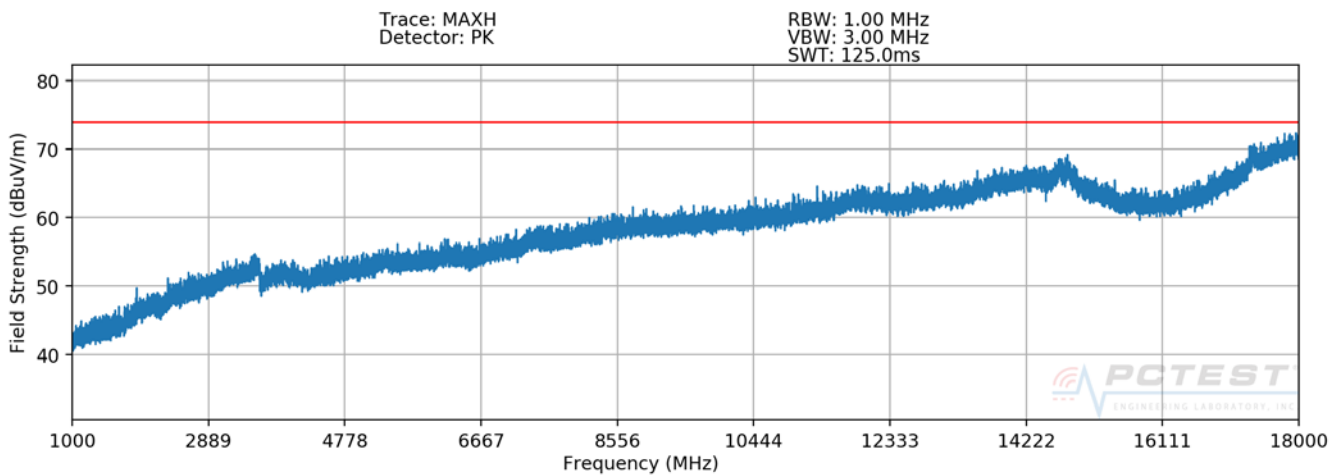
Plot 7-3. Radiated Spurious Plot above 1GHz [Ant. V Orientation]
