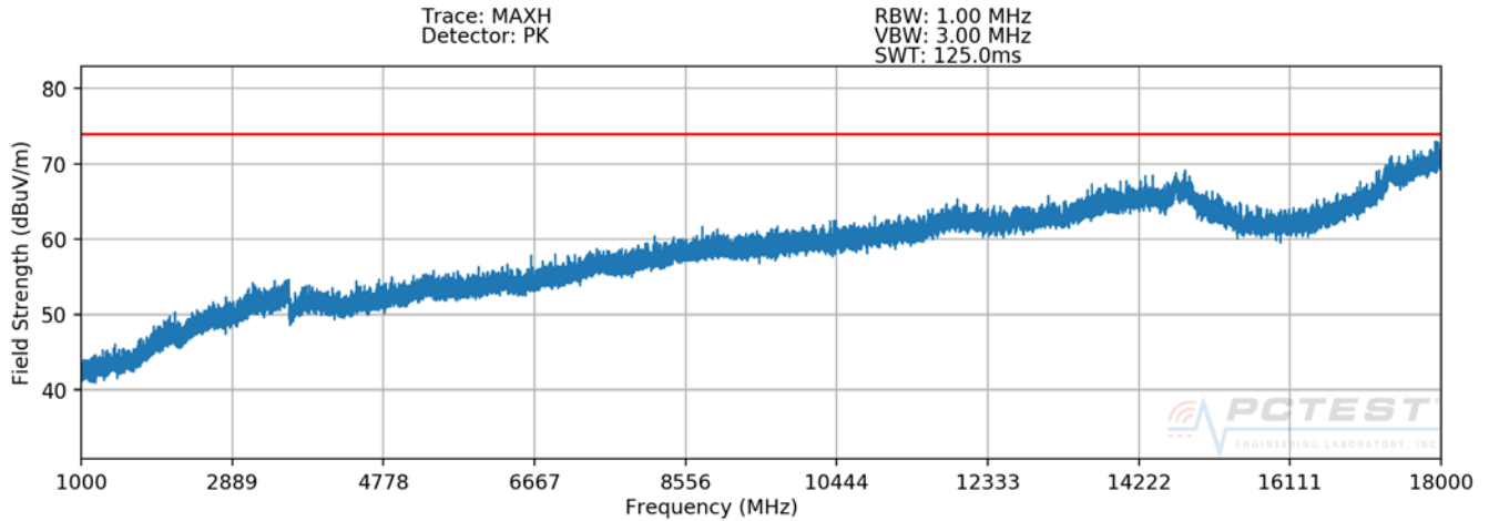
Plot 7-2. Radiated Spurious Plot above 1GHz [Ant. H Orientation]
