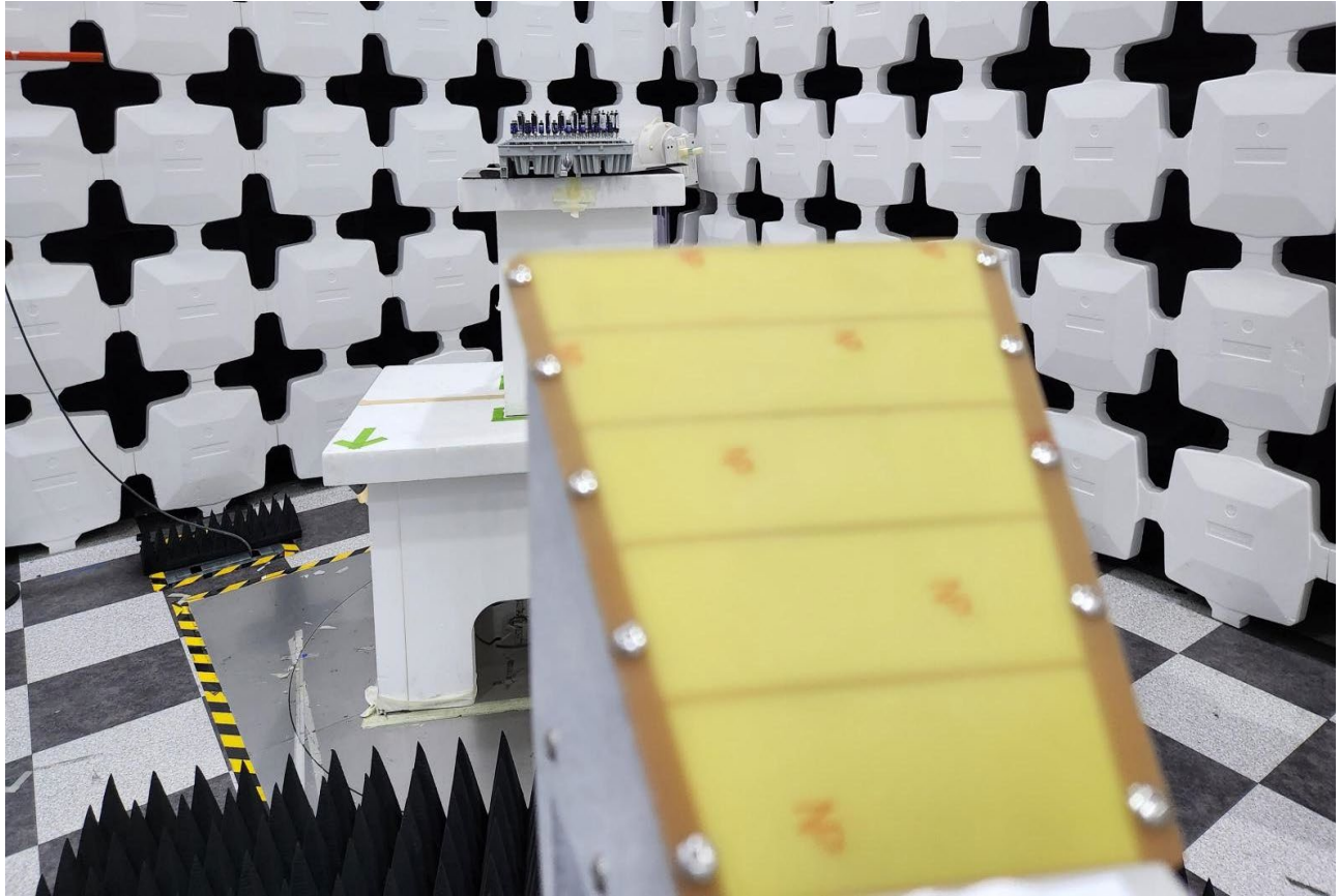
Above 1GHz Test Instrument & Measurement Setup > 1GHz
