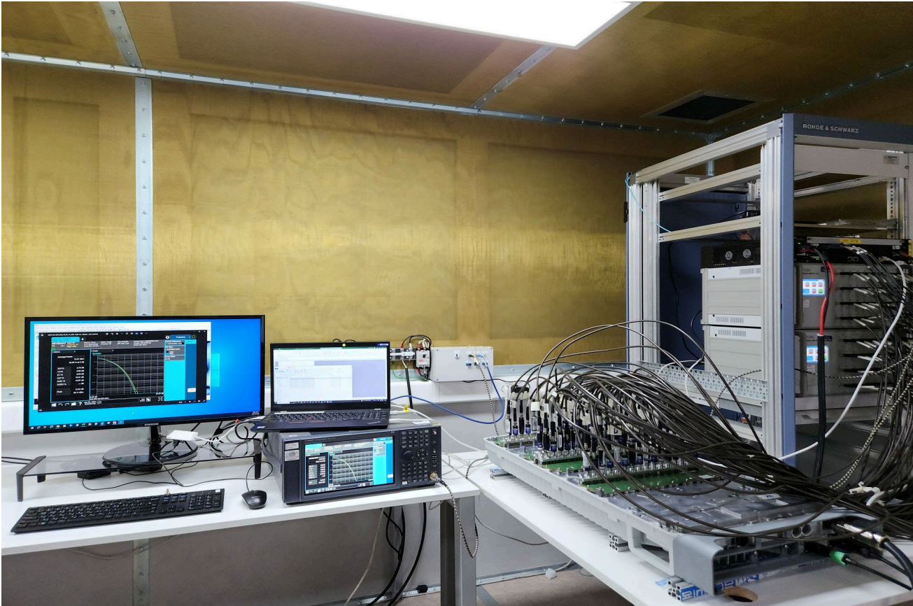
Conducted Test Instrument & Measurement Setup
