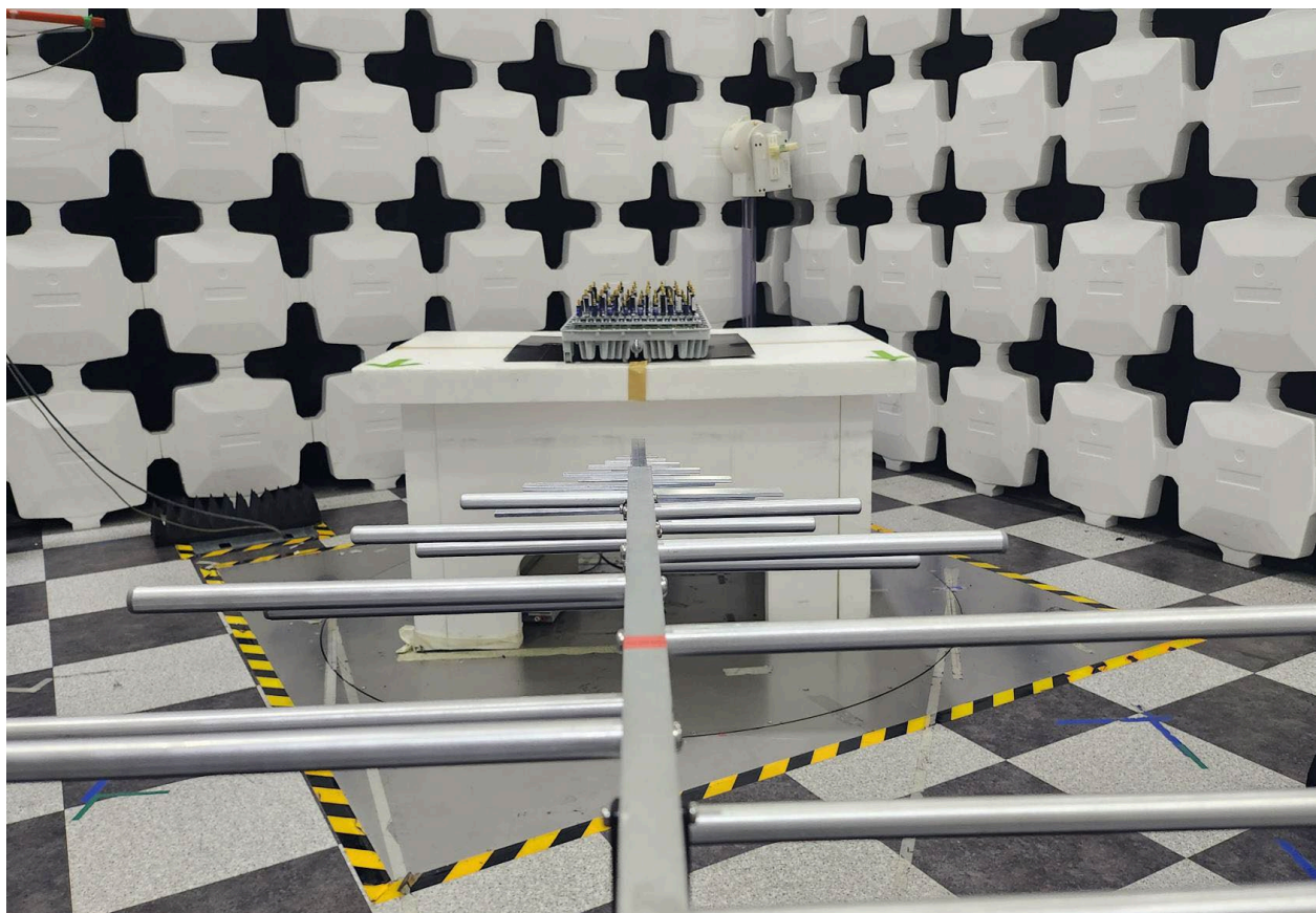
Below 1GHz Test Instrument & Measurement Setup
