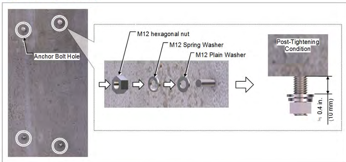
Figure 29. Drilling & Anchor (2)
