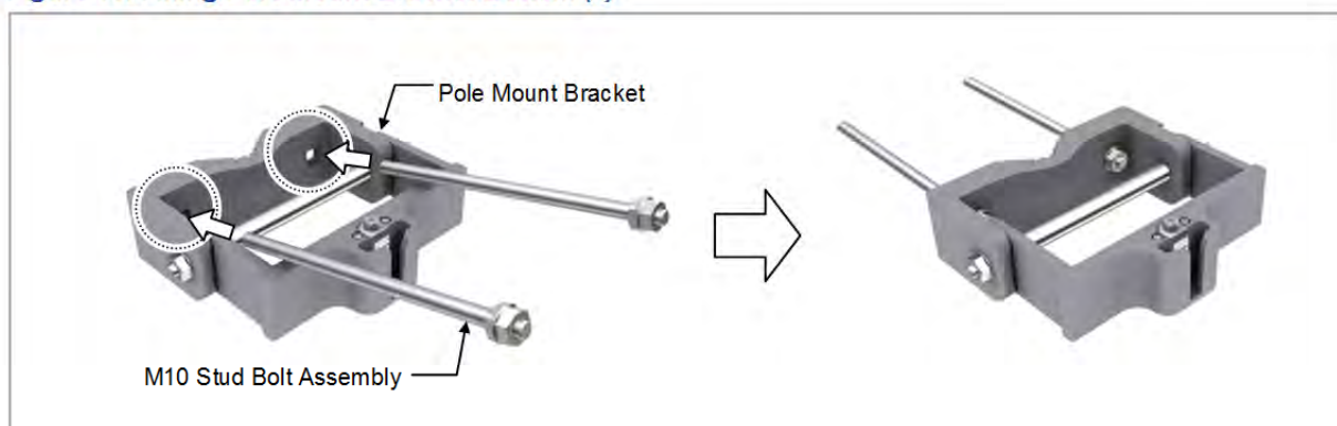
Figure 10. Fixing Pole Mount Bracket-Bottom (1)
