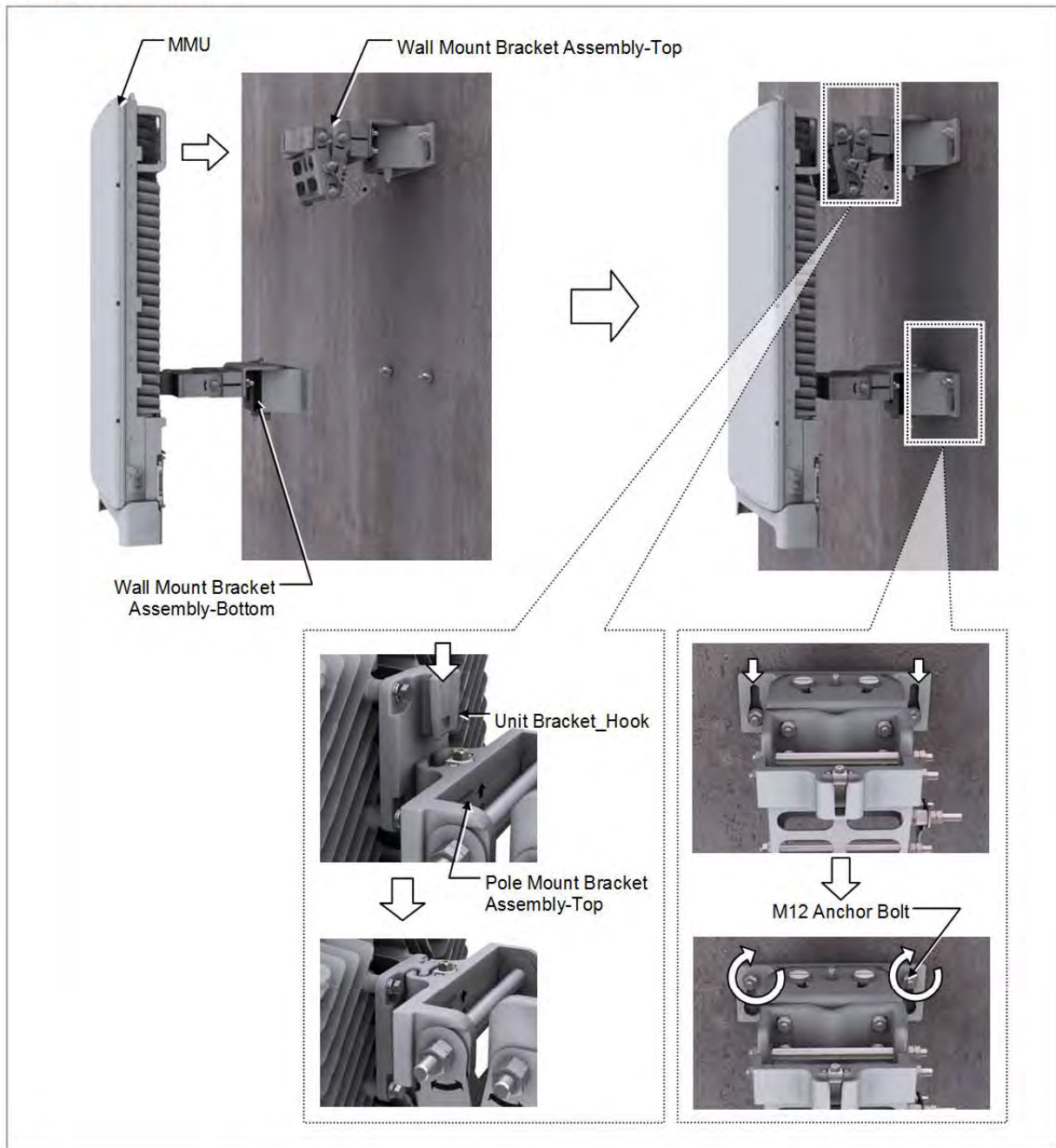
Figure 33. Fixing MMU
