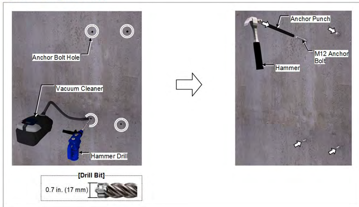
Figure 28. Drilling & Anchor (1)
