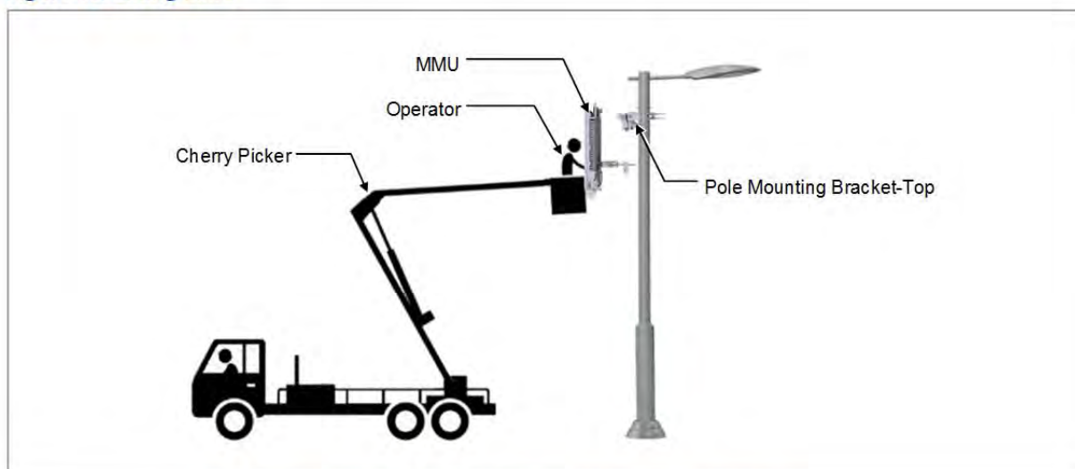
Figure 16. Lifting MMU
