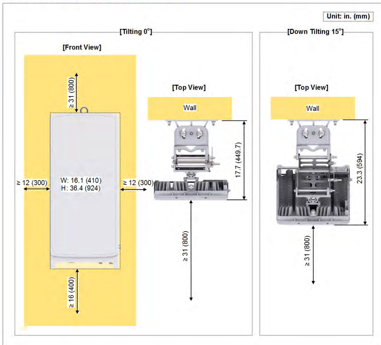
Figure 5. MMU Arrangement_Wall Type Installation
