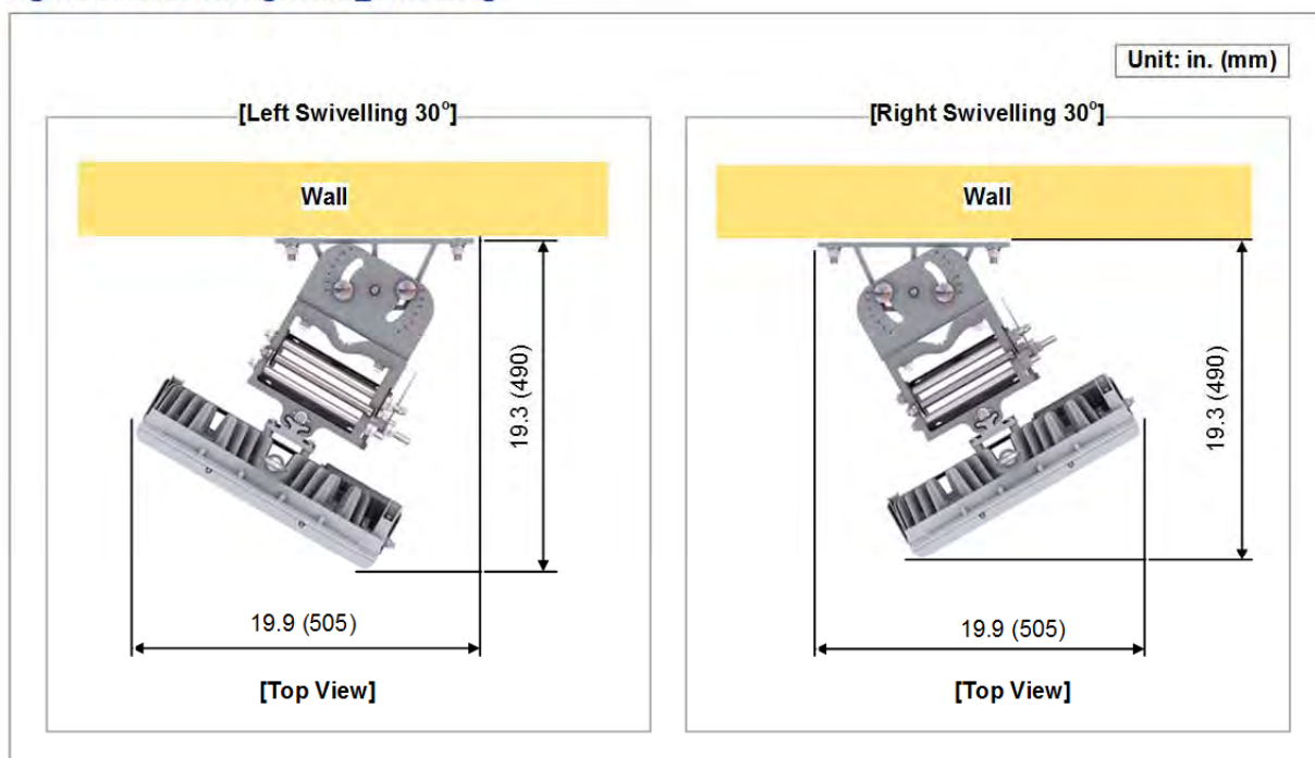
Figure 6. MMU Arrangement_Swivelling
