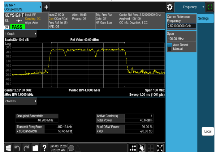
Plot 8-10. Occupied Bandwidth Plot (MSR_B/n41_3C_NR_10M+LTE_20M+20M_16QAM - Low Channel, Port 17)
