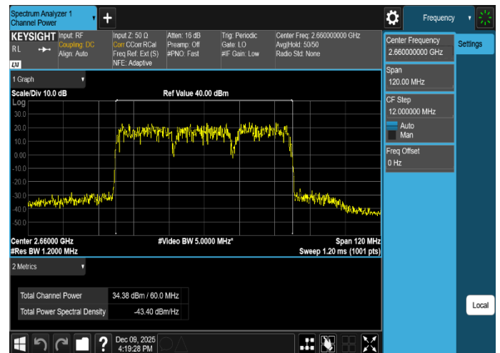
Plot 8-14. Equivalent Radiated Power Plot (LTE_B41_3C_20M+20M+20M_16QAM - High Channel, Port 35)
