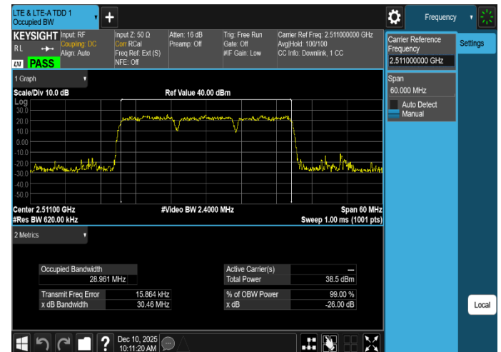
Plot 8-6. Occupied Bandwidth Plot (LTE_B41_3C_10M+10M+10M_16QAM - Low Channel, Port 5)
