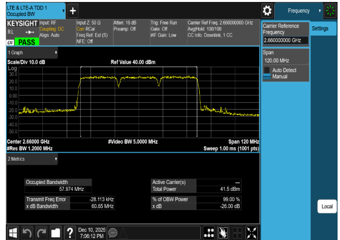
Plot 8-8. Occupied Bandwidth Plot (LTE_B41_3C_20M+20M+20M_16QAM - High Channel, Port 58)
