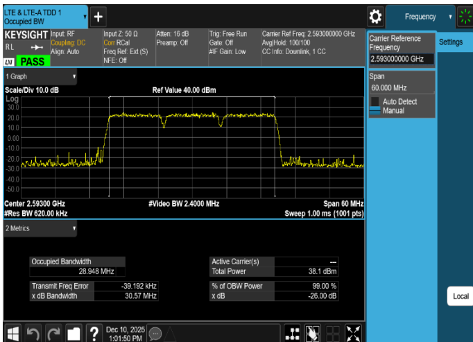
Plot 8-5. Occupied Bandwidth Plot (LTE_B41_3C_10M+10M+10M_QPSK - Mid Channel, Port 23)
