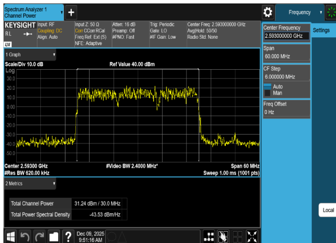
Plot 8-13. Equivalent Radiated Power Plot (LTE_B41_3C_10M+10M+10M_QPSK - Mid Channel, Port 35)
