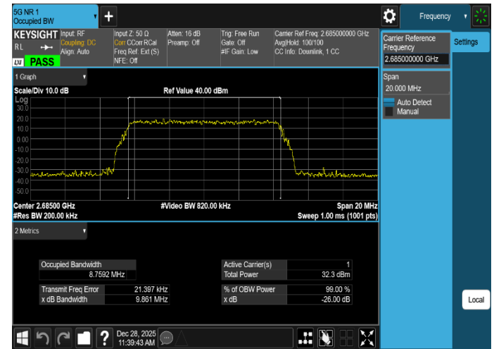
Plot 8-4. Occupied Bandwidth Plot (NR_n41_1C_10M_16QAM - High Channel, Port 22)
