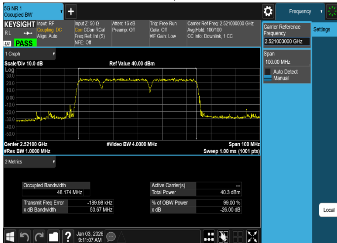
Plot 8-9. Occupied Bandwidth Plot (MSR_B/n41_3C_NR_10M+LTE_20M+20M_QPSK - Low Channel, Port 58)
