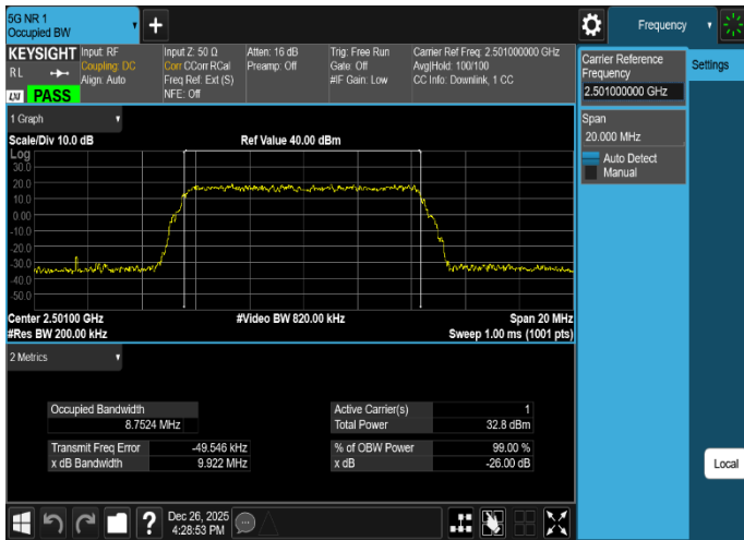
Plot 8-3. Occupied Bandwidth Plot (NR_n41_1C_10M_QPSK - Low Channel, Port 27)
