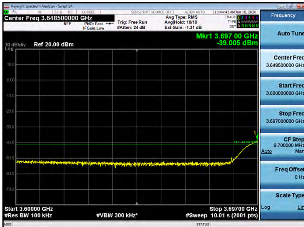
Port 24 / (64 Port) 5G NR n77 20 MHz [1 Carrier] / 3 600 MHz ~ 3 697 MHz / 16QAM / Low
