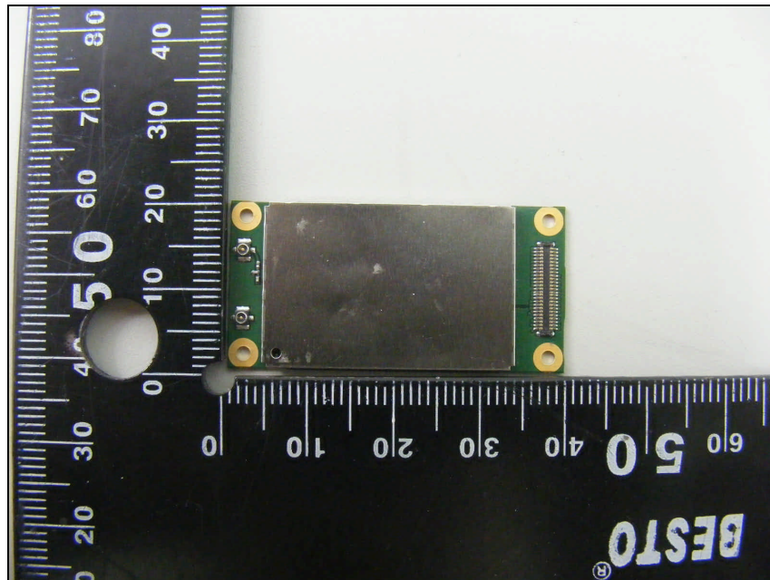
Top view of 2G, 3G Module with cover
