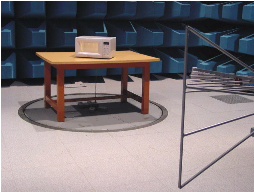
Fig. 8 Radiated Emission setup(30 - 1000MHz)
