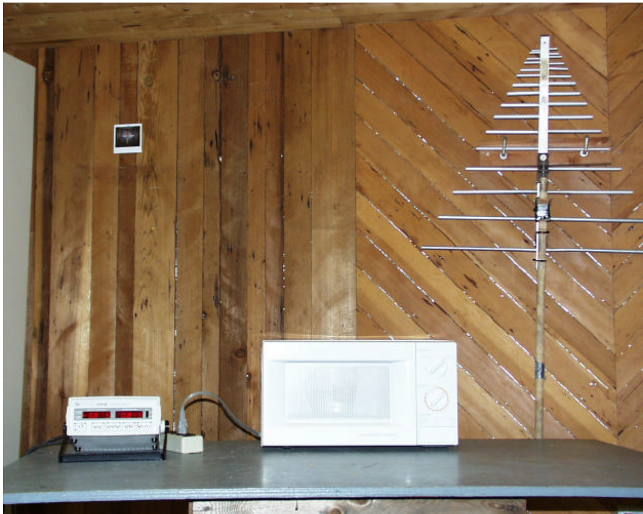
Power Input Test Setup
