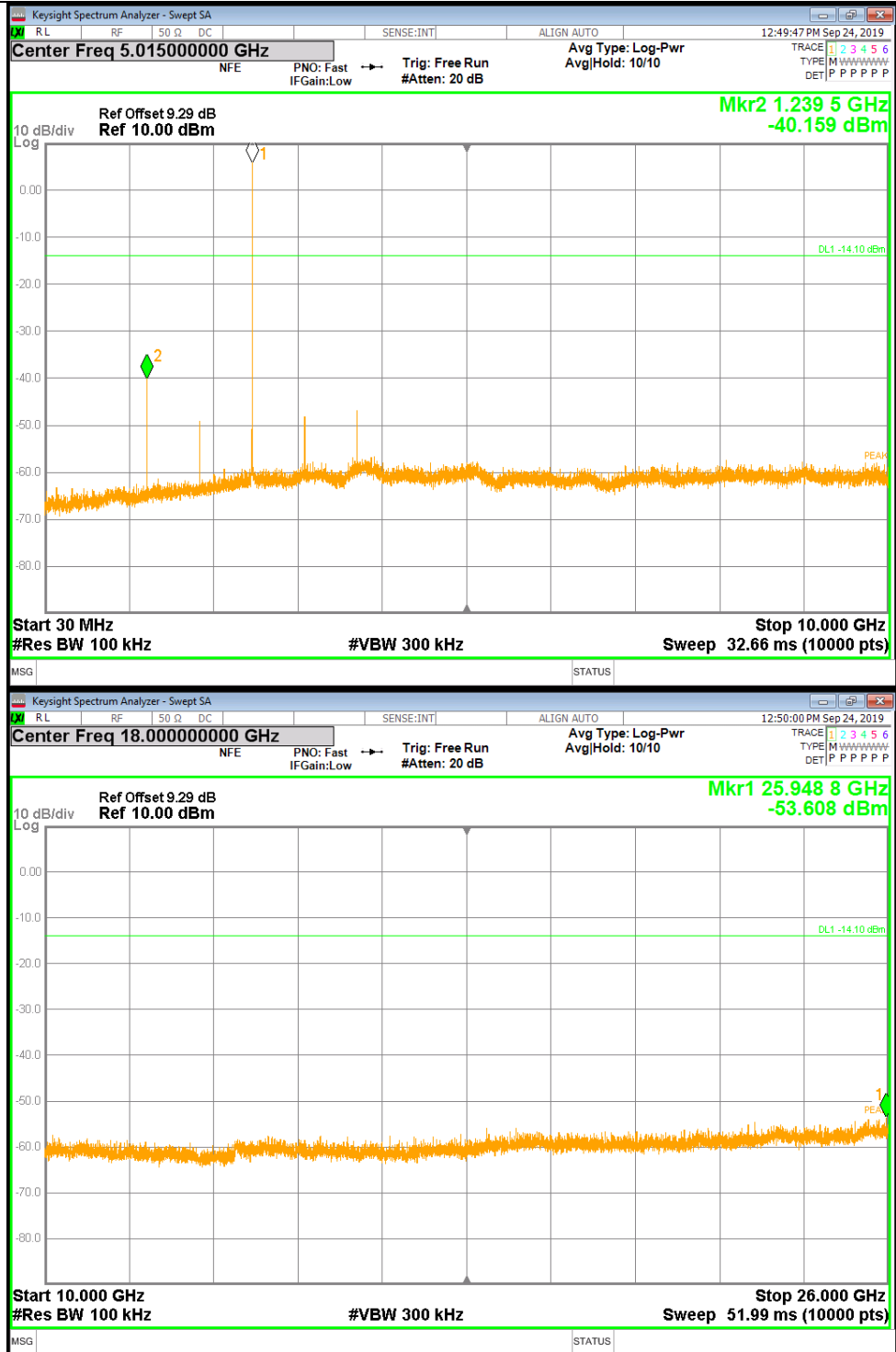
8DPSK_LCH_Graphs
