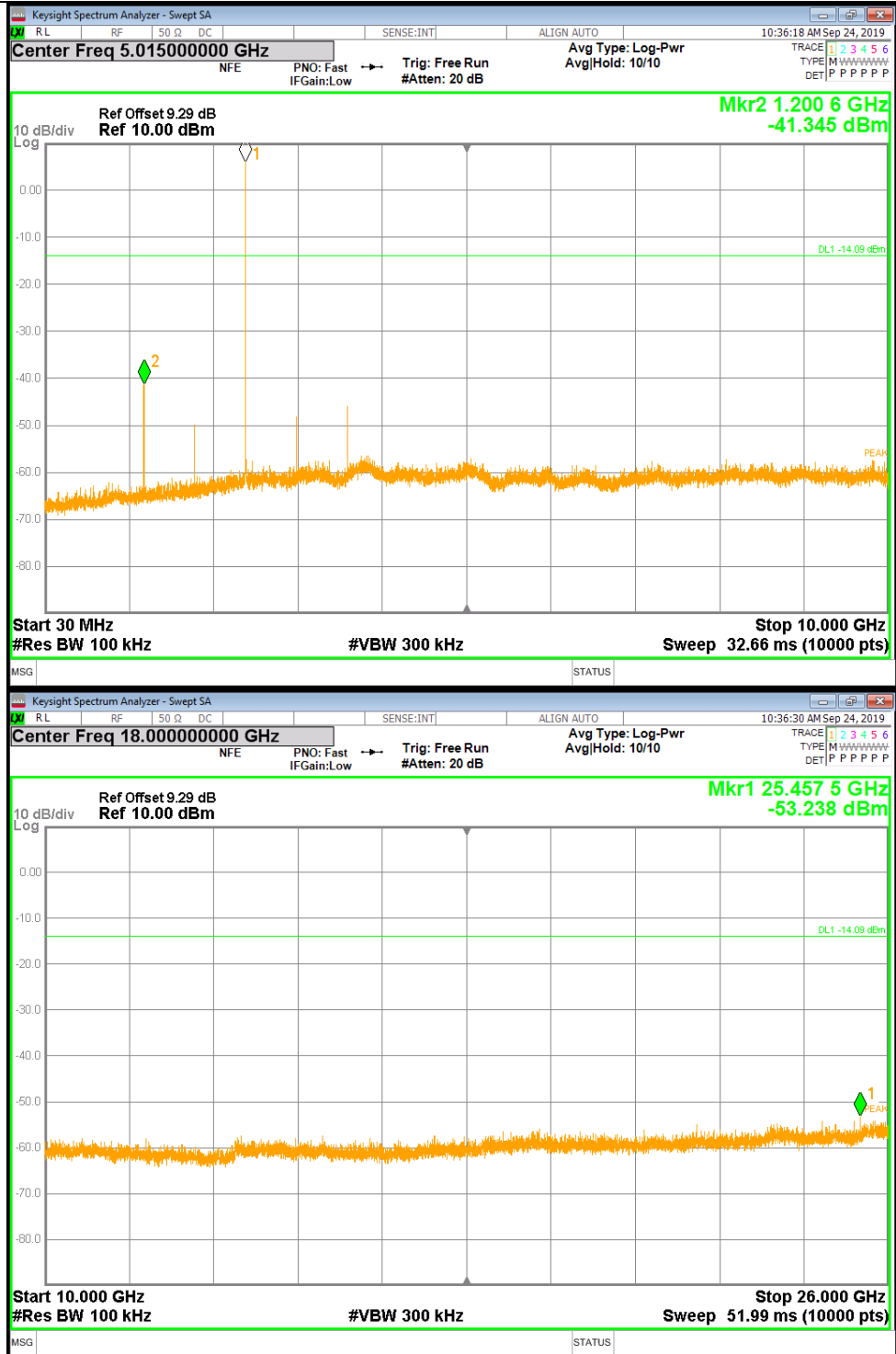
GFSK_MCH_Graphs
