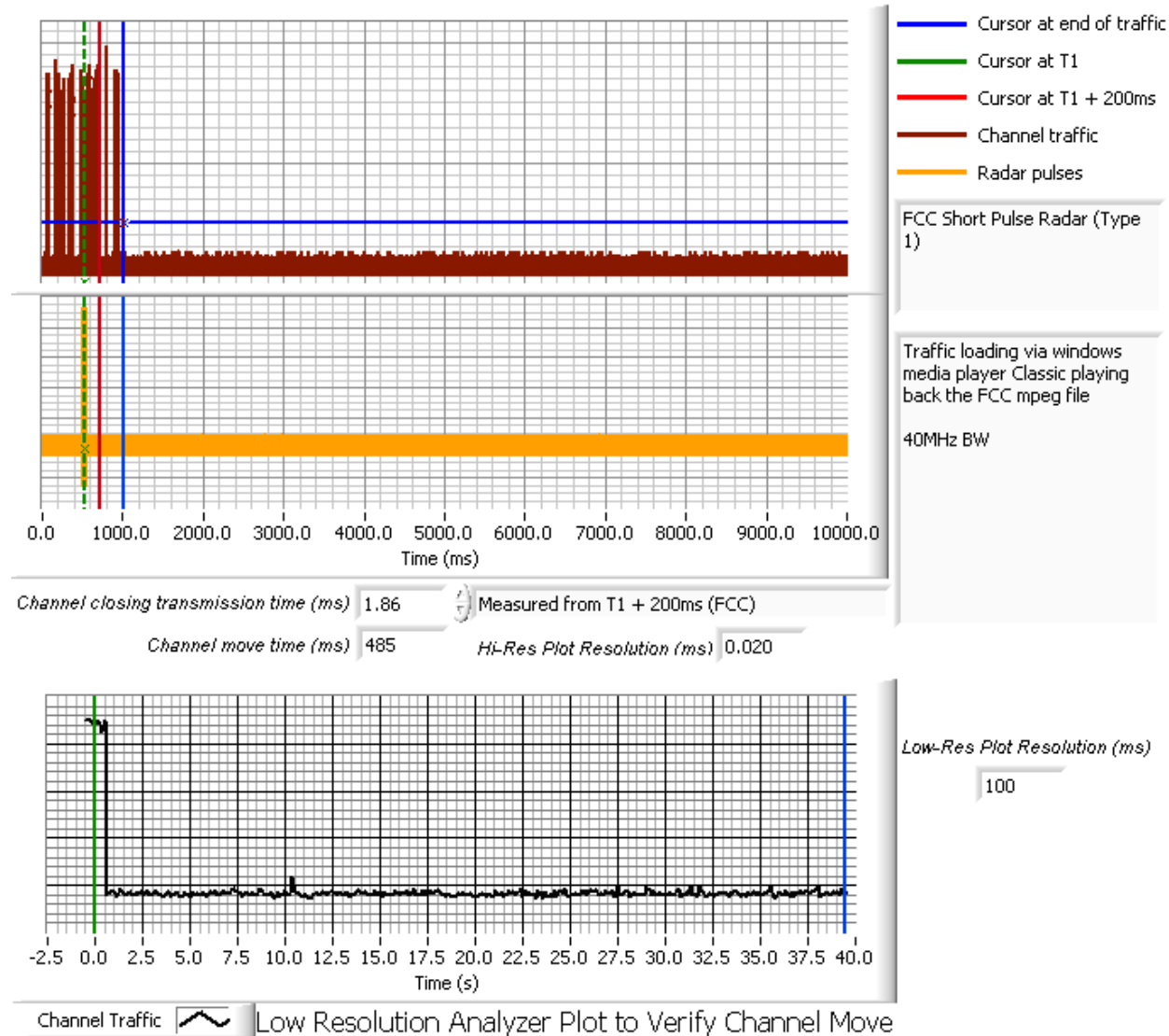
Figure 5 Channel Closing Time and Channel Move Time – 40 second plot (40MHz BW)
