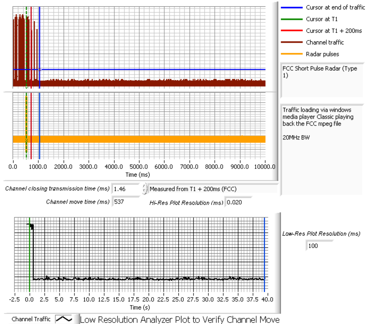
Figure 3 Channel Closing Time and Channel Move Time – 40 second plot (20MHz BW)
