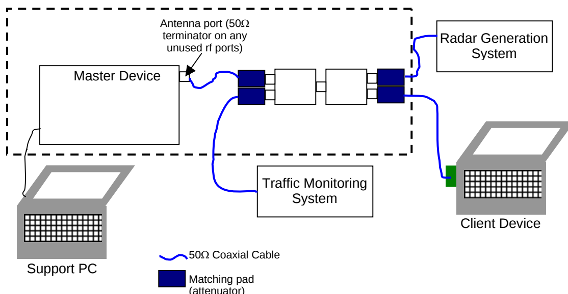
Figure 2 Test Configuration for Conducted Measurement Method
