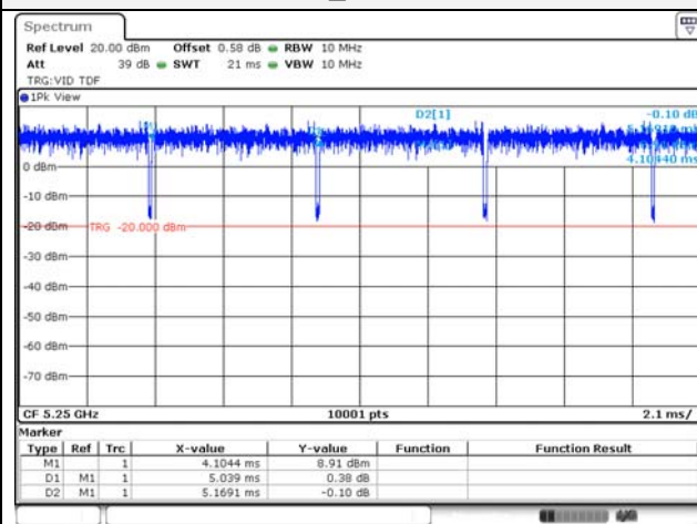
802.11ax_HE160 / 106T
