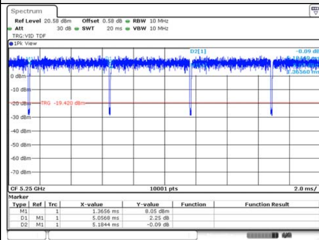
802.11ax_HE160 / 52T
