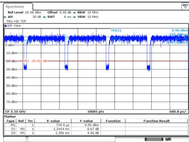
802.11ax_HE160 / 484T
