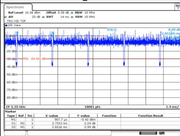
802.11ax_HE160 / 106T
