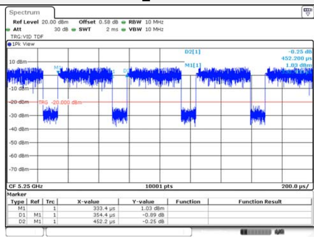
802.11ax_HE160 / 996T
