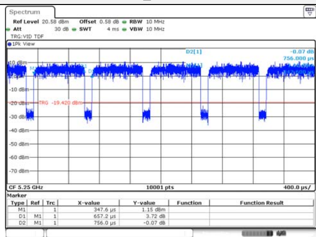
802.11ax_HE160 / 996T
