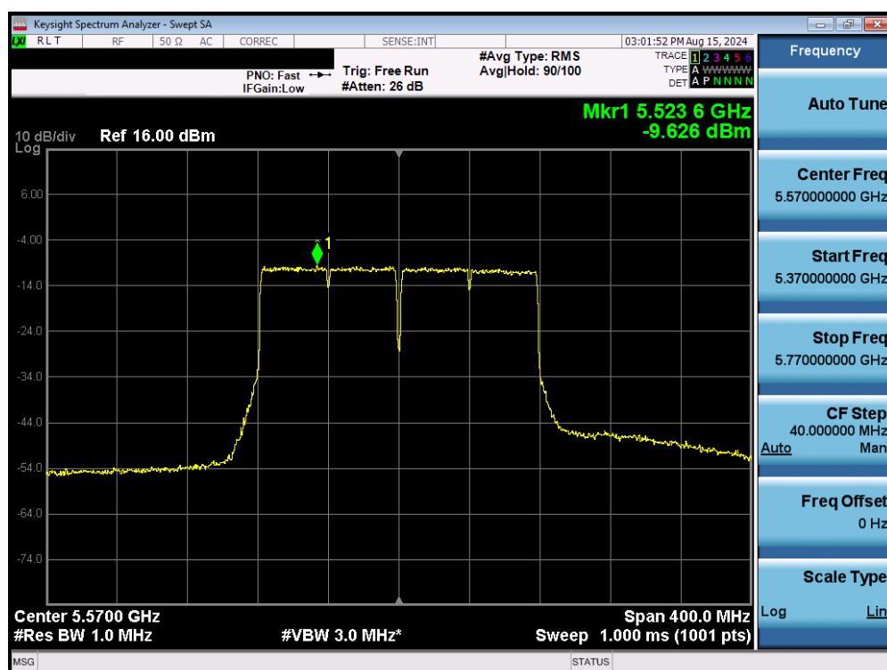
Plot 7-163. Power Spectral Density Plot MIMO ANT2 (160MHz BW 802.11ac (UNII Band 2C) – Ch. 114)
