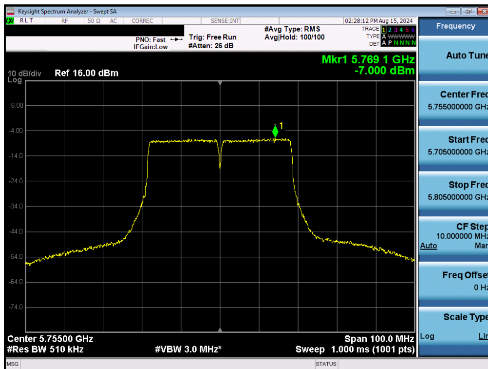
Plot 7-168. Power Spectral Density Plot MIMO ANT2 (40MHz BW 802.11n (UNII Band 3) – Ch. 151)
