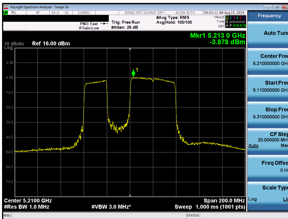
Plot 7-181. Power Spectral Density Plot MIMO ANT1 (80MHz BW 802.11be (UNII Band 1) – Ch. 42)
