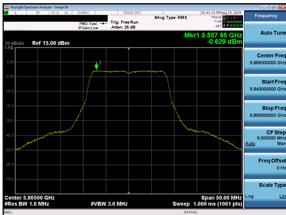
Plot 7-172. Power Spectral Density Plot MIMO ANT2 (802.11a (UNII Band 4) – Ch. 173)
