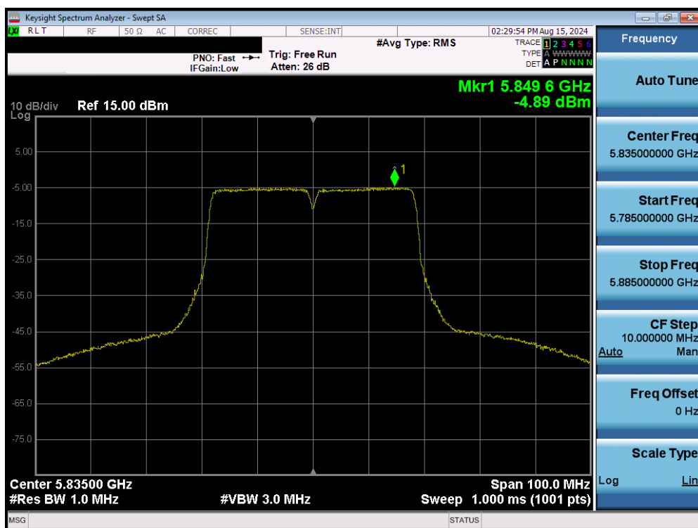
Plot 7-175. Power Spectral Density Plot MIMO ANT2 (40MHz BW 802.11n (UNII Band 3/4) – Ch. 167)
