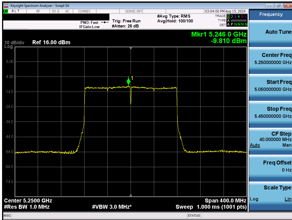
Plot 7-148. Power Spectral Density Plot MIMO ANT2 (160MHz BW 802.11be (UNII Band 1/2A) – Ch. 50)
