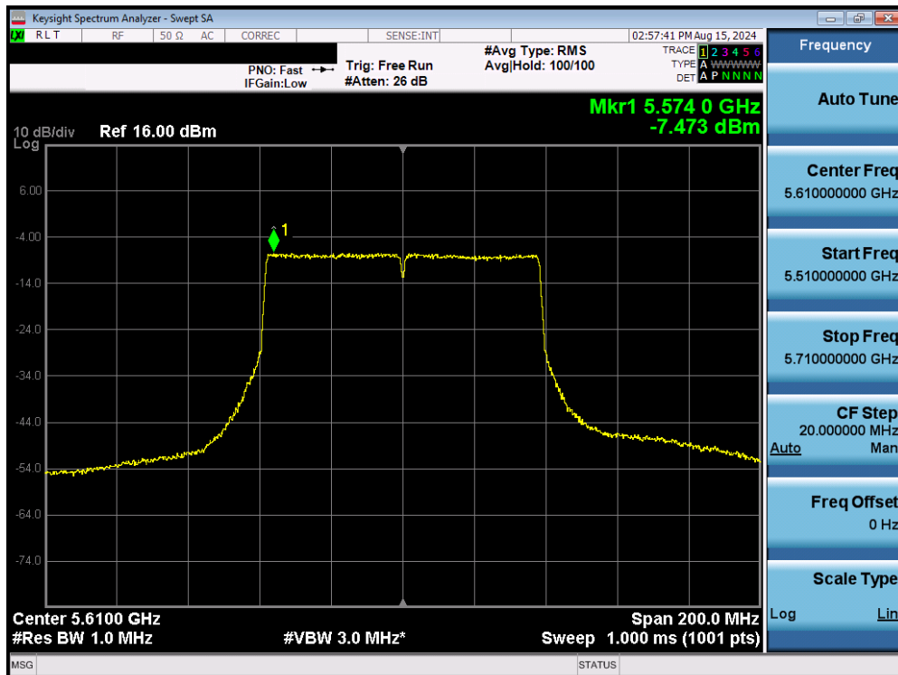
Plot 7-161. Power Spectral Density Plot MIMO ANT2 (80MHz BW 802.11ac (UNII Band 2C) – Ch. 122)
