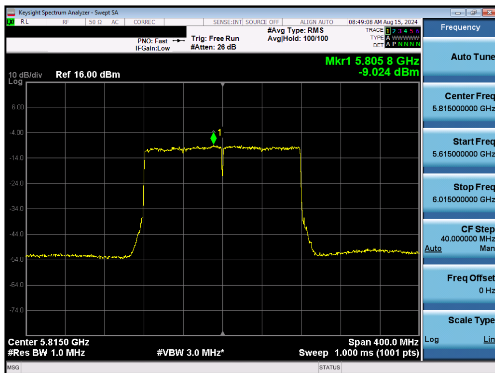
Plot 7-139. Power Spectral Density Plot MIMO ANT1 (160MHz BW 802.11be (UNII Band 3/4) – Ch. 163)
