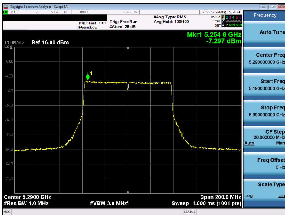
Plot 7-154. Power Spectral Density Plot MIMO ANT2 (80MHz BW 802.11ac (UNII Band 2A) – Ch. 58)
