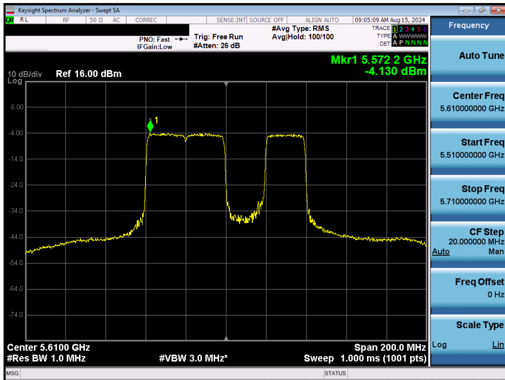
Plot 7-184. Power Spectral Density Plot MIMO ANT1 (80MHz BW 802.11be (UNII Band 2C) – Ch. 122)
