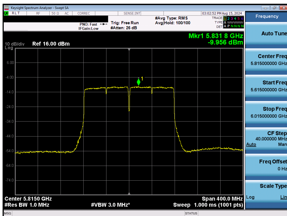
Plot 7-179. Power Spectral Density Plot MIMO ANT2 (160MHz BW 802.11ac (UNII Band 3/4) – Ch. 163)
