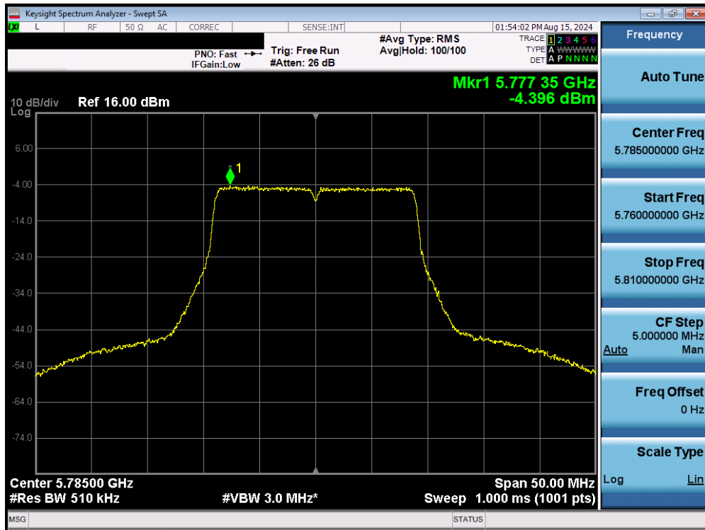
Plot 7-166. Power Spectral Density Plot MIMO ANT2 (20MHz BW 802.11n (UNII Band 3) – Ch. 157)
