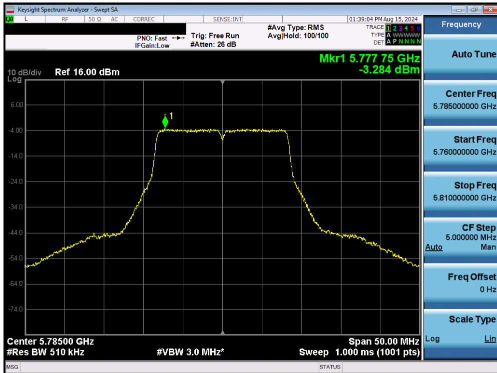
Plot 7-165. Power Spectral Density Plot MIMO ANT2 (802.11a (UNII Band 3) – Ch. 157)
