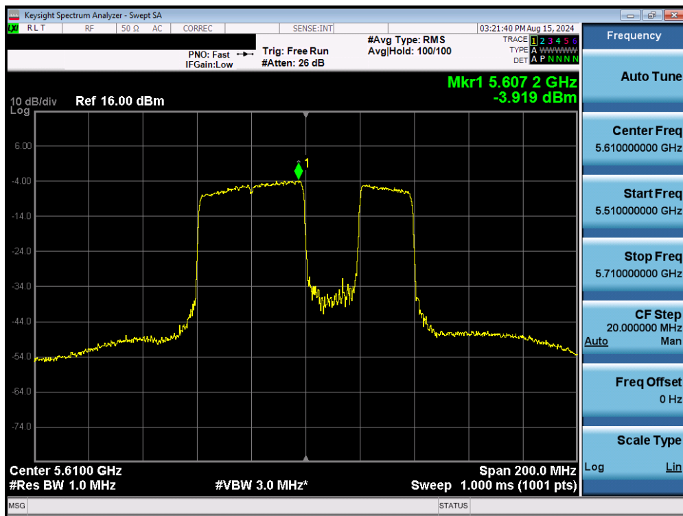
Plot 7-192. Power Spectral Density Plot MIMO ANT2 (80MHz BW 802.11be (UNII Band 2C) – Ch. 122)
