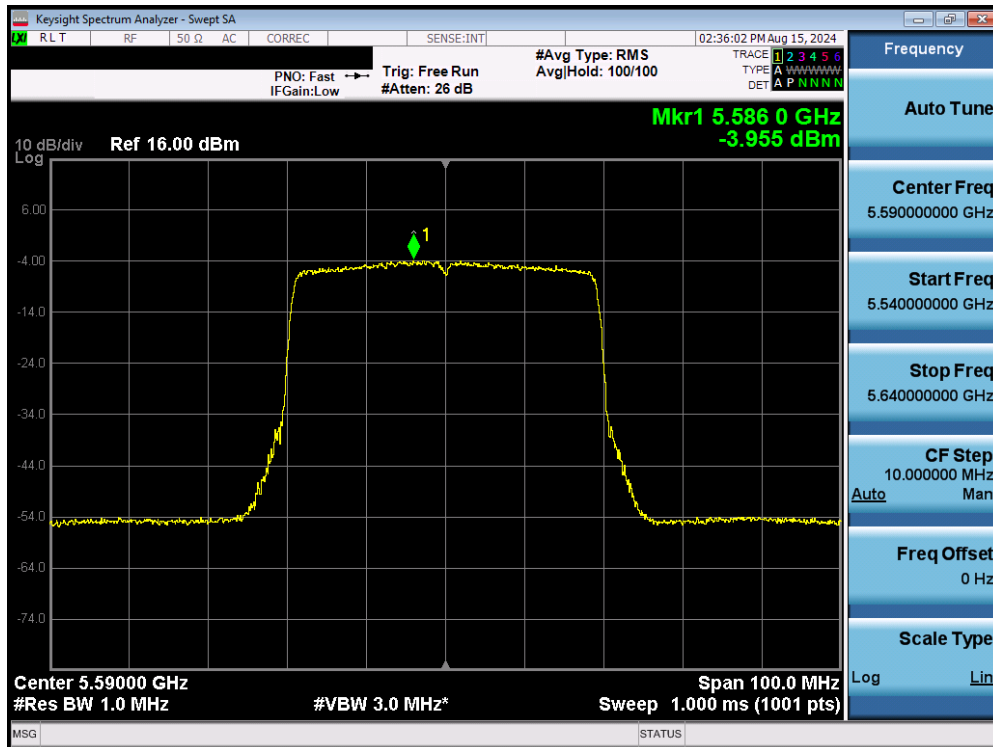
Plot 7-160. Power Spectral Density Plot MIMO ANT2 (40MHz BW 802.11be (UNII Band 2C) – Ch. 118)
