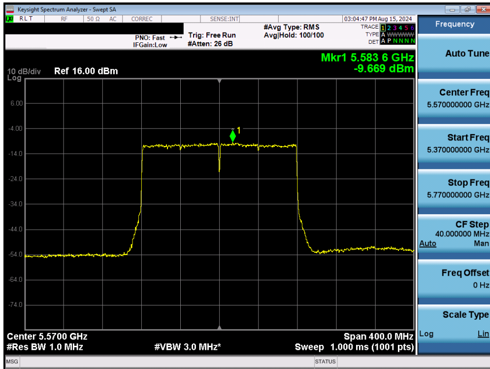
Plot 7-164. Power Spectral Density Plot MIMO ANT2 (160MHz BW 802.11be (UNII Band 2C) – Ch. 114)
