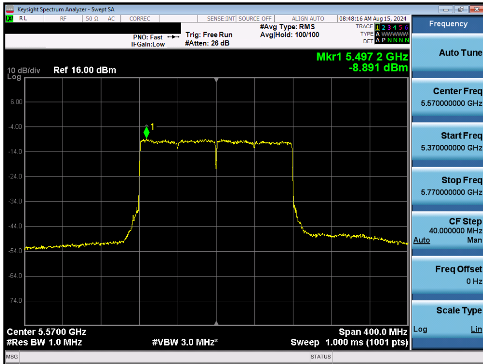
Plot 7-123. Power Spectral Density Plot MIMO ANT1 (160MHz BW 802.11be (UNII Band 2C) – Ch. 114)
