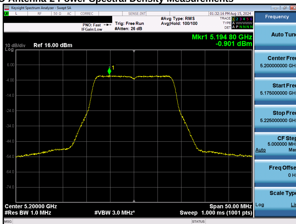
Plot 7-140. Power Spectral Density Plot MIMO ANT2 (802.11a (UNII Band 1) – Ch. 40)
