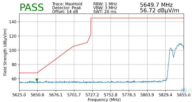
Plot 7-238. Radiated Lower Band Edge Plot MIMO (Peak – UNII Band 4 – 242 Tones)
