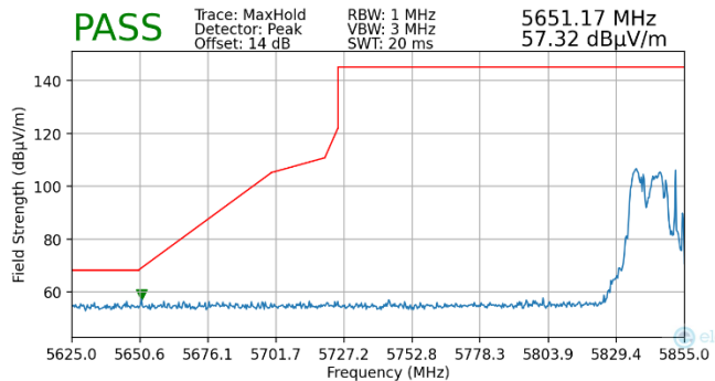
Plot 7-228. Radiated Lower Band Edge Plot MIMO (Peak – UNII Band 4 – 106+26 Tones)
