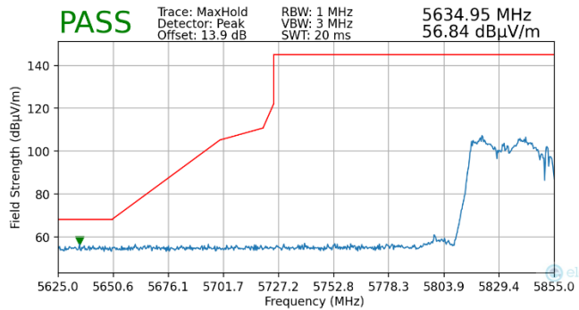
Plot 7-248. Radiated Lower Band Edge Plot MIMO (Peak - UNII Band 4 - 484 Tones)
