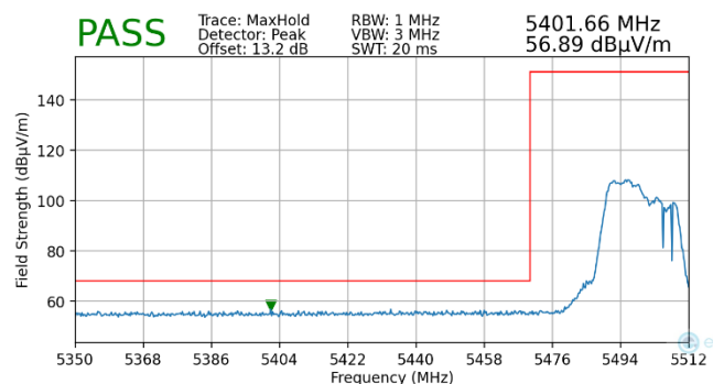
Plot 7-226. Radiated Lower Band Edge Plot MIMO (Peak – UNII Band 2C – 106+26 Tones)
