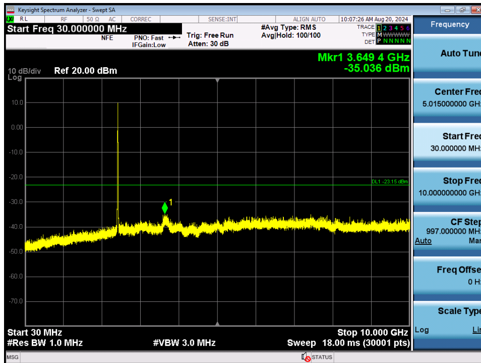
Plot 7-147. Conducted Spurious Plot MIMO ANT2 (802.11b – Ch. 6)
