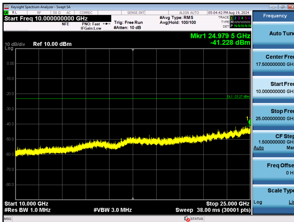
Plot 7-136. Conducted Spurious Plot SISO ANT2 (802.11b – Ch. 6)
