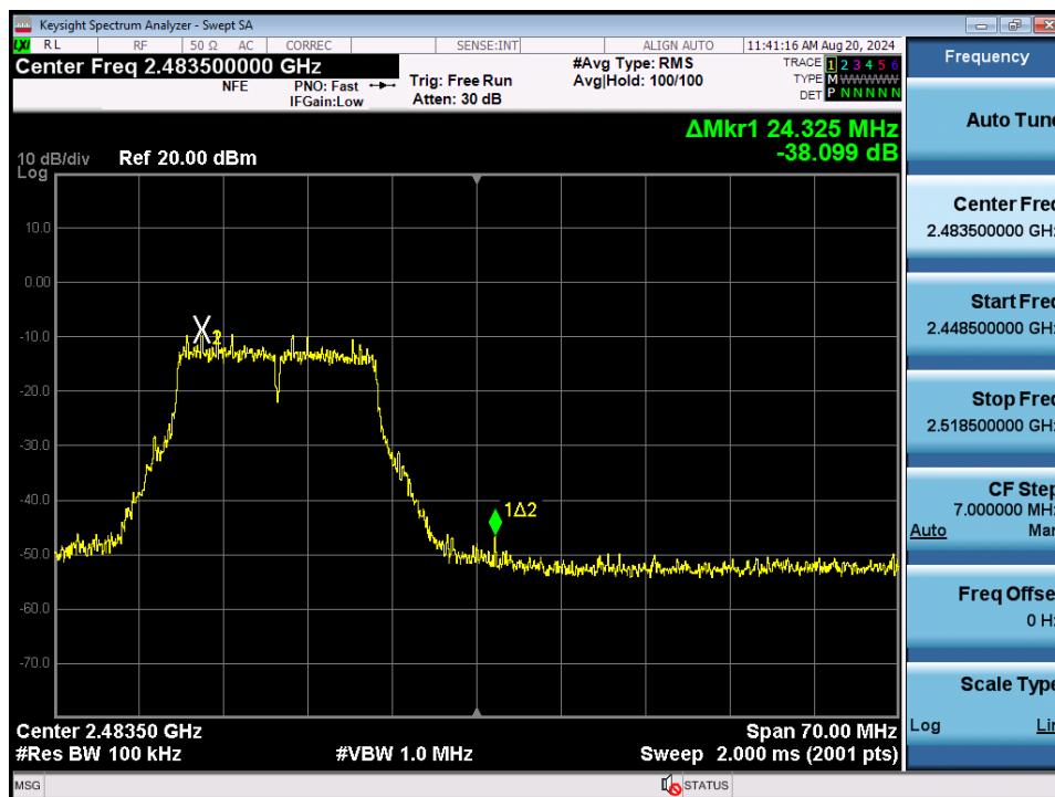
Plot 7-100. Band Edge Plot MIMO ANT1 (802.11g- Ch. 12)
