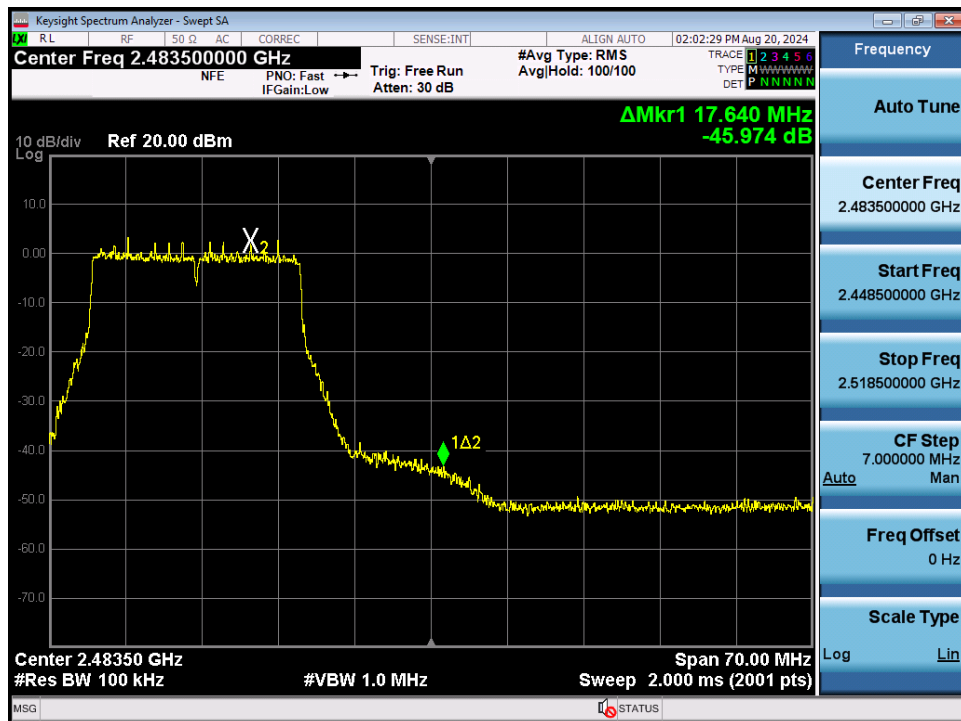
Plot 7-110. Band Edge Plot MIMO ANT1 (802.11ax/be (2.4GHz) – Ch. 11)
