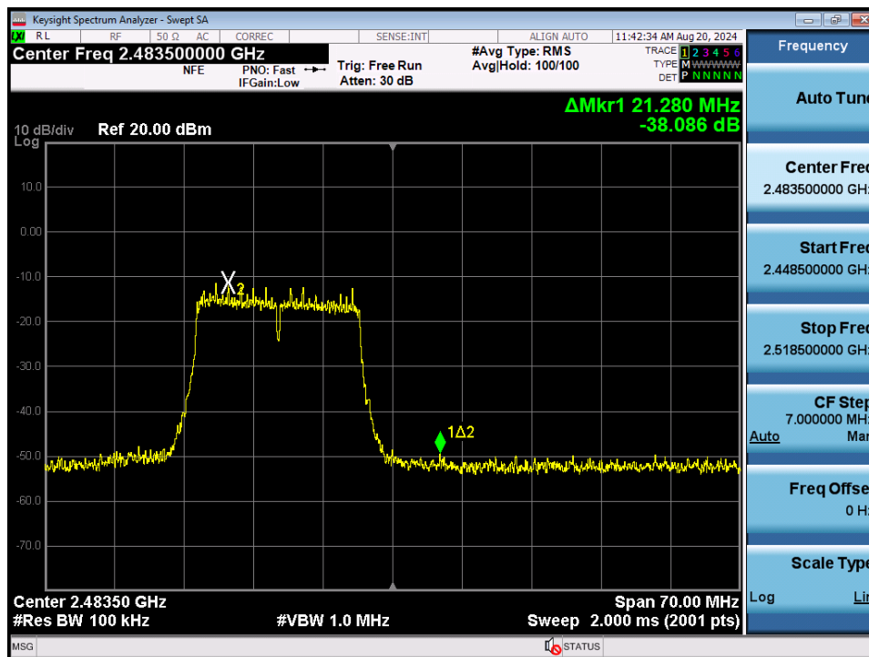
Plot 7-121. Band Edge Plot MIMO ANT2 (802.11g – Ch. 13)
