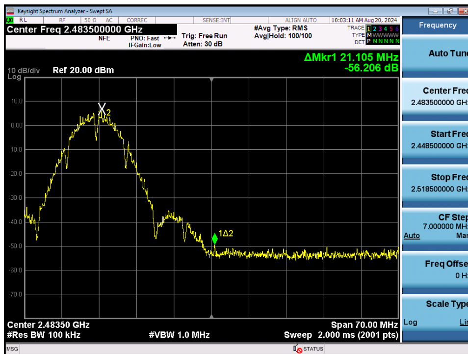
Plot 7-114. Band Edge Plot MIMO ANT2 (802.11b – Ch. 11)
