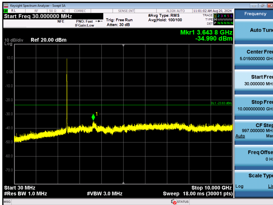
Plot 7-141. Conducted Spurious Plot MIMO ANT1 (802.11b – Ch. 6)
