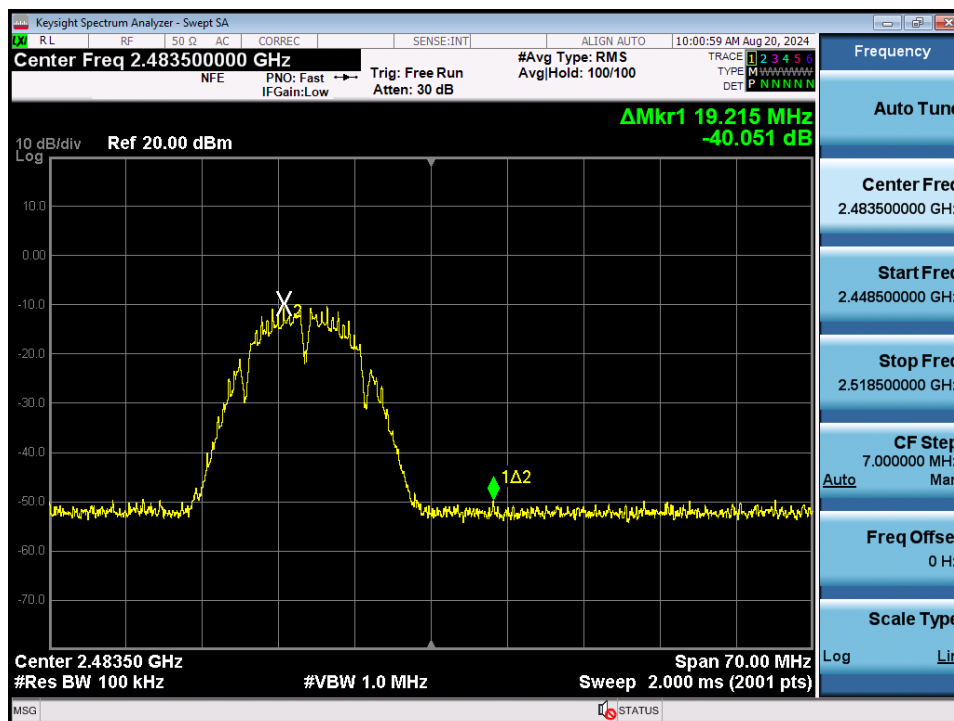
Plot 7-116. Band Edge Plot MIMO ANT2 (802.11b – Ch. 13)
