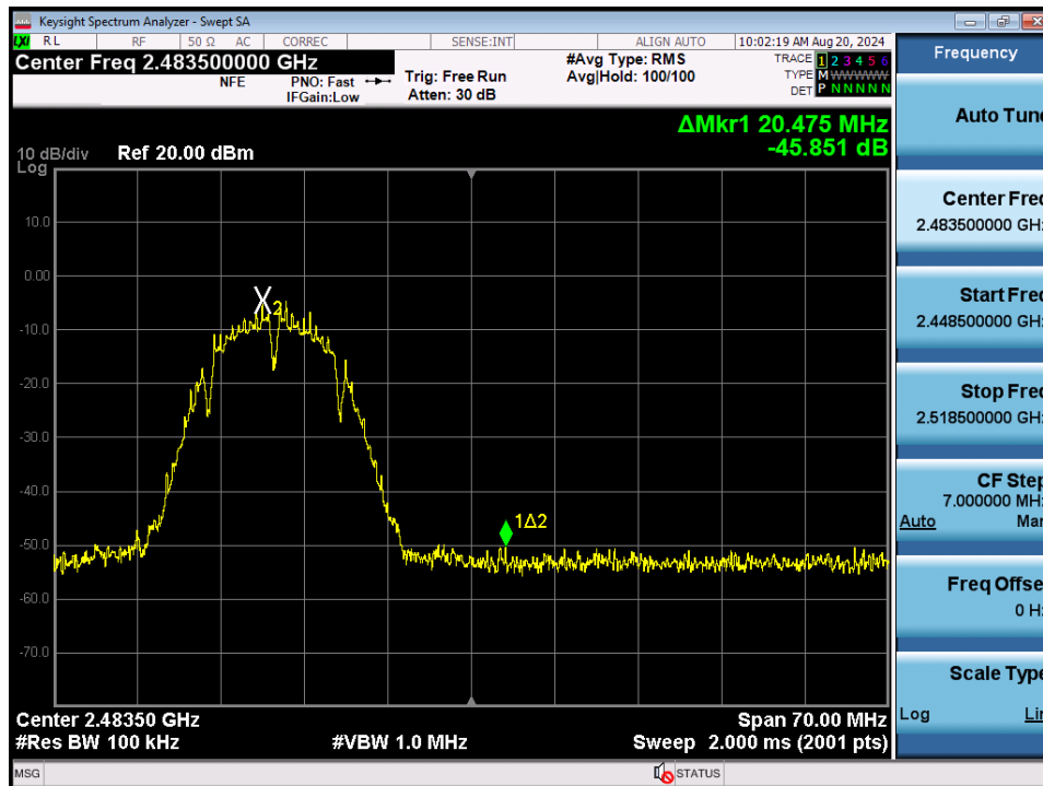
Plot 7-115. Band Edge Plot MIMO ANT2 (802.11b – Ch. 12)
