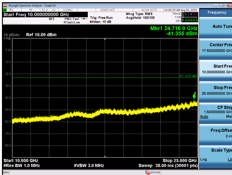
Plot 7-148. Conducted Spurious Plot MIMO ANT2 (802.11b – Ch. 6)
