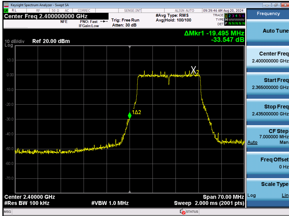
Plot 7-89. Band Edge Plot SISO ANT2 (802.11ax/be (2.4GHz) – Ch. 1)
