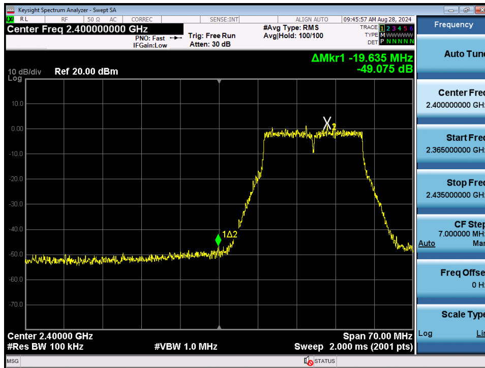
Plot 7-83. Band Edge Plot SISO ANT2 (802.11n (2.4GHz) – Ch. 2)
