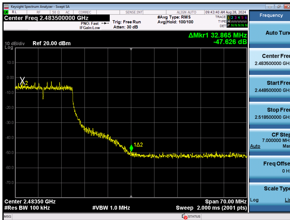
Plot 7-85. Band Edge Plot SISO ANT2 (802.11n (2.4GHz) – Ch. 10)
