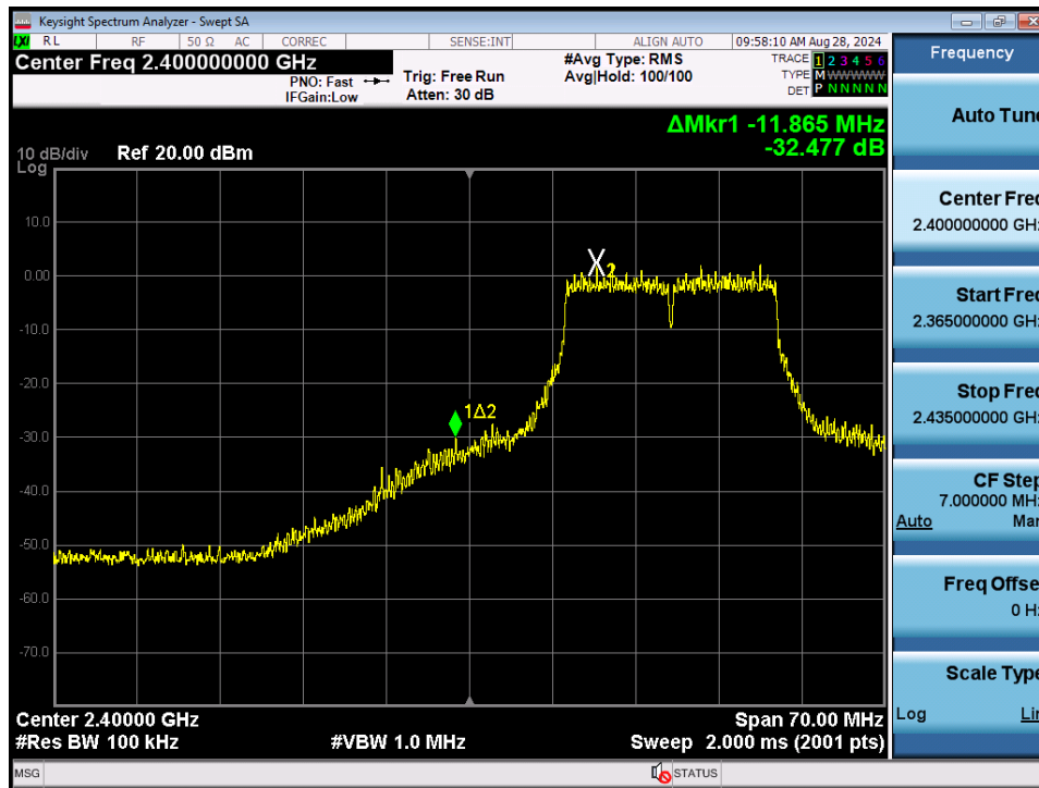
Plot 7-123. Band Edge Plot MIMO ANT2 (802.11n (2.4GHz) – Ch. 2)
