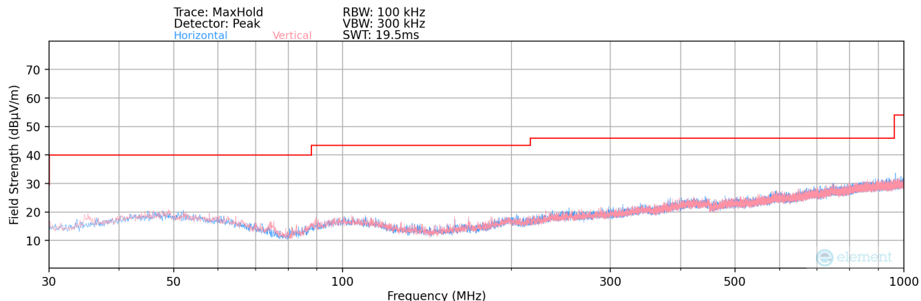
Plot 7-151. Radiated Spurious Plot below 1GHz SISO ANT2
