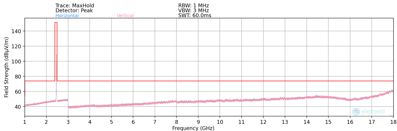
Plot 7-154. Radiated Spurious Plot above 1GHz SISO ANT2 (802.11b – Ch. 11)
