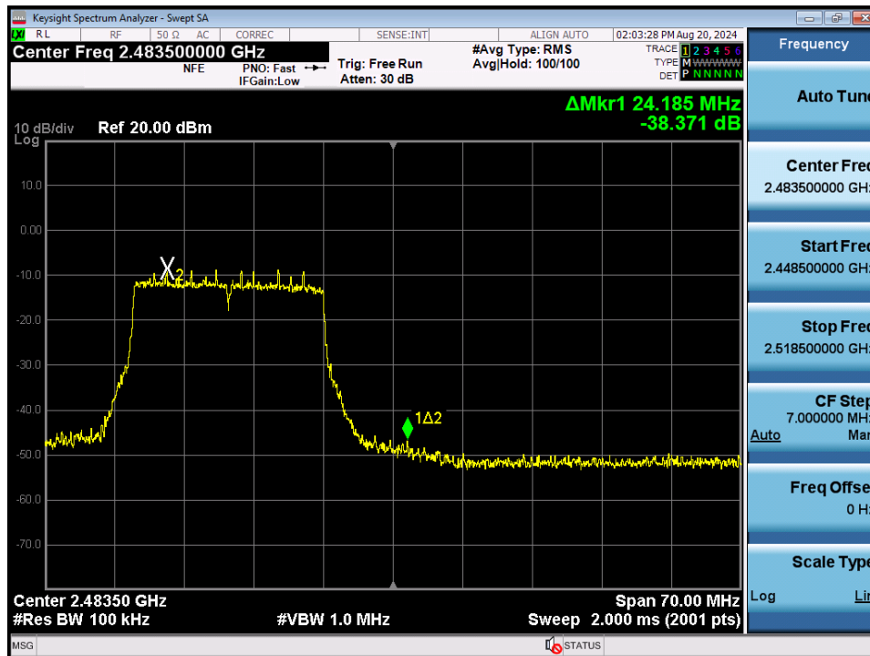
Plot 7-111. Band Edge Plot MIMO ANT1 (802.11ax/be (2.4GHz) – Ch. 12)
