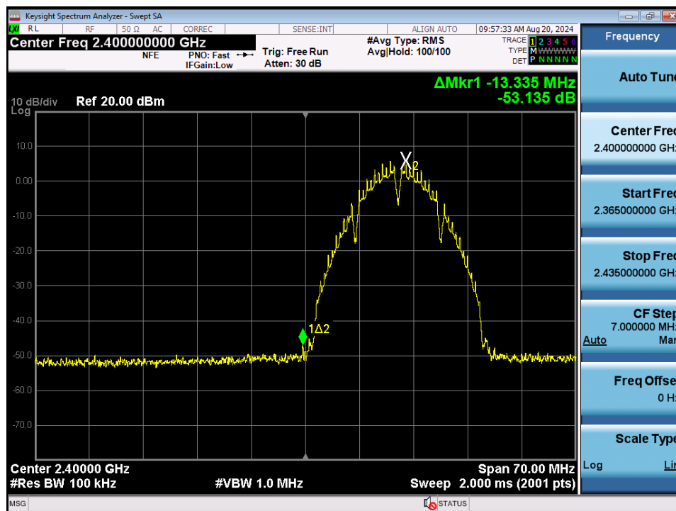
Plot 7-93. Band Edge Plot MIMO ANT1 (802.11b – Ch. 1)
