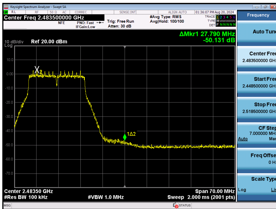
Plot 7-106. Band Edge Plot MIMO ANT1 (802.11n (2.4GHz) – Ch. 11)
