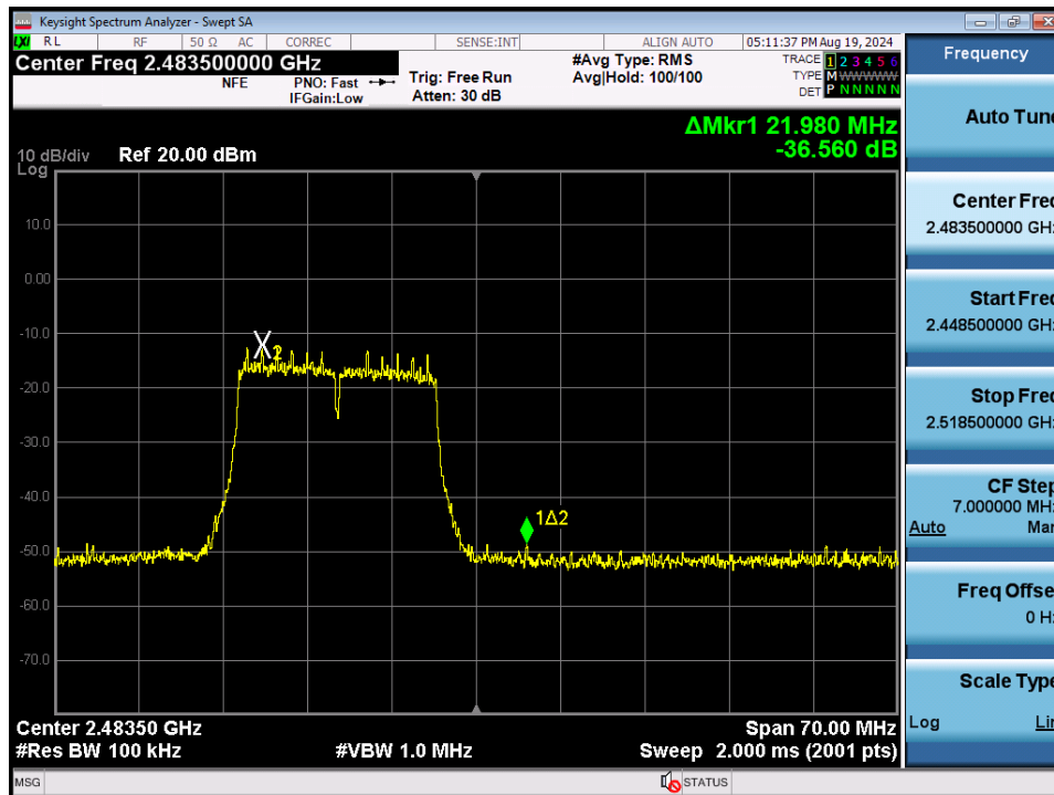
Plot 7-81. Band Edge Plot SISO ANT2 (802.11g – Ch. 13)
