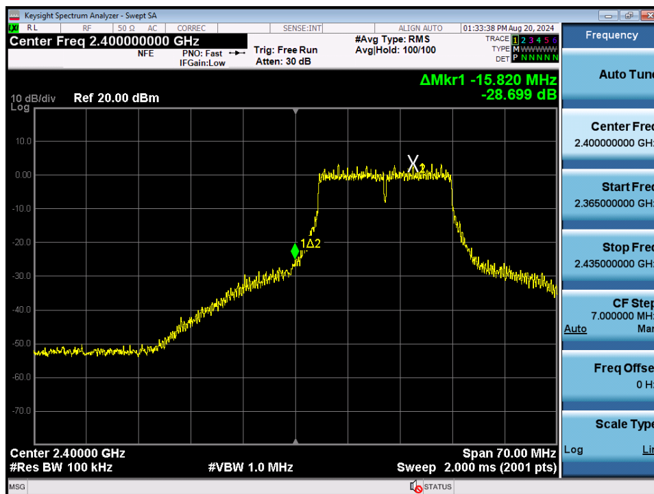
Plot 7-122. Band Edge Plot MIMO ANT2 (802.11n (2.4GHz) – Ch. 1)
