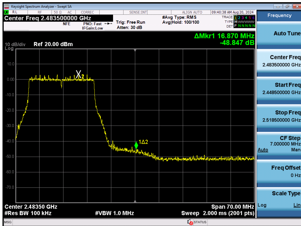
Plot 7-90. Band Edge Plot SISO ANT2 (802.11ax/be (2.4GHz) – Ch. 11)
