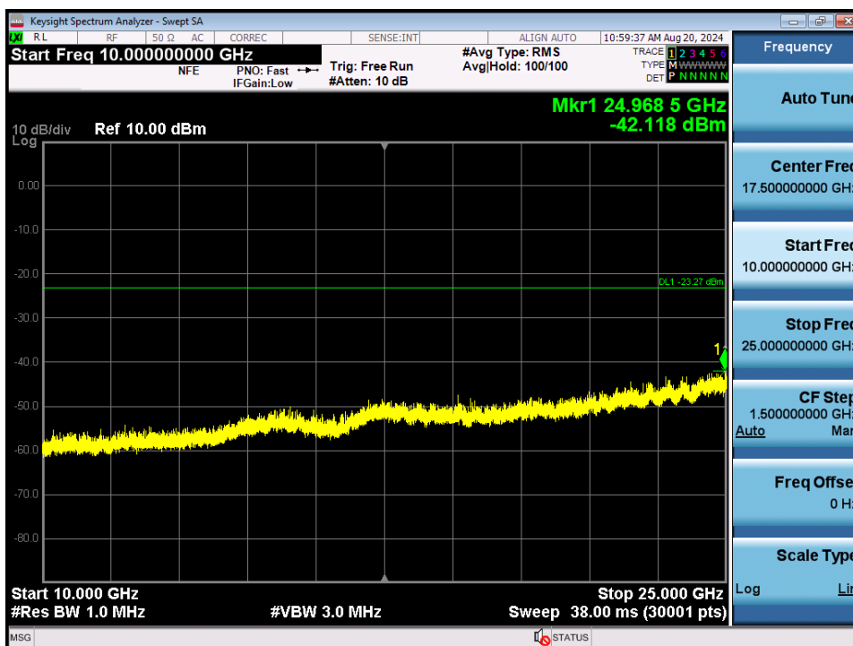
Plot 7-140. Conducted Spurious Plot MIMO ANT1 (802.11b – Ch. 1)
