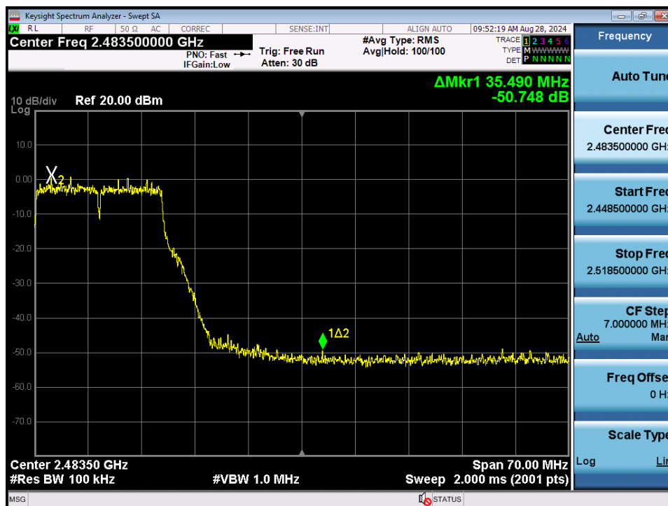
Plot 7-118. Band Edge Plot MIMO ANT2 (802.11g - Ch. 10)
