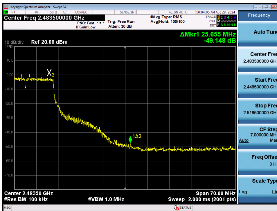
Plot 7-104. Band Edge Plot MIMO ANT1 (802.11n (2.4GHz) – Ch. 9)
