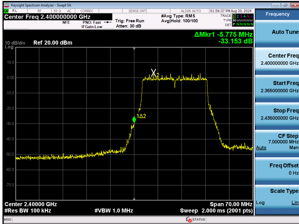
Plot 7-109. Band Edge Plot MIMO ANT1 (802.11ax/be (2.4GHz) – Ch. 1)
