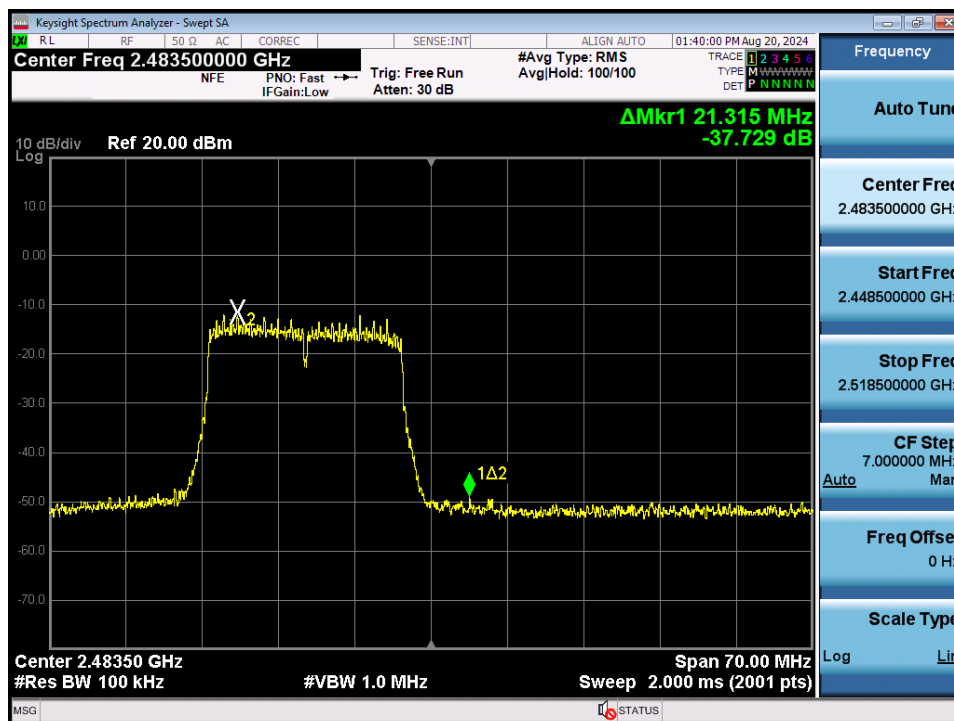
Plot 7-128. Band Edge Plot MIMO ANT2 (802.11n (2.4GHz) – Ch. 13)
