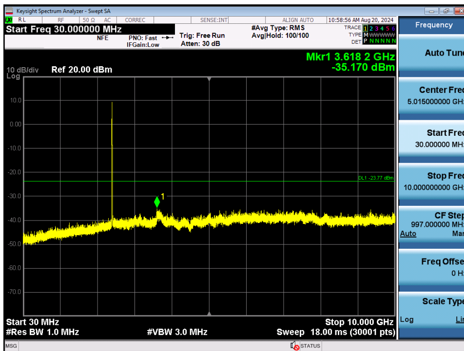
Plot 7-139. Conducted Spurious Plot MIMO ANT1 (802.11b – Ch. 1)
