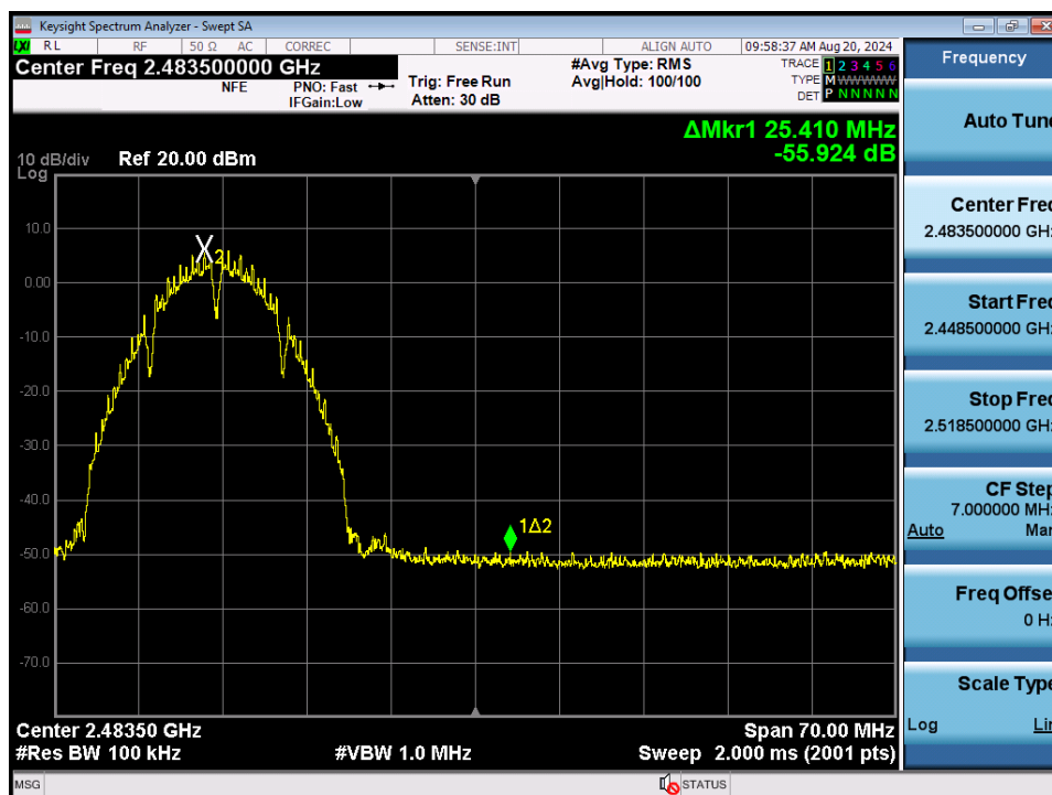
Plot 7-94. Band Edge Plot MIMO ANT1 (802.11b – Ch. 11)
