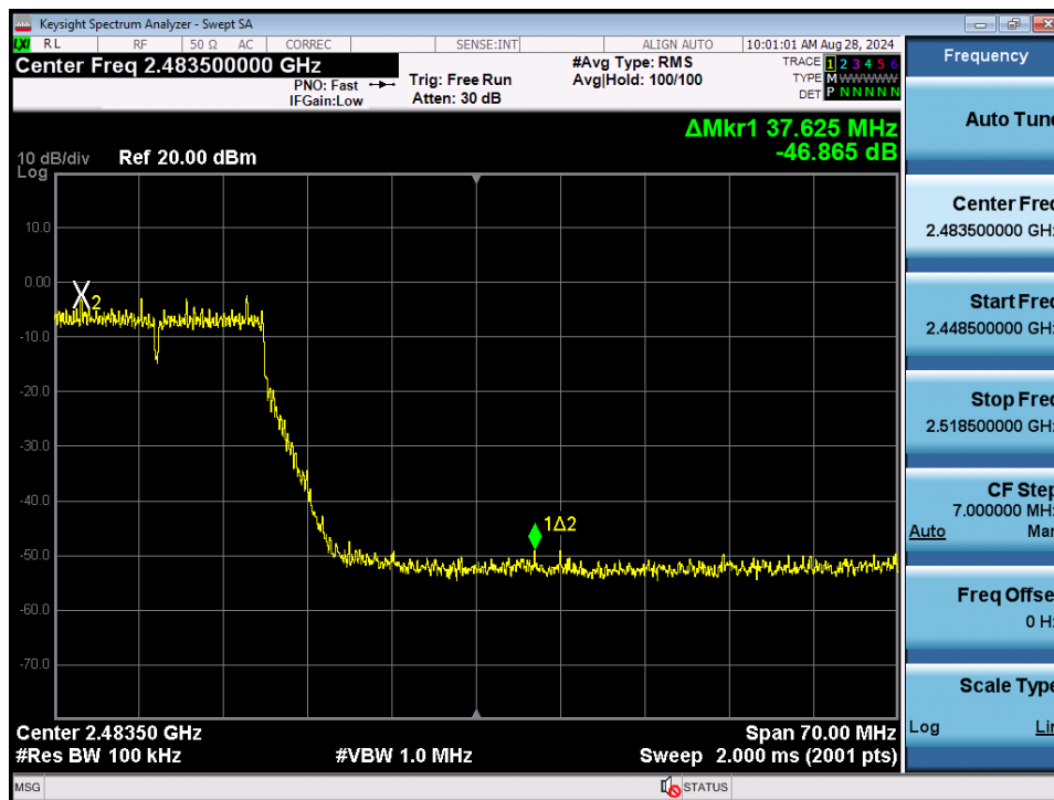
Plot 7-125. Band Edge Plot MIMO ANT2 (802.11n (2.4GHz) – Ch. 10)
