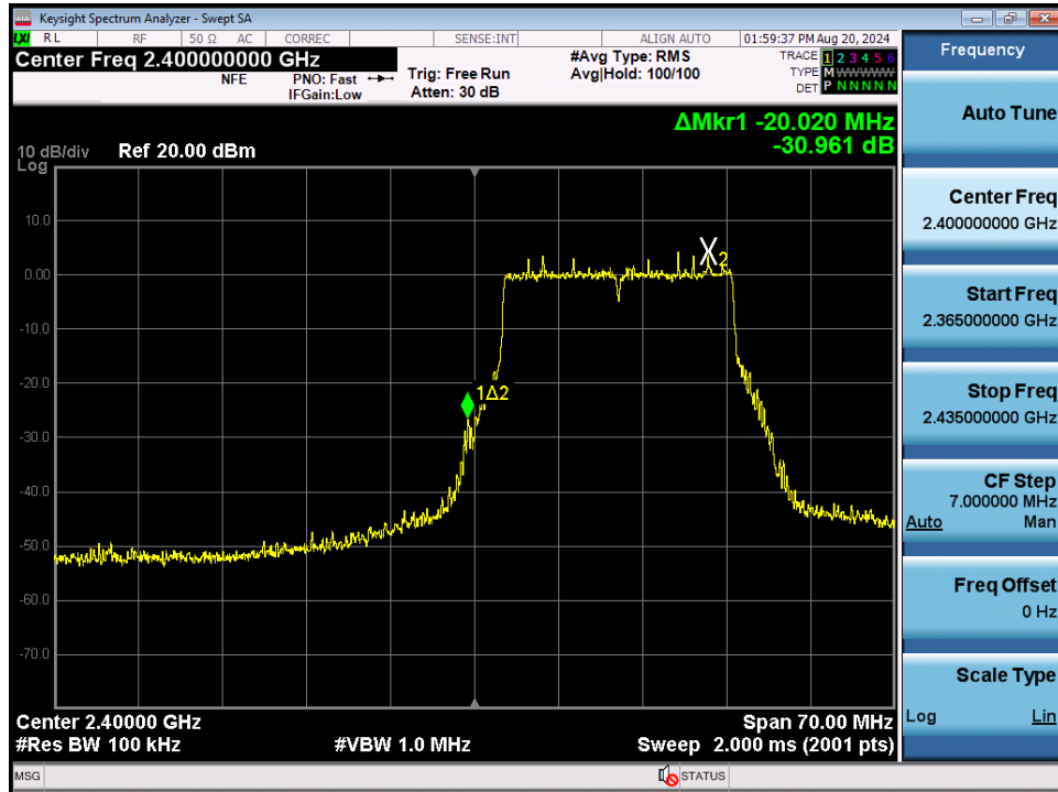
Plot 7-129. Band Edge Plot MIMO ANT2 (802.11ax/be (2.4GHz) – Ch. 1)
