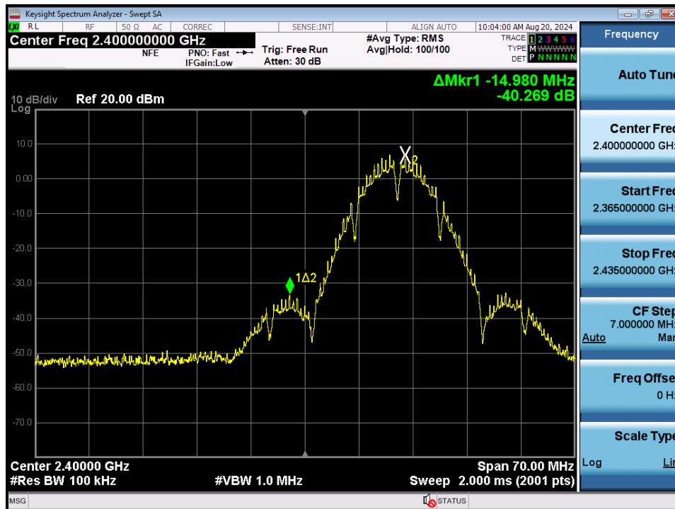
Plot 7-113. Band Edge Plot MIMO ANT2 (802.11b – Ch. 1)
