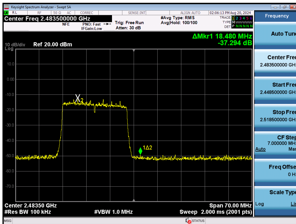
Plot 7-112. Band Edge Plot MIMO ANT1 (802.11ax/be (2.4GHz) – Ch. 13)
