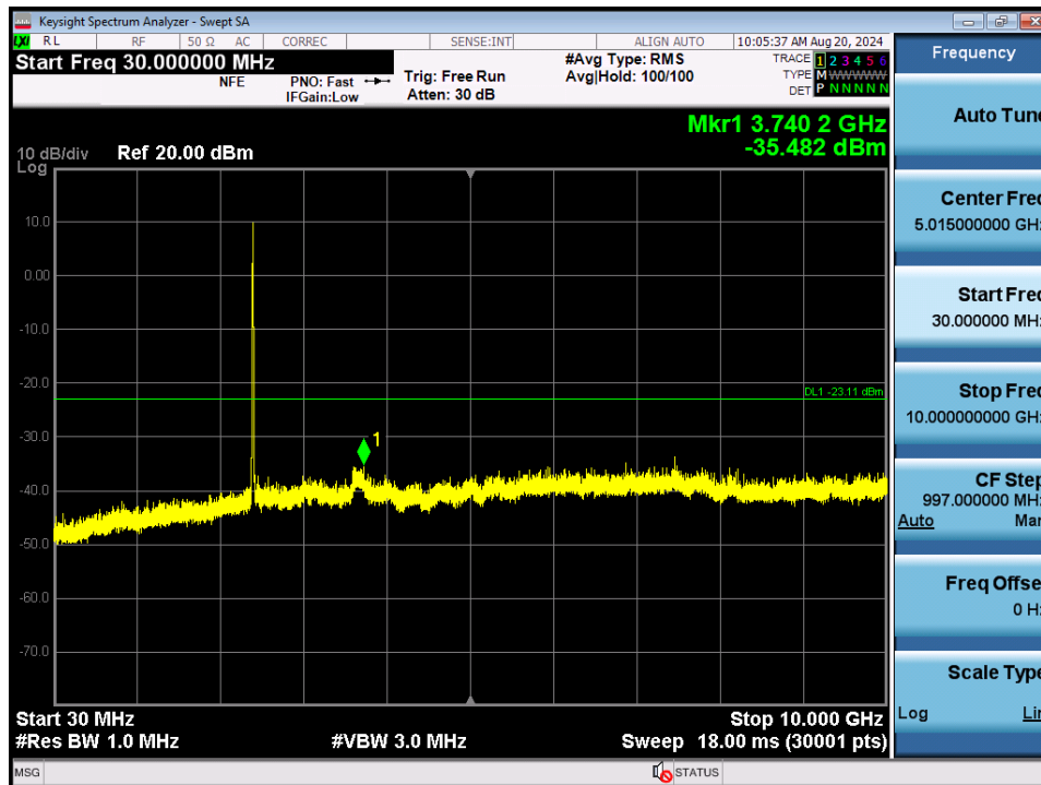
Plot 7-145. Conducted Spurious Plot MIMO ANT2 (802.11b – Ch. 1)
