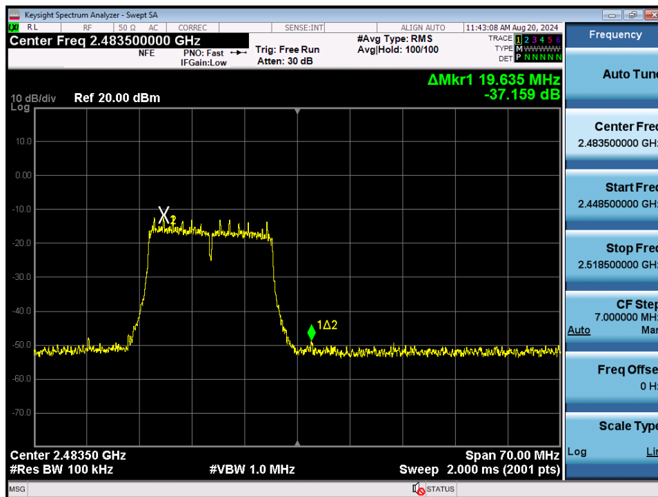
Plot 7-101. Band Edge Plot MIMO ANT1 (802.11g – Ch. 13)
