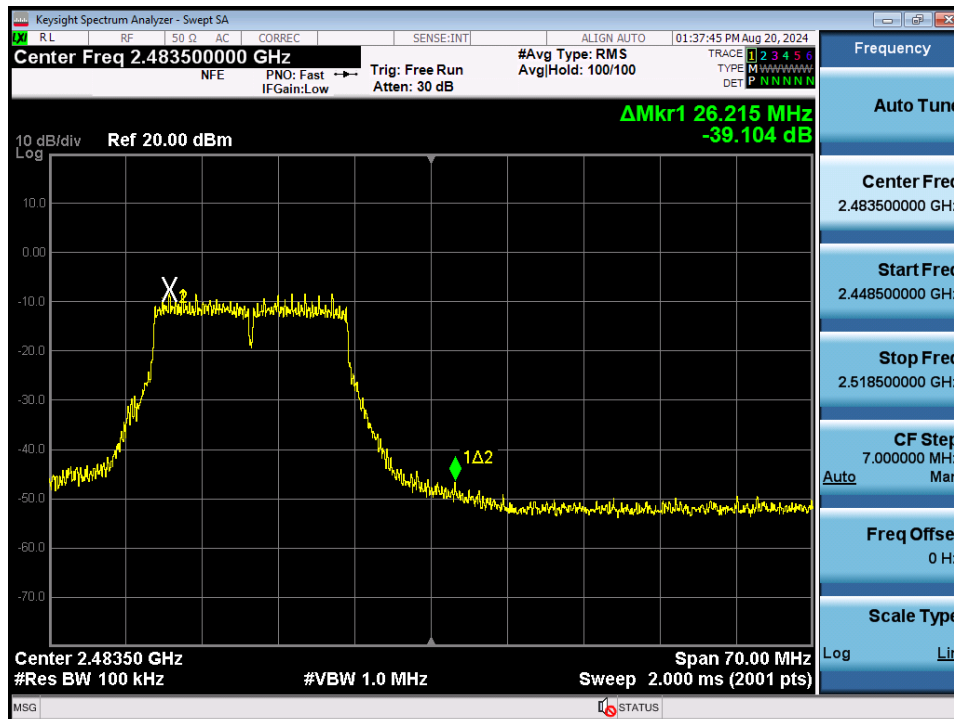
Plot 7-127. Band Edge Plot MIMO ANT2 (802.11n (2.4GHz) – Ch. 12)
