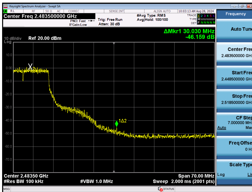
Plot 7-124. Band Edge Plot MIMO ANT2 (802.11n (2.4GHz) – Ch. 9)
