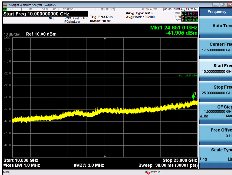
Plot 7-134. Conducted Spurious Plot SISO ANT2 (802.11b – Ch. 1)
