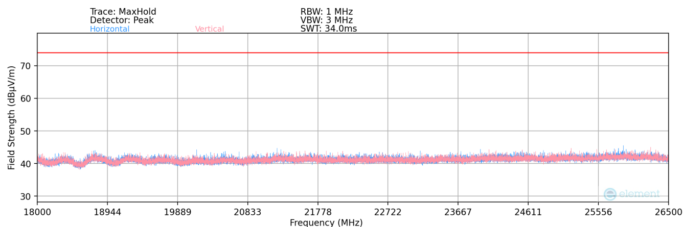
Plot 7-155. Radiated Spurious Plot above 18GHz SISO ANT2
