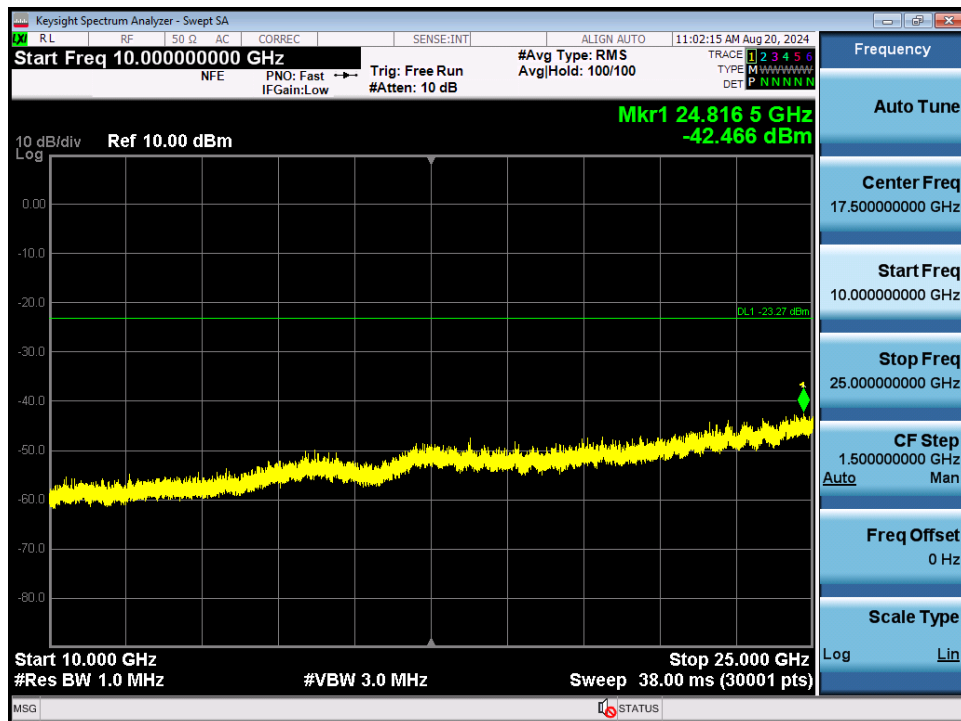
Plot 7-144. Conducted Spurious Plot MIMO ANT1 (802.11b – Ch. 11)
