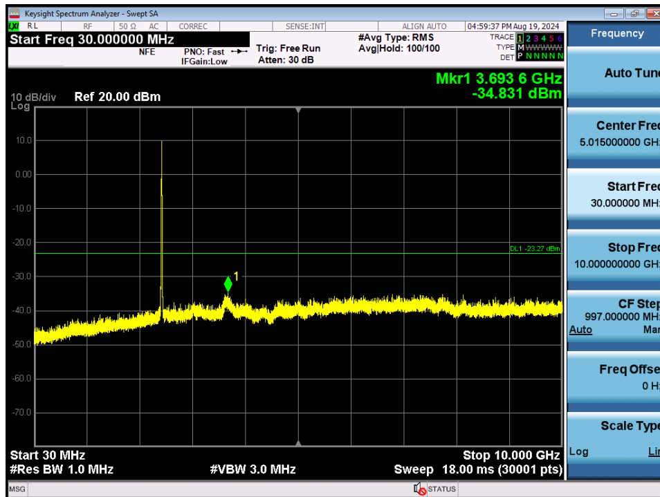
Plot 7-135. Conducted Spurious Plot SISO ANT2 (802.11b – Ch. 6)
