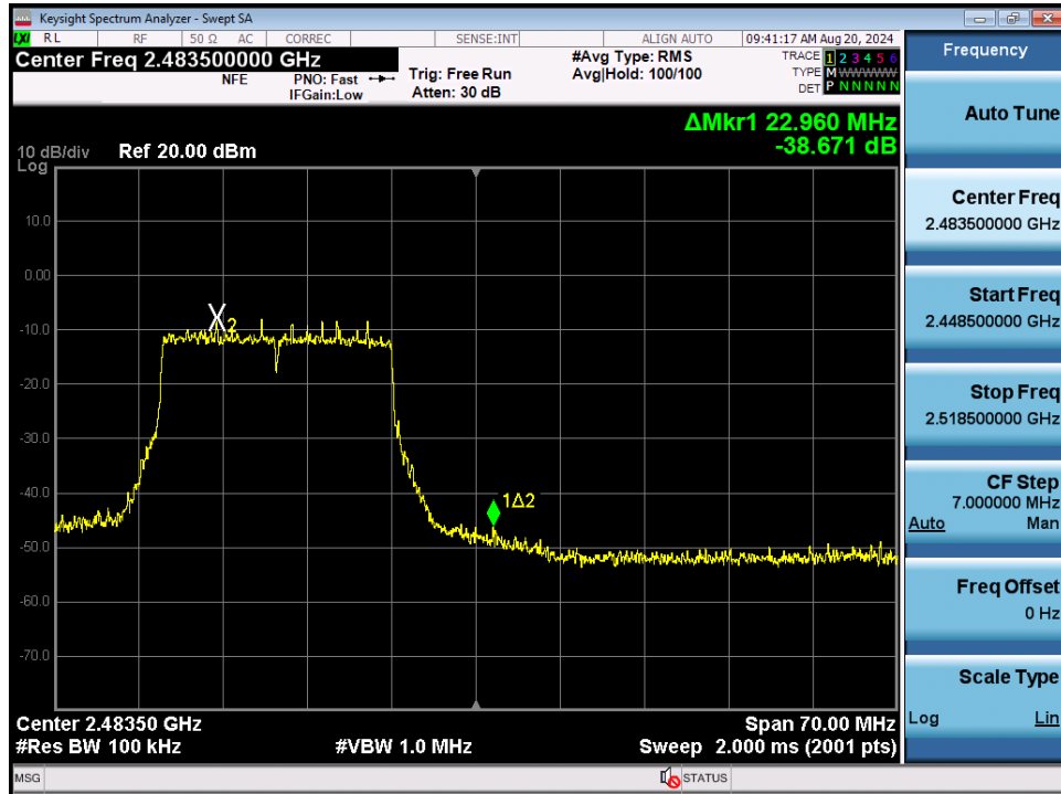
Plot 7-91. Band Edge Plot SISO ANT2 (802.11ax/be (2.4GHz) – Ch. 12)
