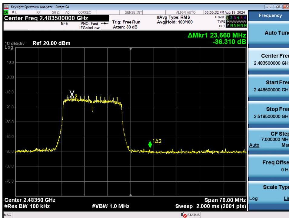
Plot 7-88. Band Edge Plot SISO ANT2 (802.11n (2.4GHz) – Ch. 13)
