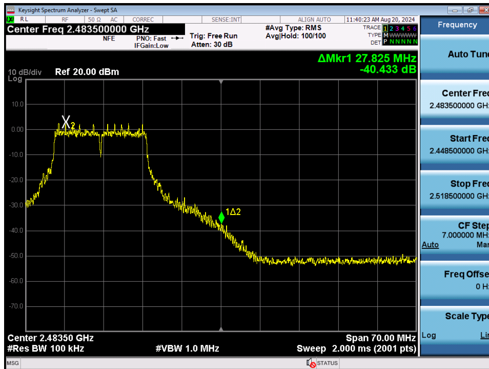
Plot 7-99. Band Edge Plot MIMO ANT1 (802.11g – Ch. 11)
