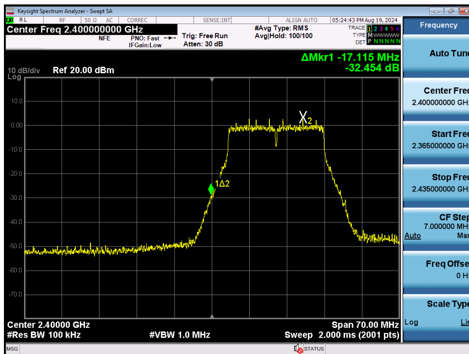
Plot 7-82. Band Edge Plot SISO ANT2 (802.11n (2.4GHz) – Ch. 1)
