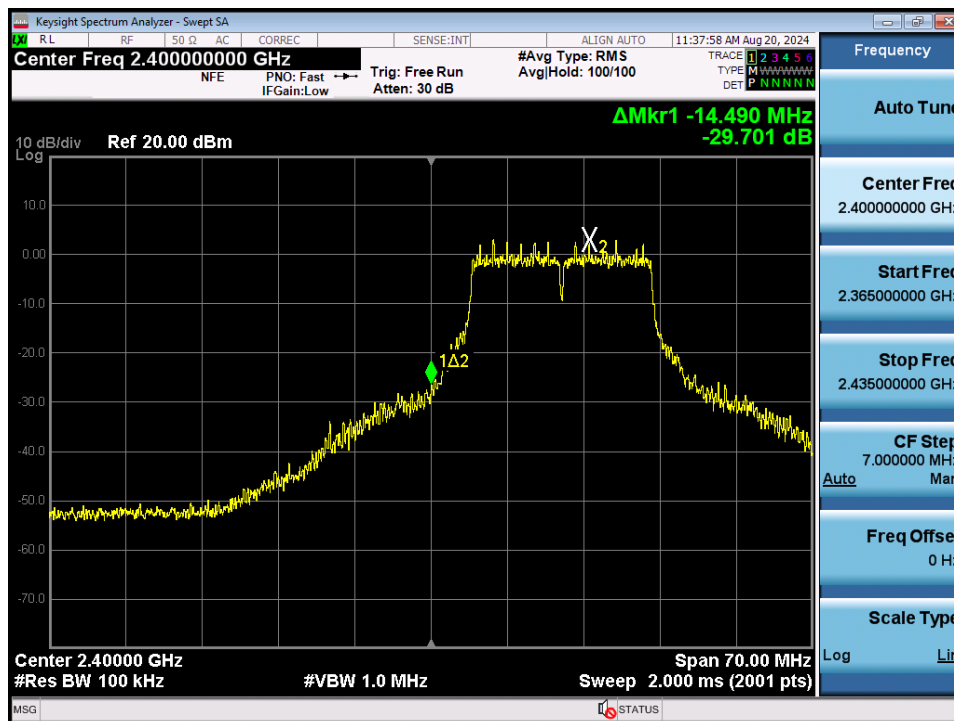
Plot 7-97. Band Edge Plot MIMO ANT1 (802.11g- Ch. 1)
