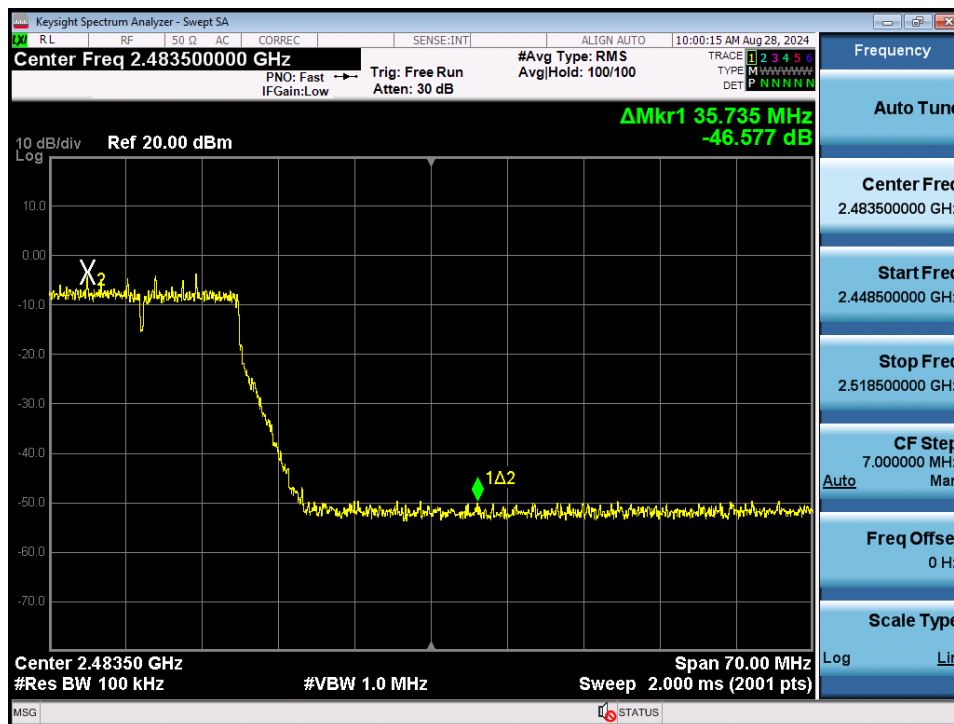
Plot 7-105. Band Edge Plot MIMO ANT1 (802.11n (2.4GHz) – Ch. 10)
