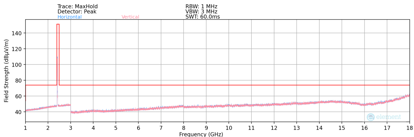
Plot 7-152. Radiated Spurious Plot above 1GHz SISO ANT2 (802.11b – Ch. 1)
