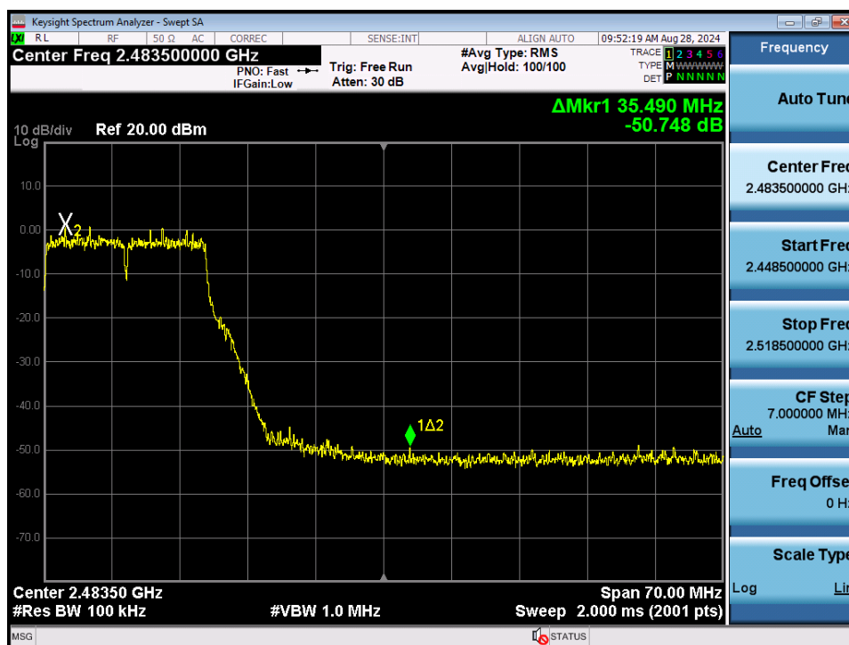
Plot 7-98. Band Edge Plot MIMO ANT1 (802.11g - Ch. 10)
