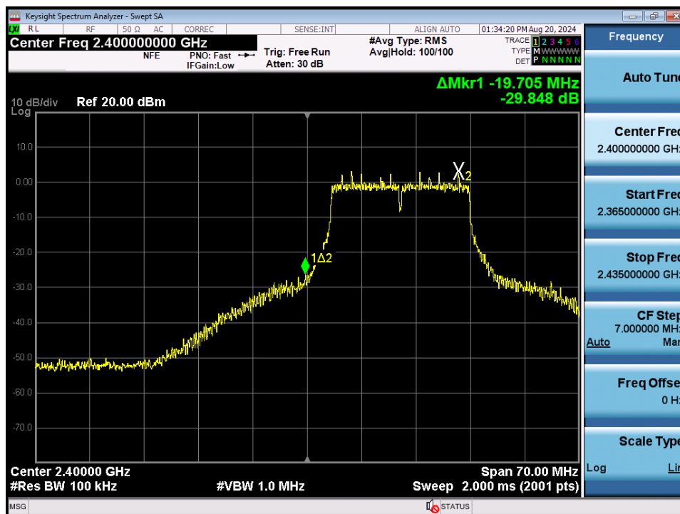
Plot 7-102. Band Edge Plot MIMO ANT1 (802.11n (2.4GHz) – Ch. 1)
