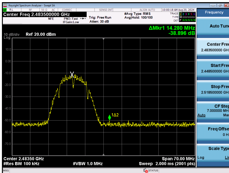
Plot 7-96. Band Edge Plot MIMO ANT1 (802.11b – Ch. 13)
