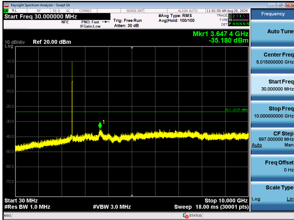
Plot 7-143. Conducted Spurious Plot MIMO ANT1 (802.11b – Ch. 11)
