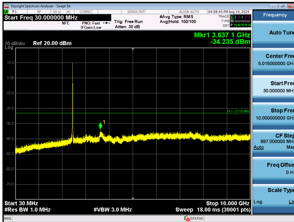
Plot 7-137. Conducted Spurious Plot SISO ANT2 (802.11b – Ch. 11)
