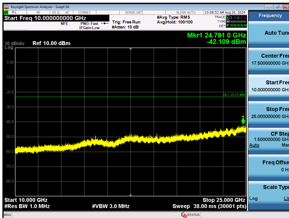
Plot 7-150. Conducted Spurious Plot MIMO ANT2 (802.11b – Ch. 11)
