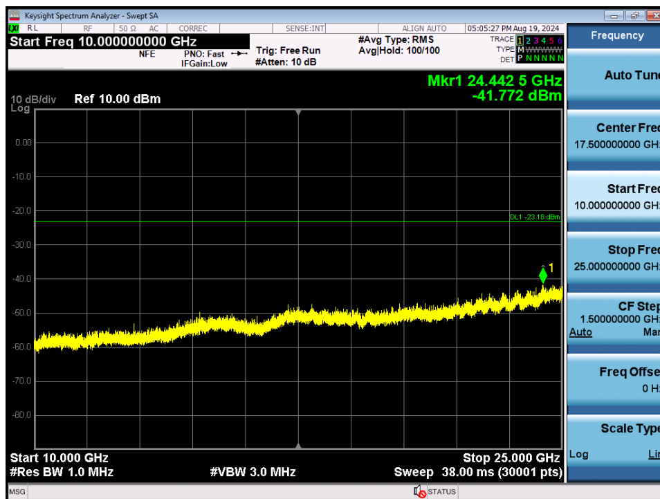
Plot 7-138. Conducted Spurious Plot SISO ANT2 (802.11b – Ch. 11)
