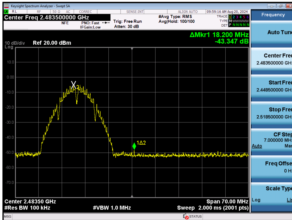
Plot 7-95. Band Edge Plot MIMO ANT1 (802.11b – Ch. 12)
