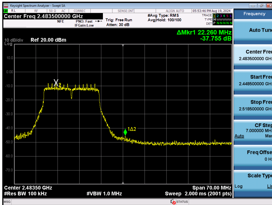
Plot 7-87. Band Edge Plot SISO ANT2 (802.11n (2.4GHz) – Ch. 12)
