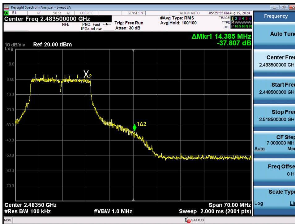
Plot 7-86. Band Edge Plot SISO ANT2 (802.11n (2.4GHz) – Ch. 11)
