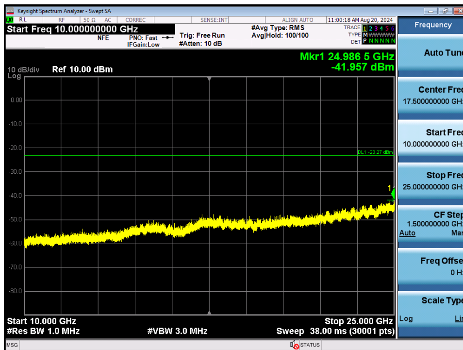
Plot 7-142. Conducted Spurious Plot MIMO ANT1 (802.11b – Ch. 6)
