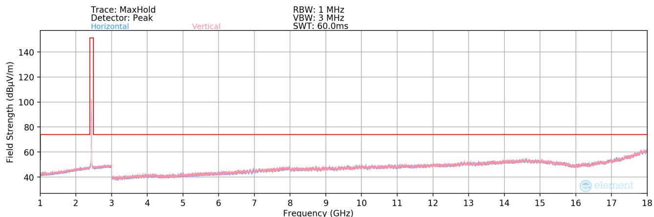
Plot 7-153. Radiated Spurious Plot above 1GHz SISO ANT2 (802.11b – Ch. 6)
