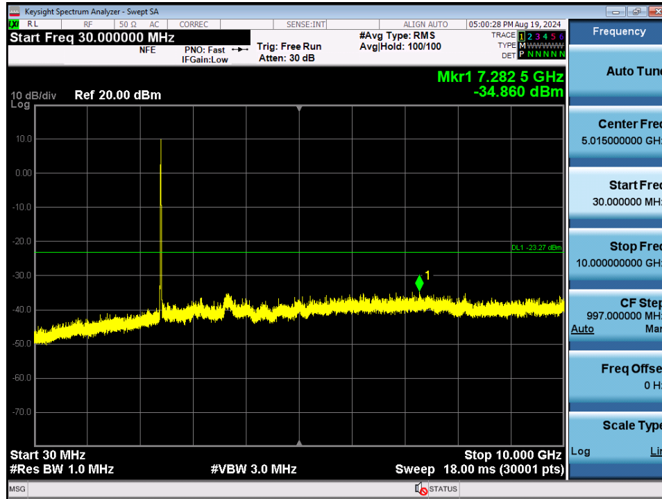
Plot 7-133. Conducted Spurious Plot SISO ANT2 (802.11b – Ch. 1)
