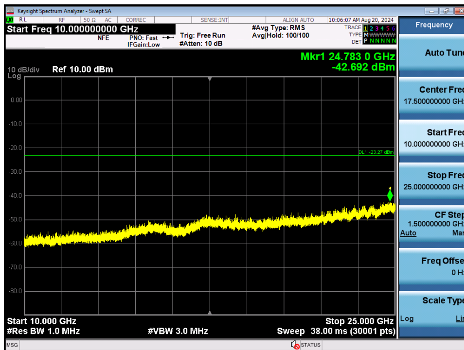
Plot 7-146. Conducted Spurious Plot MIMO ANT2 (802.11b – Ch. 1)
