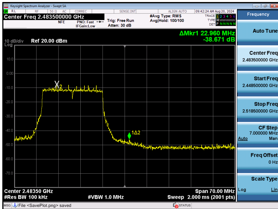
Plot 7-92. Band Edge Plot SISO ANT2 (802.11ax/be (2.4GHz) – Ch. 13)
