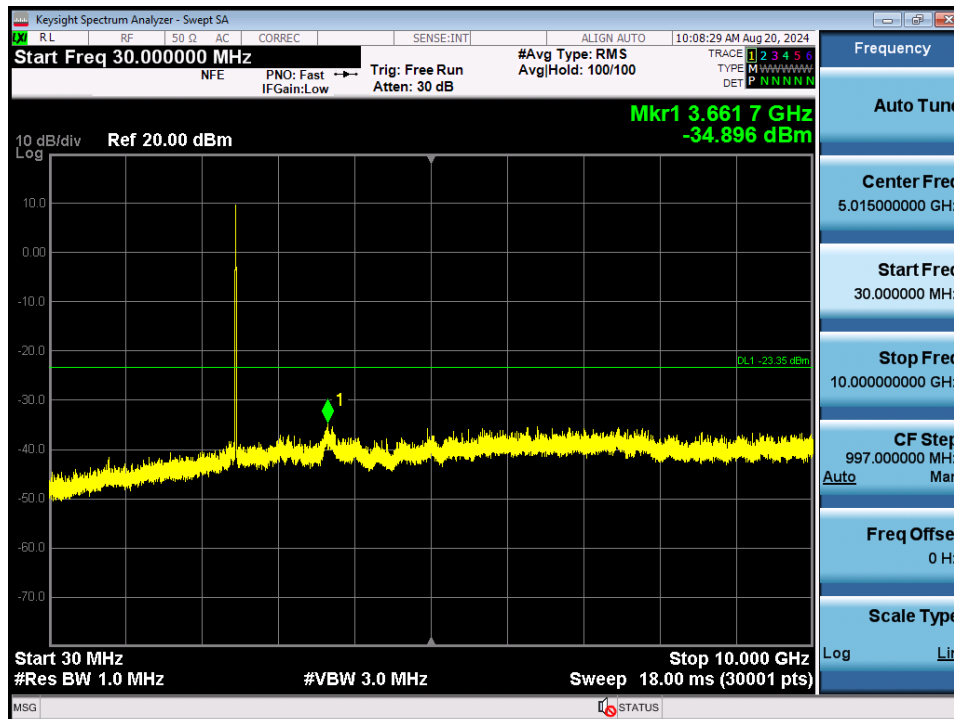
Plot 7-149. Conducted Spurious Plot MIMO ANT2 (802.11b – Ch. 11)
