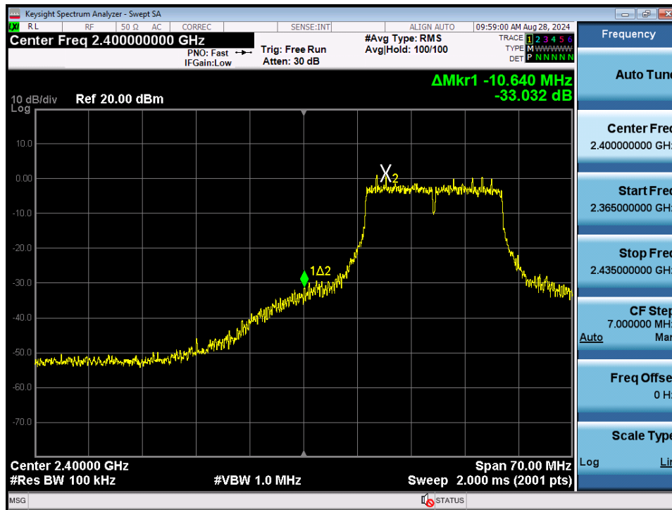
Plot 7-103. Band Edge Plot MIMO ANT1 (802.11n (2.4GHz) – Ch. 2)
