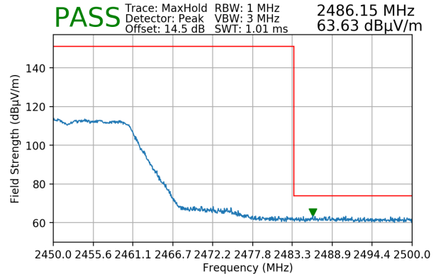
Plot 7-180. Radiated Restricted Lower Band Edge Measurement MIMO (Peak)
