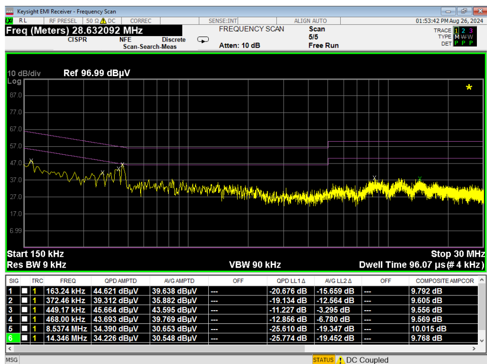
Plot 7-190. Line Conducted Plot with 802.11b (N)
