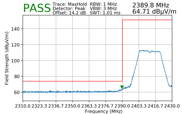
Plot 7-176. Radiated Restricted Lower Band Edge Measurement MIMO (Peak)
