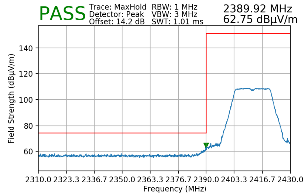
Plot 7-162. Radiated Restricted Lower Band Edge Measurement SISO ANT2 (Peak)
