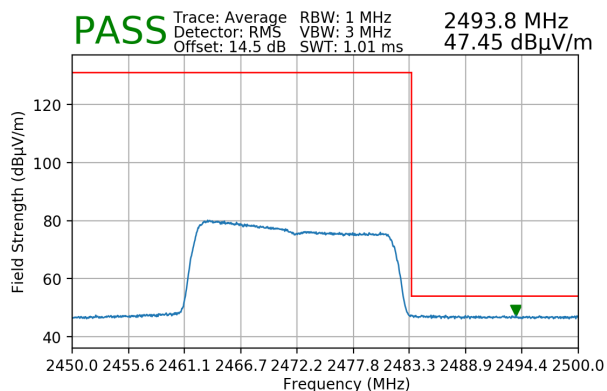
Plot 7-173. Radiated Restricted Upper Band Edge Measurement SISO ANT2 (Average)
