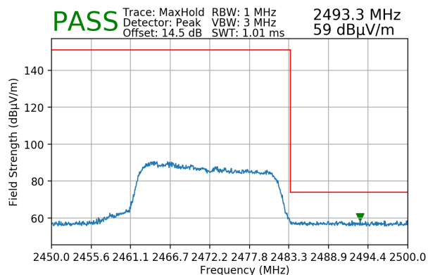
Plot 7-174. Radiated Restricted Upper Band Edge Measurement SISO ANT2 (Peak)
