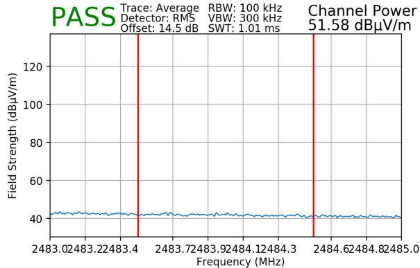
Plot 7-183. Radiated Restricted Upper Band Edge Measurement MIMO (Average)
