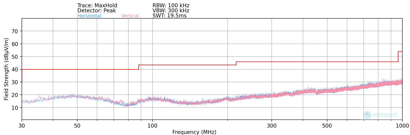
Plot 7-156. Radiated Spurious Plot below 1GHz MIMO
