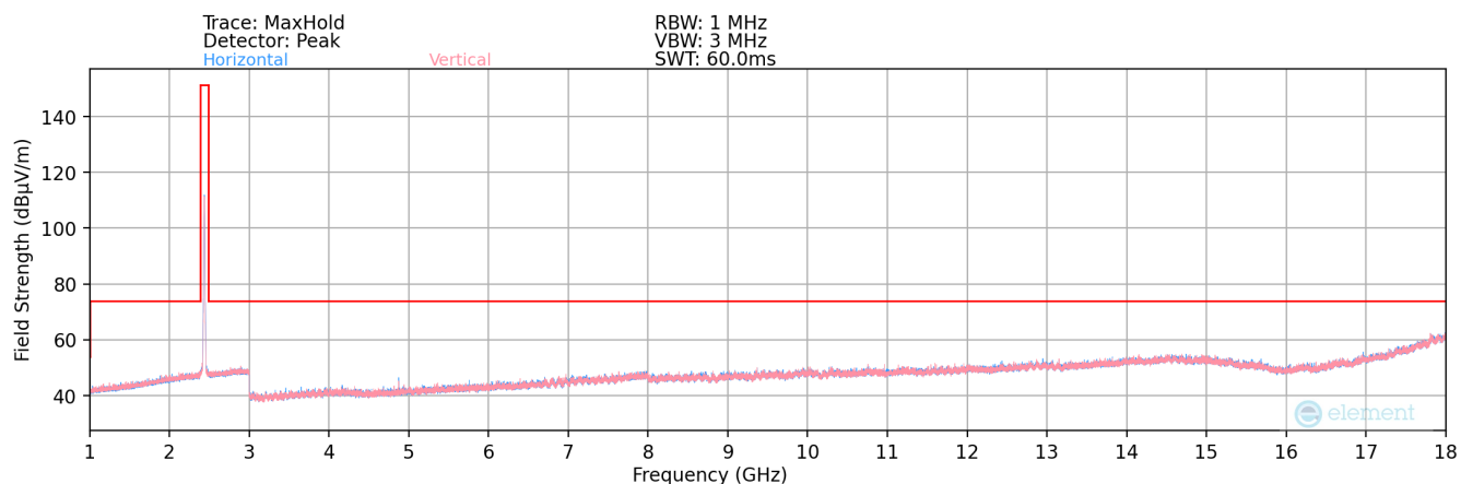
Plot 7-158. Radiated Spurious Plot above 1GHz MIMO (802.11b – Ch. 6)
