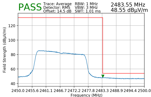
Plot 7-171. Radiated Restricted Upper Band Edge Measurement SISO ANT2 (Average)
