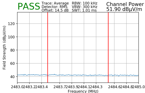
Plot 7-169. Radiated Restricted Upper Band Edge Measurement SISO ANT2 (Average)
