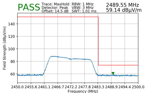
Plot 7-188. Radiated Restricted Upper Band Edge Measurement MIMO (Peak)
