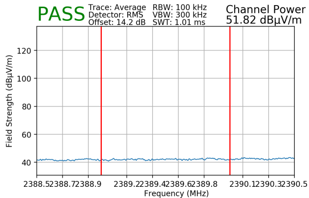
Plot 7-175. Radiated Restricted Lower Band Edge Measurement MIMO (Average)
