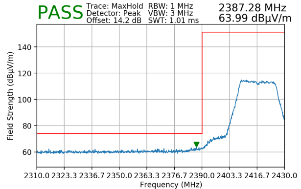
Plot 7-182. Radiated Restricted Lower Band Edge Measurement MIMO (Peak)
