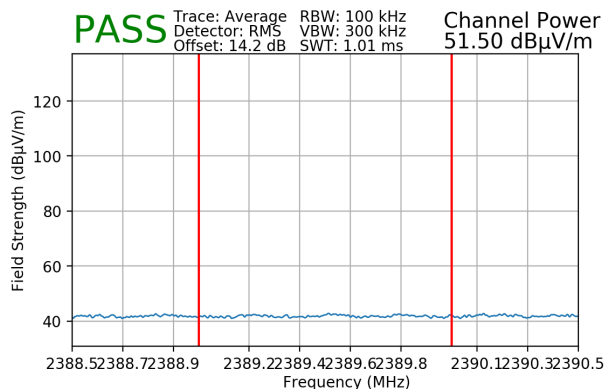
Plot 7-163. Radiated Restricted Lower Band Edge Measurement SISO ANT2 (Average)
