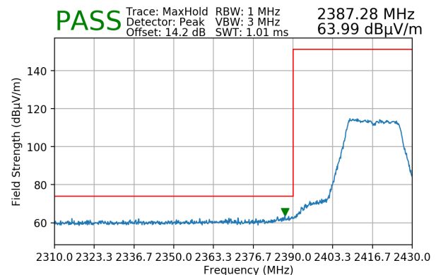
Plot 7-178. Radiated Restricted Lower Band Edge Measurement MIMO (Peak)
