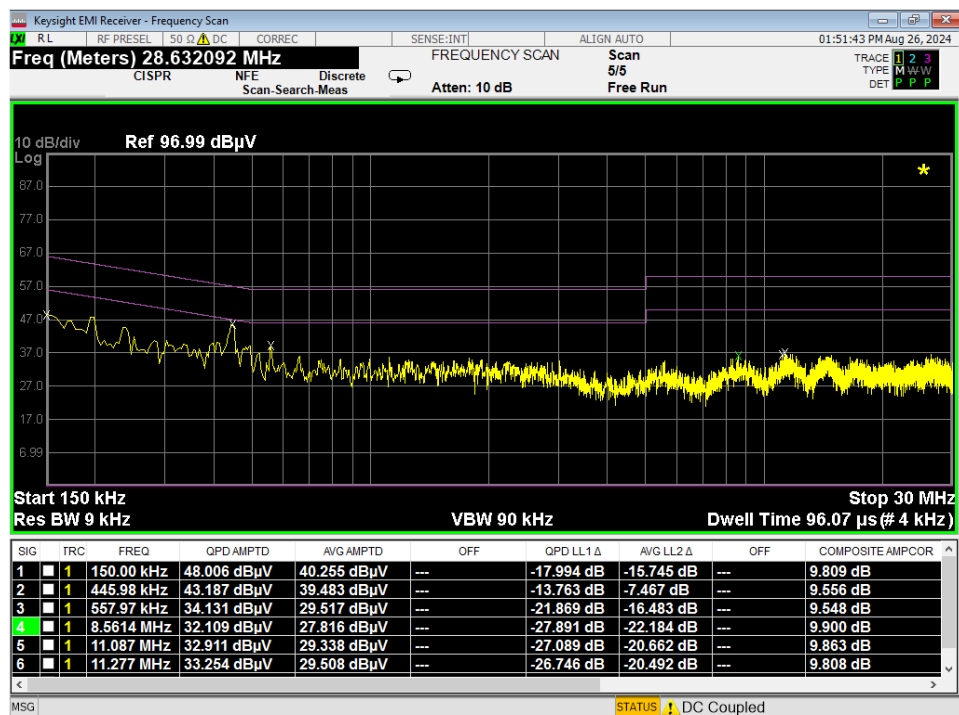
Plot 7-189. Line Conducted Plot with 802.11b (L1)
