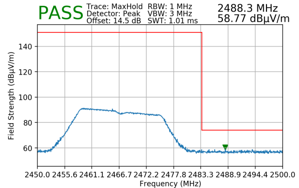
Plot 7-186. Radiated Restricted Upper Band Edge Measurement MIMO (Peak)
