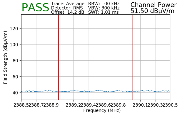
Plot 7-181. Radiated Restricted Lower Band Edge Measurement MIMO (Average)
