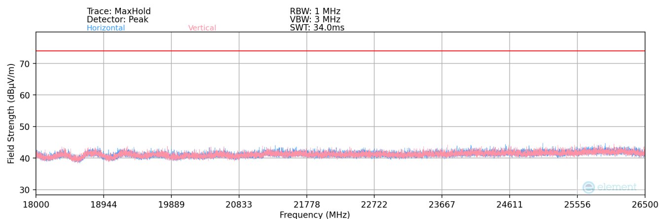
Plot 7-160. Radiated Spurious Plot above 18GHz MIMO
