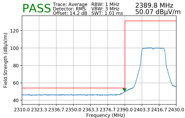
Plot 7-161. Radiated Restricted Lower Band Edge Measurement SISO ANT2 (Average)
