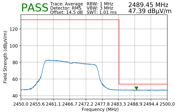
Plot 7-185. Radiated Restricted Upper Band Edge Measurement MIMO (Average)
