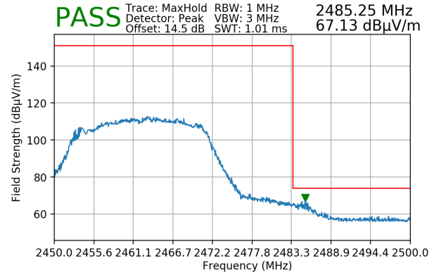
Plot 7-184. Radiated Restricted Upper Band Edge Measurement MIMO (Peak)
