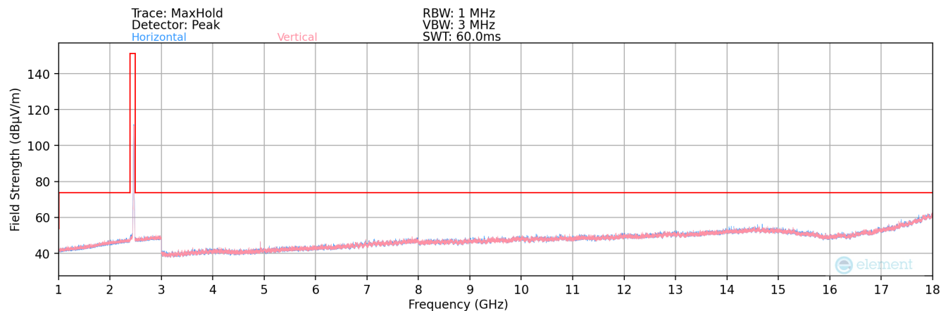
Plot 7-159. Radiated Spurious Plot above 1GHz MIMO (802.11b – Ch. 11)
