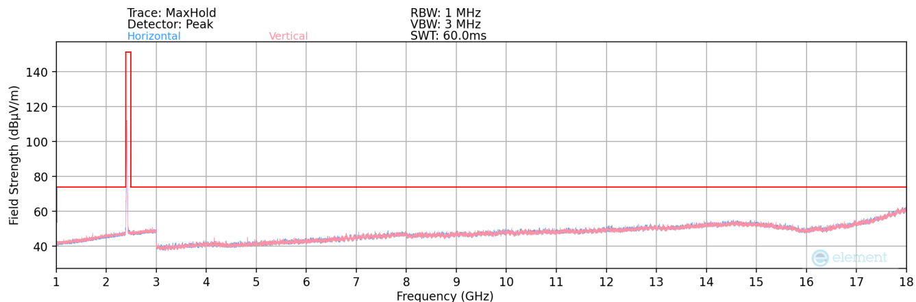
Plot 7-157. Radiated Spurious Plot above 1GHz MIMO (802.11b – Ch. 1)
