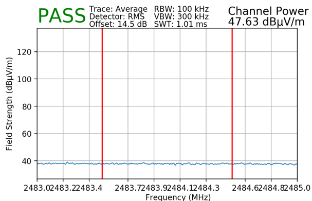
Plot 7-187. Radiated Restricted Upper Band Edge Measurement MIMO (Average)
