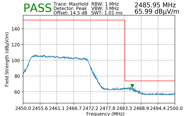
Plot 7-170. Radiated Restricted Upper Band Edge Measurement SISO ANT2 (Peak)
