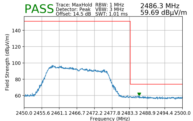
Plot 7-172. Radiated Restricted Upper Band Edge Measurement SISO ANT2 (Peak)
