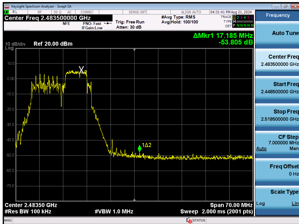
Plot 7-42. Band Edge Plot SISO ANT2 (802.11be OFDMA – 52+26 Tones – Ch. 11)
