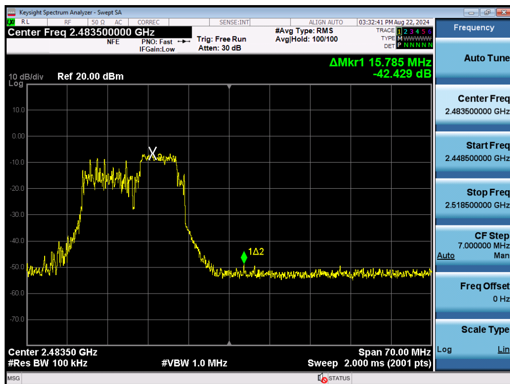
Plot 7-59. Band Edge Plot MIMO ANT1 (802.11be OFDMA – 52+26 Tones – Ch. 12)
