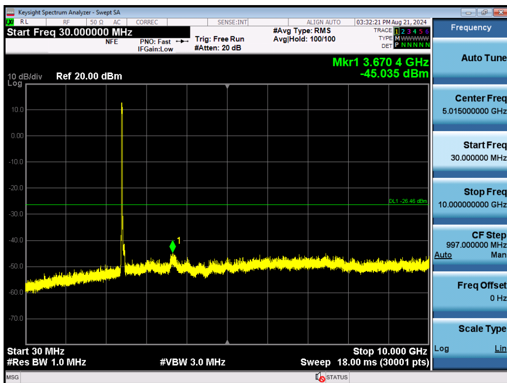
Plot 7-91. Conducted Spurious Plot SISO ANT2 (802.11ax OFDMA – 242 Tones – Ch. 1)
