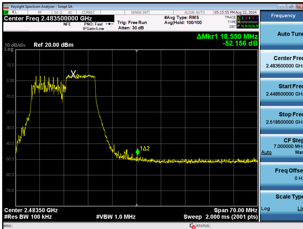
Plot 7-70. Band Edge Plot MIMO ANT2 (802.11ax OFDMA – 106 Tones – Ch. 11)
