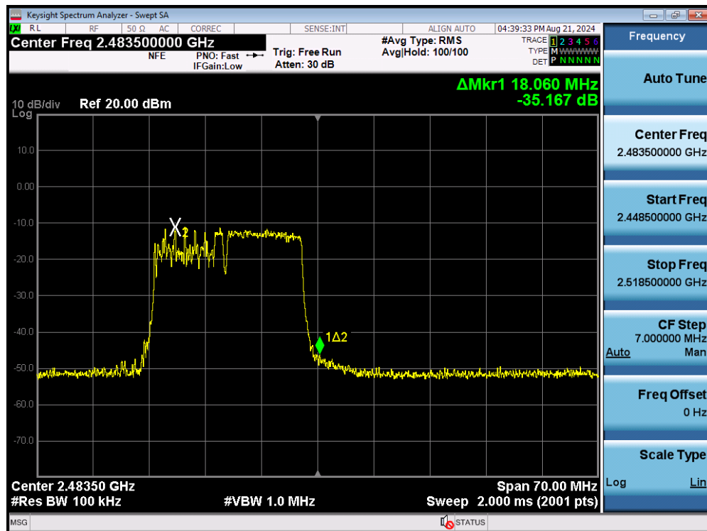
Plot 7-48. Band Edge Plot SISO ANT2 (802.11be OFDMA – 106+26 Tones – Ch. 13)
