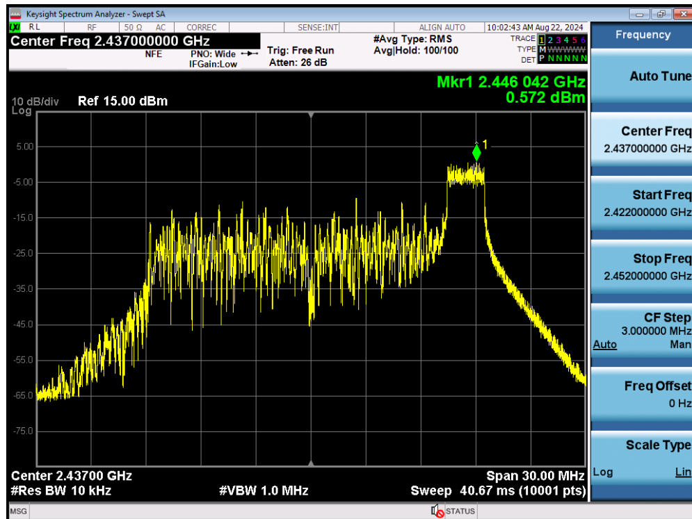
Plot 7-26. Power Spectral Density Plot MIMO ANT2 (802.11ax OFDMA – 26 Tones – Ch. 6)
