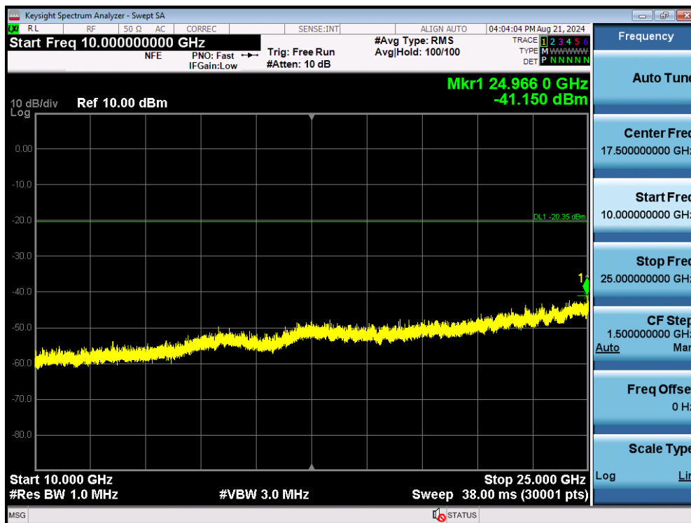
Plot 7-86. Conducted Spurious Plot SISO ANT2 (802.11ax OFDMA – 26 Tones – Ch. 1)
