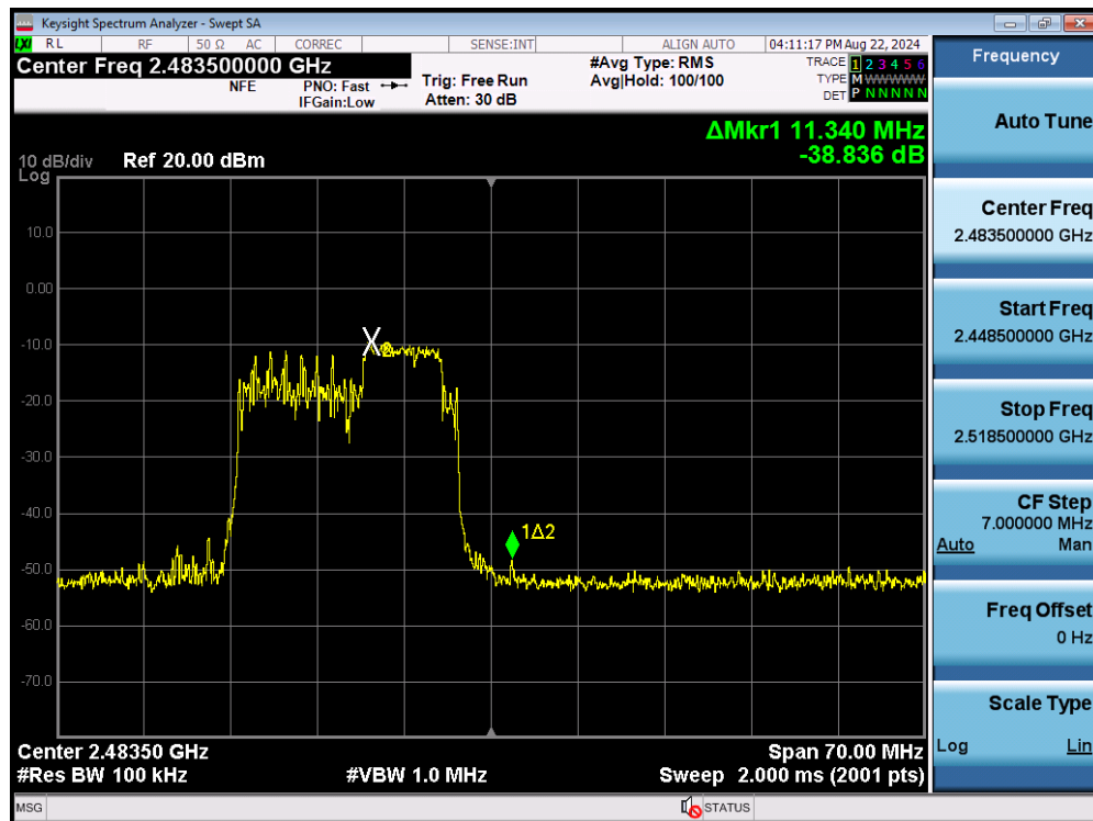
Plot 7-76. Band Edge Plot MIMO ANT2 (802.11be OFDMA – 52+26 Tones – Ch. 13)
