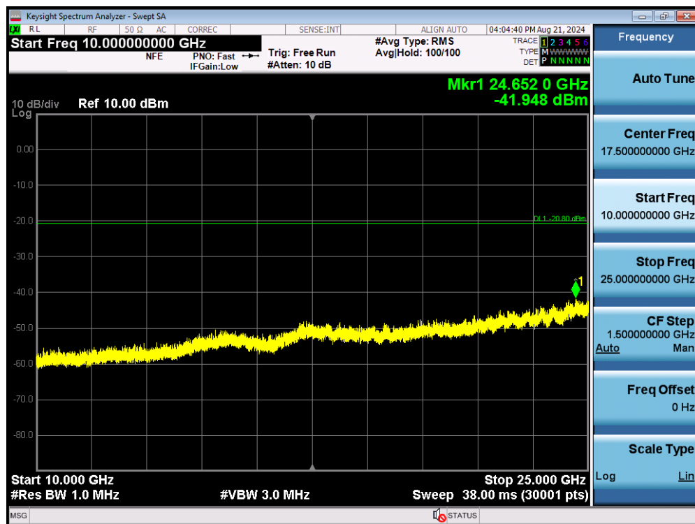
Plot 7-88. Conducted Spurious Plot SISO ANT2 (802.11ax OFDMA – 26 Tones – Ch. 6)
