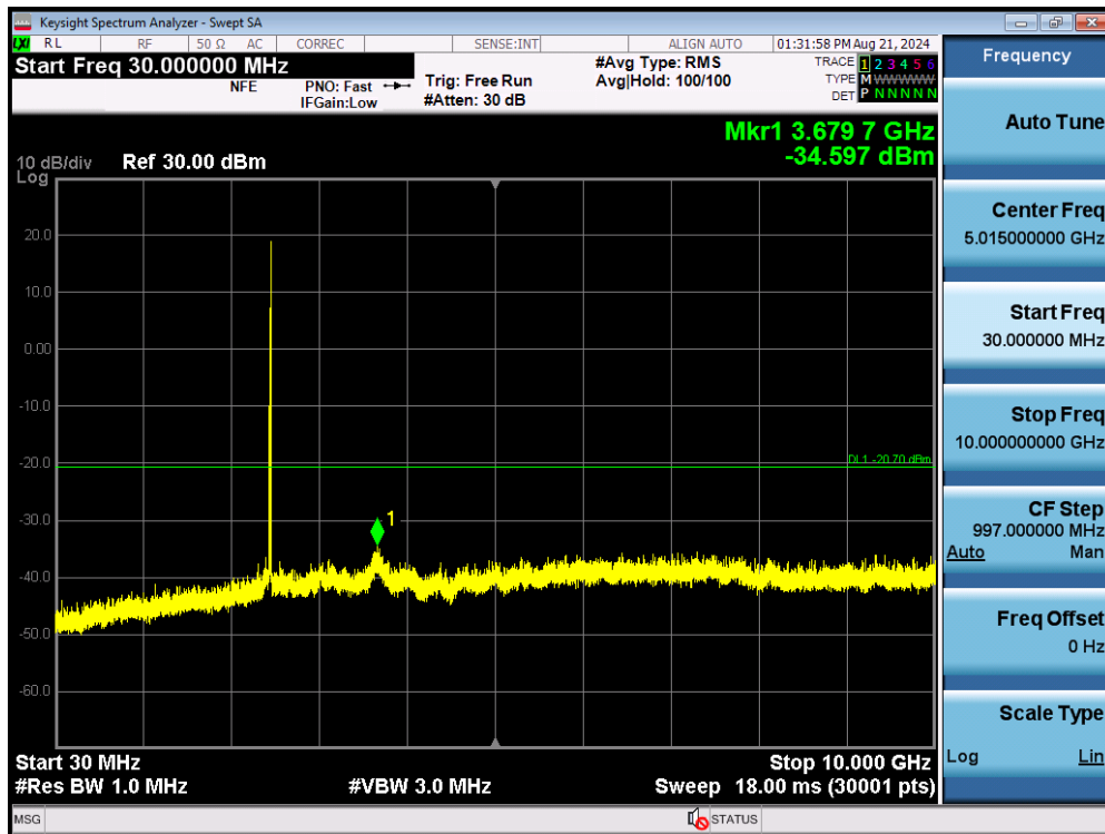
Plot 7-89. Conducted Spurious Plot SISO ANT2 (802.11ax OFDMA – 26 Tones – Ch. 11)
