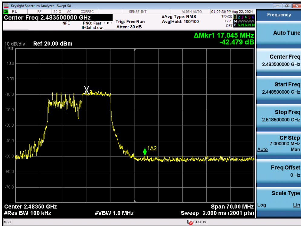
Plot 7-55. Band Edge Plot MIMO ANT1 (802.11ax OFDMA – 106 Tones – Ch. 12)
