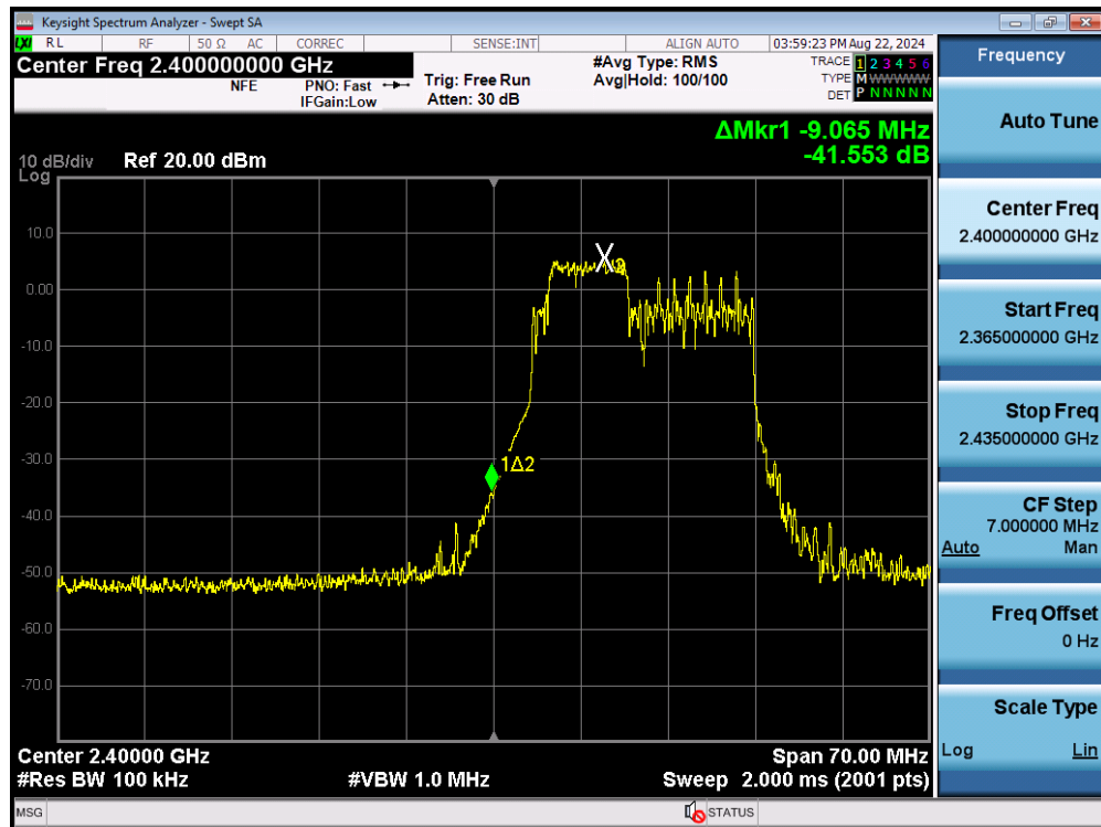
Plot 7-73. Band Edge Plot MIMO ANT2 (802.11be OFDMA – 52+26 Tones – Ch. 1)
