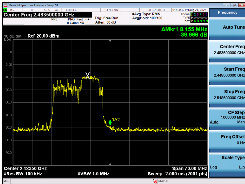
Plot 7-44. Band Edge Plot SISO ANT2 (802.11be OFDMA – 52+26 Tones – Ch. 13)
