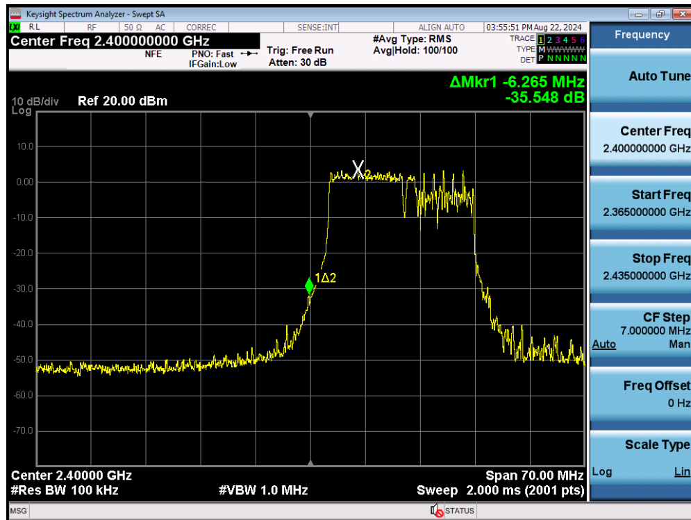
Plot 7-77. Band Edge Plot MIMO ANT2 (802.11be OFDMA – 106+26 Tones – Ch. 1)
