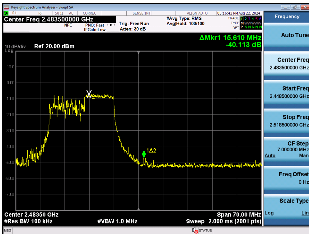
Plot 7-71. Band Edge Plot MIMO ANT2 (802.11ax OFDMA – 106 Tones – Ch. 12)
