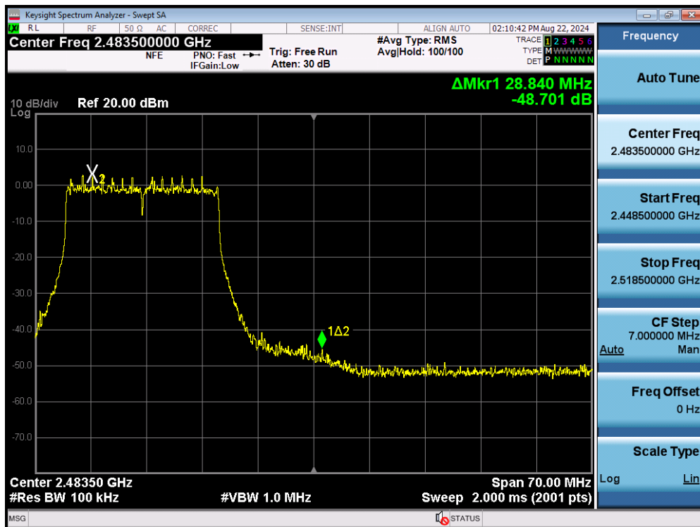
Plot 7-66. Band Edge Plot MIMO ANT1 (802.11ax OFDMA – 242 Tones – Ch. 11)
