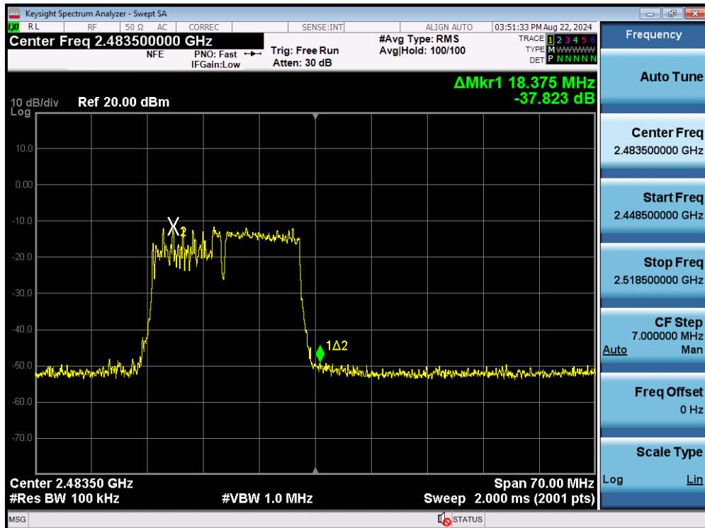
Plot 7-64. Band Edge Plot MIMO ANT1 (802.11be OFDMA – 106+26 Tones – Ch. 13)
