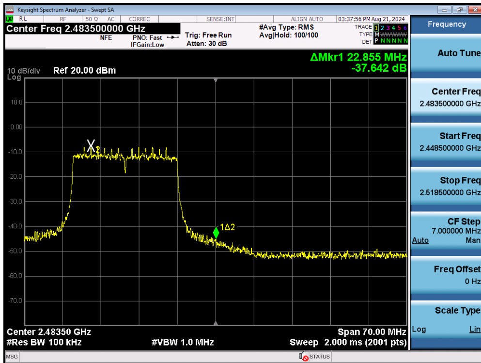
Plot 7-51. Band Edge Plot SISO ANT2 (802.11ax OFDMA – 242 Tones – Ch. 12)
