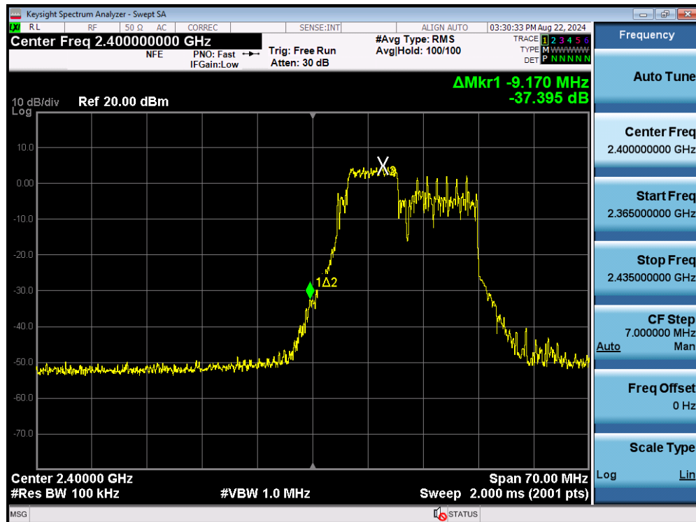
Plot 7-57. Band Edge Plot MIMO ANT1 (802.11be OFDMA – 52+26 Tones – Ch. 1)
