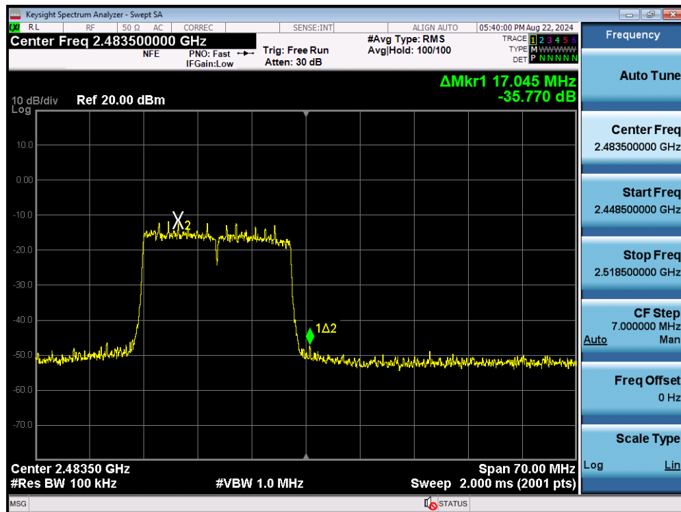
Plot 7-84. Band Edge Plot MIMO ANT2 (802.11ax OFDMA – 242 Tones – Ch. 13)
