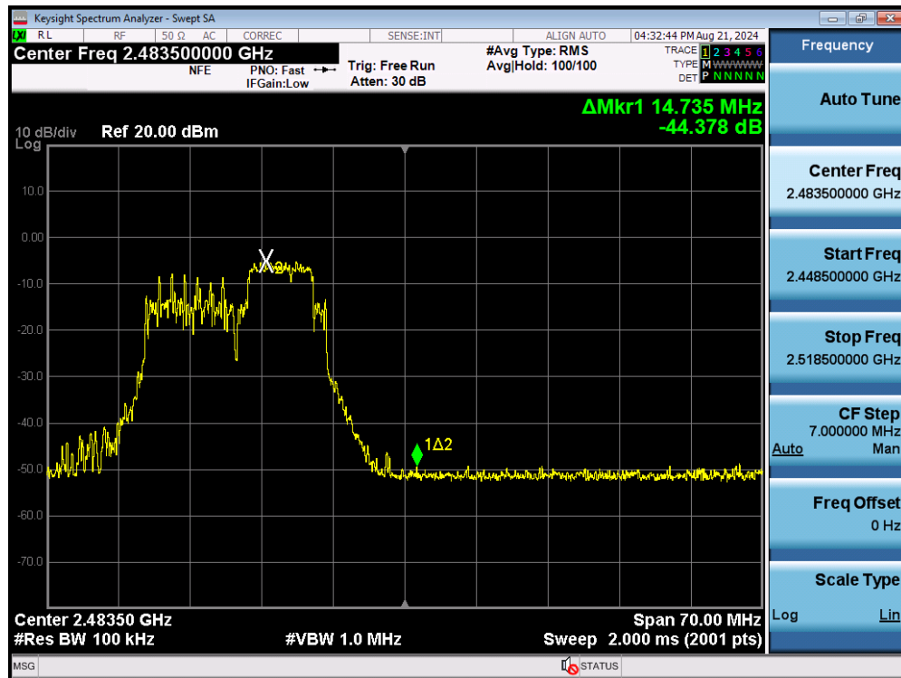
Plot 7-43. Band Edge Plot SISO ANT2 (802.11be OFDMA – 52+26 Tones – Ch. 12)
