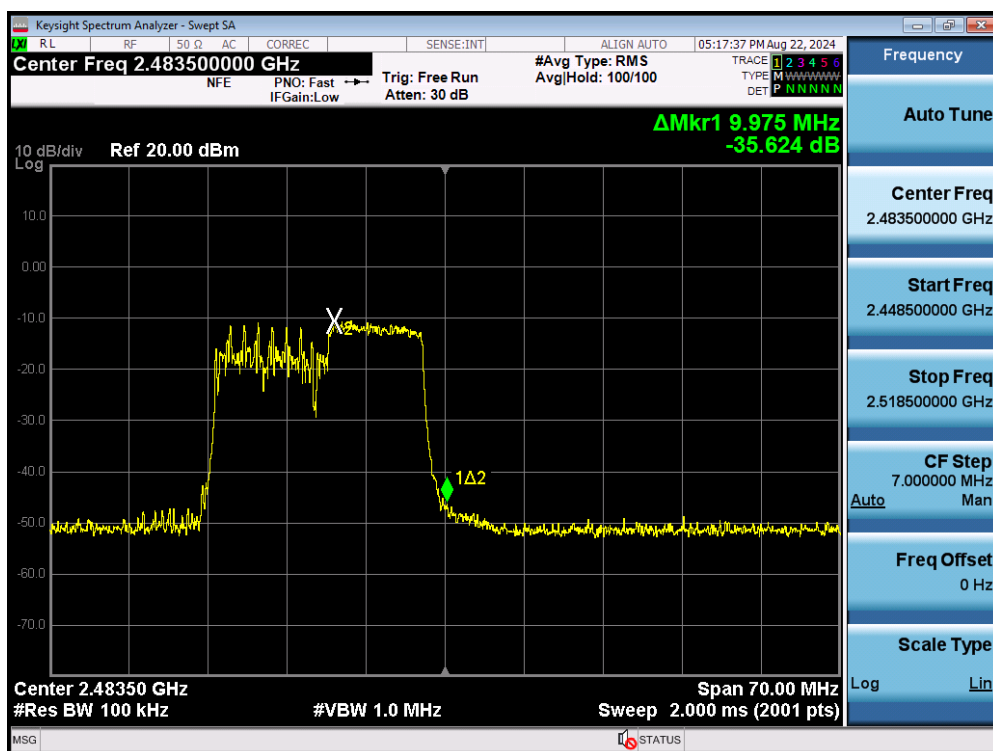
Plot 7-72. Band Edge Plot MIMO ANT2 (802.11ax OFDMA – 106 Tones – Ch. 13)
