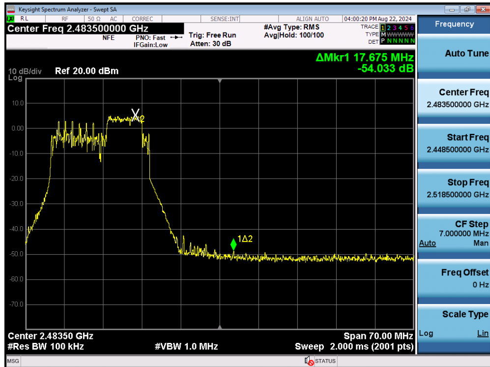
Plot 7-74. Band Edge Plot MIMO ANT2 (802.11be OFDMA – 52+26 Tones – Ch. 11)
