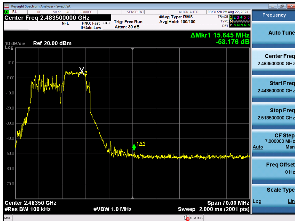
Plot 7-58. Band Edge Plot MIMO ANT1 (802.11be OFDMA – 52+26 Tones – Ch. 11)
