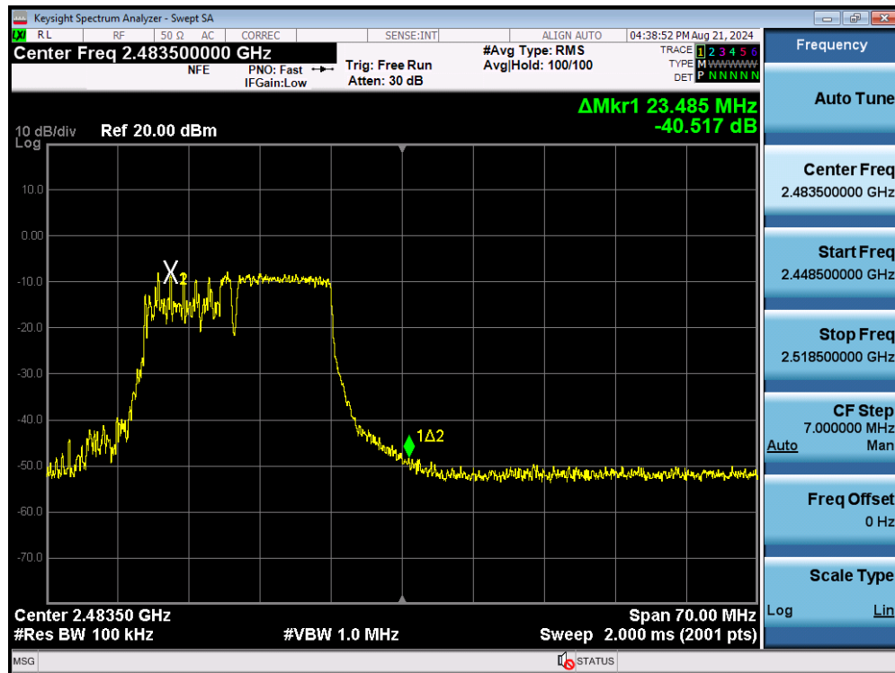
Plot 7-47. Band Edge Plot SISO ANT2 (802.11be OFDMA – 106+26 Tones – Ch. 12)
