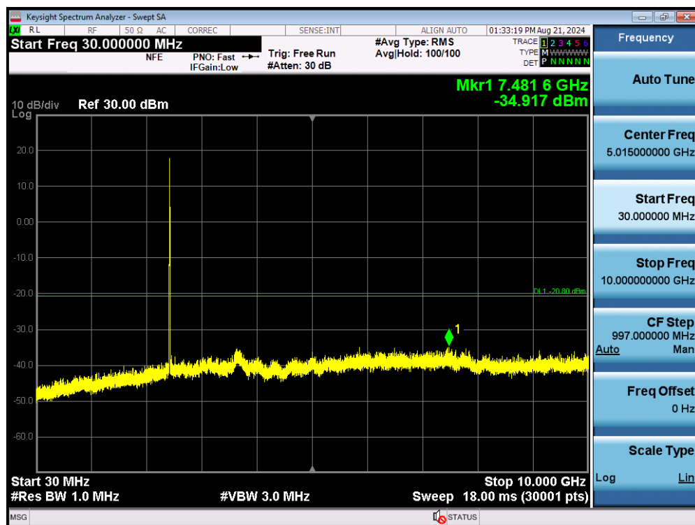
Plot 7-87. Conducted Spurious Plot SISO ANT2 (802.11ax OFDMA – 26 Tones – Ch. 6)
