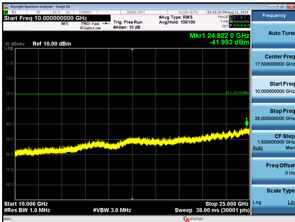
Plot 7-90. Conducted Spurious Plot SISO ANT2 (802.11ax OFDMA – 26 Tones – Ch. 11)
