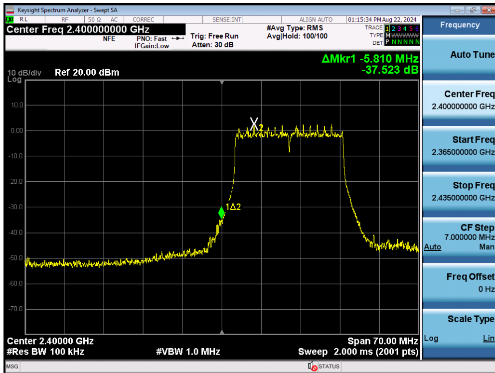
Plot 7-65. Band Edge Plot MIMO ANT1 (802.11ax OFDMA – 242 Tones – Ch. 1)
