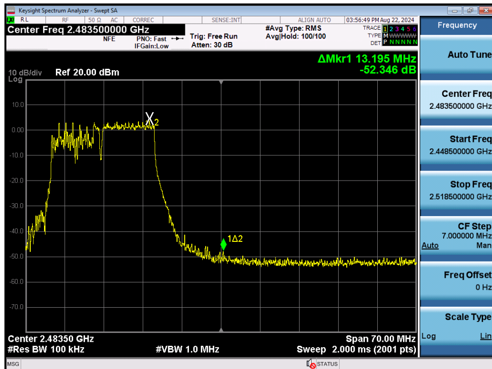
Plot 7-78. Band Edge Plot MIMO ANT2 (802.11be OFDMA – 106+26 Tones – Ch. 11)
