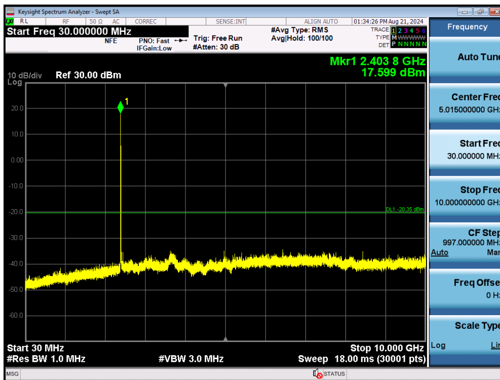
Plot 7-85. Conducted Spurious Plot SISO ANT2 (802.11ax OFDMA – 26 Tones – Ch. 1)
