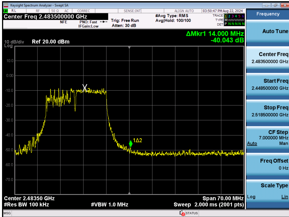
Plot 7-63. Band Edge Plot MIMO ANT1 (802.11be OFDMA – 106+26 Tones – Ch. 12)
