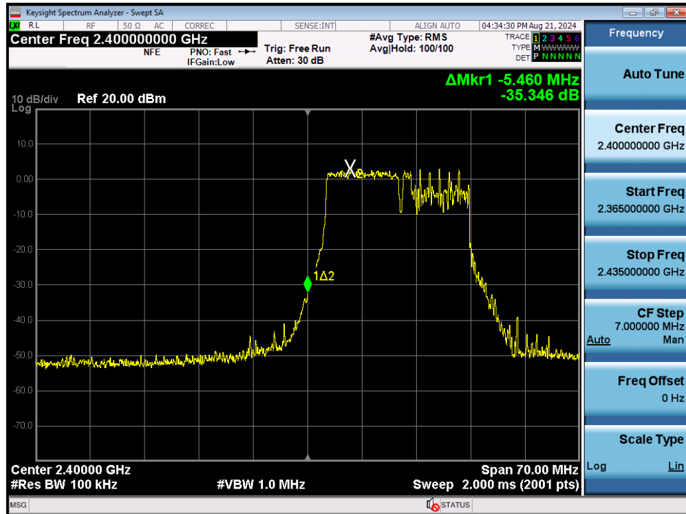
Plot 7-45. Band Edge Plot SISO ANT2 (802.11be OFDMA – 106+26 Tones – Ch. 1)
