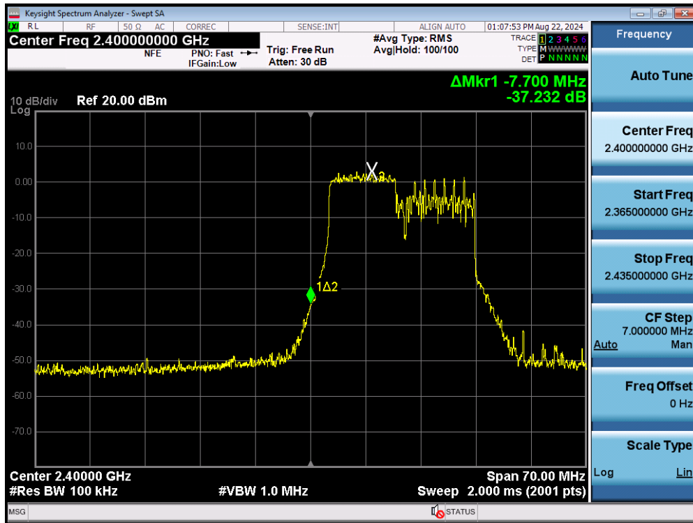
Plot 7-53. Band Edge Plot MIMO ANT1 (802.11ax OFDMA – 106 Tones – Ch. 1)
