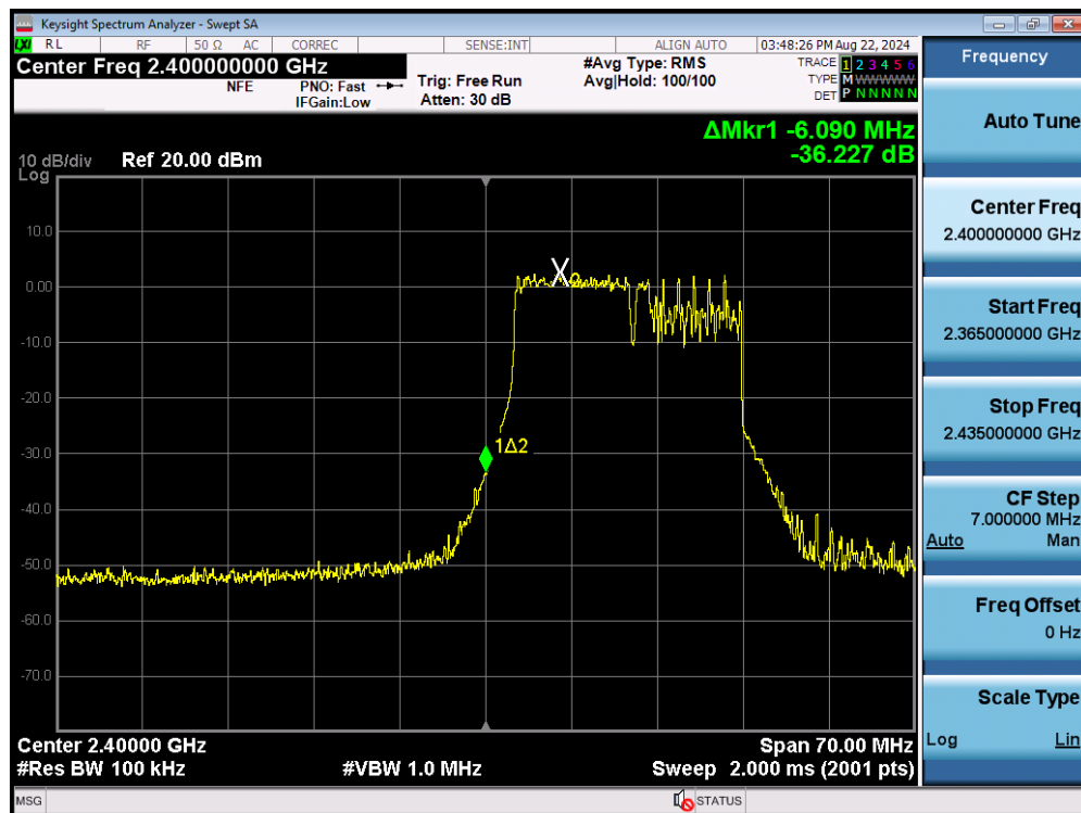
Plot 7-61. Band Edge Plot MIMO ANT1 (802.11be OFDMA – 106+26 Tones – Ch. 1)
