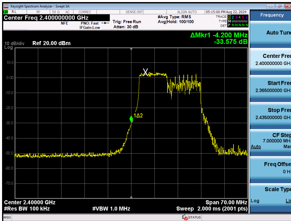
Plot 7-69. Band Edge Plot MIMO ANT2 (802.11ax OFDMA – 106 Tones – Ch. 1)
