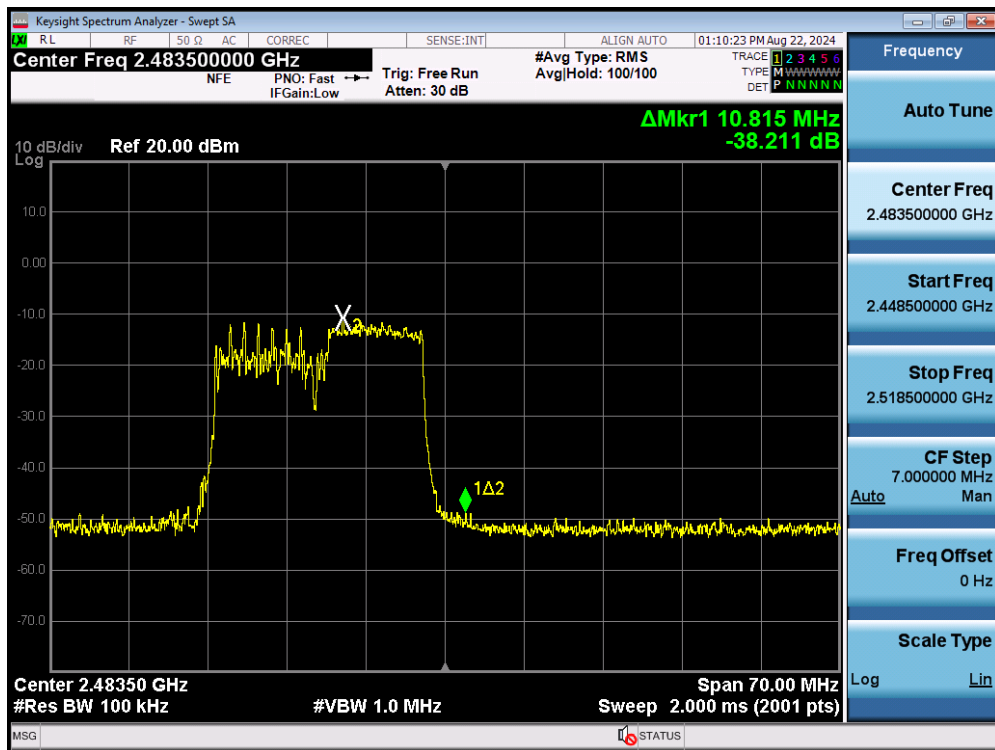
Plot 7-56. Band Edge Plot MIMO ANT1 (802.11ax OFDMA – 106 Tones – Ch. 13)
