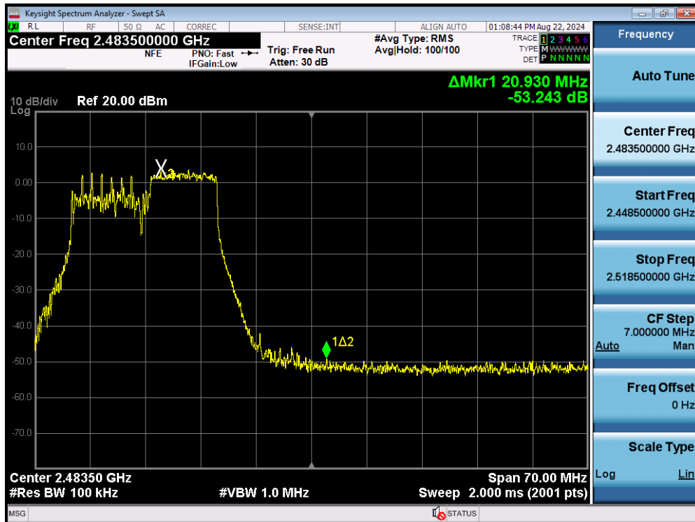
Plot 7-54. Band Edge Plot MIMO ANT1 (802.11ax OFDMA – 106 Tones – Ch. 11)
