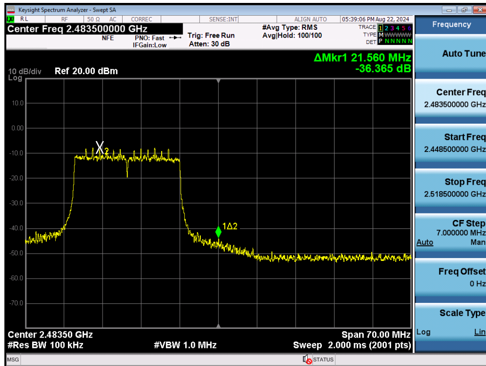
Plot 7-83. Band Edge Plot MIMO ANT2 (802.11ax OFDMA – 242 Tones – Ch. 12)
