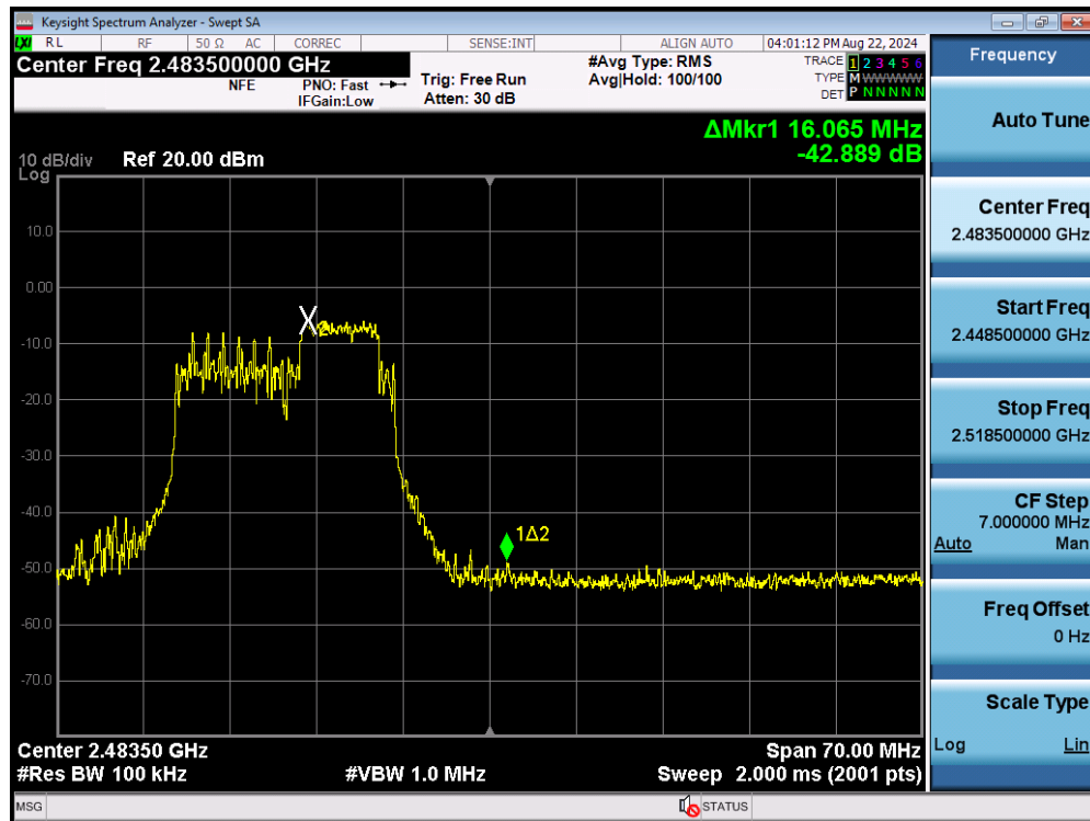
Plot 7-75. Band Edge Plot MIMO ANT2 (802.11be OFDMA – 52+26 Tones – Ch. 12)
