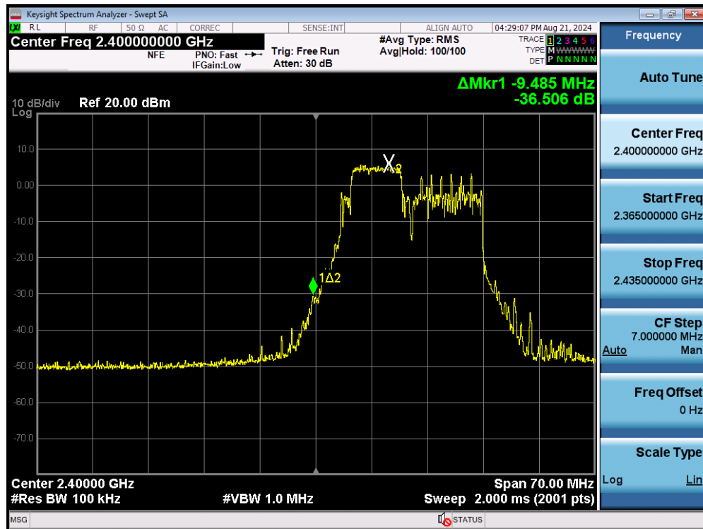
Plot 7-41. Band Edge Plot SISO ANT2 (802.11be OFDMA – 52+26 Tones – Ch. 1)
