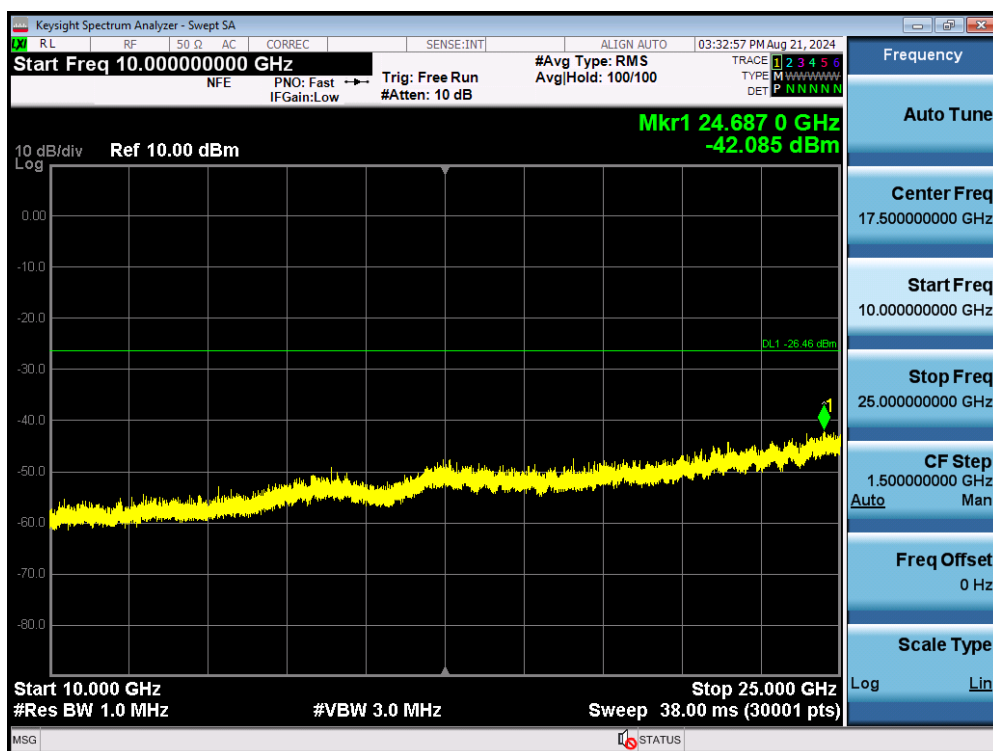
Plot 7-92. Conducted Spurious Plot SISO ANT2 (802.11ax OFDMA – 242 Tones – Ch. 1)
