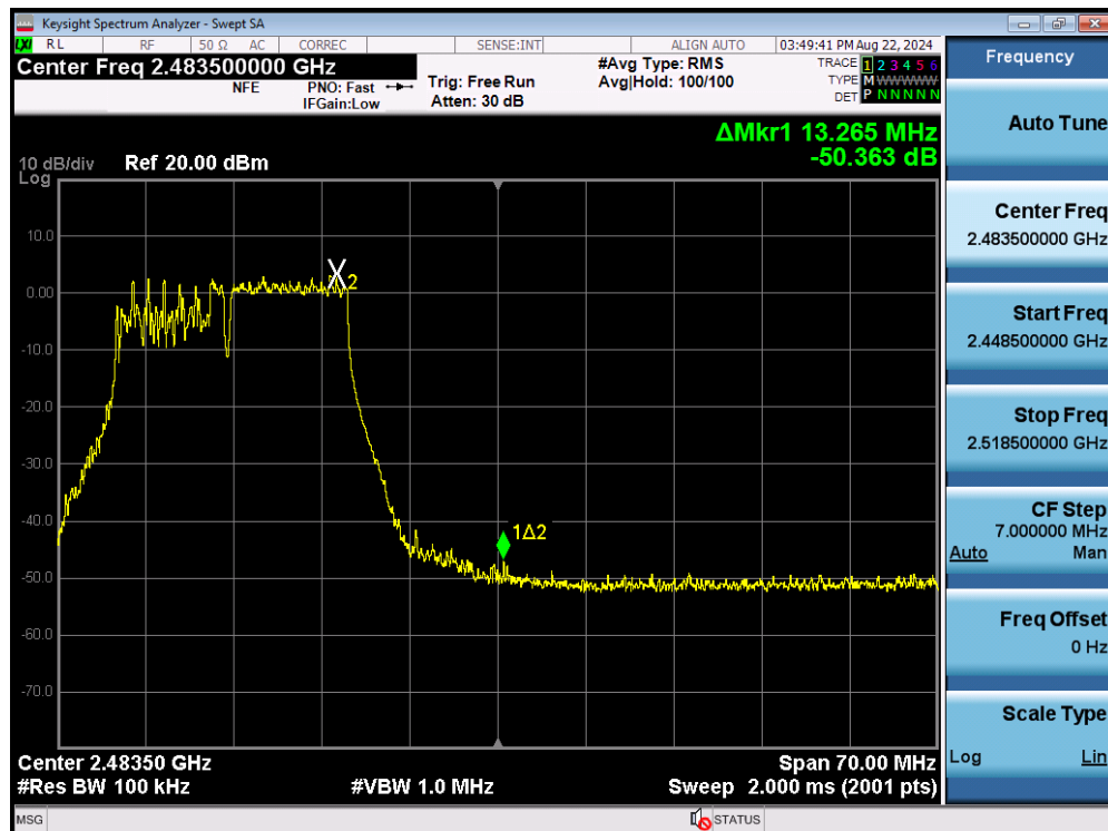
Plot 7-62. Band Edge Plot MIMO ANT1 (802.11be OFDMA – 106+26 Tones – Ch. 11)
