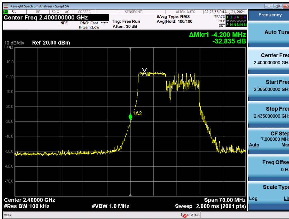
Plot 7-37. Band Edge Plot SISO ANT2 (802.11ax OFDMA – 106 Tones – Ch. 1)
