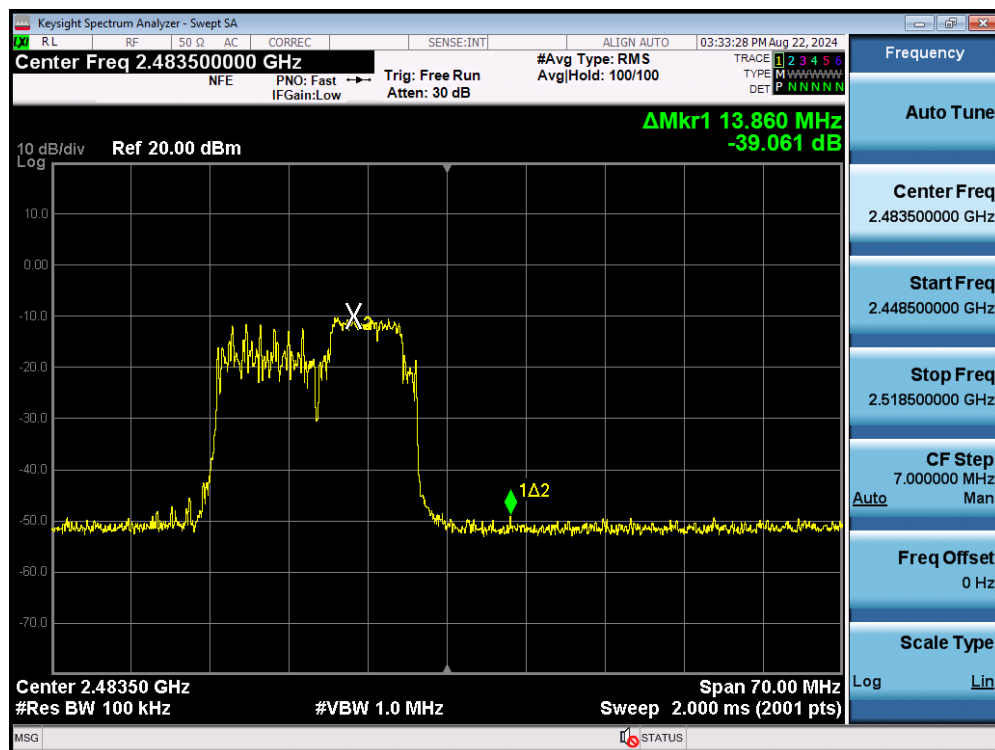
Plot 7-60. Band Edge Plot MIMO ANT1 (802.11be OFDMA – 52+26 Tones – Ch. 13)
