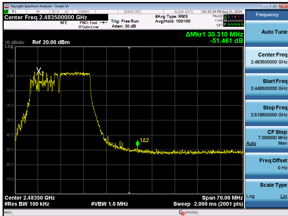
Plot 7-46. Band Edge Plot SISO ANT2 (802.11be OFDMA – 106+26 Tones – Ch. 11)
