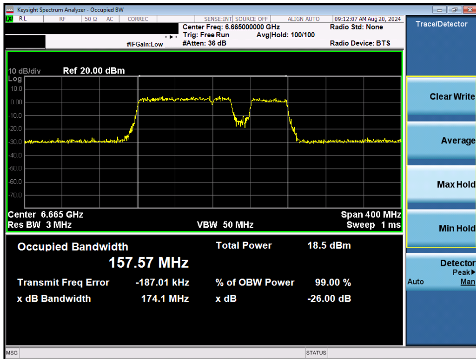
Plot 7-70. 26dB Bandwidth Plot MIMO ANT2 (160MHz 802.11be (UNII Band 7) – Ch. 143) – 20MHz Punctured
