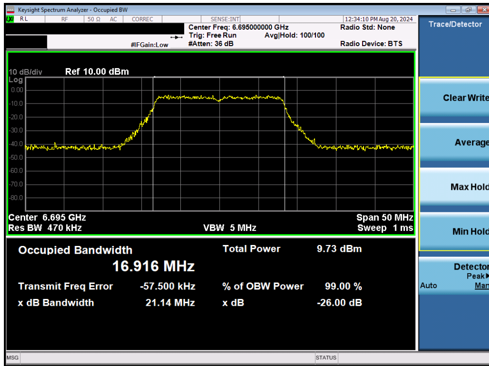
Plot 7-22. 26dB Bandwidth Plot MIMO ANT1 (20MHz 802.11a (UNII Band 7) – Ch. 149)
