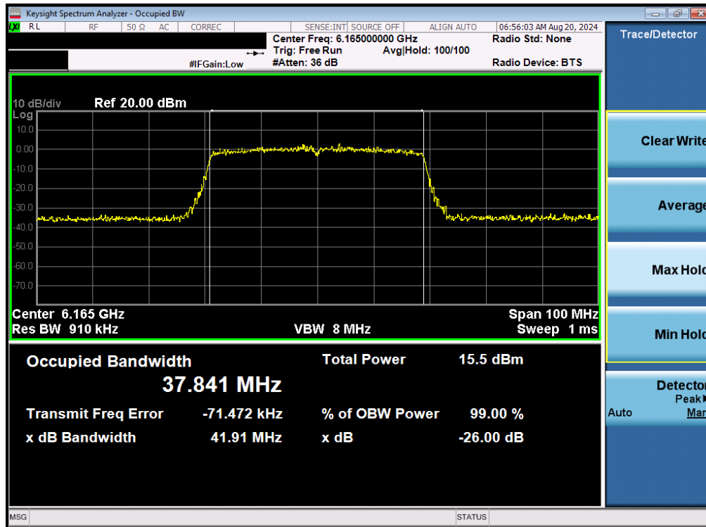
Plot 7-44. 26dB Bandwidth Plot MIMO ANT2 (40MHz 802.11be (UNII Band 5) – Ch. 43)
