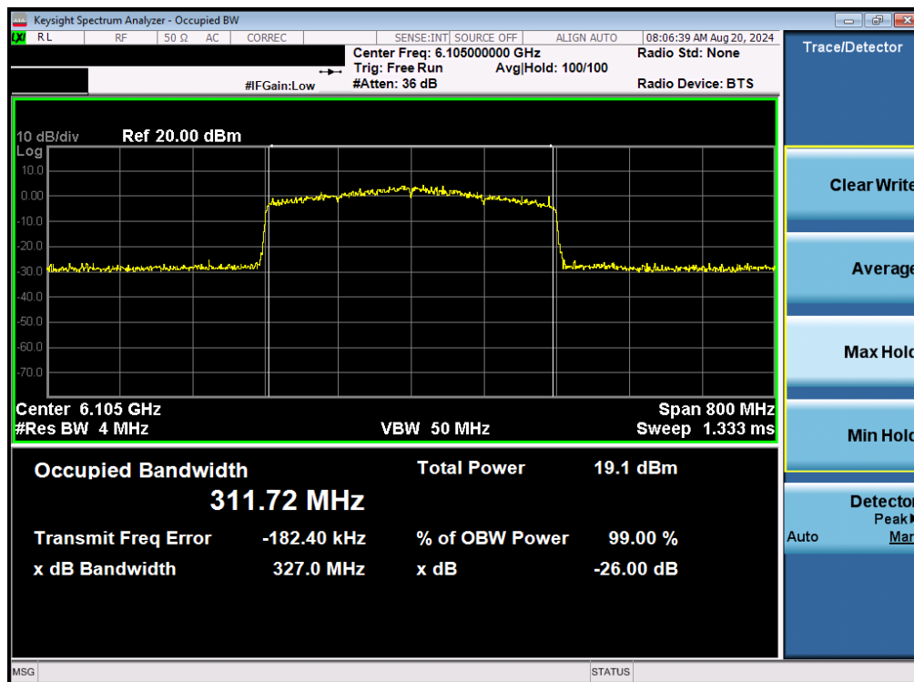
Plot 7-47. 26dB Bandwidth Plot MIMO ANT2 (320MHz 802.11be (UNII Band 5) – Ch. 31)
