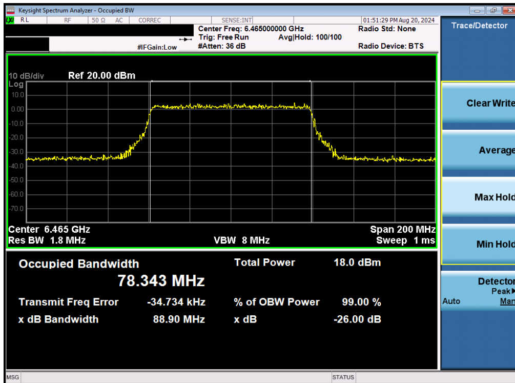
Plot 7-16. 26dB Bandwidth Plot MIMO ANT1 (80MHz 802.11be (UNII Band 6) – Ch. 103)
