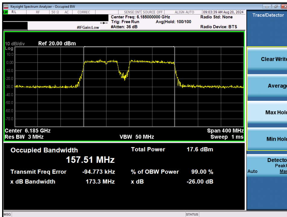
Plot 7-49. 26dB Bandwidth Plot MIMO ANT1 (160MHz 802.11be (UNII Band 5) – Ch. 47) – 20MHz Punctured
