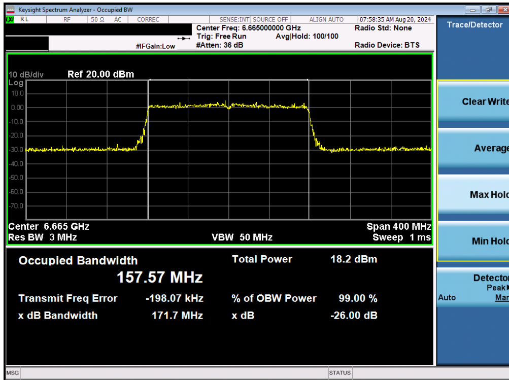
Plot 7-67. 26dB Bandwidth Plot MIMO ANT2 (160MHz 802.11be (UNII Band 7) – Ch. 143)
