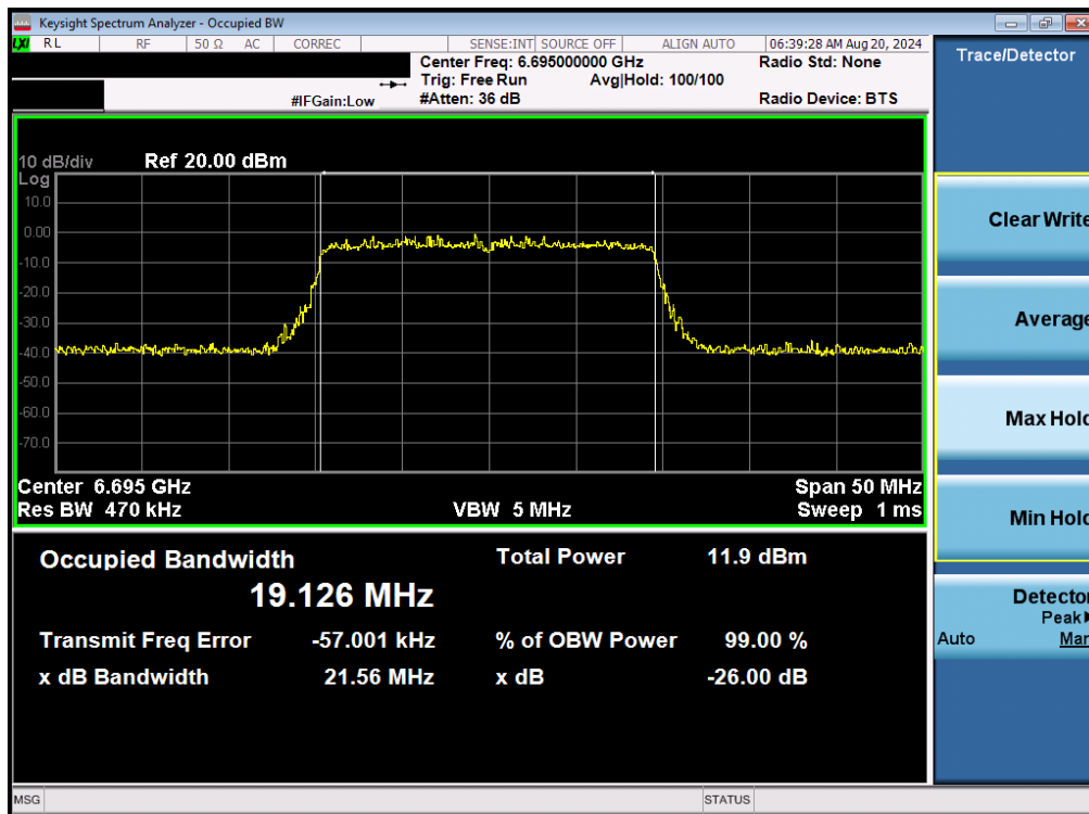
Plot 7-64. 26dB Bandwidth Plot MIMO ANT2 (20MHz 802.11be (UNII Band 7) – Ch. 149)
