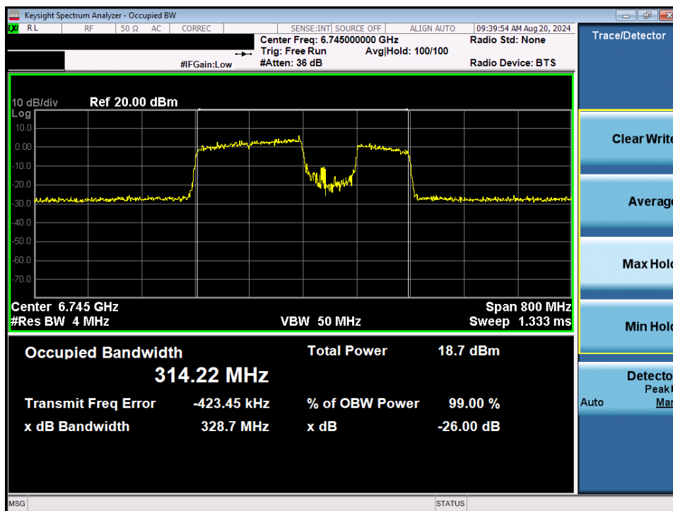
Plot 7-71. 26dB Bandwidth Plot MIMO ANT2 (320MHz 802.11be (UNII Band 7) – Ch. 159) – 80MHz Punctured
