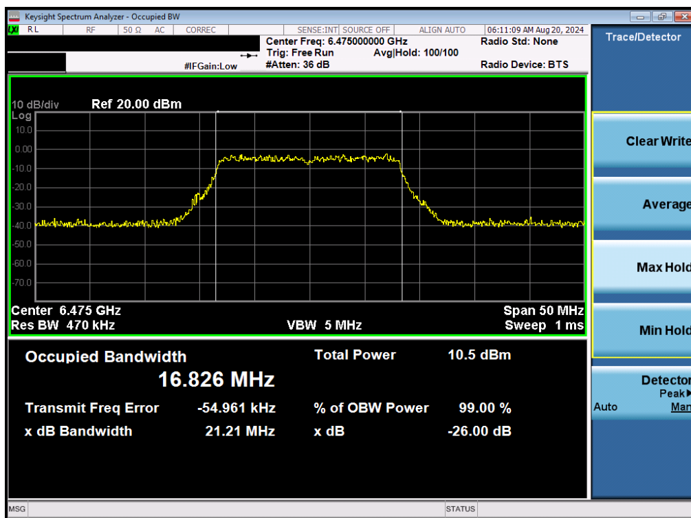
Plot 7-54. 26dB Bandwidth Plot MIMO ANT2 (20MHz 802.11a (UNII Band 6) – Ch. 105)
