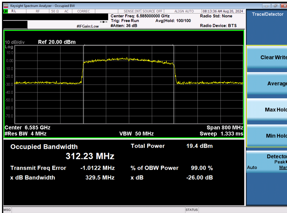
Plot 7-68. 26dB Bandwidth Plot MIMO ANT2 (320MHz 802.11be (UNII Band 7) – Ch. 127)
