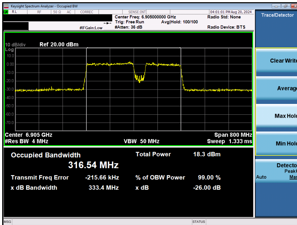
Plot 7-39. 26dB Bandwidth Plot MIMO ANT1 (320MHz 802.11be (UNII Band 8) – Ch. 191) – 40MHz Punctured
