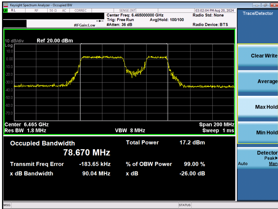
Plot 7-19. 26dB Bandwidth Plot MIMO ANT1 (80MHz 802.11be (UNII Band 6) – Ch. 103) – 20MHz Punctured
