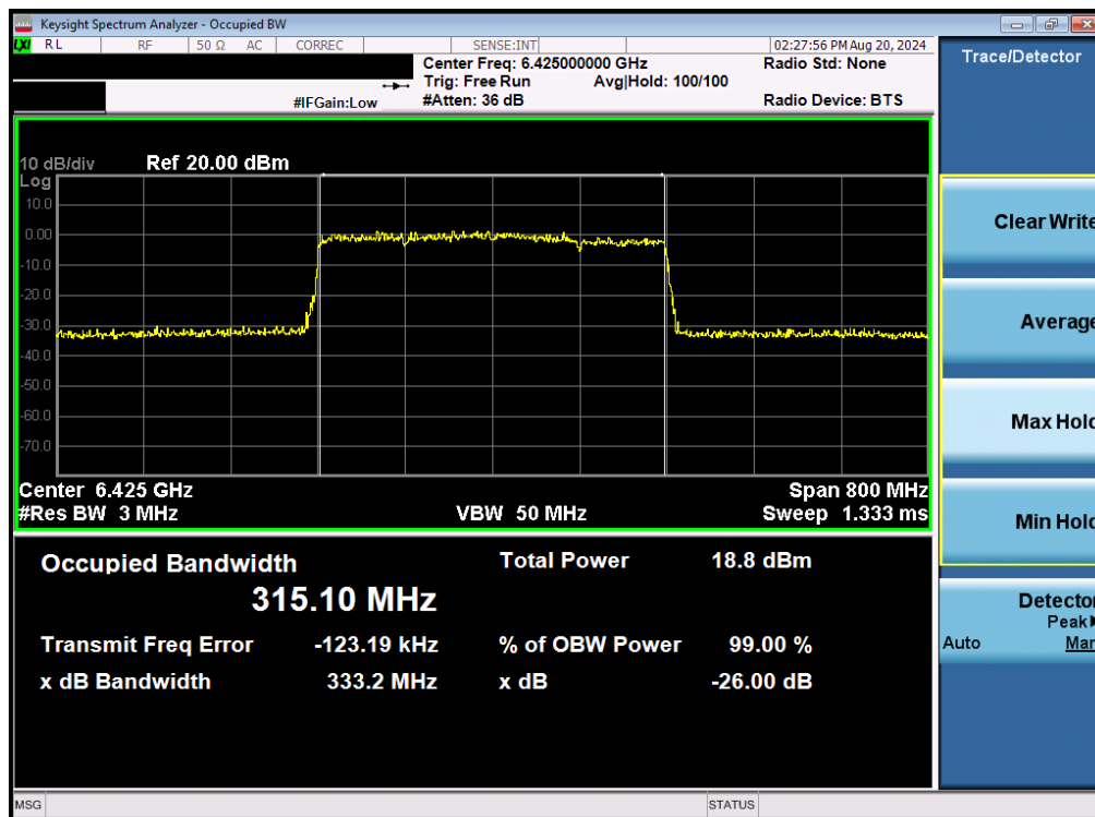
Plot 7-18. 26dB Bandwidth Plot MIMO ANT1 (320MHz 802.11be (UNII Band 5/6/7) – Ch. 95)
