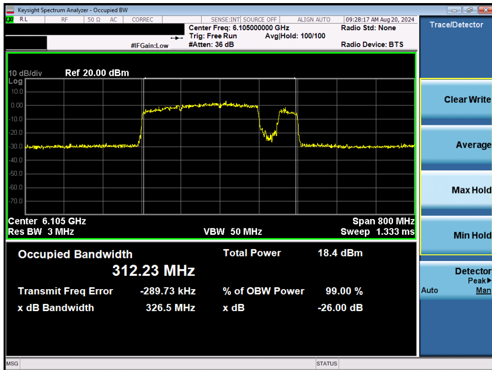
Plot 7-51. 26dB Bandwidth Plot MIMO ANT1 (320MHz 802.11be (UNII Band 5) – Ch. 31) – 40MHz Punctured
