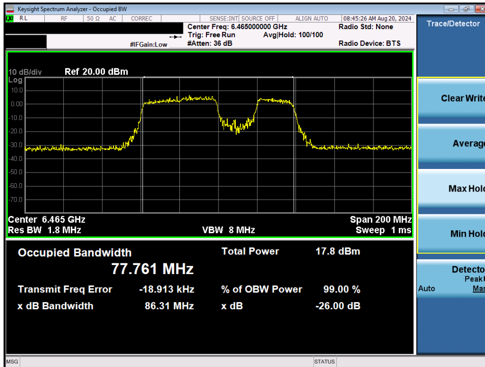
Plot 7-60. 26dB Bandwidth Plot MIMO ANT2 (80MHz 802.11be (UNII Band 6) – Ch. 103) – 20MHz Punctured
