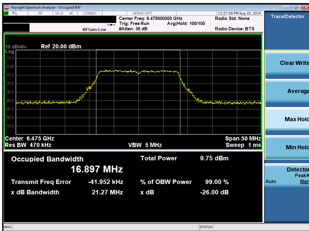
Plot 7-13. 26dB Bandwidth Plot MIMO ANT1 (20MHz 802.11a (UNII Band 6) – Ch. 105)
