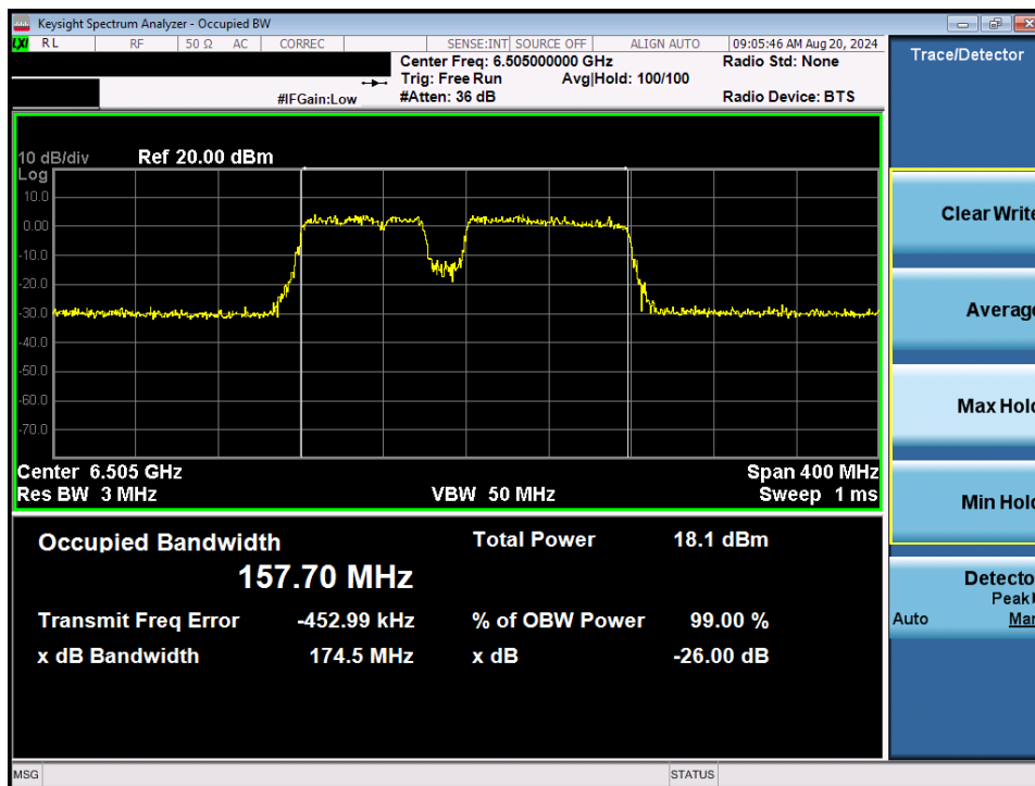
Plot 7-61. 26dB Bandwidth Plot MIMO ANT2 (160MHz 802.11be (UNII Band 6) – Ch. 111) – 20MHz Punctured
