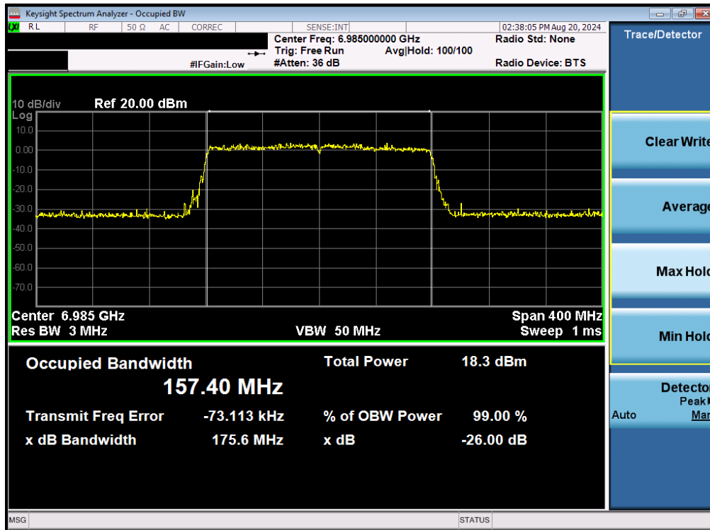
Plot 7-35. 26dB Bandwidth Plot MIMO ANT1 (160MHz 802.11be (UNII Band 8) – Ch. 207)
