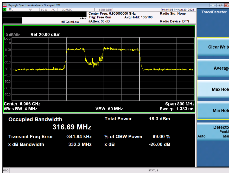
Plot 7-40. 26dB Bandwidth Plot MIMO ANT1 (320MHz 802.11be (UNII Band 8) – Ch. 191) – 80MHz Punctured
