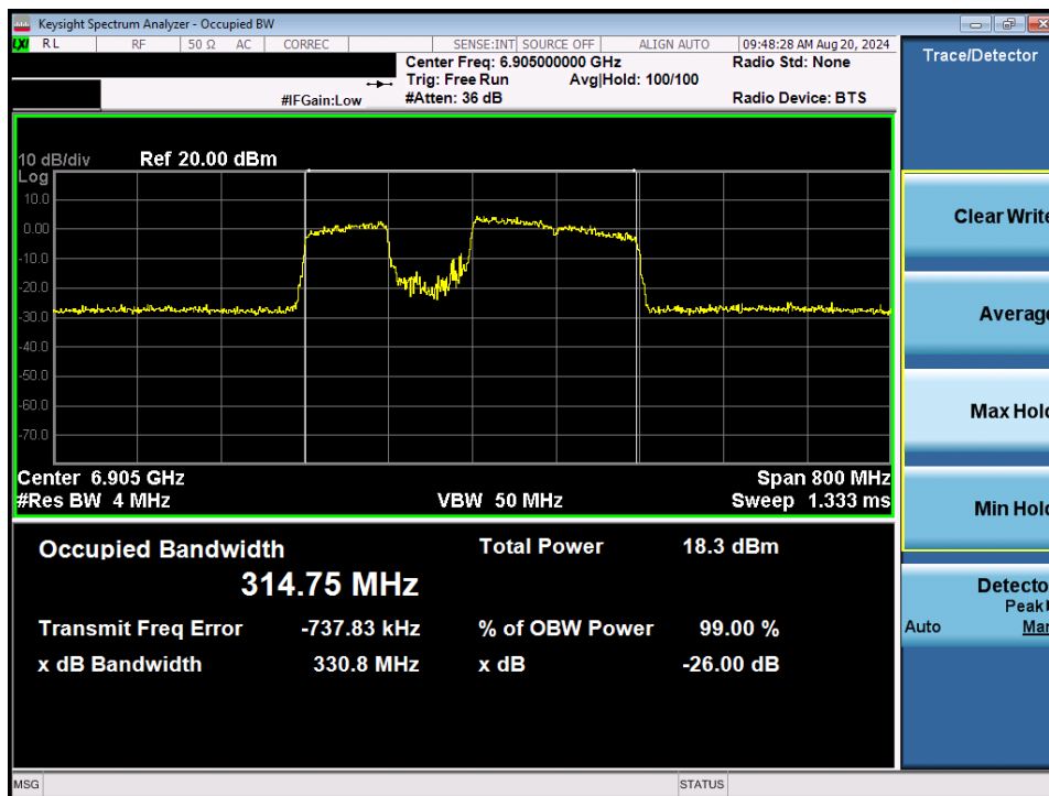
Plot 7-81. 26dB Bandwidth Plot MIMO ANT2 (320MHz 802.11be (UNII Band 8) – Ch. 191) – 80MHz Punctured
