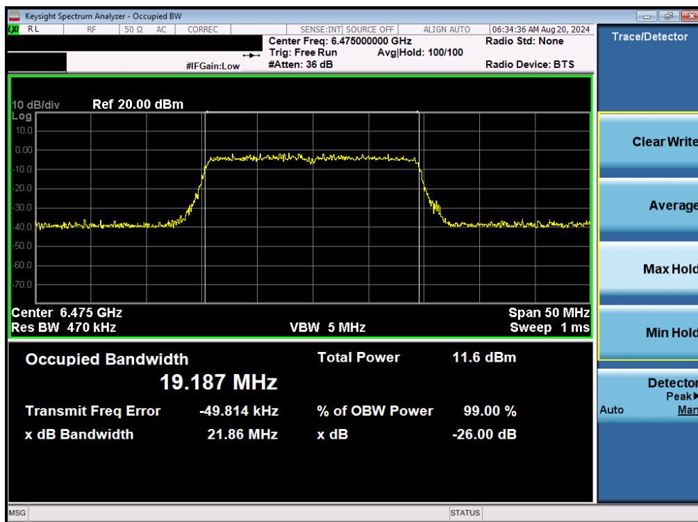
Plot 7-55. 26dB Bandwidth Plot MIMO ANT2 (20MHz 802.11be (UNII Band 6) – Ch. 105)
