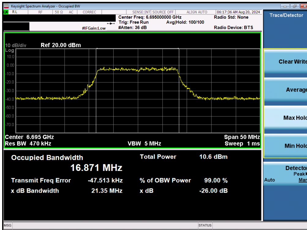
Plot 7-63. 26dB Bandwidth Plot MIMO ANT2 (20MHz 802.11a (UNII Band 7) – Ch. 149)
