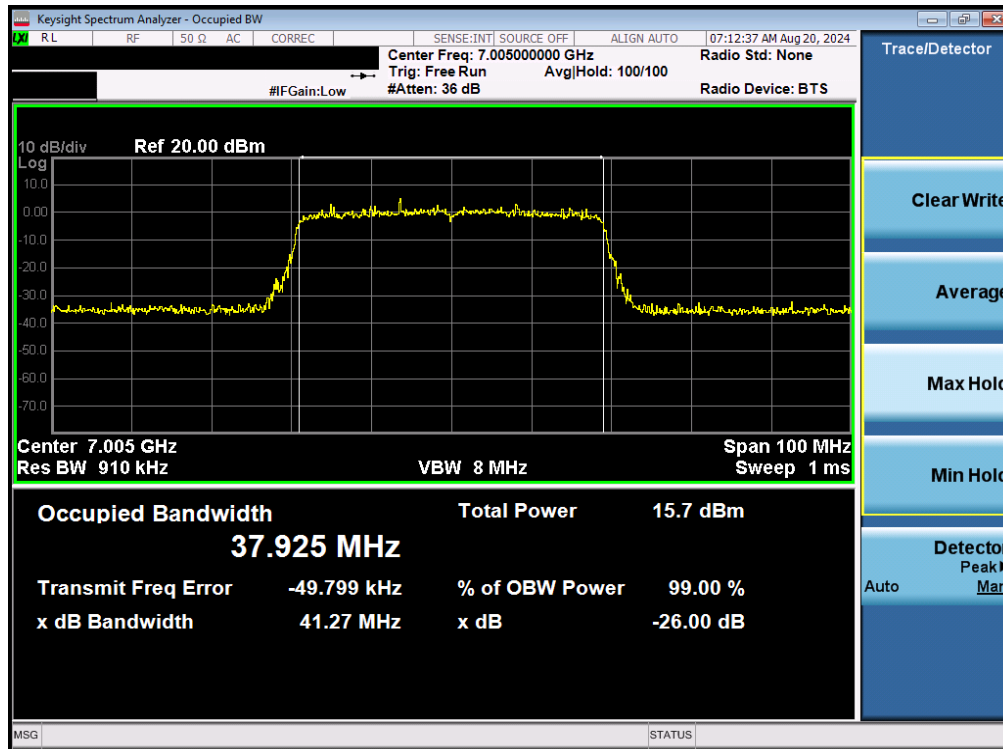
Plot 7-74. 26dB Bandwidth Plot MIMO ANT2 (40MHz 802.11be (UNII Band 8) – Ch. 211)
