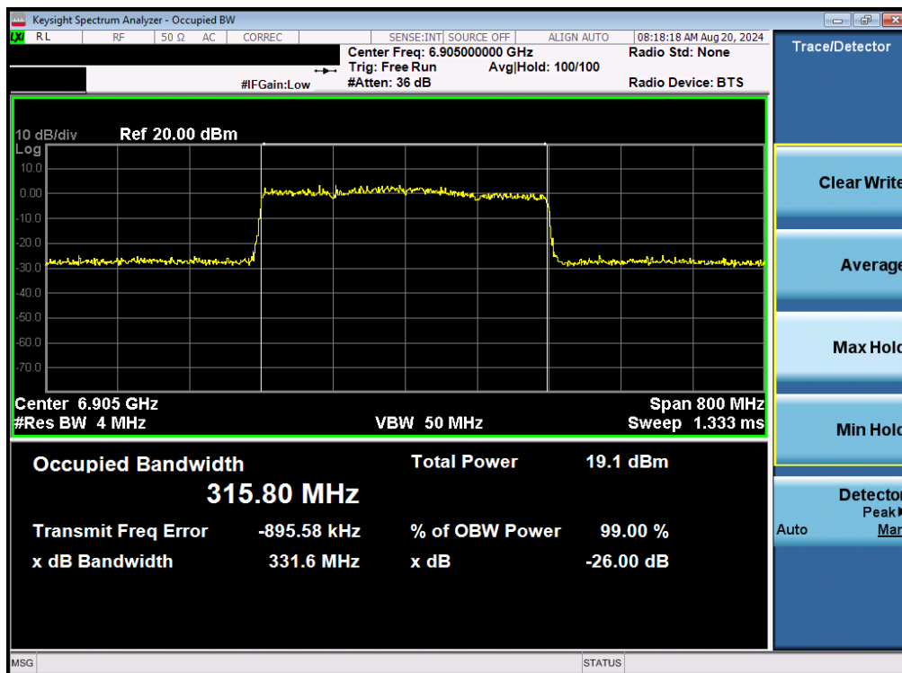
Plot 7-77. 26dB Bandwidth Plot MIMO ANT2 (320MHz 802.11be (UNII Band 7/8) – Ch. 191)
