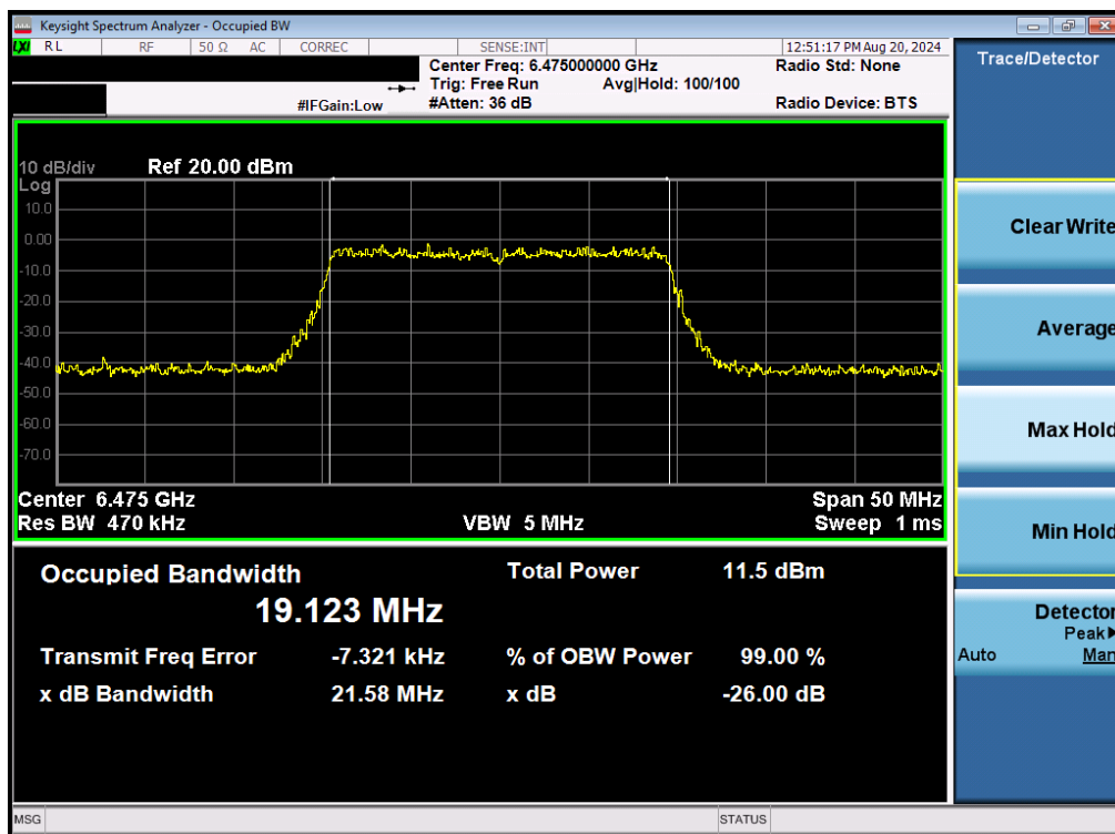
Plot 7-14. 26dB Bandwidth Plot MIMO ANT1 (20MHz 802.11be (UNII Band 6) – Ch. 105)
