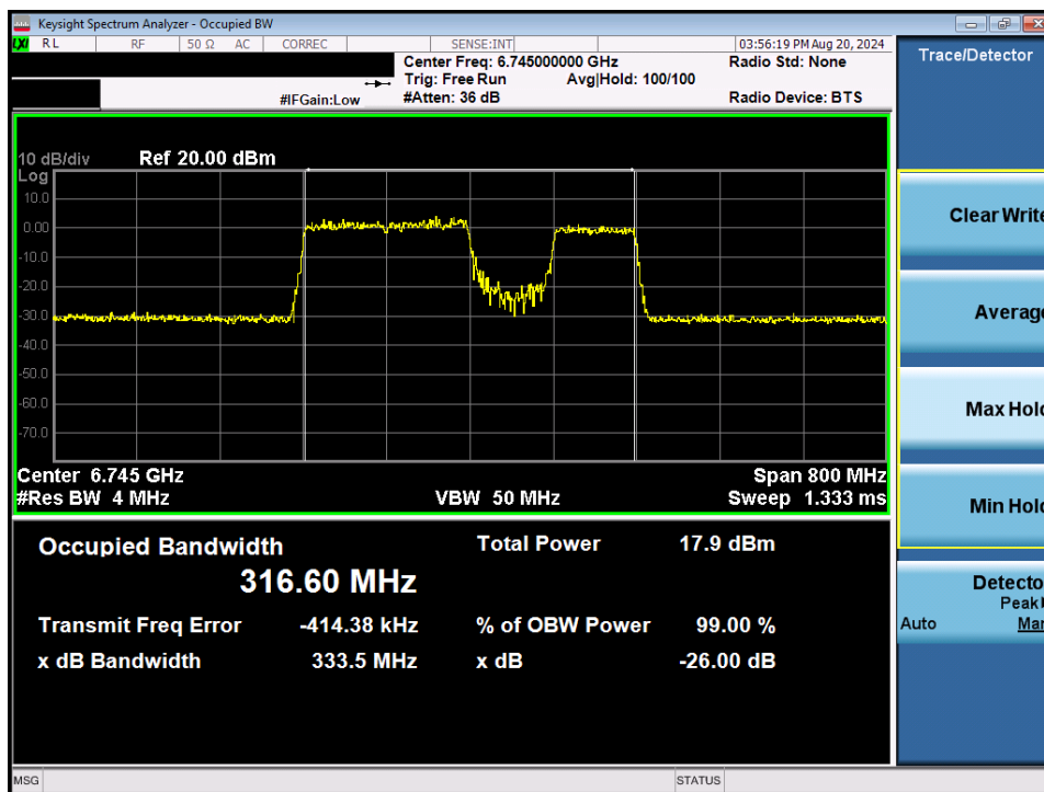
Plot 7-30. 26dB Bandwidth Plot MIMO ANT1 (320MHz 802.11be (UNII Band 7) – Ch. 159) – 80MHz Punctured
