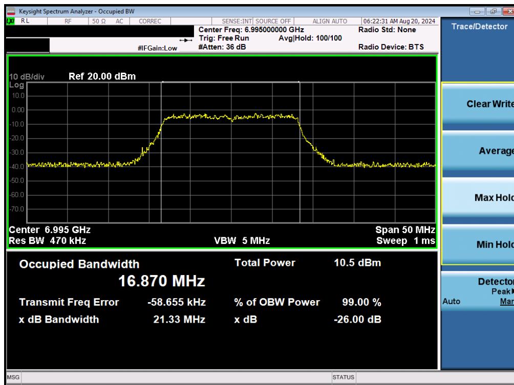
Plot 7-72. 26dB Bandwidth Plot MIMO ANT2 (20MHz 802.11a (UNII Band 8) – Ch. 209)
