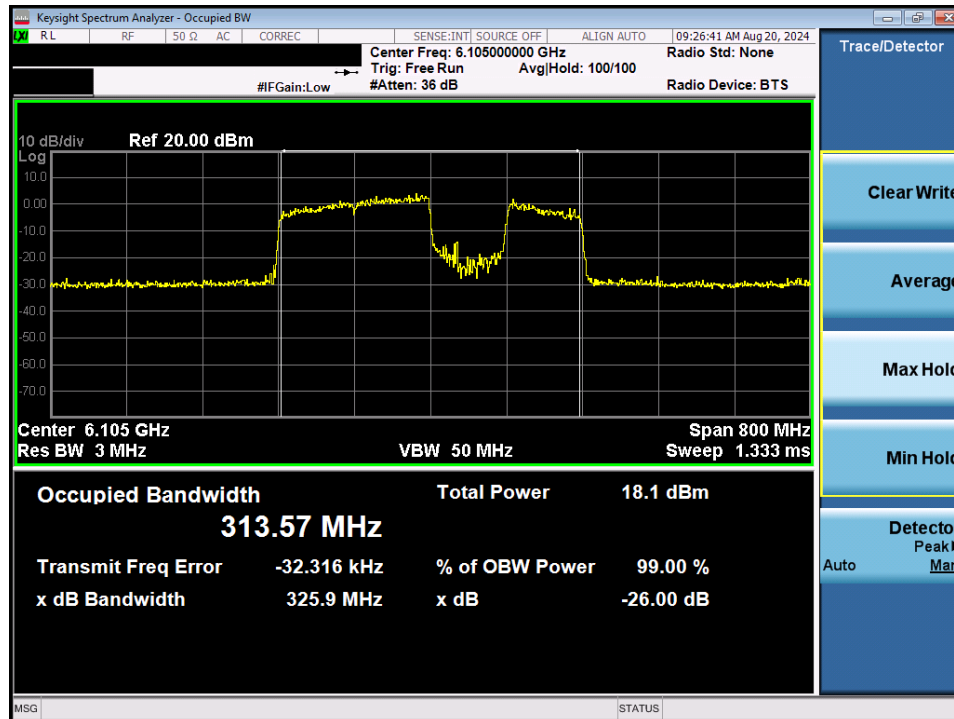
Plot 7-52. 26dB Bandwidth Plot MIMO ANT1 (320MHz 802.11be (UNII Band 5) – Ch. 31) – 80MHz Punctured
