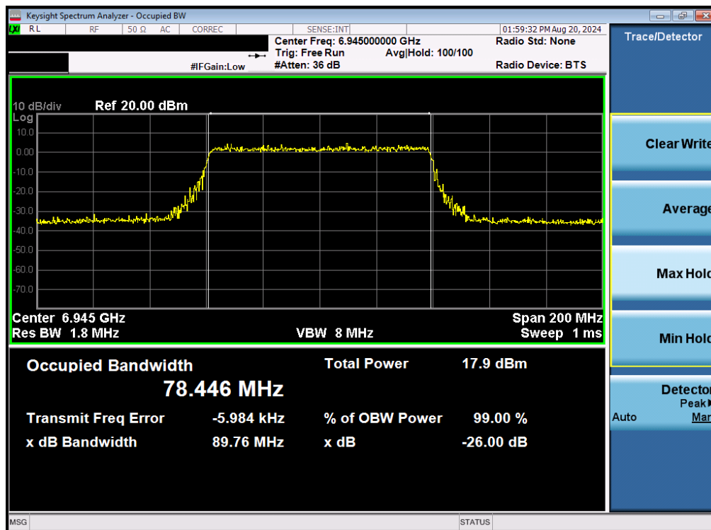
Plot 7-34. 26dB Bandwidth Plot MIMO ANT1 (80MHz 802.11be (UNII Band 8) – Ch. 199)
