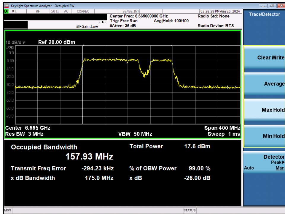
Plot 7-29. 26dB Bandwidth Plot MIMO ANT1 (160MHz 802.11be (UNII Band 7) – Ch. 143) – 20MHz Punctured
