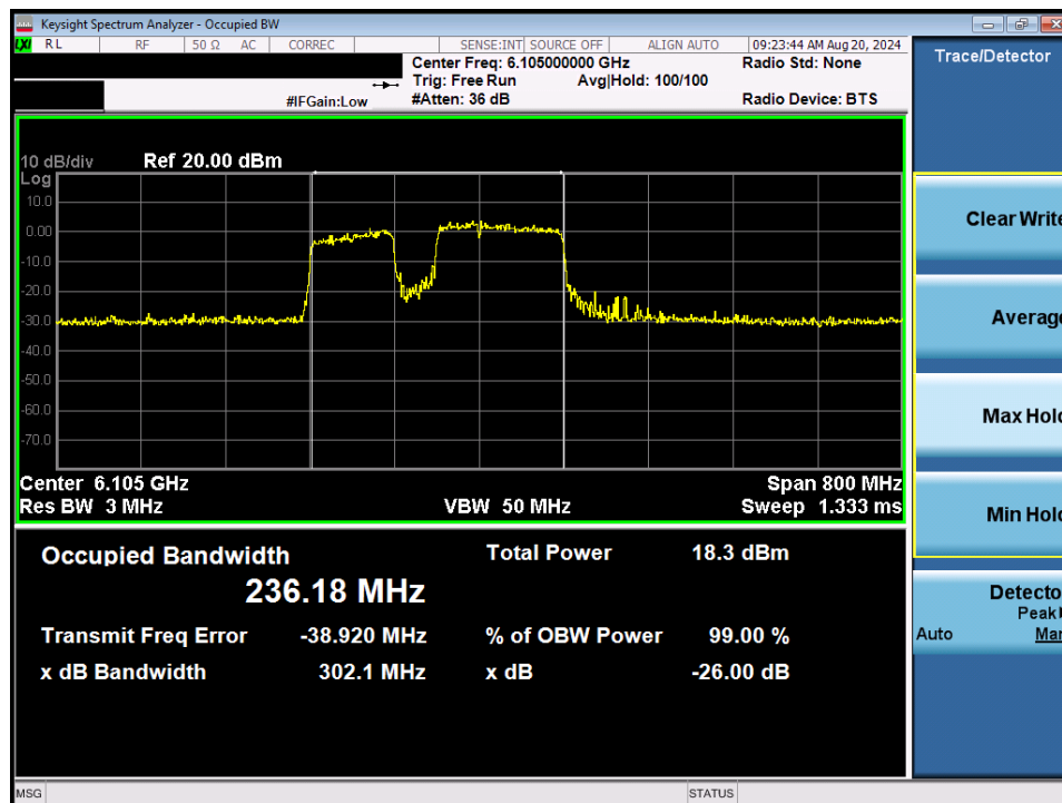
Plot 7-53. 26dB Bandwidth Plot MIMO ANT1 (320MHz 802.11be (UNII Band 5) – Ch. 31) – 120MHz Punctured
