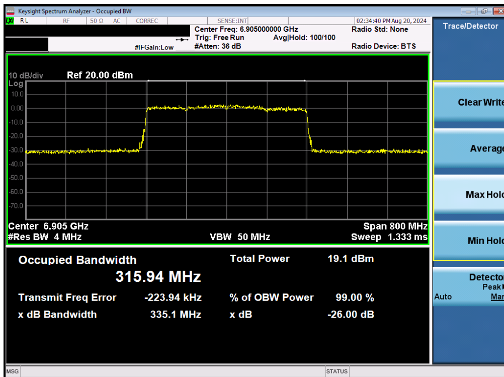
Plot 7-36. 26dB Bandwidth Plot MIMO ANT1 (320MHz 802.11be (UNII Band 7/8) – Ch. 191)
