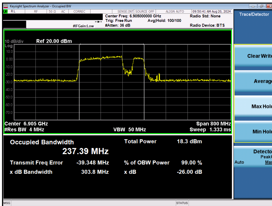
Plot 7-82. 26dB Bandwidth Plot MIMO ANT2 (320MHz 802.11be (UNII Band 8) – Ch. 191) – 120MHz Punctured
