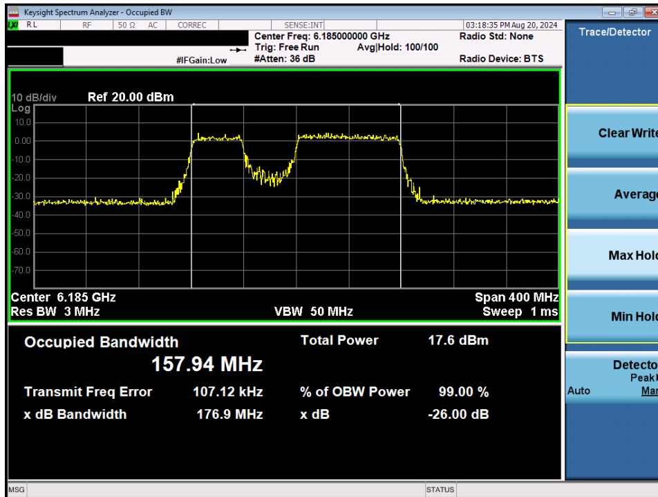
Plot 7-9. 26dB Bandwidth Plot MIMO ANT1 (160MHz 802.11be (UNII Band 5) – Ch. 47) – 40MHz Punctured
