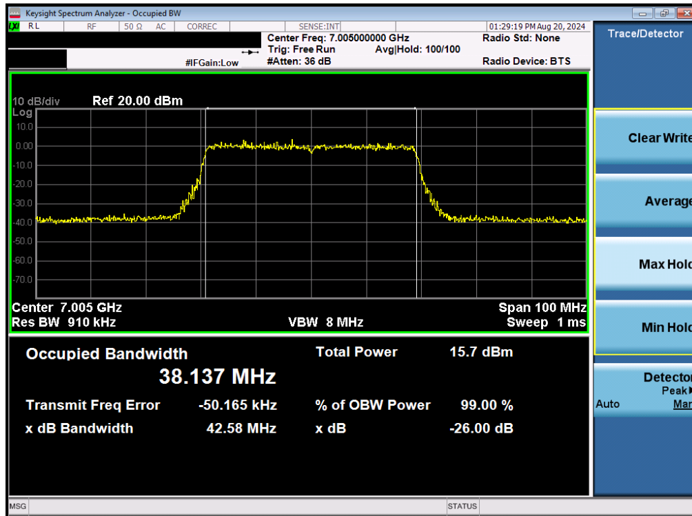
Plot 7-33. 26dB Bandwidth Plot MIMO ANT1 (40MHz 802.11be (UNII Band 8) – Ch. 211)
