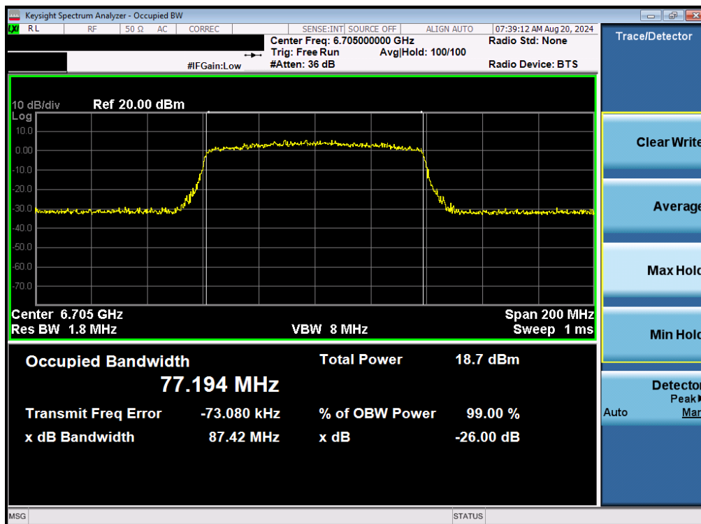
Plot 7-66. 26dB Bandwidth Plot MIMO ANT2 (80MHz 802.11be (UNII Band 7) – Ch. 151)
