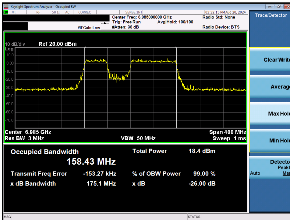
Plot 7-38. 26dB Bandwidth Plot MIMO ANT1 (160MHz 802.11be (UNII Band 8) – Ch. 207) – 40MHz Punctured
