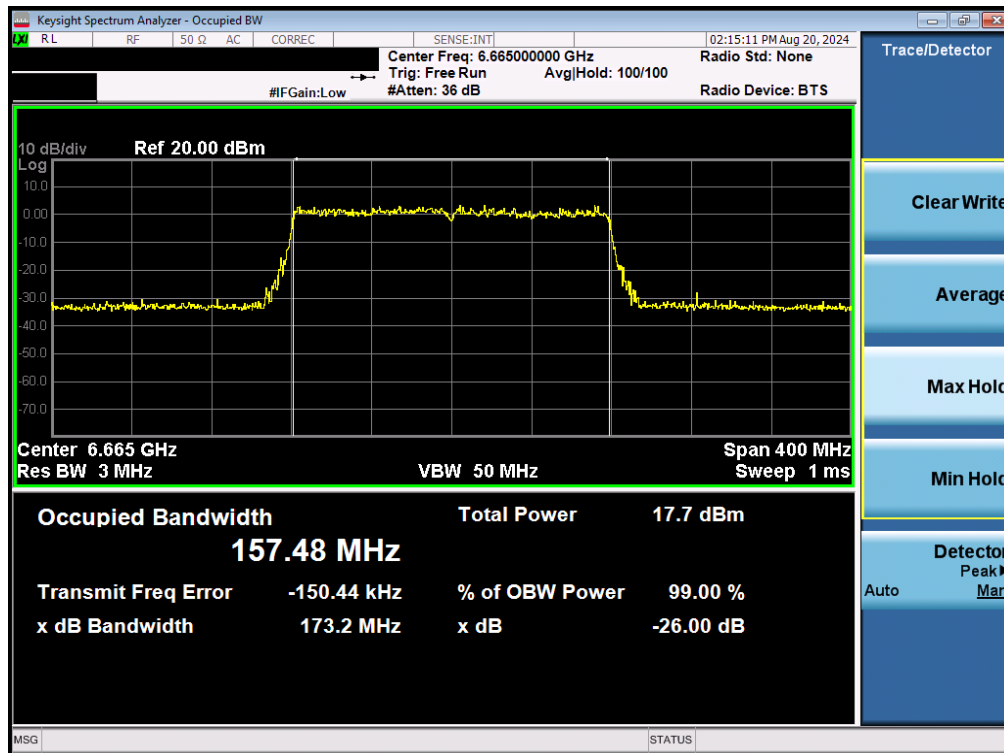
Plot 7-26. 26dB Bandwidth Plot MIMO ANT1 (160MHz 802.11be (UNII Band 7) – Ch. 143)
