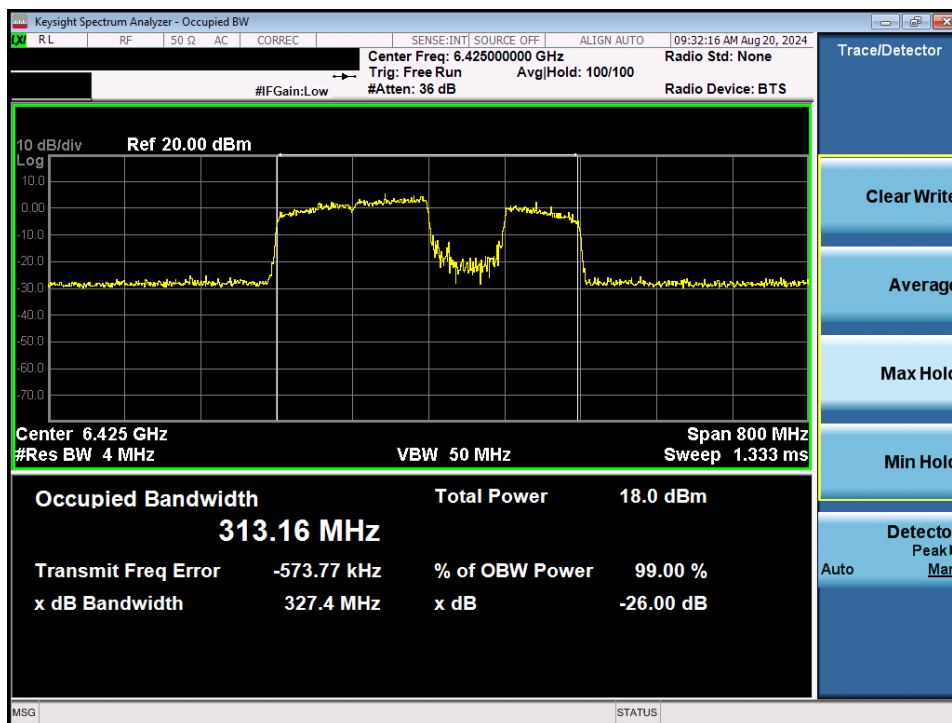
Plot 7-62. 26dB Bandwidth Plot MIMO ANT2 (320MHz 802.11be (UNII Band 6) – Ch. 95) – 80MHz Punctured
