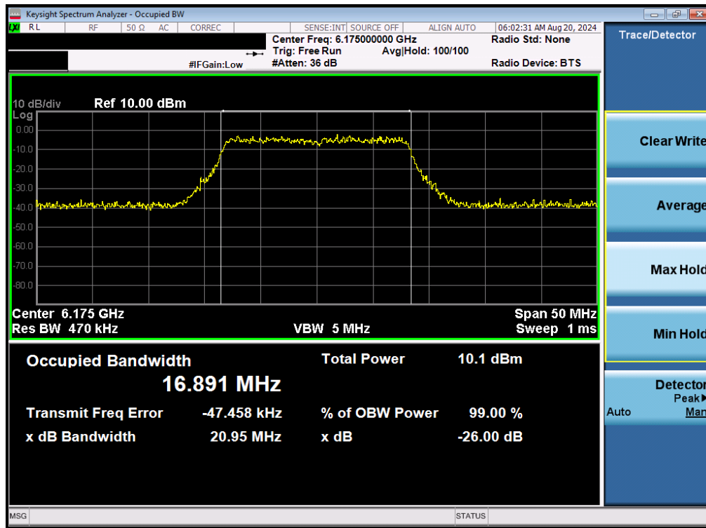
Plot 7-42. 26dB Bandwidth Plot MIMO ANT2 (20MHz 802.11a (UNII Band 5) – Ch. 45)
