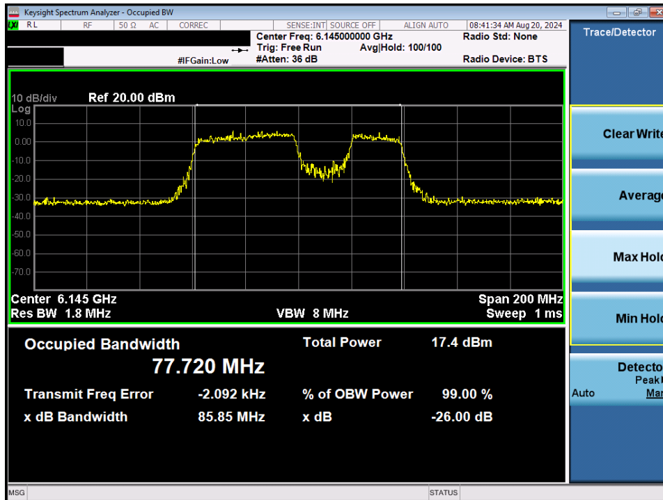
Plot 7-48. 26dB Bandwidth Plot MIMO ANT1 (80MHz 802.11be (UNII Band 5) – Ch. 39) – 20MHz Punctured
