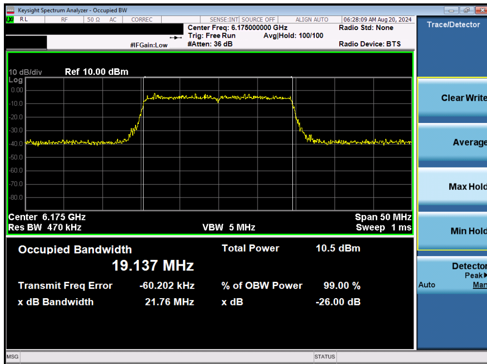
Plot 7-43. 26dB Bandwidth Plot MIMO ANT2 (20MHz 802.11be (UNII Band 5) – Ch. 45)
