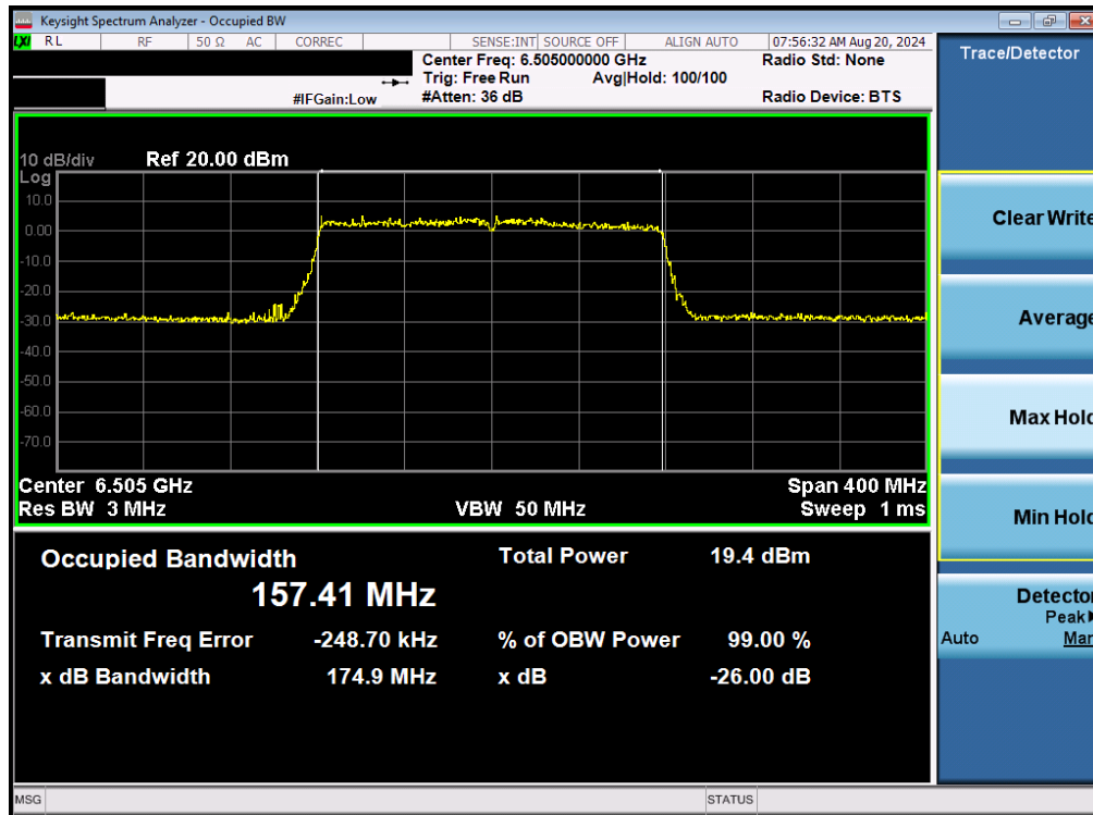
Plot 7-58. 26dB Bandwidth Plot MIMO ANT2 (160MHz 802.11be (UNII Band 6) – Ch. 111)
