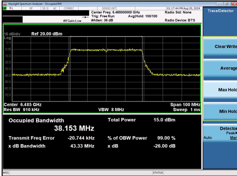
Plot 7-15. 26dB Bandwidth Plot MIMO ANT1 (40MHz 802.11be (UNII Band 6) – Ch. 107)
