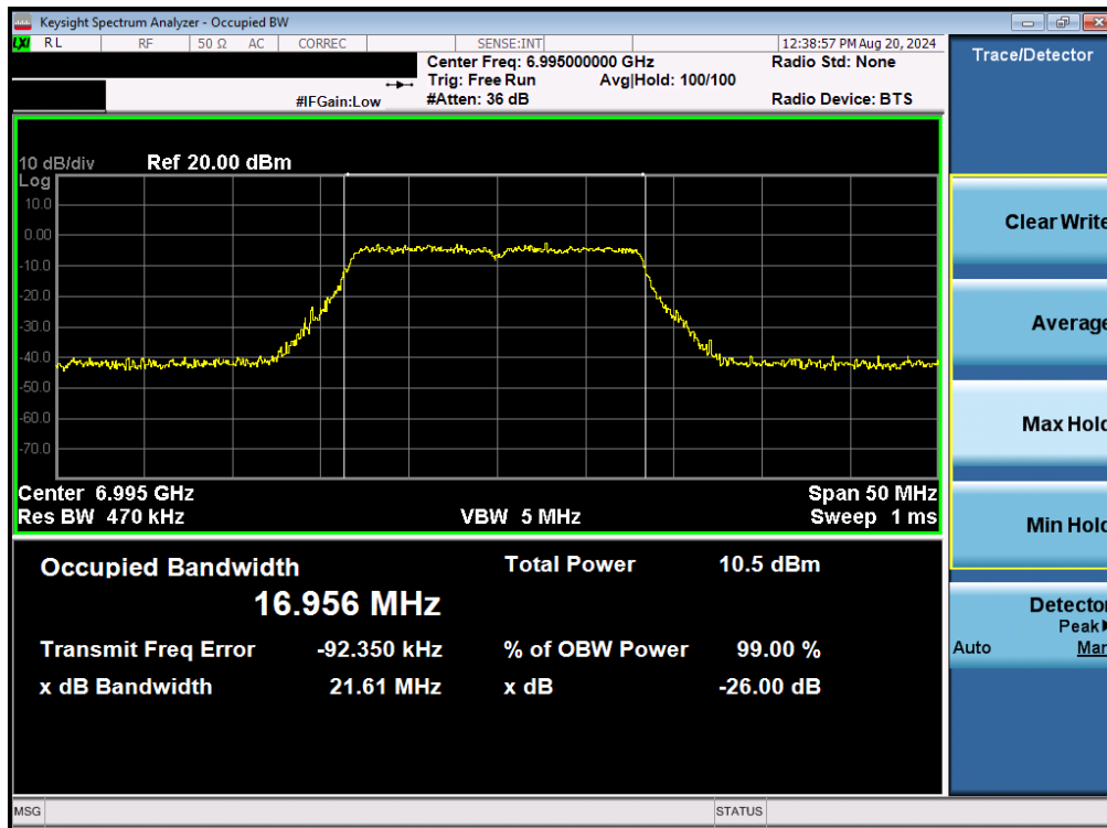
Plot 7-31. 26dB Bandwidth Plot MIMO ANT1 (20MHz 802.11a (UNII Band 8) – Ch. 209)
