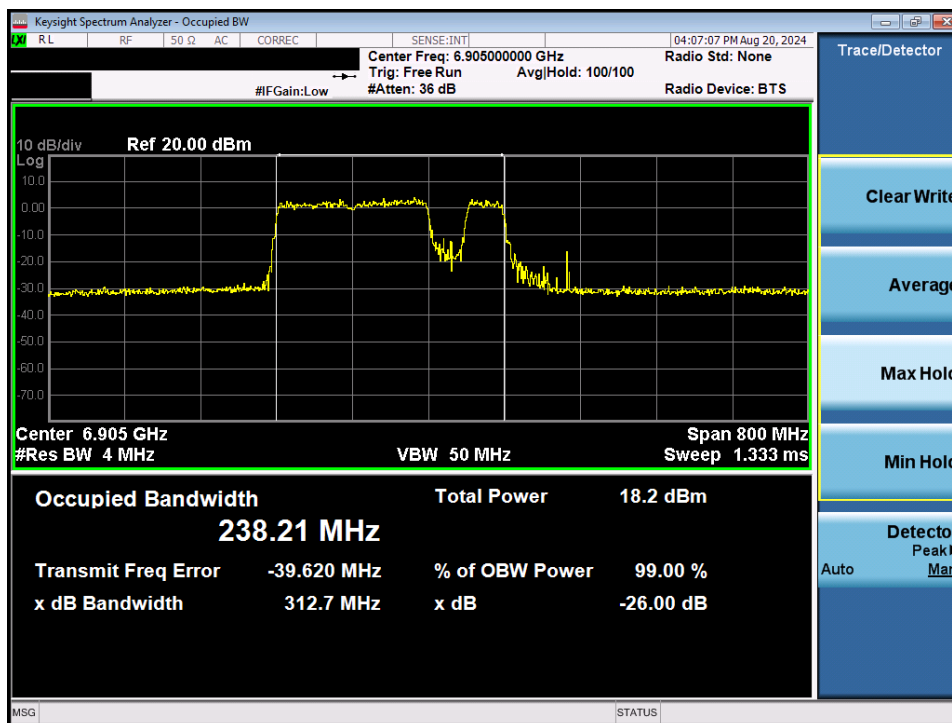
Plot 7-41. 26dB Bandwidth Plot MIMO ANT1 (320MHz 802.11be (UNII Band 8) – Ch. 191) – 120MHz Punctured
