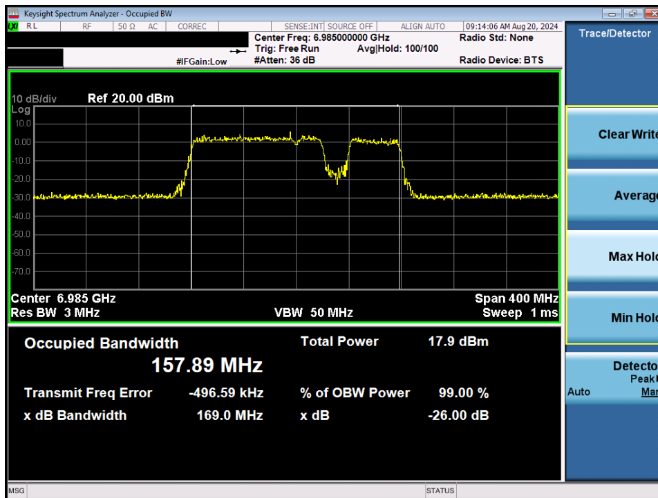
Plot 7-78. 26dB Bandwidth Plot MIMO ANT2 (160MHz 802.11be (UNII Band 8) – Ch. 207) – 20MHz Punctured
