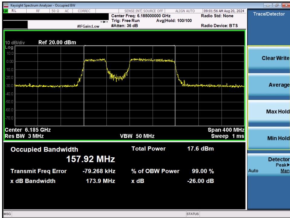
Plot 7-50. 26dB Bandwidth Plot MIMO ANT1 (160MHz 802.11be (UNII Band 5) – Ch. 47) – 40MHz Punctured
