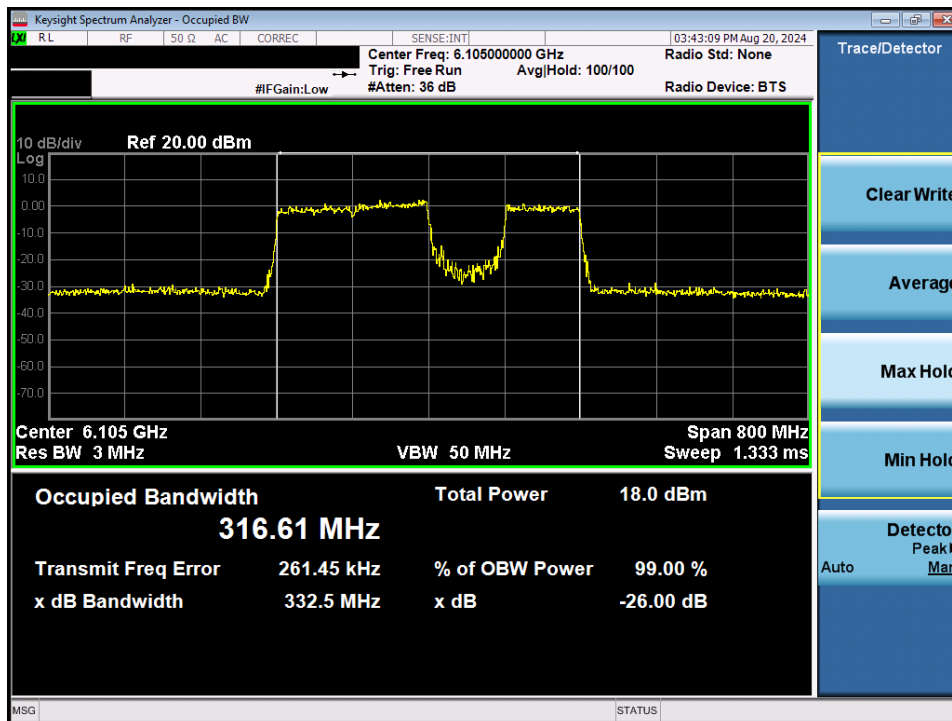
Plot 7-11. 26dB Bandwidth Plot MIMO ANT1 (320MHz 802.11be (UNII Band 5) – Ch. 31) – 80MHz Punctured
