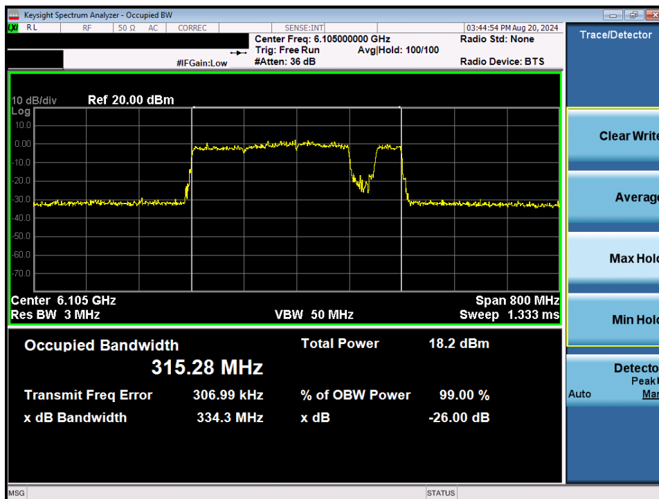
Plot 7-10. 26dB Bandwidth Plot MIMO ANT1 (320MHz 802.11be (UNII Band 5) – Ch. 31) – 40MHz Punctured
