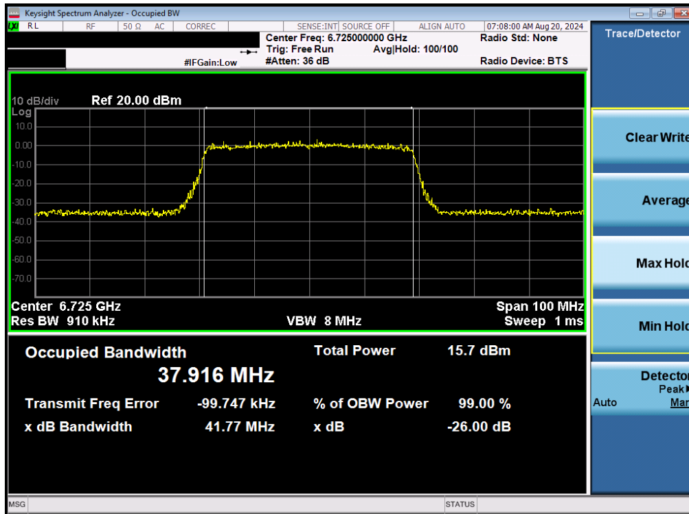
Plot 7-65. 26dB Bandwidth Plot MIMO ANT2 (40MHz 802.11be (UNII Band 7) – Ch. 155)
