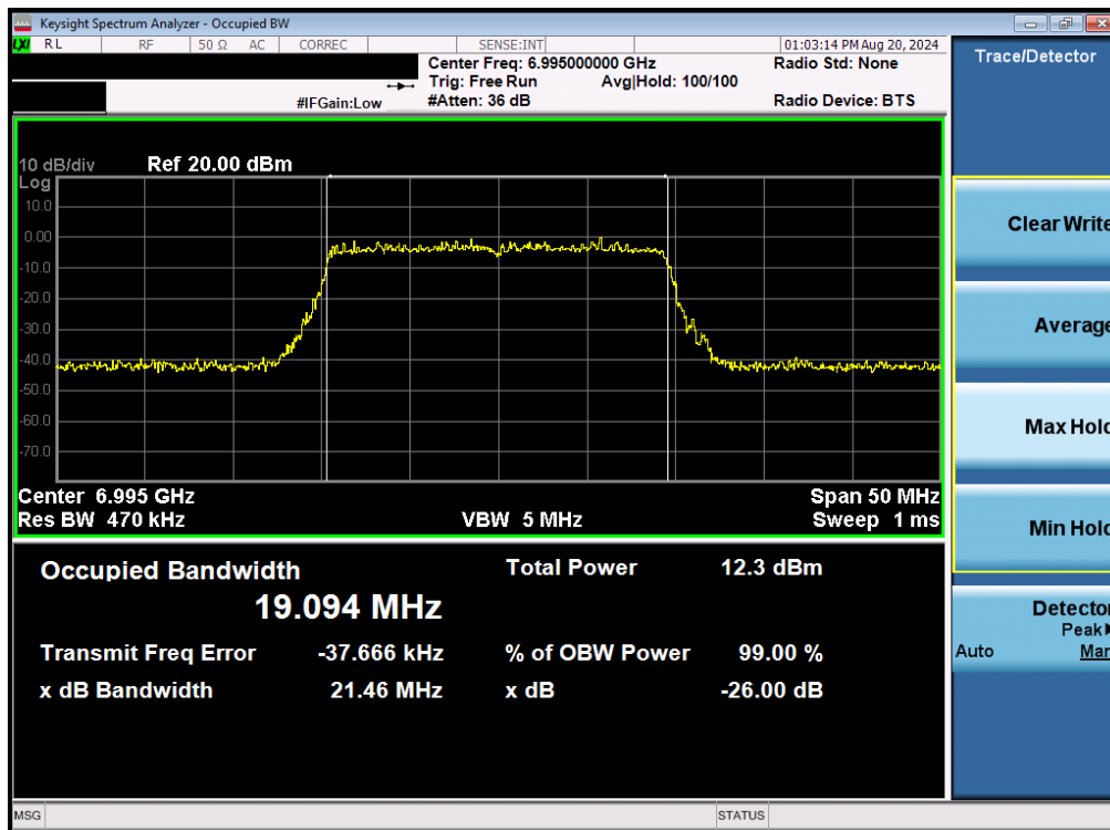
Plot 7-32. 26dB Bandwidth Plot MIMO ANT1 (20MHz 802.11be (UNII Band 8) – Ch. 209)
