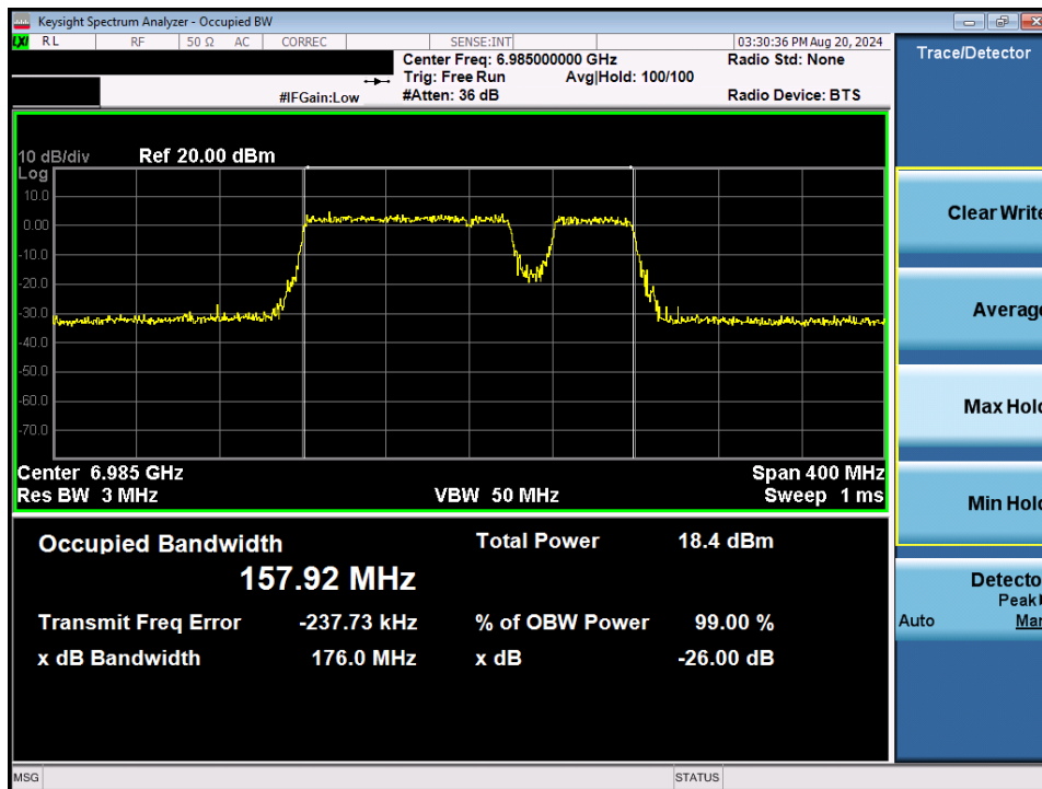
Plot 7-37. 26dB Bandwidth Plot MIMO ANT1 (160MHz 802.11be (UNII Band 8) – Ch. 207) – 20MHz Punctured
