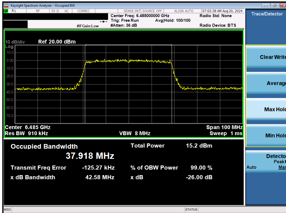
Plot 7-56. 26dB Bandwidth Plot MIMO ANT2 (40MHz 802.11be (UNII Band 6) – Ch. 107)
