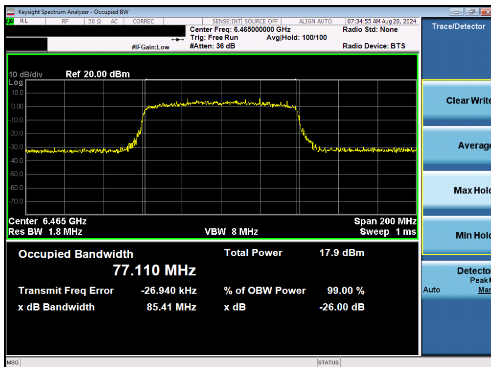
Plot 7-57. 26dB Bandwidth Plot MIMO ANT2 (80MHz 802.11be (UNII Band 6) – Ch. 103)
