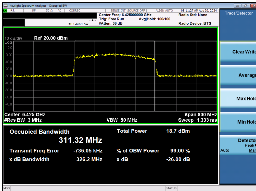
Plot 7-59. 26dB Bandwidth Plot MIMO ANT2 (320MHz 802.11be (UNII Band 5/6/7) – Ch. 95)
