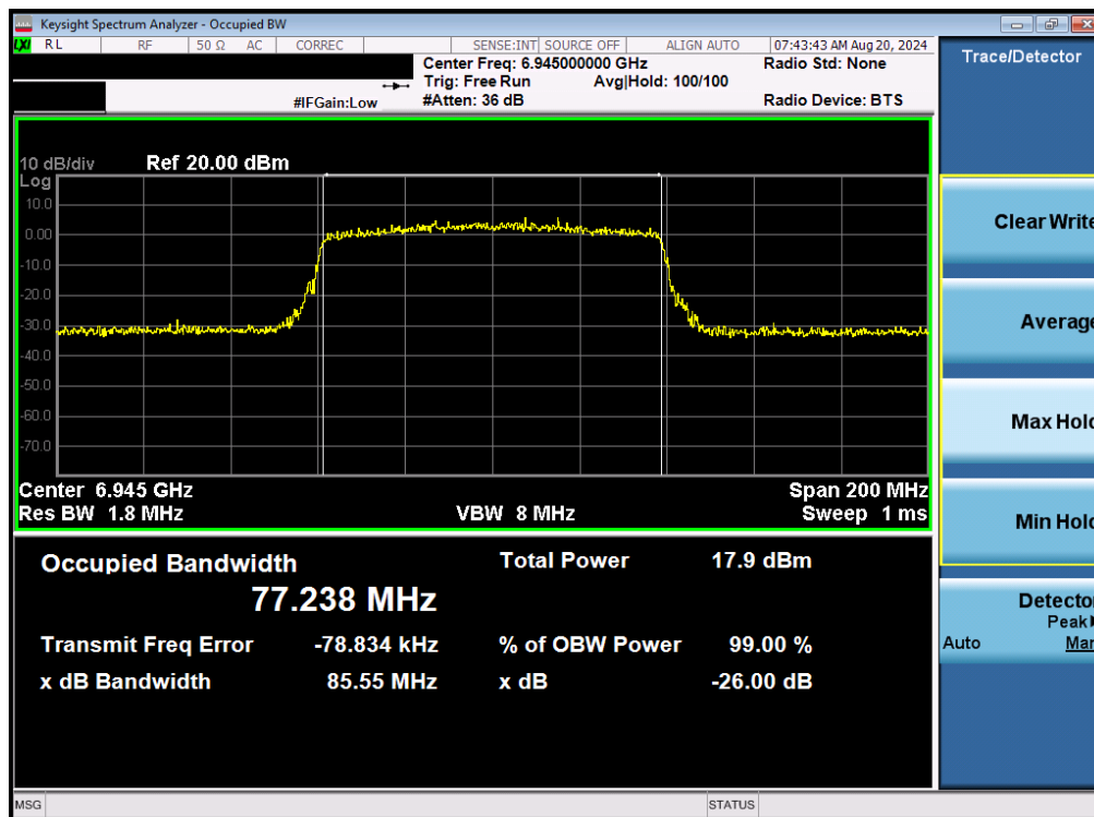
Plot 7-75. 26dB Bandwidth Plot MIMO ANT2 (80MHz 802.11be (UNII Band 8) – Ch. 199)
