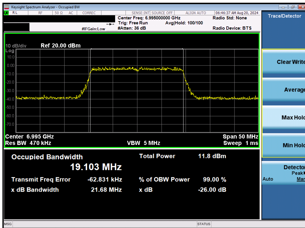
Plot 7-73. 26dB Bandwidth Plot MIMO ANT2 (20MHz 802.11be (UNII Band 8) – Ch. 209)
