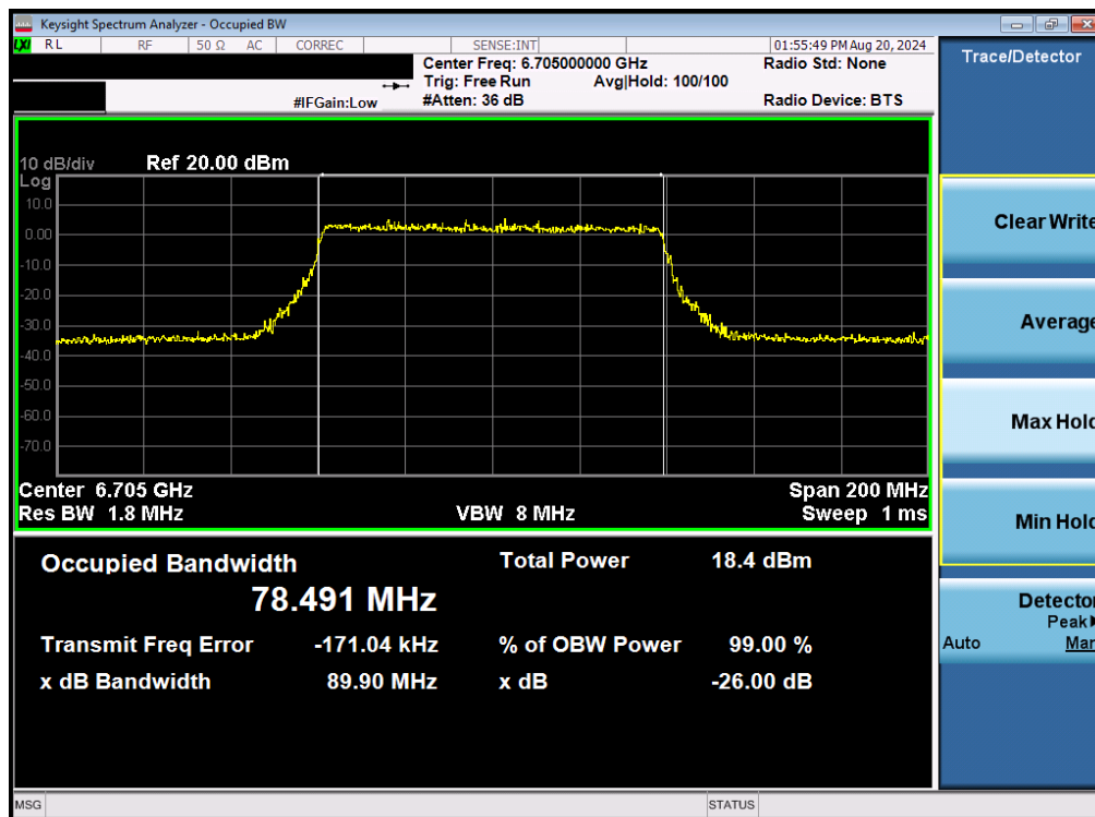
Plot 7-25. 26dB Bandwidth Plot MIMO ANT1 (80MHz 802.11be (UNII Band 7) – Ch. 151)
