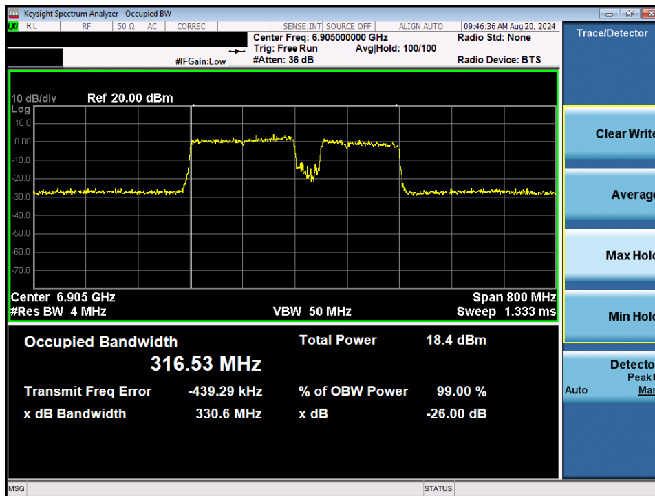
Plot 7-80. 26dB Bandwidth Plot MIMO ANT2 (320MHz 802.11be (UNII Band 8) – Ch. 191) – 40MHz Punctured
