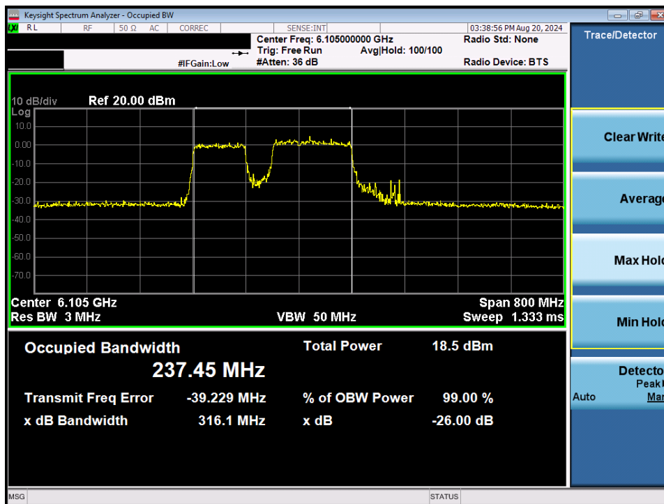
Plot 7-12. 26dB Bandwidth Plot MIMO ANT1 (320MHz 802.11be (UNII Band 5) – Ch. 31) – 120MHz Punctured
