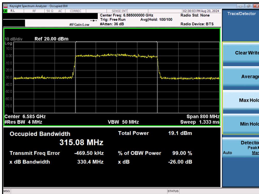
Plot 7-27. 26dB Bandwidth Plot MIMO ANT1 (320MHz 802.11be (UNII Band 7) – Ch. 127)
