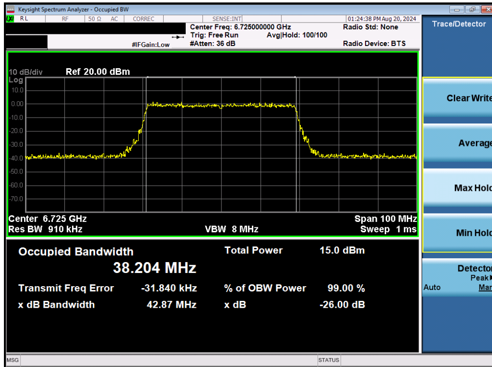
Plot 7-24. 26dB Bandwidth Plot MIMO ANT1 (40MHz 802.11be (UNII Band 7) – Ch. 155)
