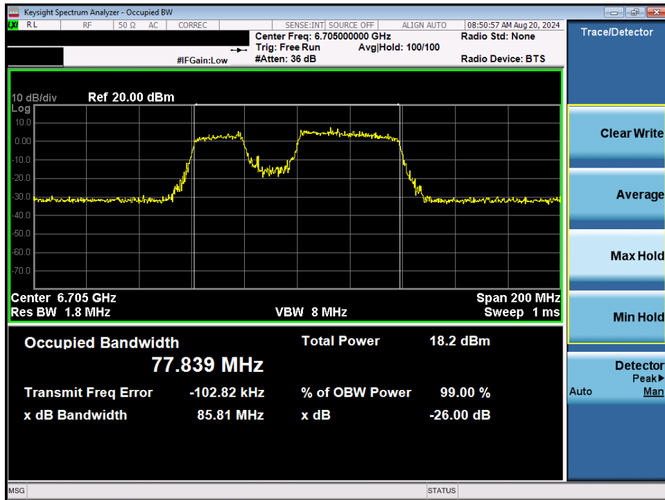
Plot 7-69. 26dB Bandwidth Plot MIMO ANT2 (80MHz 802.11be (UNII Band 7) – Ch. 151) – 20MHz Punctured
