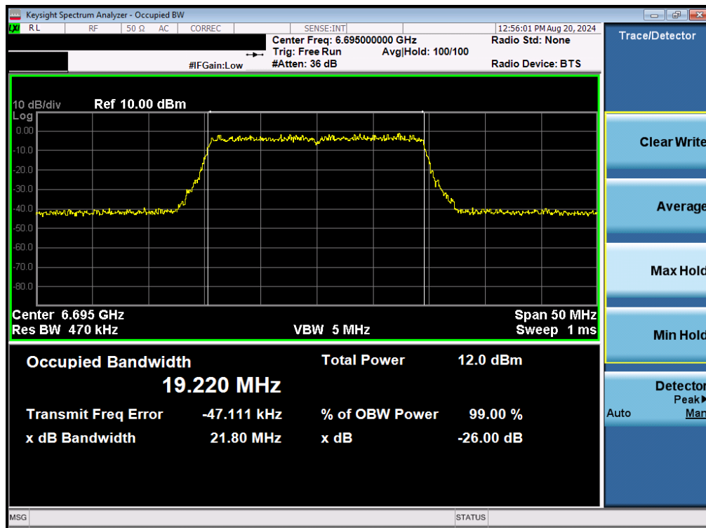
Plot 7-23. 26dB Bandwidth Plot MIMO ANT1 (20MHz 802.11be (UNII Band 7) – Ch. 149)
