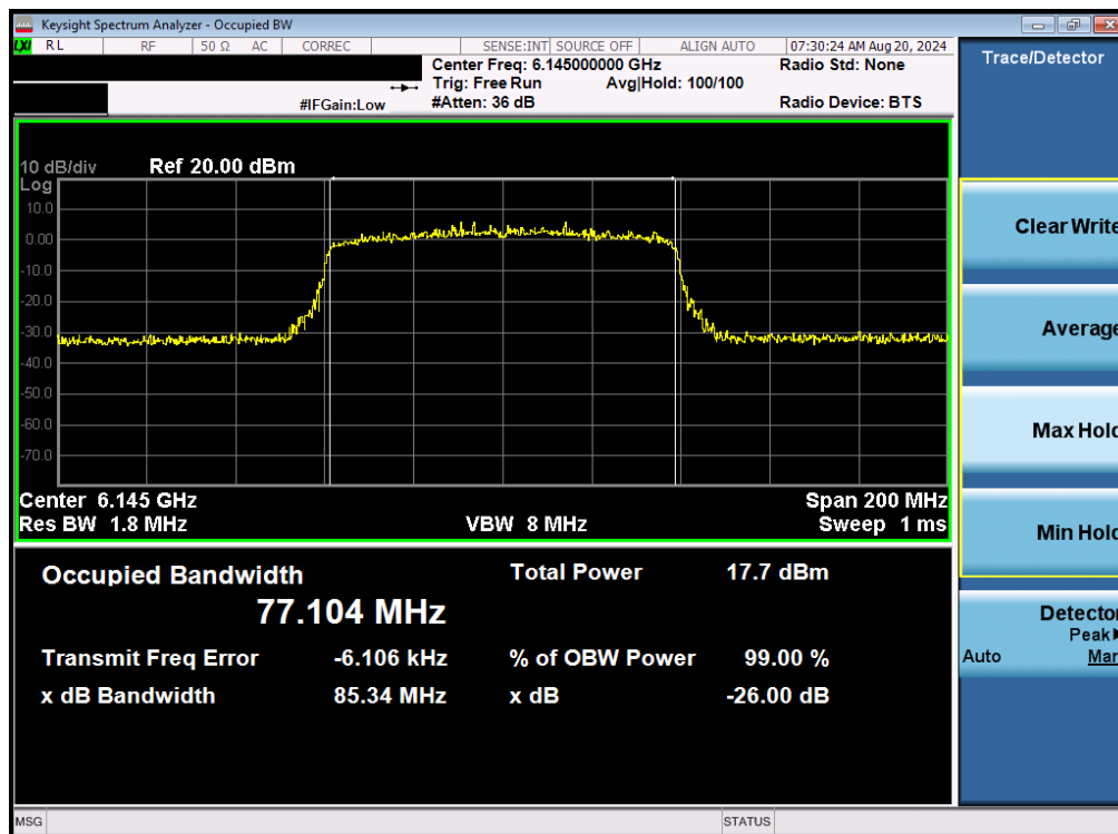
Plot 7-45. 26dB Bandwidth Plot MIMO ANT2 (80MHz 802.11be (UNII Band 5) – Ch. 39)
