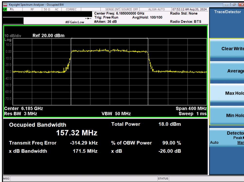
Plot 7-46. 26dB Bandwidth Plot MIMO ANT2 (160MHz 802.11be (UNII Band 5) – Ch. 47)
