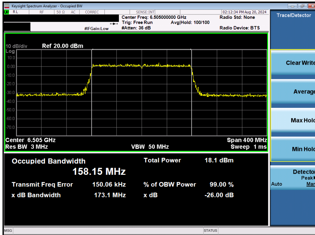
Plot 7-17. 26dB Bandwidth Plot MIMO ANT1 (160MHz 802.11be (UNII Band 6) – Ch. 111)
