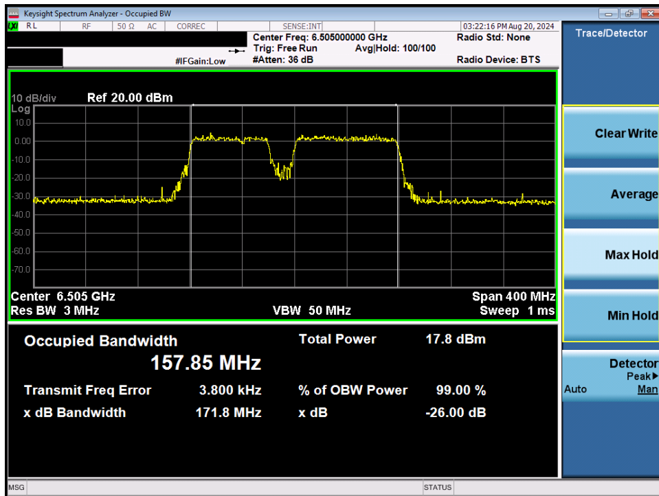
Plot 7-20. 26dB Bandwidth Plot MIMO ANT1 (160MHz 802.11be (UNII Band 6) – Ch. 111) – 20MHz Punctured
