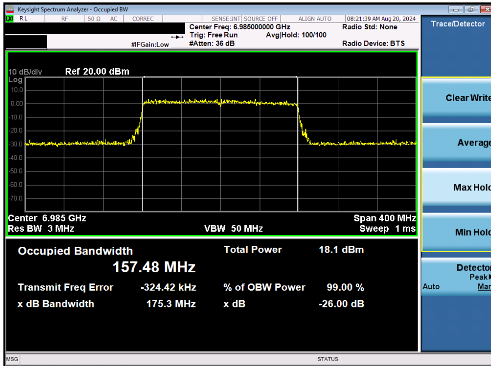
Plot 7-76. 26dB Bandwidth Plot MIMO ANT2 (160MHz 802.11be (UNII Band 8) – Ch. 207)
