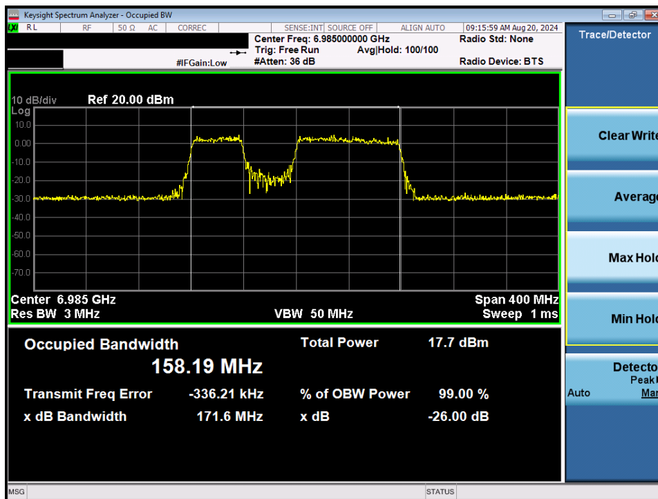
Plot 7-79. 26dB Bandwidth Plot MIMO ANT2 (160MHz 802.11be (UNII Band 8) – Ch. 207) – 40MHz Punctured
