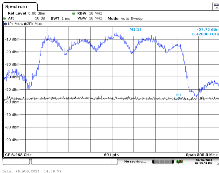
Plot 7-412. CBP 320MHz Channel - Injection Upper Edge – [6420 MHz]
