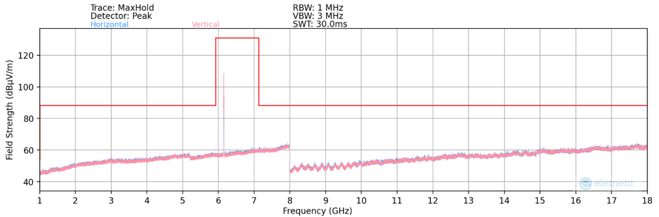
Plot 7-413. Radiated Spurious Plot 1GHz – 18GHz MIMO (802.11ax – UNII Band 5 Ch. 45) – SP
