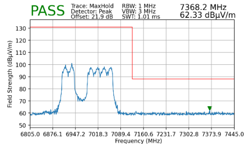
Plot 7-456. Radiated Upper Band Edge Plot MIMO (Peak – UNII Band 8 – 3x996+484T)
