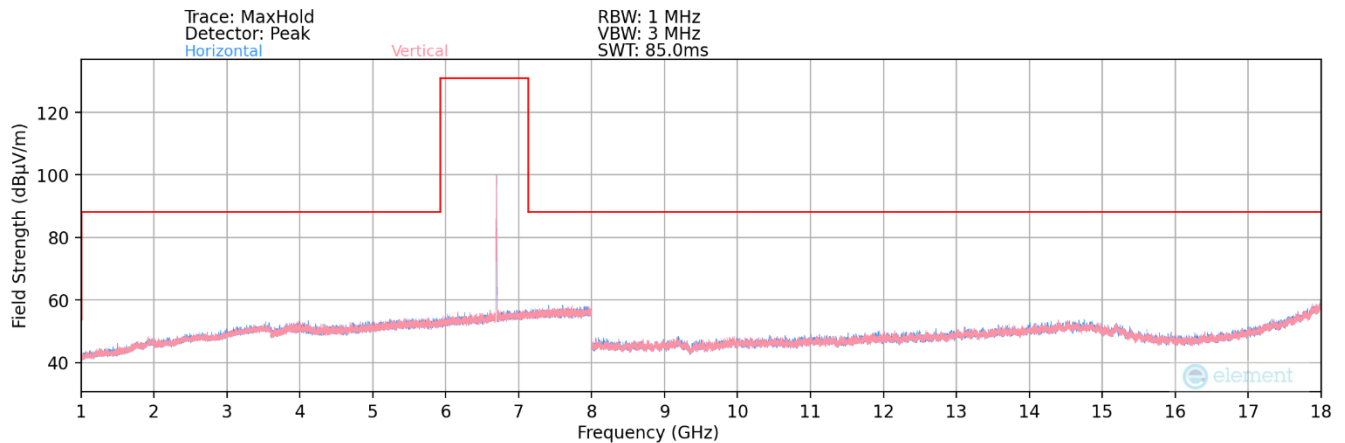
Plot 7-415. Radiated Spurious Plot 1GHz – 18GHz MIMO (802.11ax – UNII Band 7 Ch. 149) – SP
