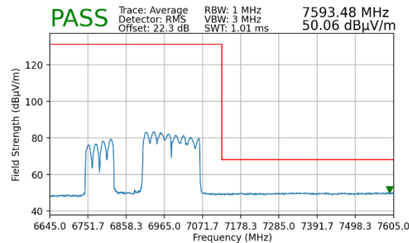
Plot 7-459. Radiated Upper Band Edge Plot MIMO (Average – UNII Band 8 – 3x996T)
