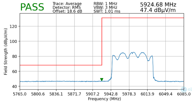
Plot 7-441. Radiated Lower Band Edge Plot MIMO (Average – UNII Band 5 – 996T)
