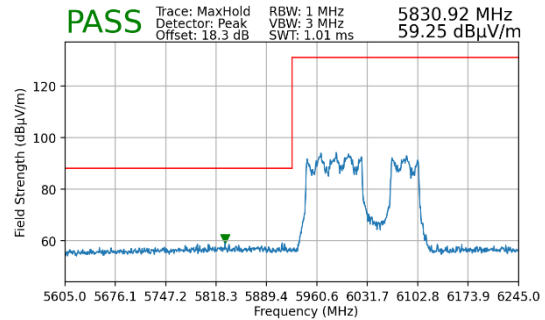
Plot 7-454. Radiated Lower Band Edge Plot MIMO (Peak – UNII Band 5 – 996+484T)
