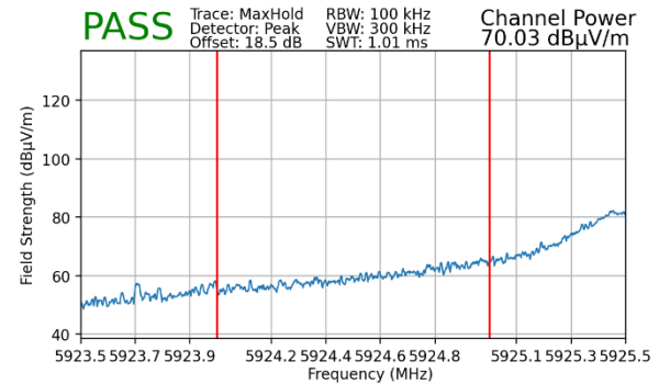
Plot 7-434. Radiated Lower Band Edge Plot MIMO (Peak – UNII Band 5 – 106+26T)
