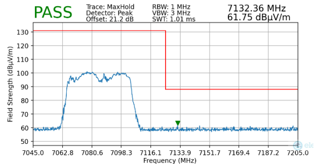
Plot 7-440. Radiated Upper Band Edge Plot MIMO (Peak – UNII Band 8 – 484T)
