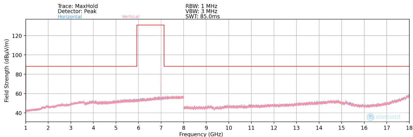
Plot 7-416. Radiated Spurious Plot 1GHz – 18GHz MIMO (802.11ax – UNII Band 8 Ch. 209) – LPI
