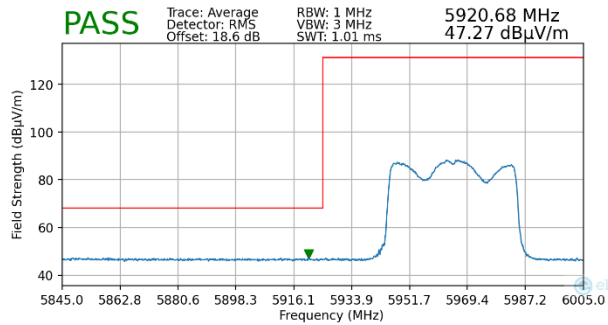
Plot 7-437. Radiated Lower Band Edge Plot MIMO (Average – UNII Band 5 – 484T)
