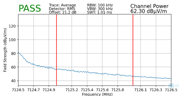
Plot 7-435. Radiated Upper Band Edge Plot MIMO (Average – UNII Band 8 – 106+26T)
