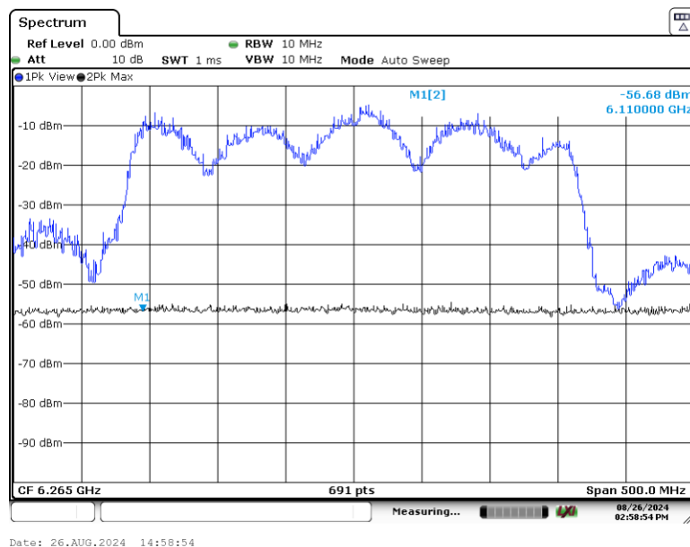
Plot 7-410. CBP 320MHz Channel - Injection Lower Edge – [6110 MHz]
