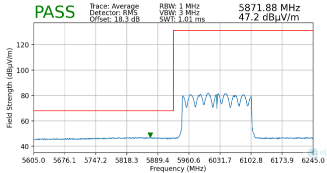
Plot 7-449. Radiated Lower Band Edge Plot MIMO (Average – UNII Band 5 – 2x996T)
