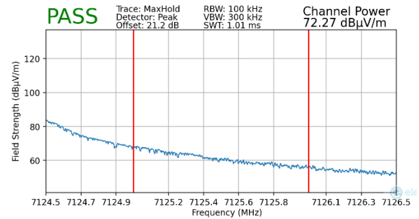
Plot 7-432. Radiated Upper Band Edge Plot MIMO (Peak – UNII Band 8 – 242T)
