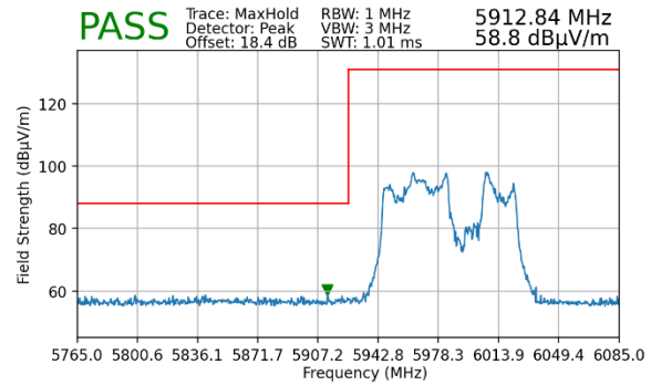
Plot 7-446. Radiated Lower Band Edge Plot MIMO (Peak – UNII Band 5 – 484+242T)
