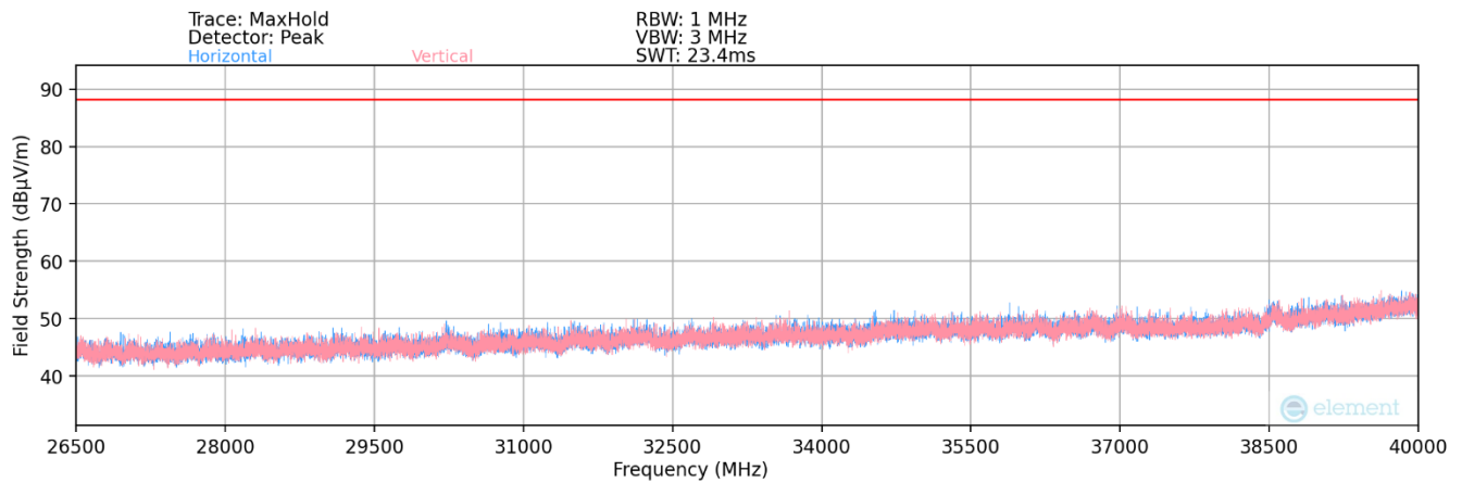
Plot 7-424. Radiated Spurious Plot 26.5GHz - 40GHz (802.11ax) – SP
