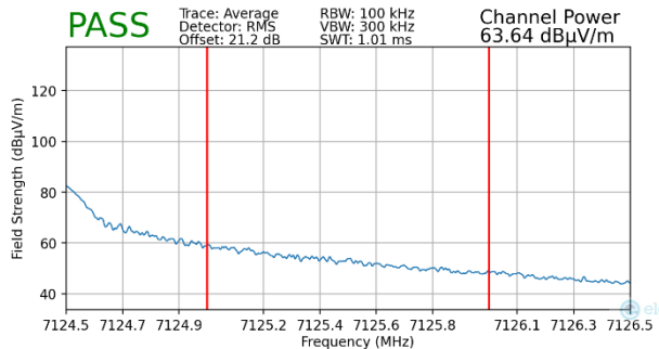
Plot 7-427. Radiated Upper Band Edge Plot MIMO (Average – UNII Band 8 – 106T)
