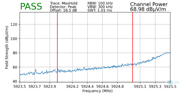
Plot 7-430. Radiated Lower Band Edge Plot MIMO (Peak – UNII Band 5 – 242T)
