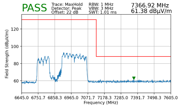
Plot 7-460. Radiated Upper Band Edge Plot MIMO (Peak – UNII Band 8 – 3x996T)
