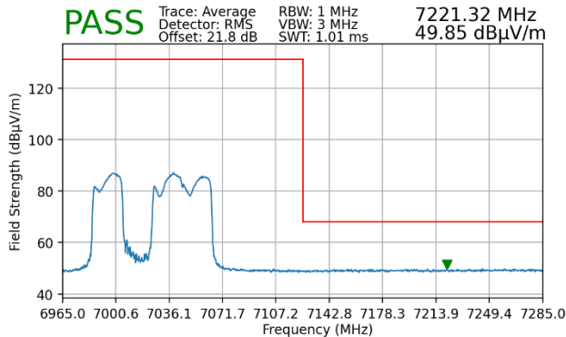
Plot 7-447. Radiated Upper Band Edge Plot MIMO (Average – UNII Band 8 – 484+242T)
