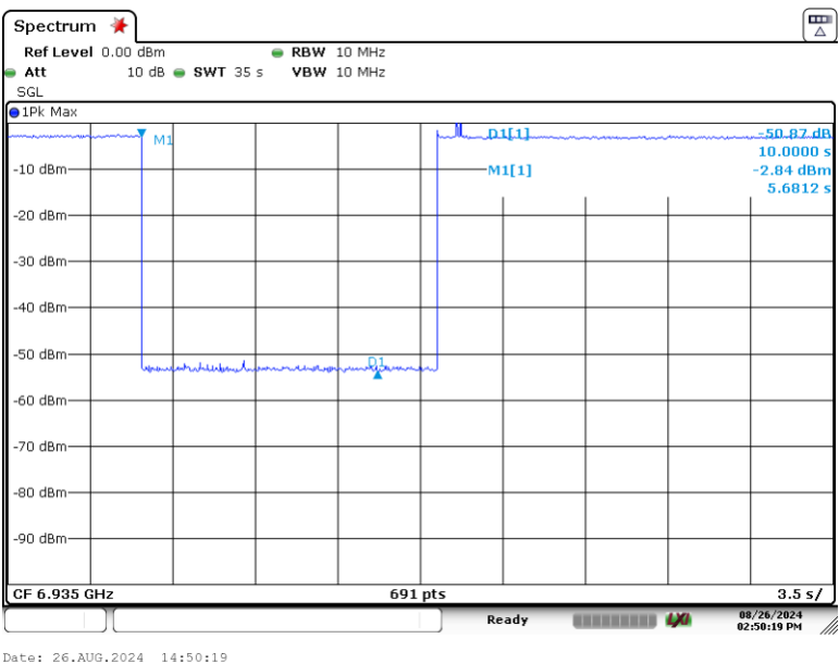
Plot 7-406. Contention Based Protocol Timing Plot (20MHz (UNII Band 8) – Ch. 197)
