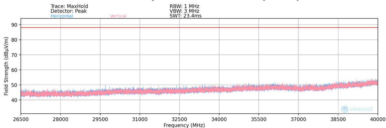
Plot 7-418. Radiated Spurious Plot 26.5GHz - 40GHz (802.11ax) – SP
