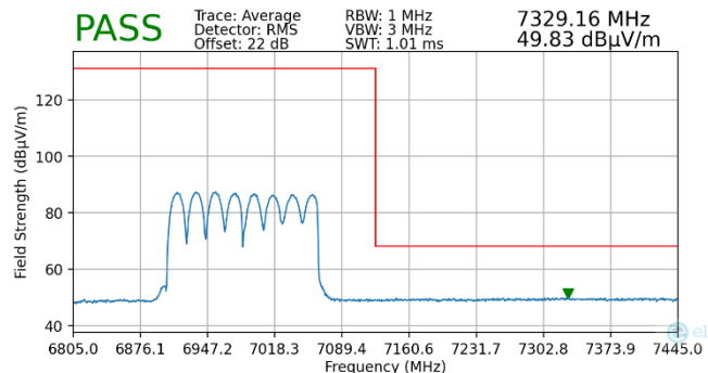
Plot 7-451. Radiated Upper Band Edge Plot MIMO (Average – UNII Band 8 – 2x996T)
