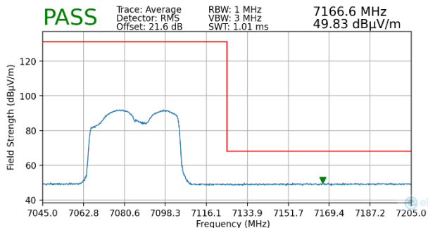
Plot 7-439. Radiated Upper Band Edge Plot MIMO (Average – UNII Band 8 – 484T)
