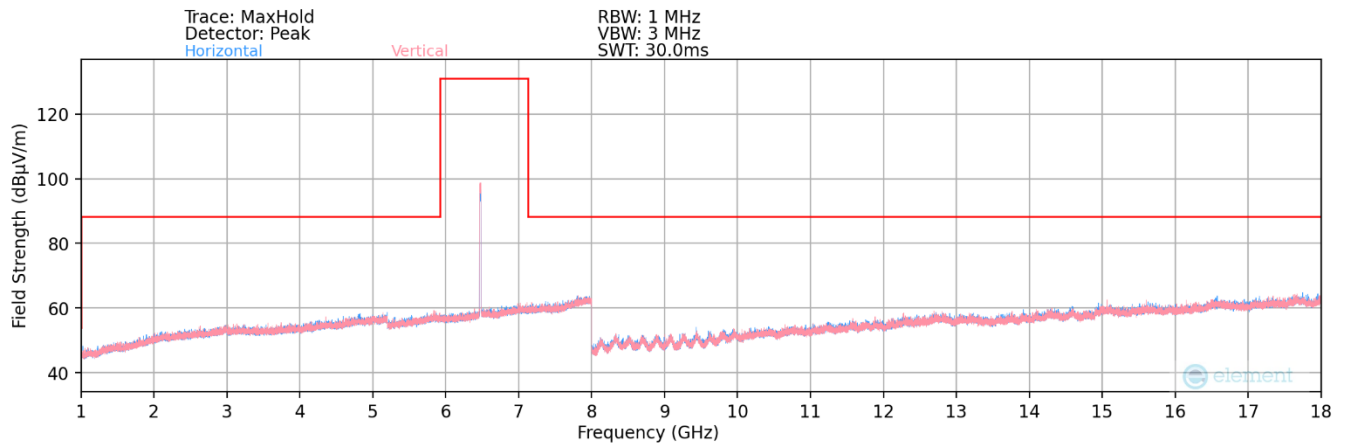
Plot 7-420. Radiated Spurious Plot 1GHz – 18GHz MIMO (802.11ax – UNII Band 6 Ch. 105) – LPI
