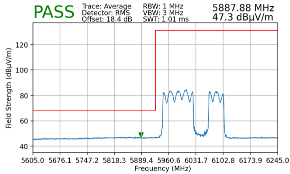
Plot 7-453. Radiated Lower Band Edge Plot MIMO (Average – UNII Band 5 – 996+484T)
