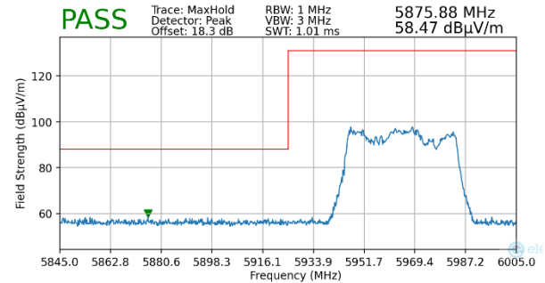
Plot 7-438. Radiated Lower Band Edge Plot MIMO (Peak – UNII Band 5 – 484T)
