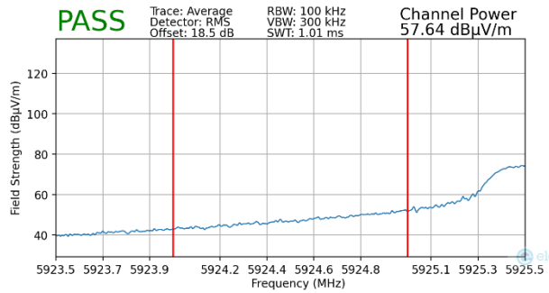
Plot 7-429. Radiated Lower Band Edge Plot MIMO (Average – UNII Band 5 – 242T)
