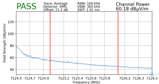
Plot 7-431. Radiated Upper Band Edge Plot MIMO (Average – UNII Band 8 – 242T)
