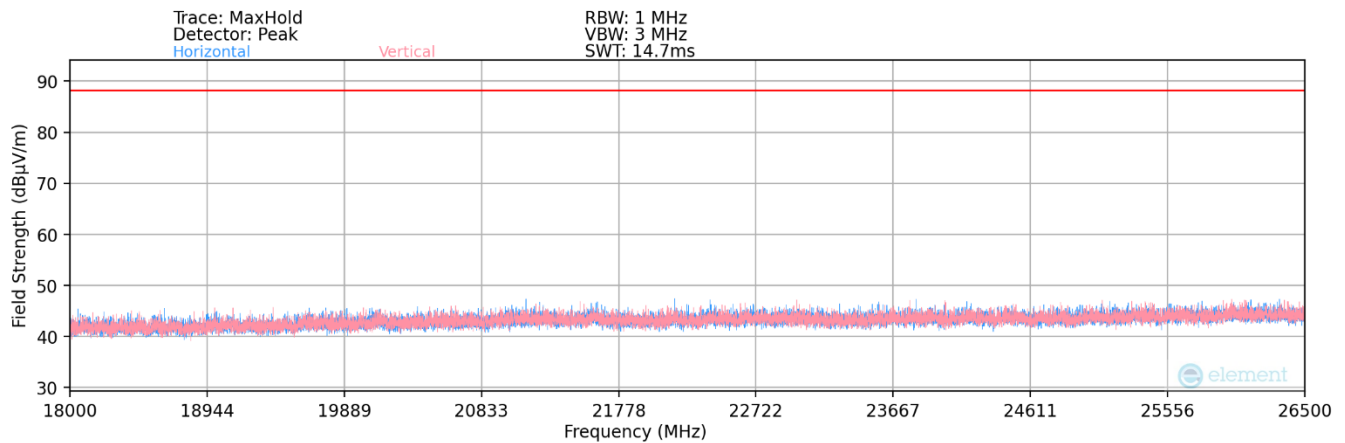
Plot 7-423. Radiated Spurious Plot 18GHz - 26.5GHz (802.11ax) – SP
