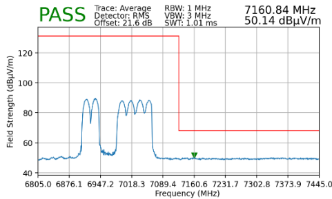
Plot 7-455. Radiated Upper Band Edge Plot MIMO (Average – UNII Band 8 – 3x996+484T)
