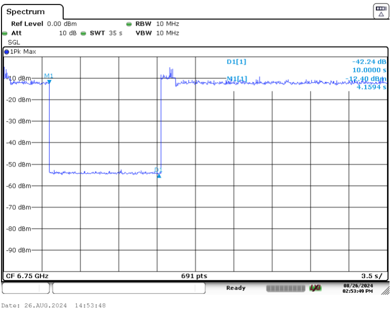
Plot 7-407. Contention Based Protocol Timing Plot (320MHz (UNII Band 8) – Ch. 191 Low)
