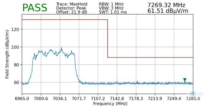
Plot 7-444. Radiated Upper Band Edge Plot MIMO (Peak – UNII Band 8 – 996T)
