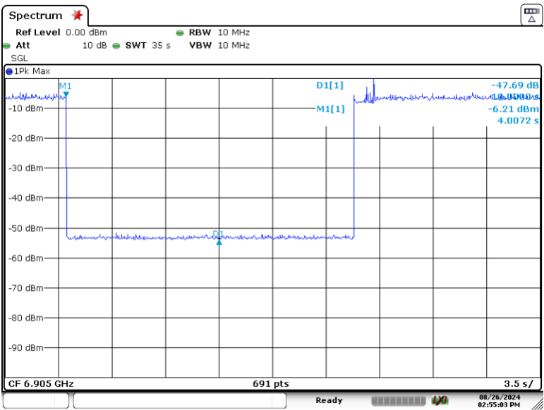
Plot 7-408. Contention Based Protocol Timing Plot (320MHz (UNII Band 8) – Ch. 191 Mid)
