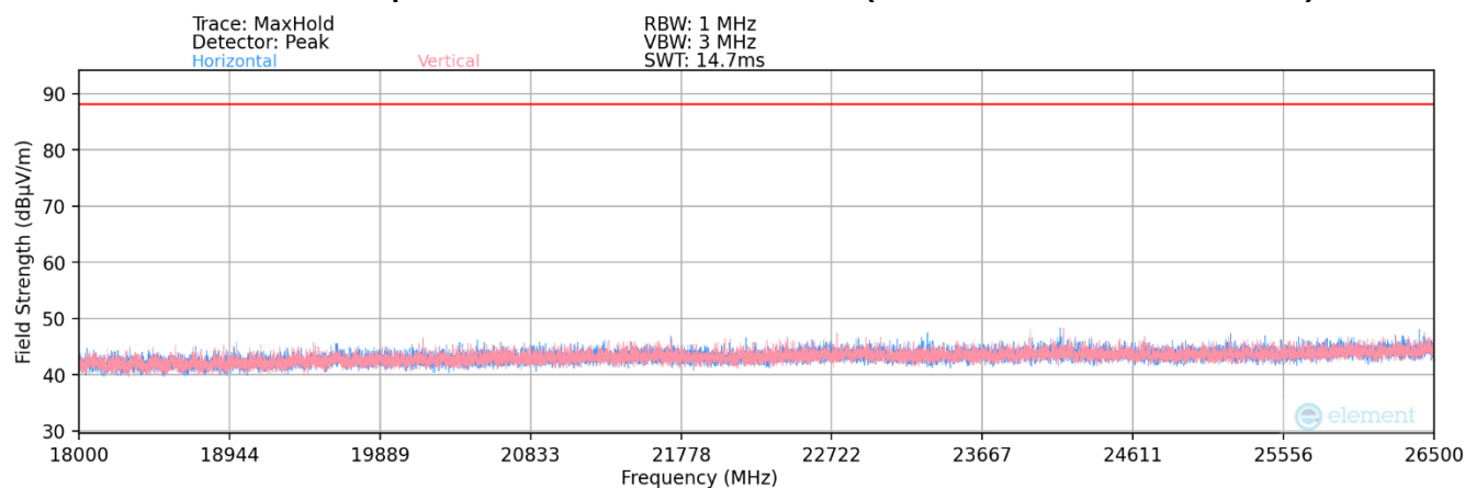
Plot 7-417. Radiated Spurious Plot 18GHz - 26.5GHz (802.11ax) – SP
