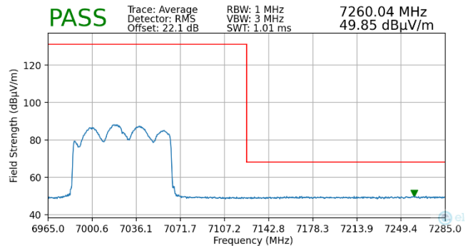
Plot 7-443. Radiated Upper Band Edge Plot MIMO (Average – UNII Band 8 – 996T)
