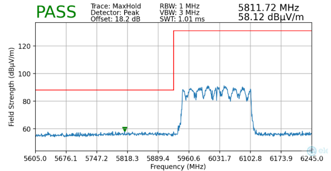
Plot 7-450. Radiated Lower Band Edge Plot MIMO (Peak – UNII Band 5 – 2x996T)
