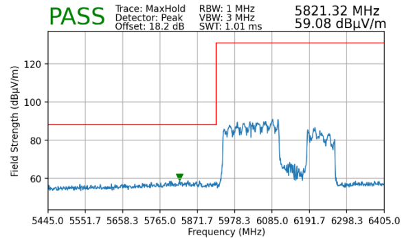
Plot 7-458. Radiated Lower Band Edge Plot MIMO (Peak – UNII Band 5 – 3x996T)
