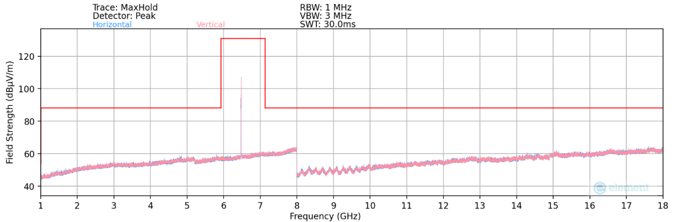
Plot 7-414. Radiated Spurious Plot 1GHz – 18GHz MIMO (802.11ax – UNII Band 6 Ch. 105) – LPI
