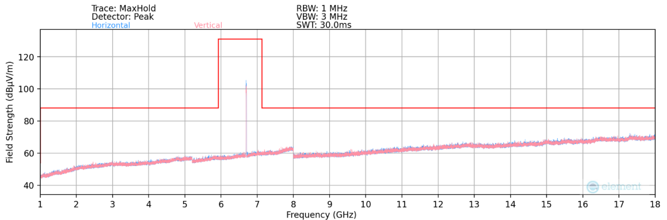
Plot 7-421. Radiated Spurious Plot 1GHz – 18GHz MIMO (802.11ax – UNII Band 7 Ch. 149) – SP
