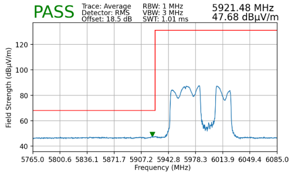
Plot 7-445. Radiated Lower Band Edge Plot MIMO (Average – UNII Band 5 – 484+242T)
