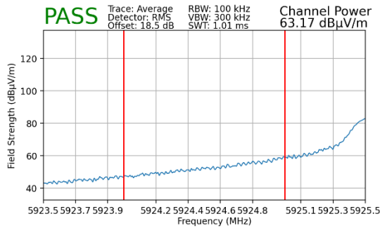
Plot 7-425. Radiated Lower Band Edge Plot MIMO (Average – UNII Band 5 – 106T)
