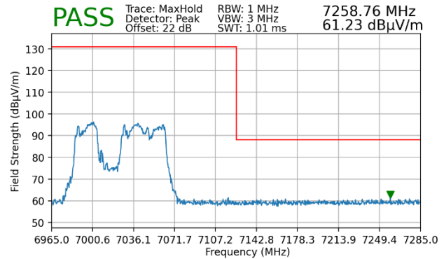
Plot 7-448. Radiated Upper Band Edge Plot MIMO (Peak – UNII Band 8 – 484+242T)
