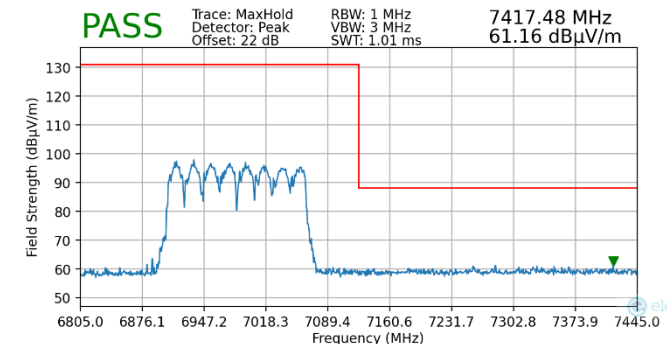
Plot 7-452. Radiated Upper Band Edge Plot MIMO (Peak – UNII Band 8 – 2x996T)
