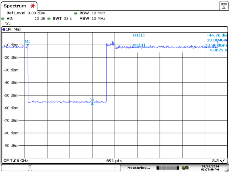
Plot 7-409. Contention Based Protocol Timing Plot (320MHz (UNII Band 8) – Ch. 191 High)
