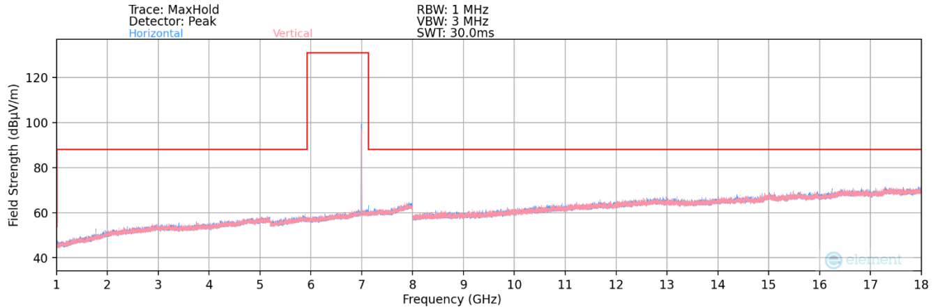
Plot 7-422. Radiated Spurious Plot 1GHz – 18GHz MIMO (802.11ax – UNII Band 8 Ch. 209) – LPI
