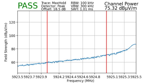
Plot 7-426. Radiated Lower Band Edge Plot MIMO (Peak – UNII Band 5 – 106T)
