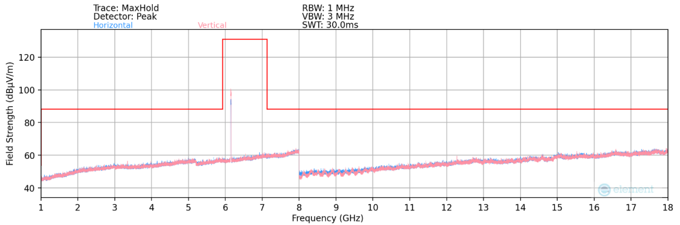
Plot 7-419. Radiated Spurious Plot 1GHz – 18GHz MIMO (802.11ax – UNII Band 5 Ch. 45) – SP
