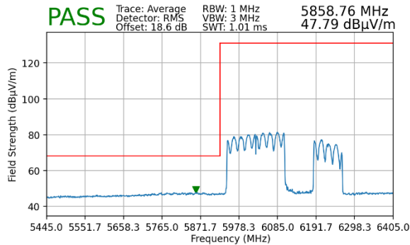
Plot 7-457. Radiated Lower Band Edge Plot MIMO (Average – UNII Band 5 – 3x996T)
