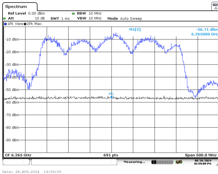
Plot 7-411. CBP 320MHz Channel - Injection Center – [6265 MHz]
