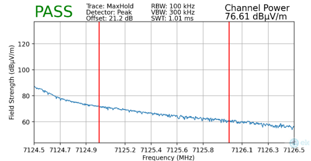
Plot 7-428. Radiated Upper Band Edge Plot MIMO (Peak – UNII Band 8 – 106T)
