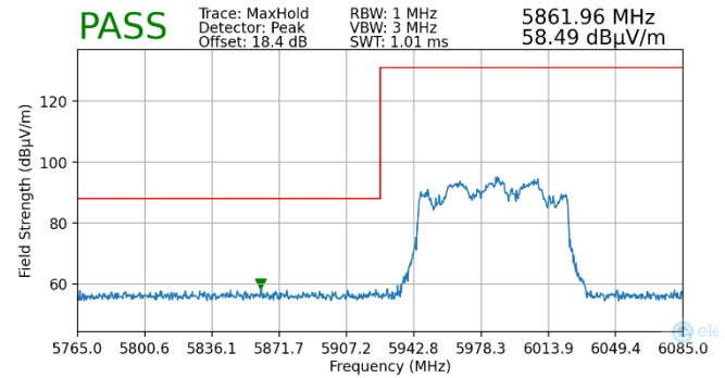
Plot 7-442. Radiated Lower Band Edge Plot MIMO (Peak – UNII Band 5 – 996T)
