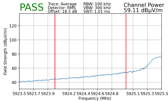
Plot 7-433. Radiated Lower Band Edge Plot MIMO (Average – UNII Band 5 – 106+26T)
