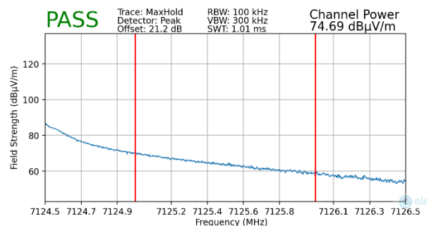
Plot 7-436. Radiated Upper Band Edge Plot MIMO (Peak – UNII Band 8 – 106+26T)
