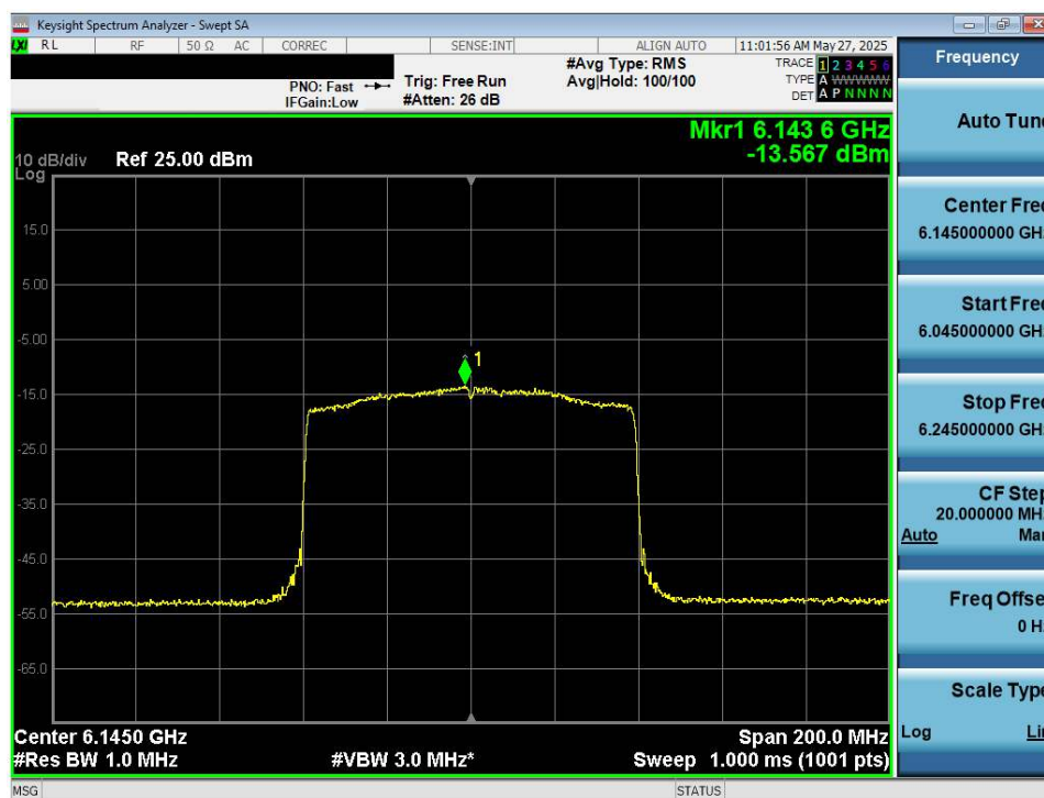
Plot 7-22. Power Spectral Density Plot MIMO ANT1 (80MHz 802.11ax/be (UNII Band 5) – Ch. 39) - VLP
