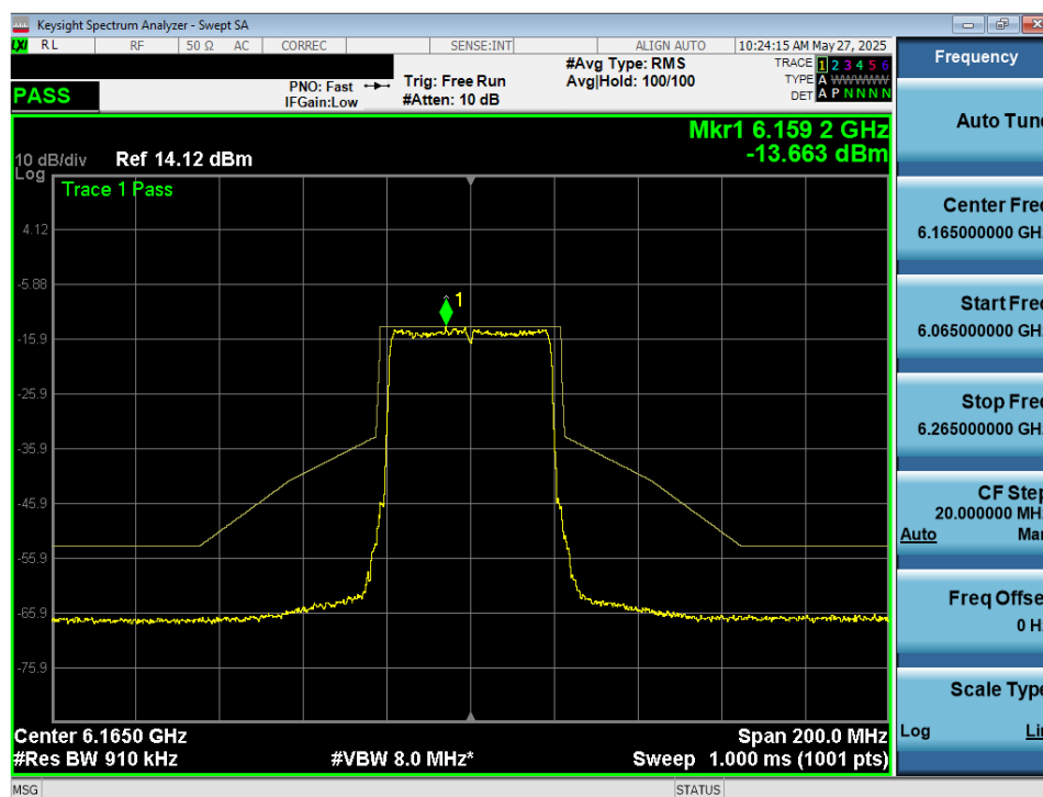
Plot 7-39. In Band Emissions Plot MIMO ANT1 (40MHz 802.11ax/be (UNII Band 5) – Ch. 43) - VLP
