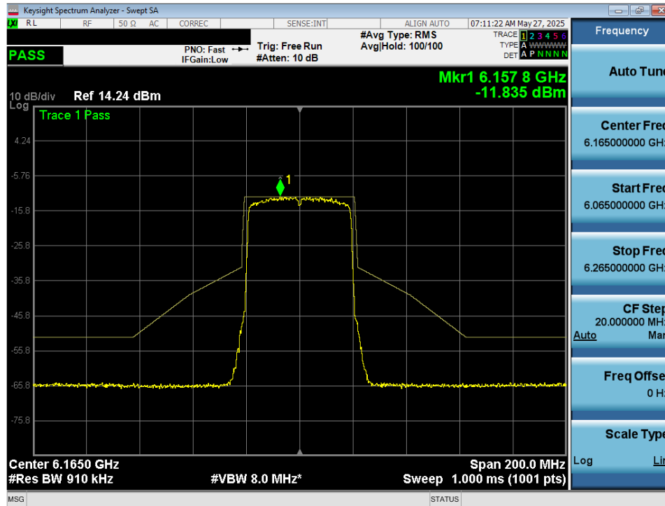
Plot 7-48. In Band Emissions Plot MIMO ANT2 (40MHz 802.11ax/be (UNII Band 5) – Ch. 43) - VLP
