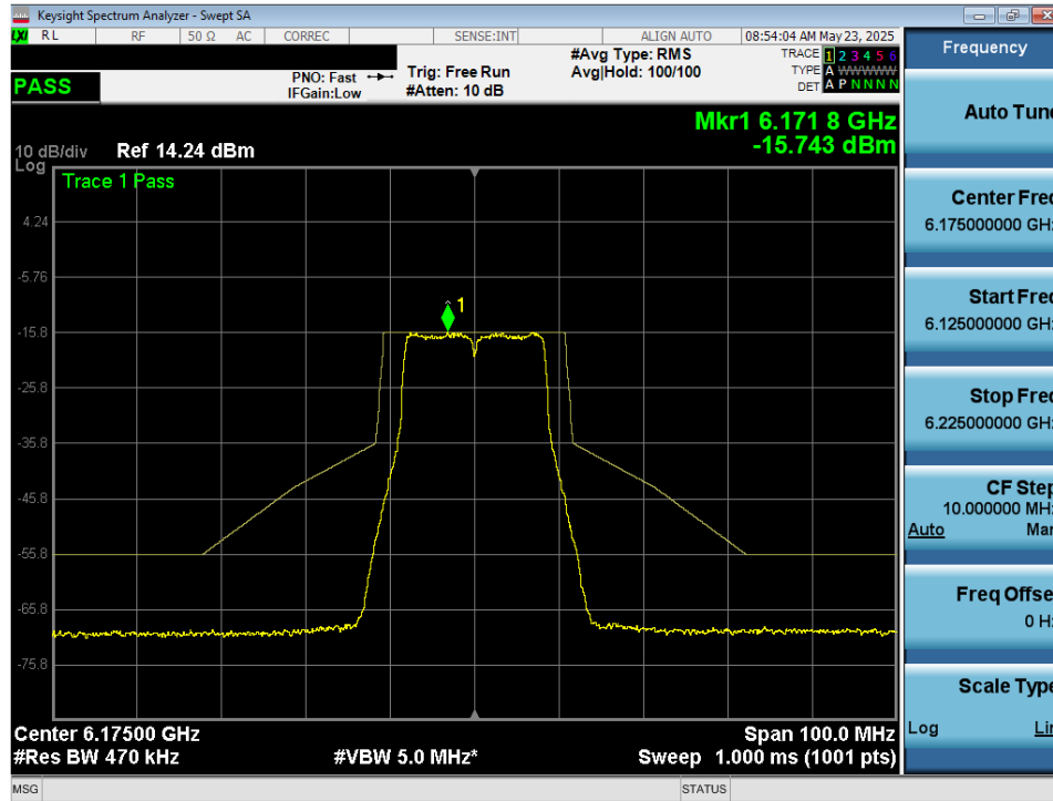
Plot 7-46. In Band Emissions Plot MIMO ANT2 (20MHz 802.11a (UNII Band 5) – Ch. 45) - VLP
