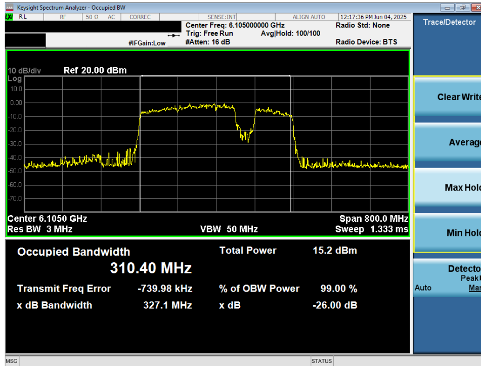
Plot 7-18. 26dB Bandwidth Plot MIMO ANT2 (320MHz 802.11be (UNII Band 5) – Ch. 31) – 40MHz Punctured - VLP
