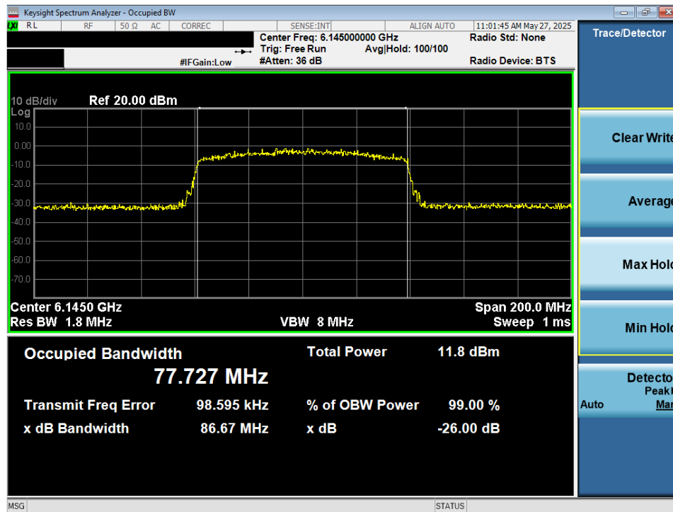
Plot 7-4. 26dB Bandwidth Plot MIMO ANT1 (80MHz 802.11ax/be (UNII Band 5) – Ch. 39) - VLP
