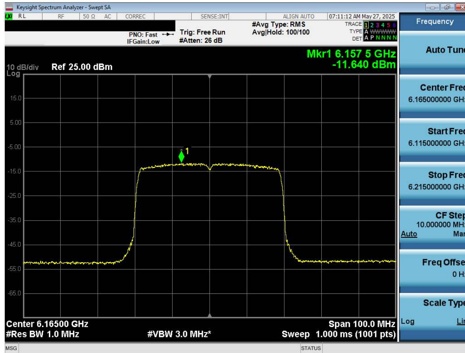
Plot 7-30. Power Spectral Density Plot MIMO ANT2 (40MHz 802.11ax/be (UNII Band 5) – Ch. 43) - VLP
