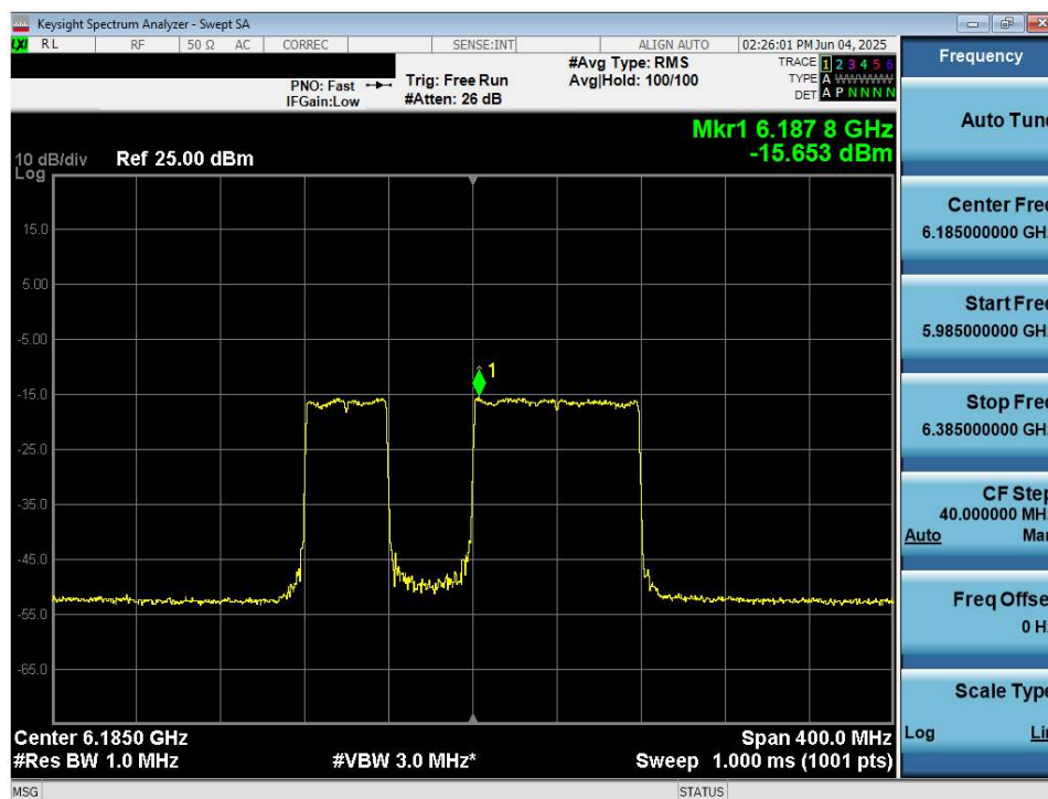
Plot 7-26. Power Spectral Density Plot MIMO ANT1 (160MHz 802.11be (UNII Band 5) – Ch. 47) – 40MHz Punctured - VLP
