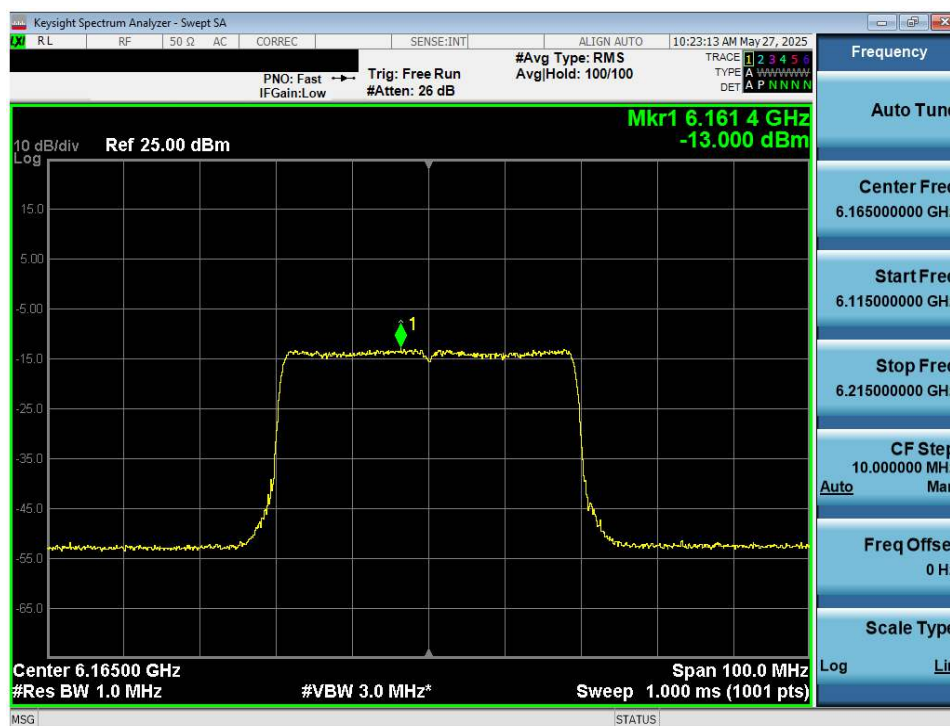
Plot 7-21. Power Spectral Density Plot MIMO ANT1 (40MHz 802.11ax/be (UNII Band 5) – Ch. 43) - VLP
