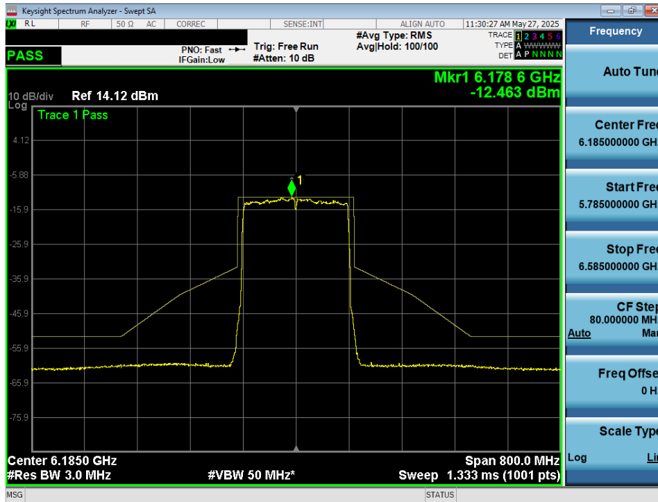
Plot 7-41. In Band Emissions Plot MIMO ANT1 (160MHz 802.11ax/be (UNII Band 5) – Ch. 47) - VLP
