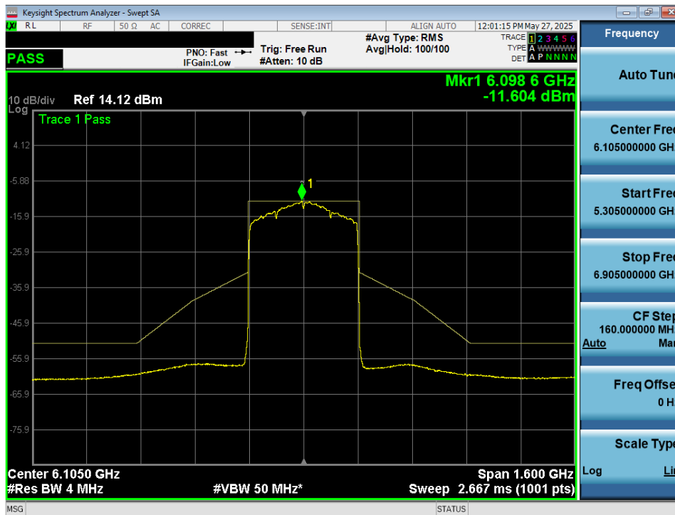
Plot 7-42. In Band Emissions Plot MIMO ANT1 (320MHz 802.11ax/be (UNII Band 5) – Ch. 31) - VLP
