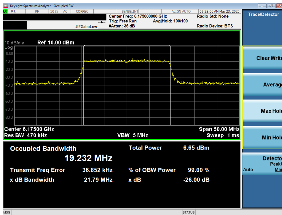
Plot 7-11. 26dB Bandwidth Plot MIMO ANT2 (20MHz 802.11ax/be (UNII Band 5) – Ch. 45) - VLP
