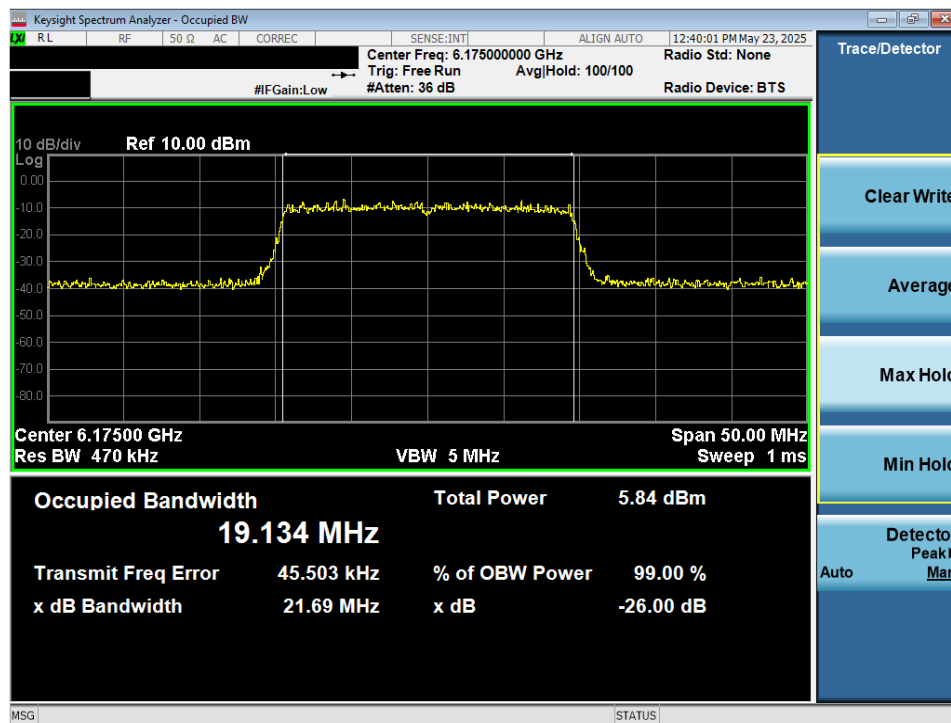
Plot 7-2. 26dB Bandwidth Plot MIMO ANT1 (20MHz 802.11ax/be (UNII Band 5) – Ch. 45) - VLP
