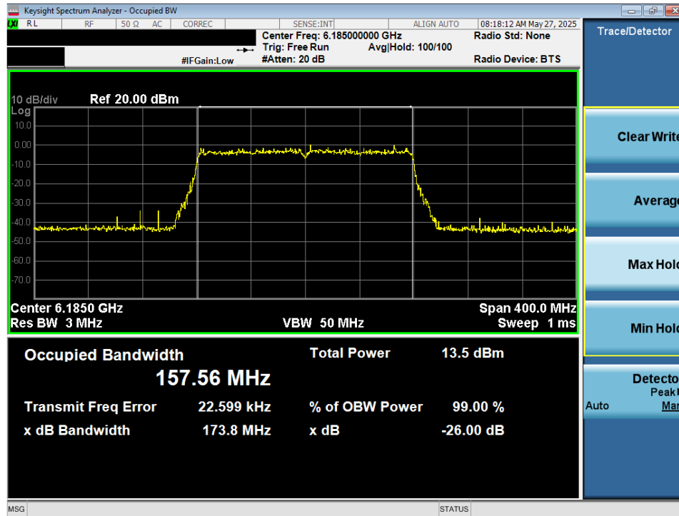
Plot 7-14. 26dB Bandwidth Plot MIMO ANT2 (160MHz 802.11ax/be (UNII Band 5) – Ch. 47) - VLP
