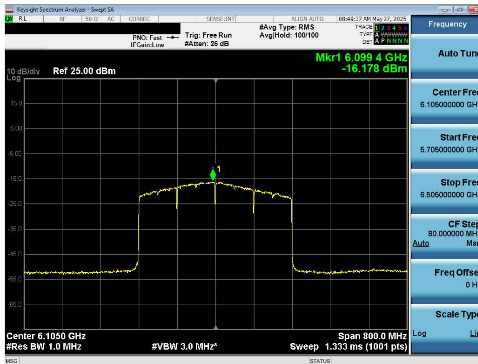
Plot 7-33. Power Spectral Density Plot MIMO ANT2 (320MHz 802.11ax/be (UNII Band 5) – Ch. 31) - VLP
