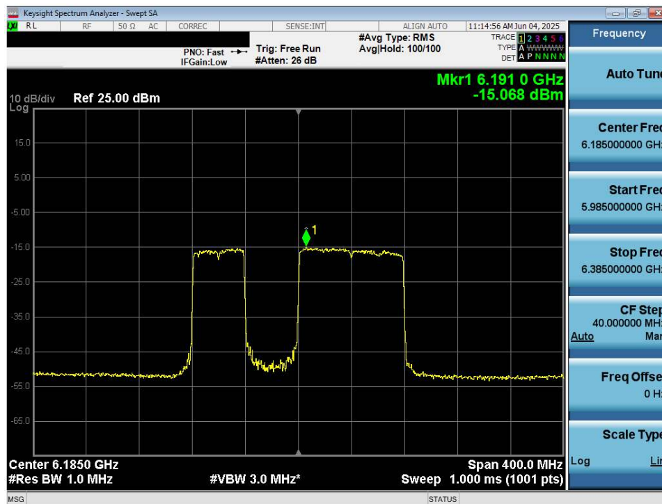
Plot 7-35. Power Spectral Density Plot MIMO ANT2 (160MHz 802.11be (UNII Band 5) – Ch. 47) – 40MHz Punctured - VLP
