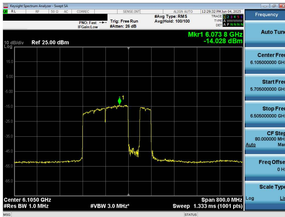
Plot 7-36. Power Spectral Density Plot MIMO ANT2 (320MHz 802.11be (UNII Band 5) – Ch. 31) – 120MHz Punctured – VLP
