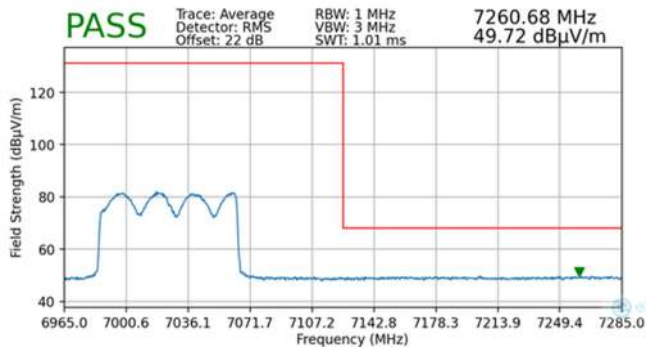
Plot 7-94. Radiated Upper Band Edge Plot MIMO (Average – UNII Band 8)
