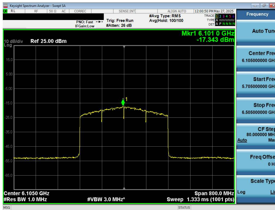
Plot 7-24. Power Spectral Density Plot MIMO ANT1 (320MHz 802.11ax/be (UNII Band 5) – Ch. 31) - VLP
