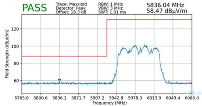
Plot 7-93. Radiated Lower Band Edge Plot MIMO (Peak – UNII Band 5)
