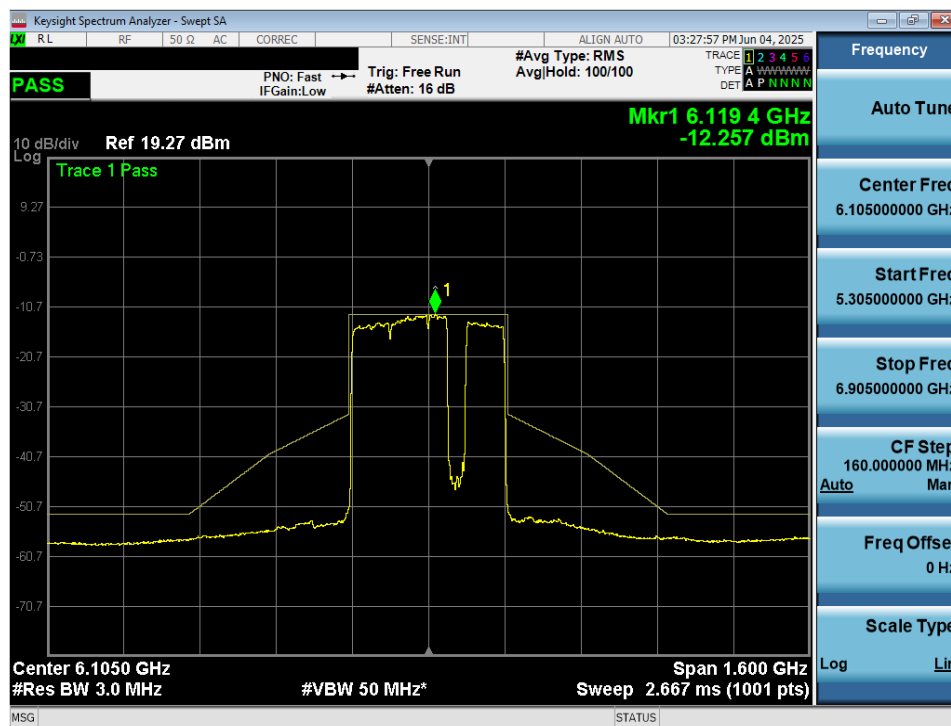
Plot 7-45. In Band Emissions Plot MIMO ANT1 (320MHz 802.11be (UNII Band 5) – Ch. 31) – 40MHz Punctured - VLP
