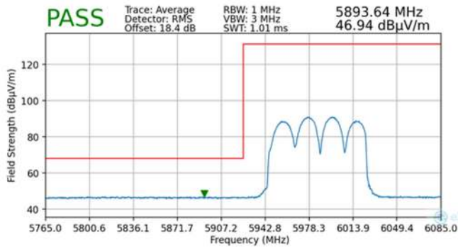
Plot 7-92. Radiated Lower Band Edge Plot MIMO (Average – UNII Band 5)
