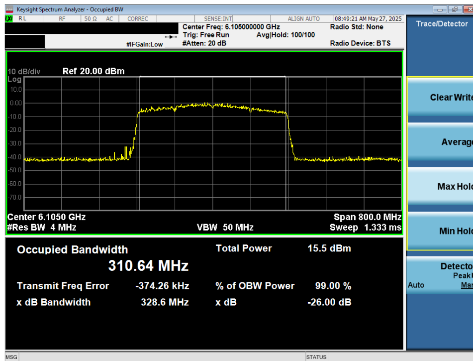
Plot 7-15. 26dB Bandwidth Plot MIMO ANT2 (320MHz 802.11ax/be (UNII Band 5) – Ch. 31) - VLP
