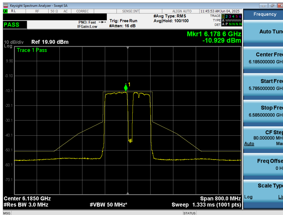
Plot 7-53. In Band Emissions Plot MIMO ANT2 (160MHz 802.11be (UNII Band 5) – Ch. 47) – 20MHz Punctured - VLP
