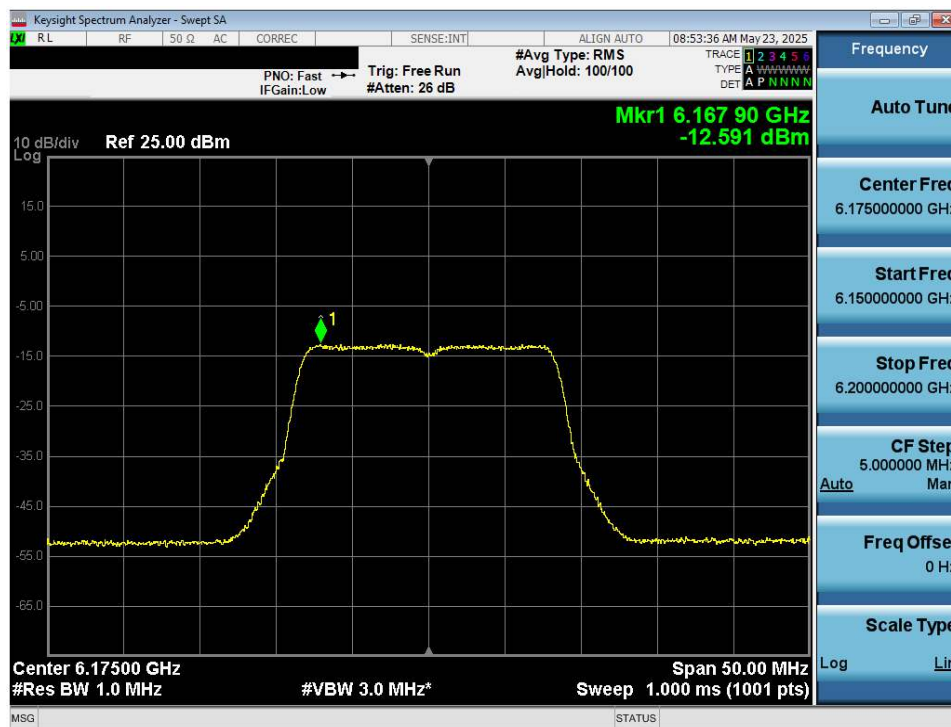
Plot 7-28. Power Spectral Density Plot MIMO ANT2 (20MHz 802.11a (UNII Band 5) – Ch. 45) - VLP
