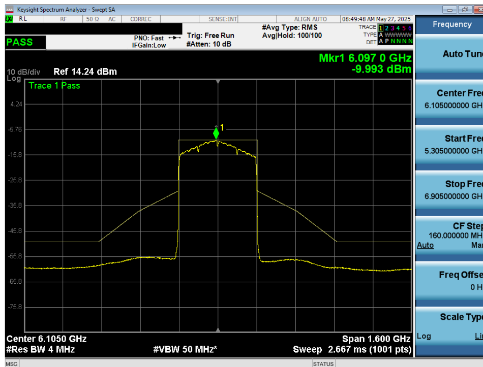
Plot 7-51. In Band Emissions Plot MIMO ANT2 (320MHz 802.11ax/be (UNII Band 5) – Ch. 31) - VLP
