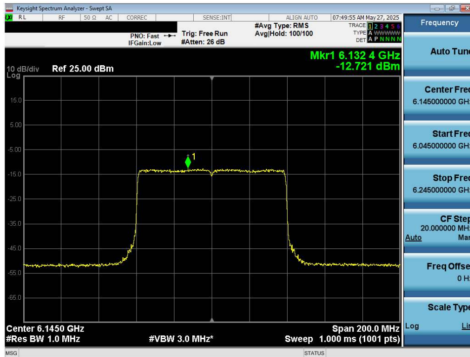
Plot 7-31. Power Spectral Density Plot MIMO ANT2 (80MHz 802.11ax/be (UNII Band 5) – Ch. 39) - VLP
