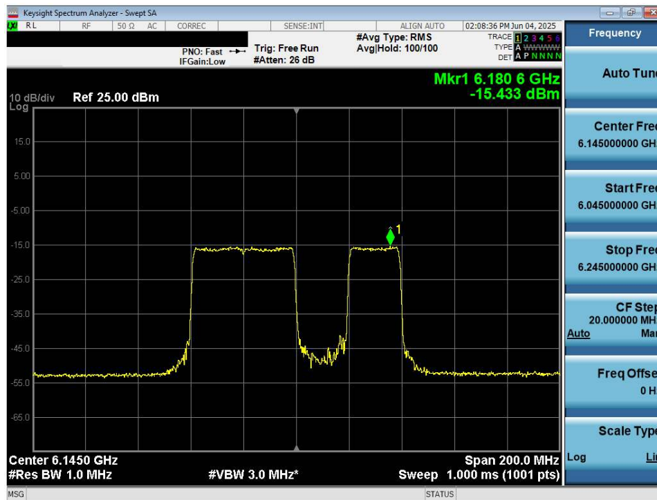
Plot 7-25. Power Spectral Density Plot MIMO ANT1 (80MHz 802.11be (UNII Band 5) – Ch. 39) – 20MHz Punctured - VLP
