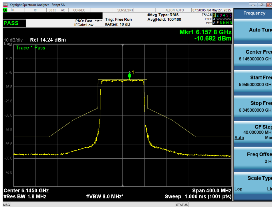
Plot 7-49. In Band Emissions Plot MIMO ANT2 (80MHz 802.11ax/be (UNII Band 5) – Ch. 39) - VLP
