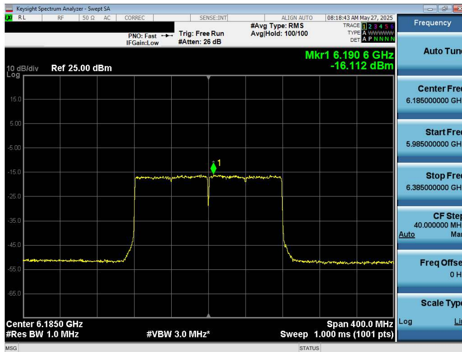
Plot 7-32. Power Spectral Density Plot MIMO ANT2 (160MHz 802.11ax/be (UNII Band 5) – Ch. 47) - VLP
