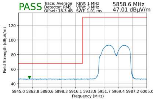
Plot 7-88. Radiated Lower Band Edge Plot MIMO (Average – UNII Band 5)
