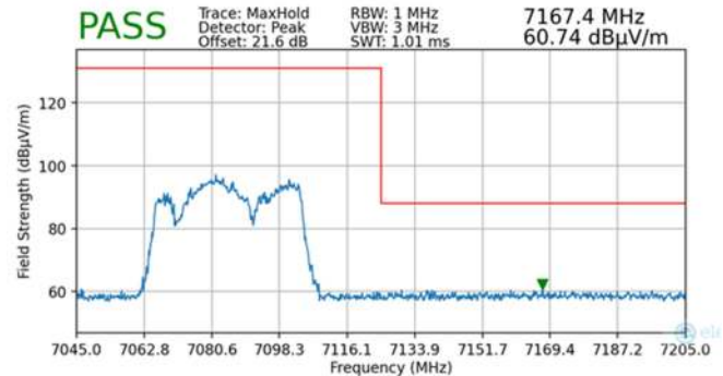
Plot 7-91. Radiated Upper Band Edge Plot MIMO (Peak – UNII Band 8)
