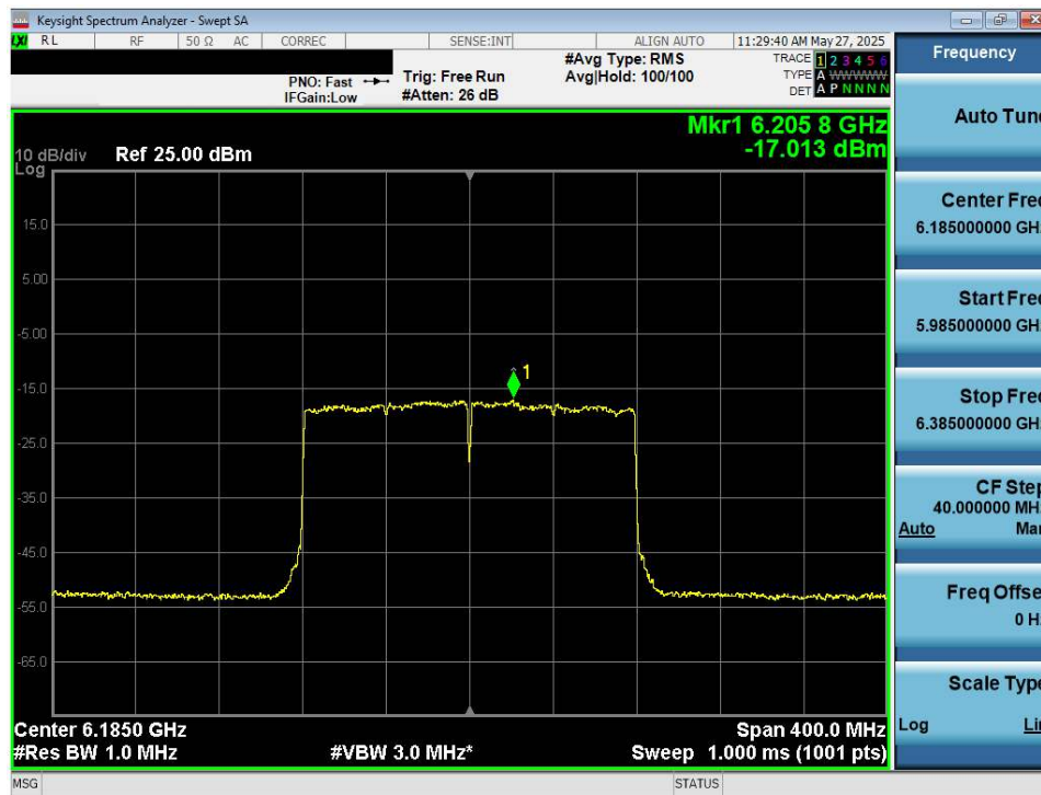
Plot 7-23. Power Spectral Density Plot MIMO ANT1 (160MHz 802.11ax/be (UNII Band 5) – Ch. 47) - VLP
