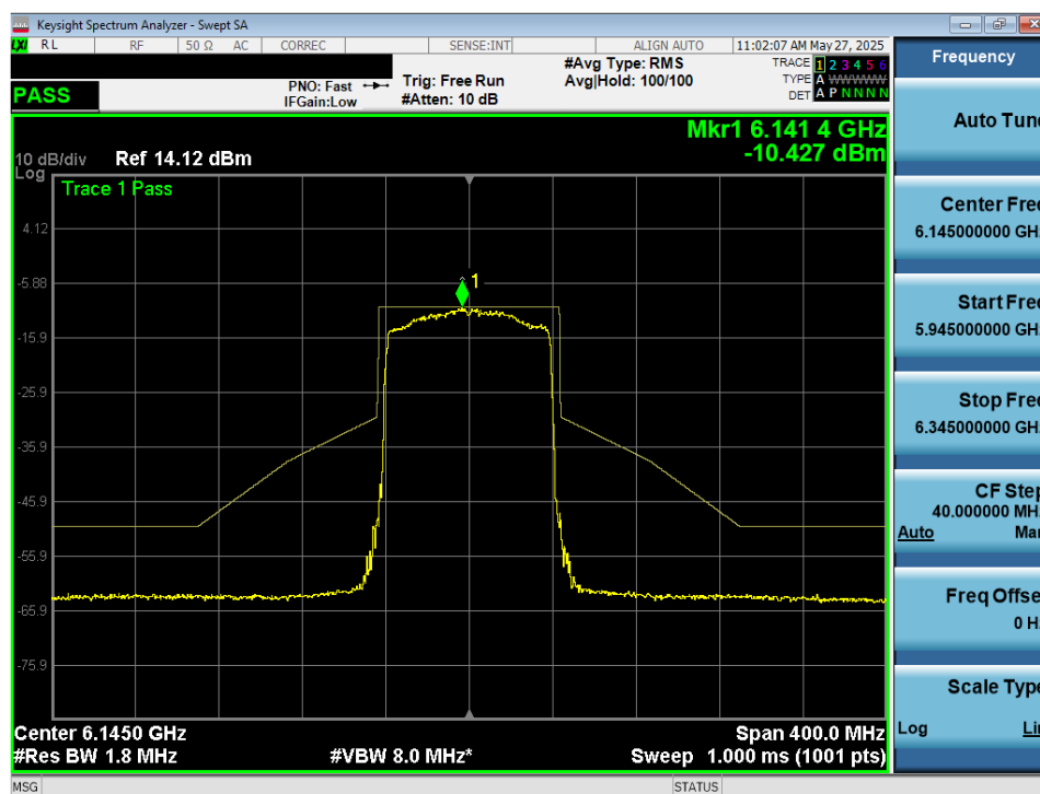
Plot 7-40. In Band Emissions Plot MIMO ANT1 (80MHz 802.11ax/be (UNII Band 5) – Ch. 39) - VLP
