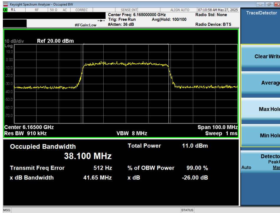
Plot 7-12. 26dB Bandwidth Plot MIMO ANT2 (40MHz 802.11ax/be (UNII Band 5) – Ch. 43) - VLP
