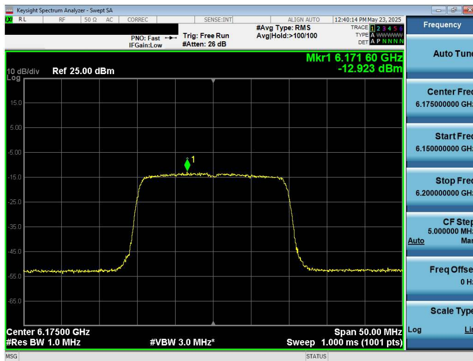
Plot 7-20. Power Spectral Density Plot MIMO ANT1 (20MHz 802.11ax/be (UNII Band 5) – Ch. 45) - VLP
