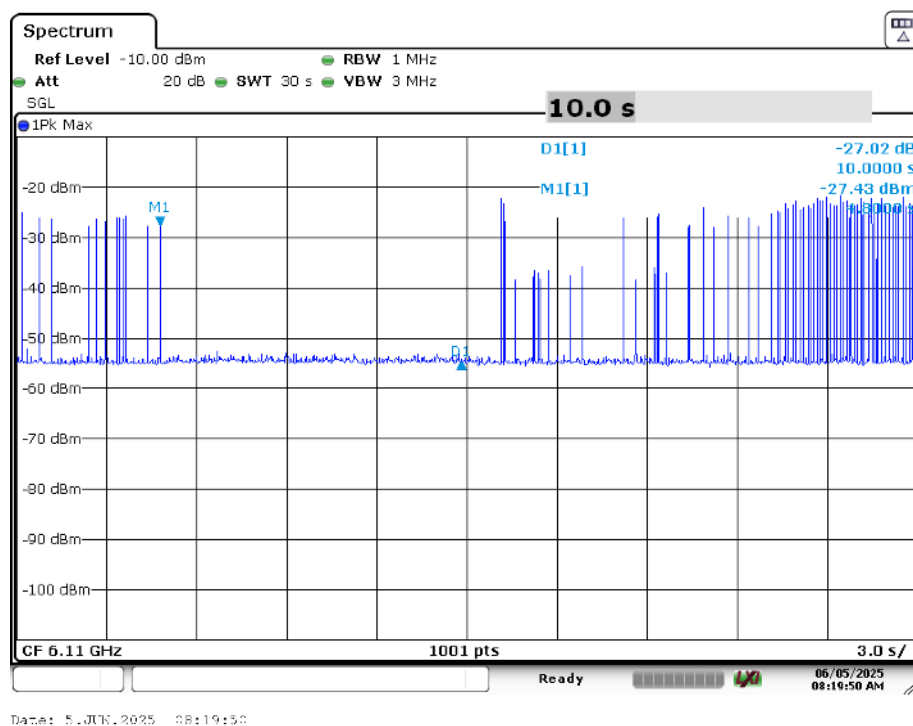
Plot 7-57. Contention Based Protocol Timing Plot (320MHz (UNII Band 5) – Ch. 31 Low)
