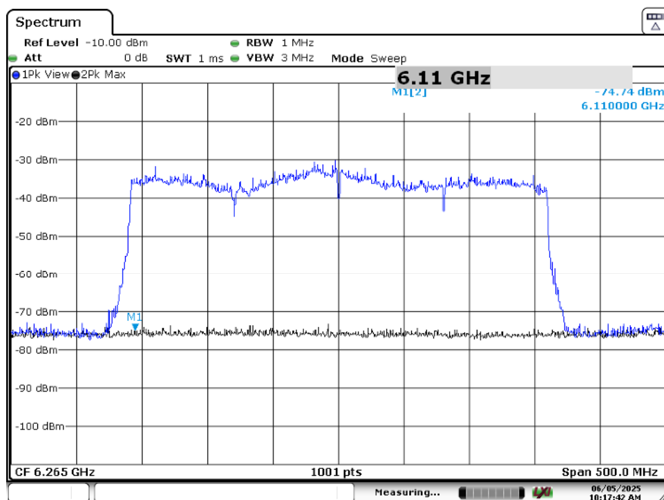
Plot 7-72. CBP 320MHz Channel - Injection Lower Edge – [6110 MHz]
