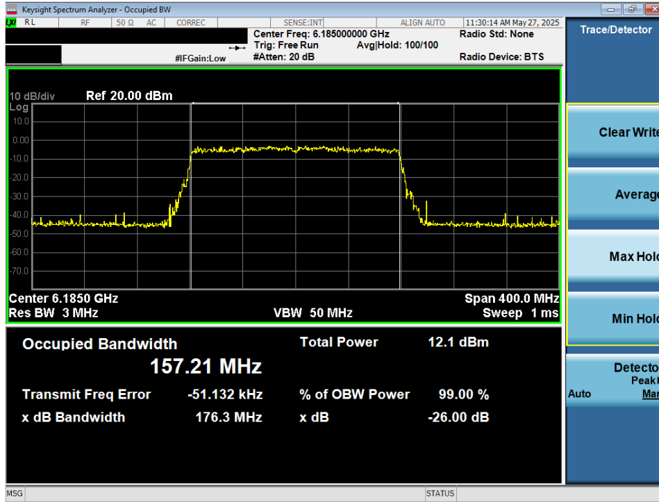
Plot 7-5. 26dB Bandwidth Plot MIMO ANT1 (160MHz 802.11ax/be (UNII Band 5) – Ch. 47) - VLP
