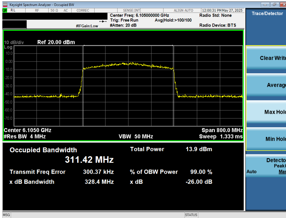
Plot 7-6. 26dB Bandwidth Plot MIMO ANT1 (320MHz 802.11ax/be (UNII Band 5) – Ch. 31) - VLP
