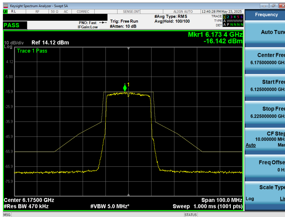
Plot 7-38. In Band Emissions Plot MIMO ANT1 (20MHz 802.11ax/be (UNII Band 5) – Ch. 45) - VLP
