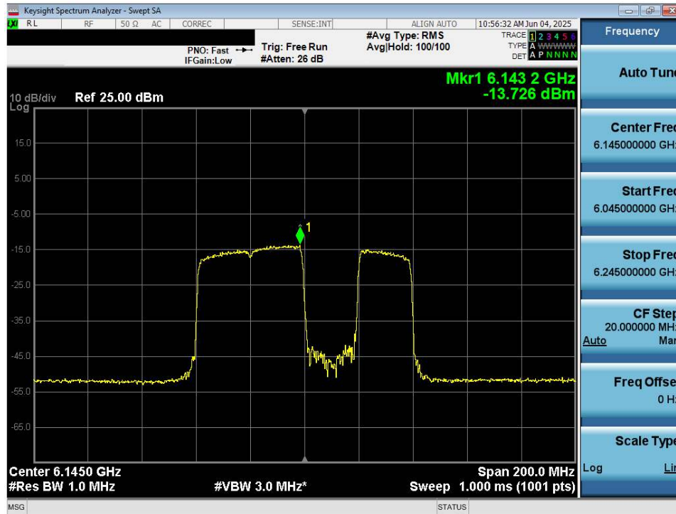
Plot 7-34. Power Spectral Density Plot MIMO ANT2 (80MHz 802.11be (UNII Band 5) – Ch. 39) – 20MHz Punctured - VLP
