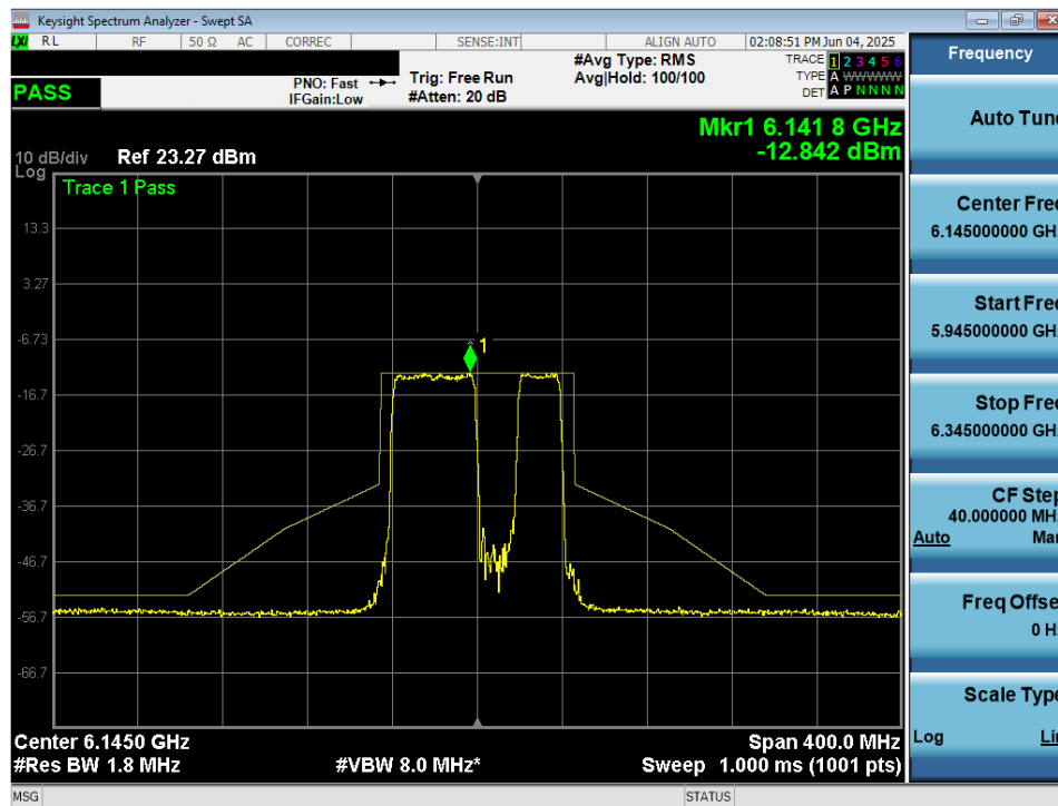
Plot 7-43. In Band Emissions Plot MIMO ANT1 (80MHz 802.11be (UNII Band 5) – Ch. 39) – 20MHz Punctured - VLP
