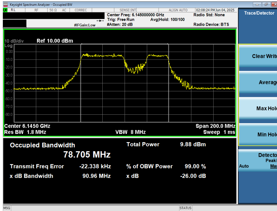
Plot 7-7. 26dB Bandwidth Plot MIMO ANT1 (80MHz 802.11be (UNII Band 5) – Ch. 39) – 20MHz Punctured - VLP
