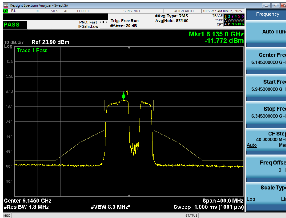
Plot 7-52. In Band Emissions Plot MIMO ANT2 (80MHz 802.11be (UNII Band 5) – Ch. 39) – 20MHz Punctured - VLP
