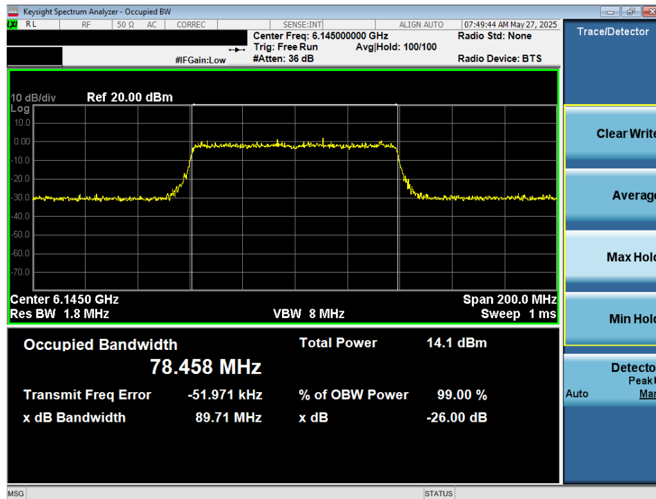
Plot 7-13. 26dB Bandwidth Plot MIMO ANT2 (80MHz 802.11ax/be (UNII Band 5) – Ch. 39) - VLP
