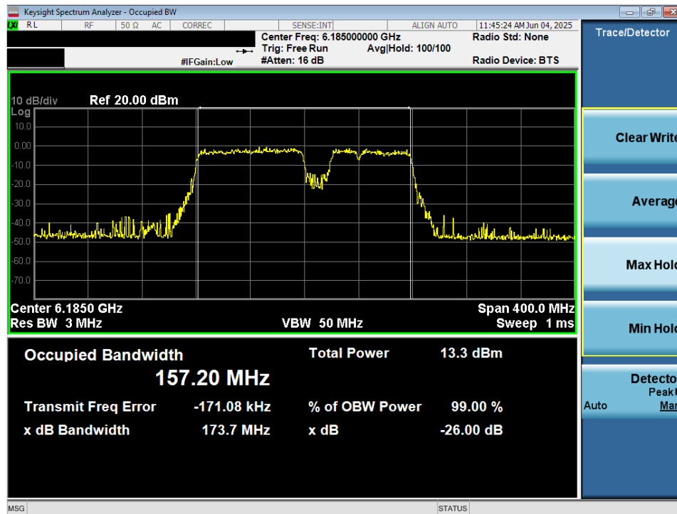
Plot 7-17. 26dB Bandwidth Plot MIMO ANT2 (160MHz 802.11be (UNII Band 5) – Ch. 47) – 20MHz Punctured - VLP
