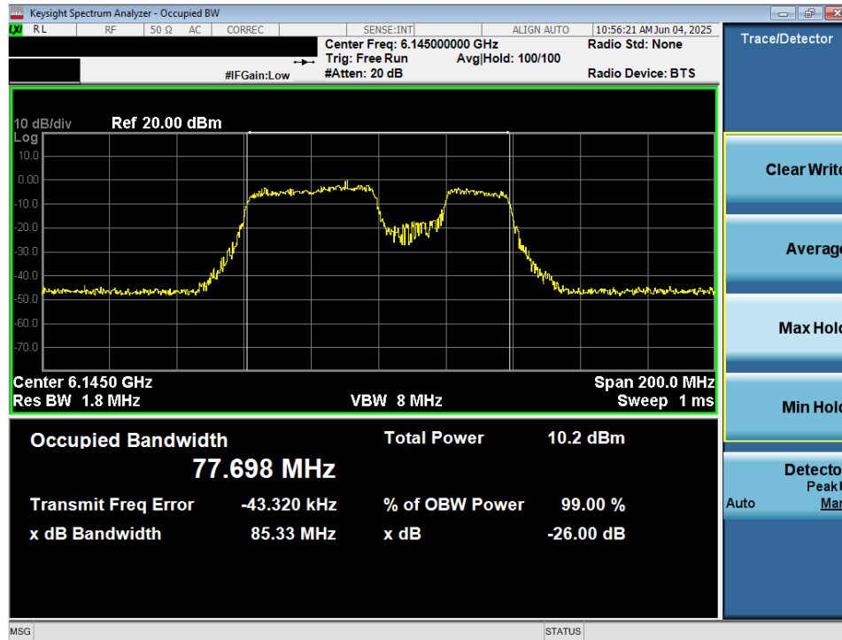
Plot 7-16. 26dB Bandwidth Plot MIMO ANT2 (80MHz 802.11be (UNII Band 5) – Ch. 39) – 20MHz Punctured - VLP
