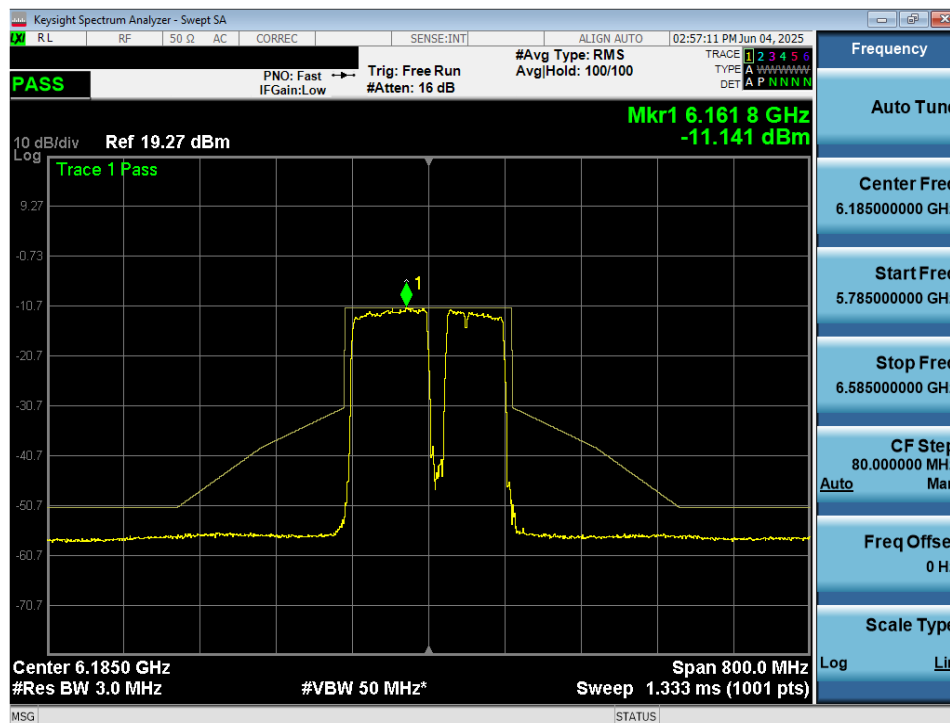
Plot 7-44. In Band Emissions Plot MIMO ANT1 (160MHz 802.11be (UNII Band 5) – Ch. 47) – 20MHz Punctured - VLP
