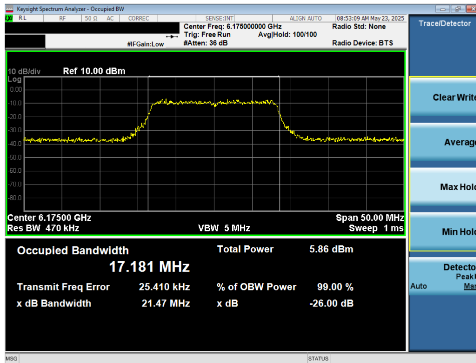
Plot 7-10. 26dB Bandwidth Plot MIMO ANT2 (20MHz 802.11a (UNII Band 5) – Ch. 45) - VLP
