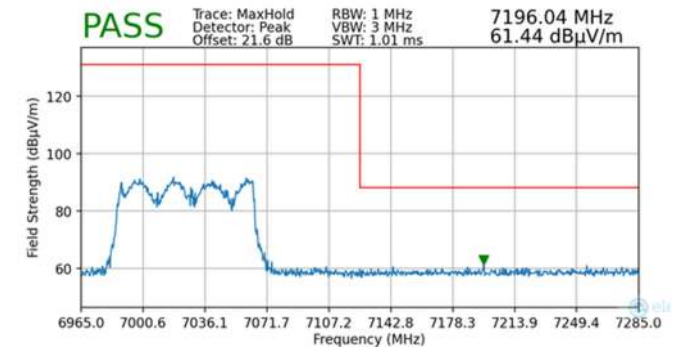
Plot 7-95. Radiated Upper Band Edge Plot MIMO (Peak – UNII Band 8)
