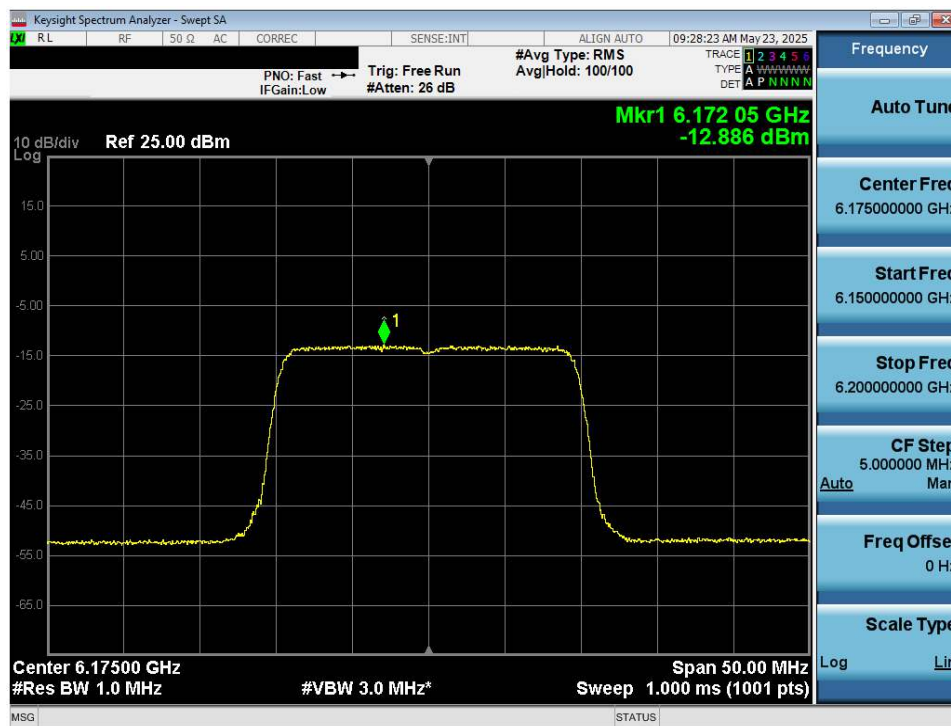
Plot 7-29. Power Spectral Density Plot MIMO ANT2 (20MHz 802.11ax/be (UNII Band 5) – Ch. 45) - VLP
