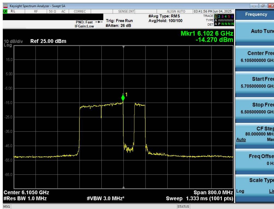
Plot 7-27. Power Spectral Density Plot MIMO ANT1 (320MHz 802.11be (UNII Band 5) – Ch. 31) – 120MHz Punctured - VLP
