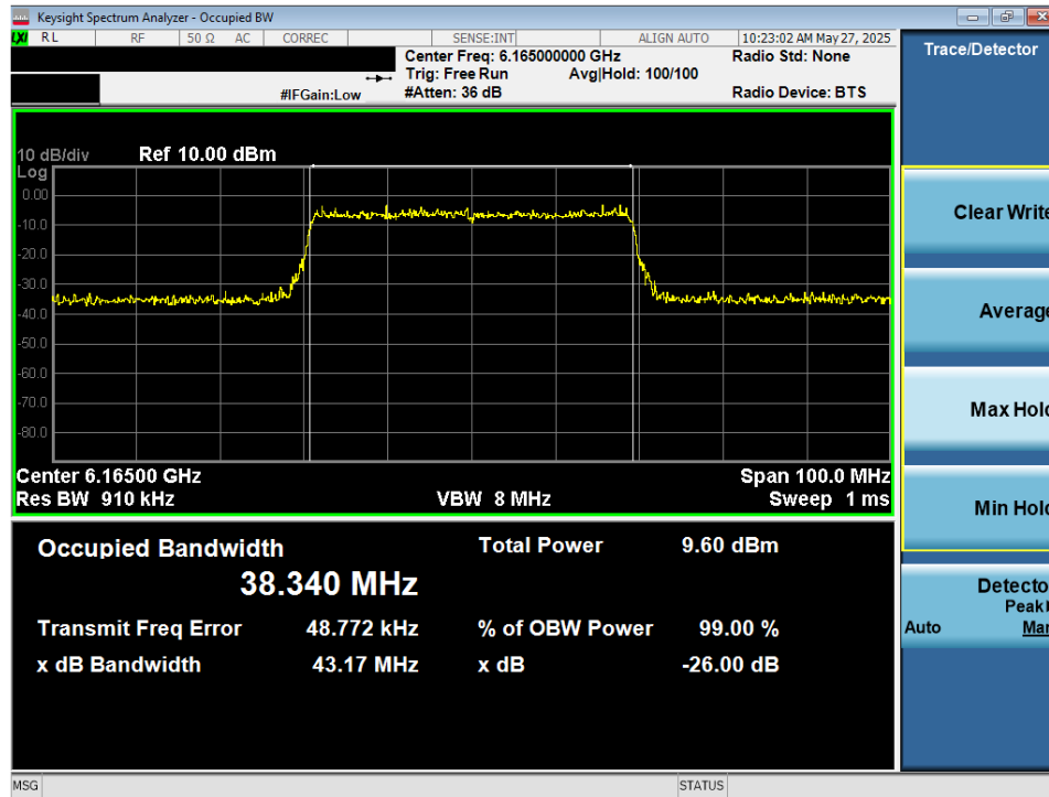
Plot 7-3. 26dB Bandwidth Plot MIMO ANT1 (40MHz 802.11ax/be (UNII Band 5) – Ch. 43) - VLP
