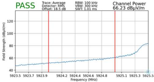
Plot 7-84. Radiated Lower Band Edge Plot MIMO (Average – UNII Band 5)
