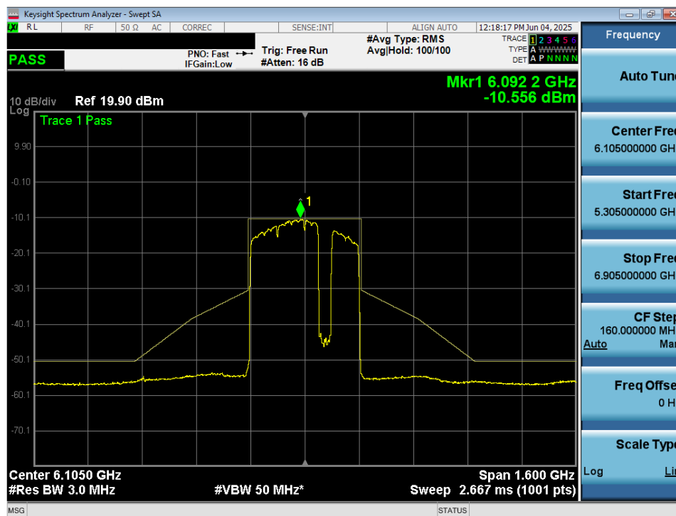
Plot 7-54. In Band Emissions Plot MIMO ANT2 (320MHz 802.11be (UNII Band 5) – Ch. 31) – 40MHz Punctured - VLP
