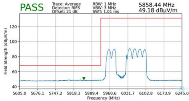
Plot 7-104. Radiated Lower Band Edge Plot MIMO (Average – UNII Band 5)
