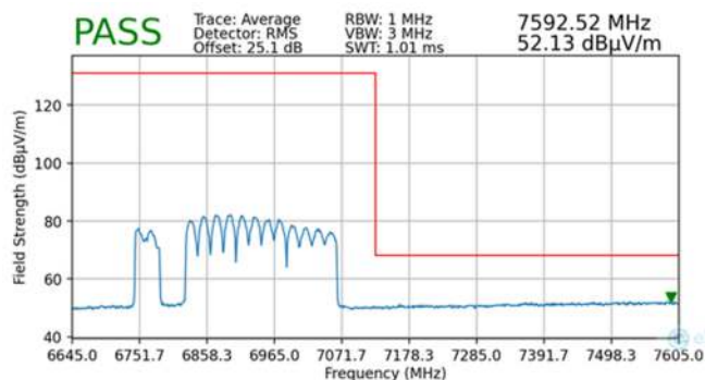
Plot 7-114. Radiated Upper Band Edge Plot MIMO (Average – UNII Band 8)
