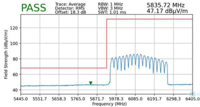
Plot 7-108. Radiated Lower Band Edge Plot MIMO (Average – UNII Band 5)
