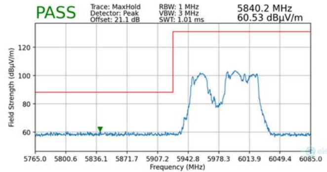
Plot 7-97. Radiated Lower Band Edge Plot MIMO (Peak – UNII Band 5)
