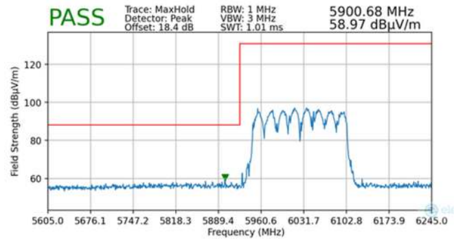
Plot 7-101. Radiated Lower Band Edge Plot MIMO (Peak – UNII Band 5)
