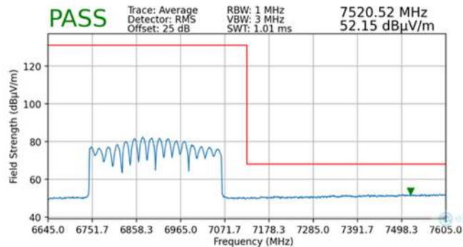
Plot 7-110. Radiated Upper Band Edge Plot MIMO (Average – UNII Band 8)
