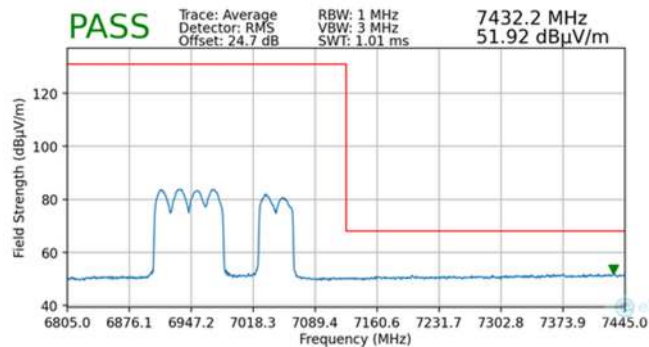
Plot 7-106. Radiated Upper Band Edge Plot MIMO (Average – UNII Band 8)
