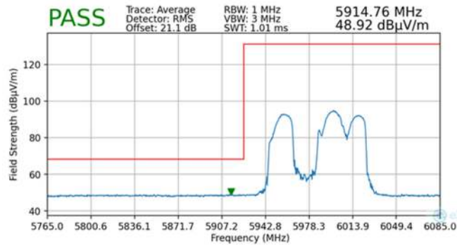
Plot 7-96. Radiated Lower Band Edge Plot MIMO (Average – UNII Band 5)
