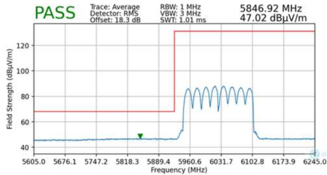
Plot 7-100. Radiated Lower Band Edge Plot MIMO (Average – UNII Band 5)
