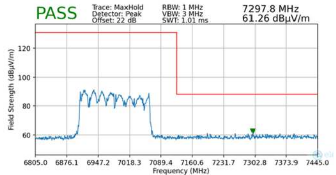
Plot 7-103. Radiated Upper Band Edge Plot MIMO (Peak – UNII Band 8)
