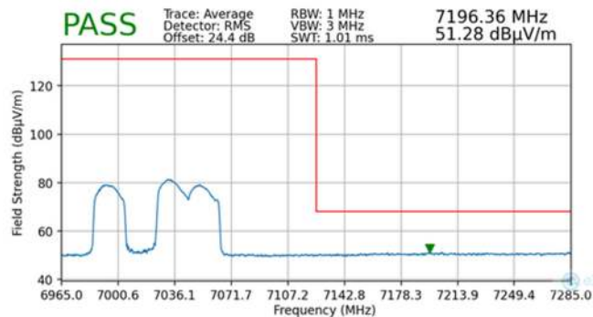
Plot 7-98. Radiated Upper Band Edge Plot MIMO (Average – UNII Band 8)
