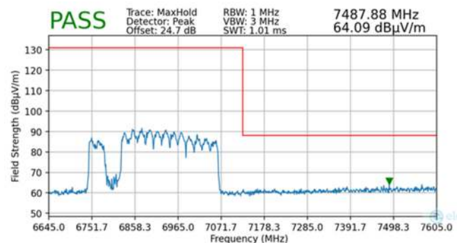
Plot 7-115. Radiated Upper Band Edge Plot MIMO (Peak – UNII Band 8)
