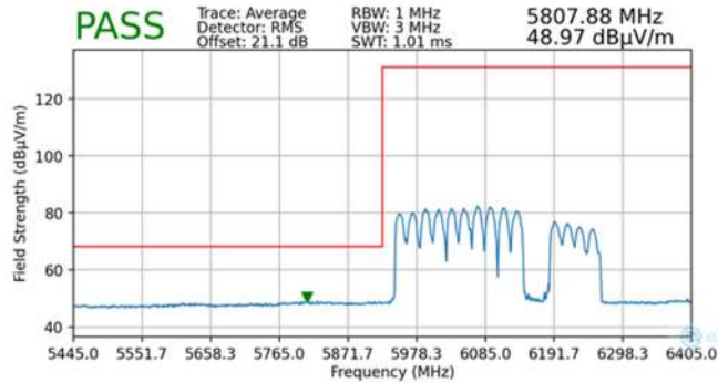
Plot 7-112. Radiated Lower Band Edge Plot MIMO (Average – UNII Band 5)
