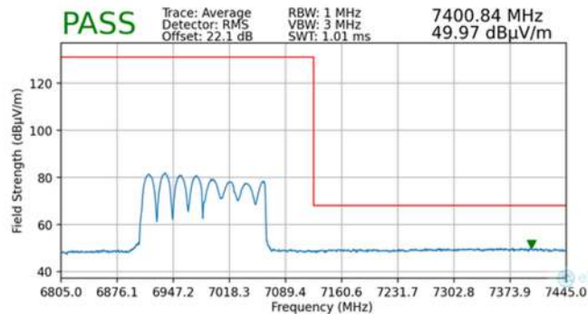
Plot 7-102. Radiated Upper Band Edge Plot MIMO (Average – UNII Band 8)
