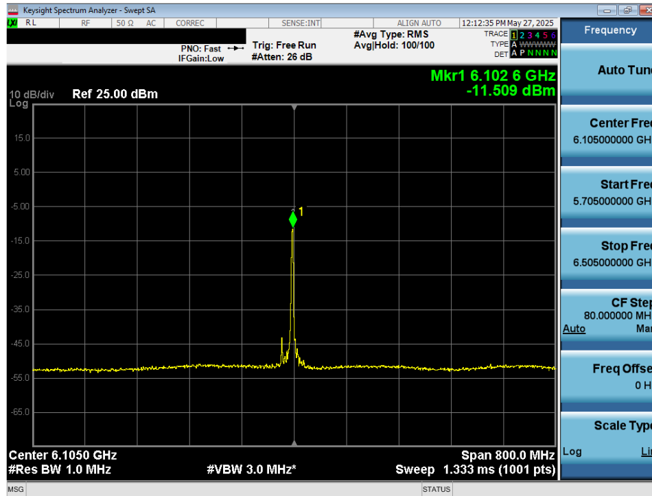
Plot 7-47. Power Spectral Density Plot MIMO ANT2 (320MHz 802.11be (26 Tones) (UNII Band 5) – Ch. 31) - VLP
