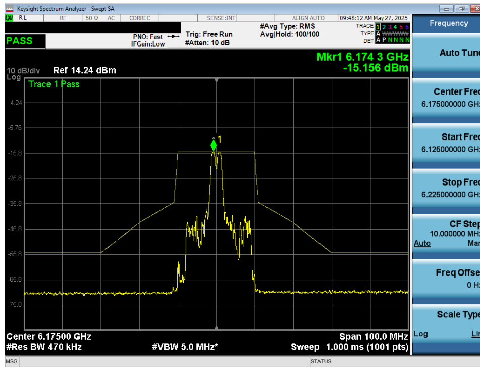
Plot 7-71. In Band Emissions Plot MIMO ANT2 (20MHz 802.11ax/be (26 Tones) (UNII Band 5) – Ch. 45) - VLP
