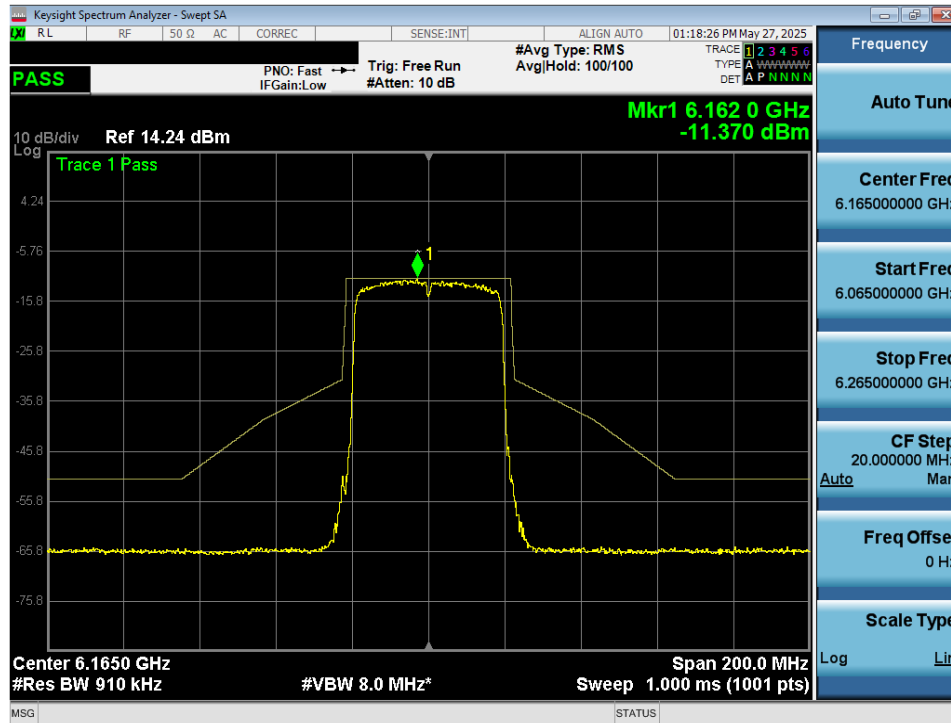
Plot 7-81. In Band Emissions Plot MIMO ANT2 (40MHz 802.11ax/be (Full Tones) (UNII Band 5) – Ch. 43) - VLP
