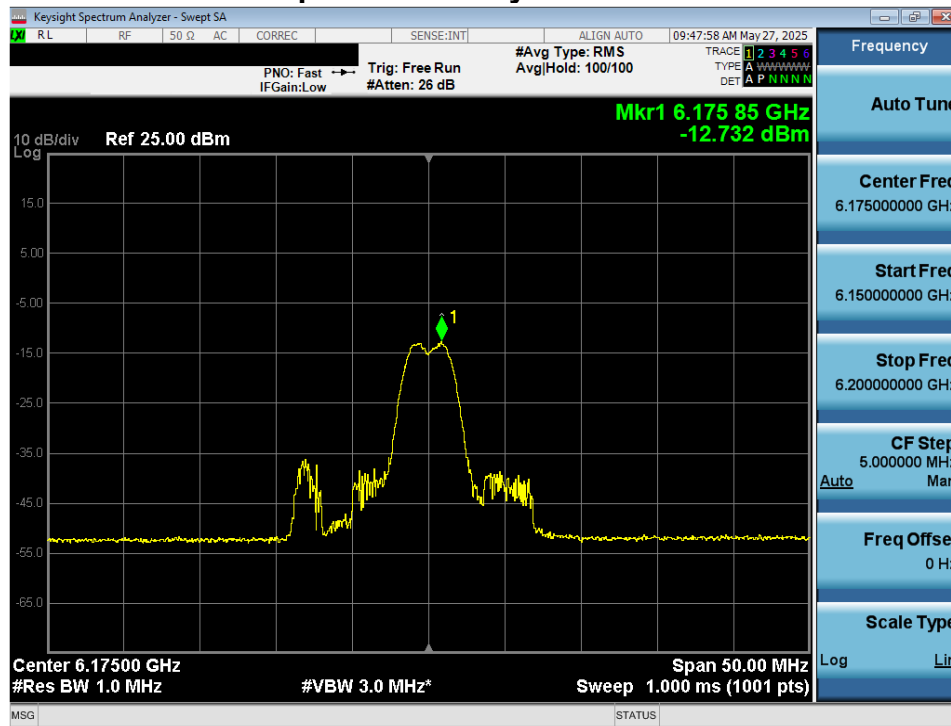
Plot 7-43. Power Spectral Density Plot MIMO ANT2 (20MHz 802.11ax/be (26 Tones) (UNII Band 5) – Ch. 45) - VLP
