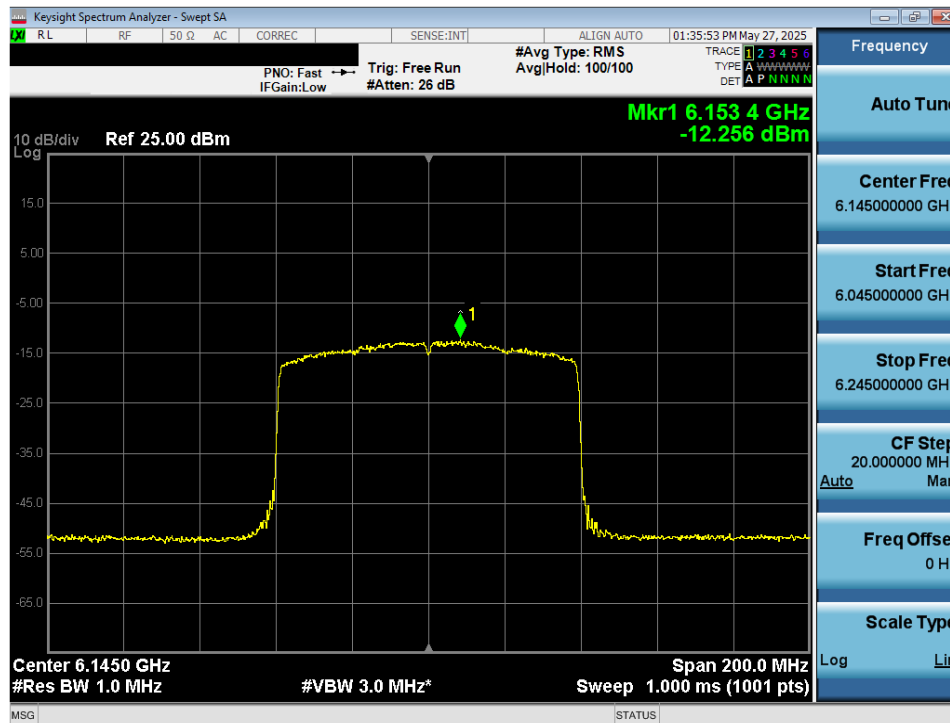
Plot 7-54. Power Spectral Density Plot MIMO ANT2 (80MHz 802.11ax/be (Full Tones) (UNII Band 5) – Ch. 39) - VLP
