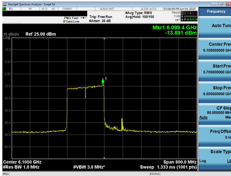
Plot 7-42. Power Spectral Density Plot MIMO ANT1 (320MHz 802.11be (2*996 Tones) (UNII Band 5) – Ch. 31) - VLP
