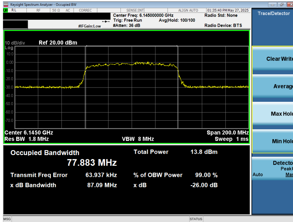
Plot 7-26. 26dB Bandwidth Plot MIMO ANT2 (80MHz 802.11ax/be (Full Tones) (UNII Band 5) – Ch. 39) - VLP
