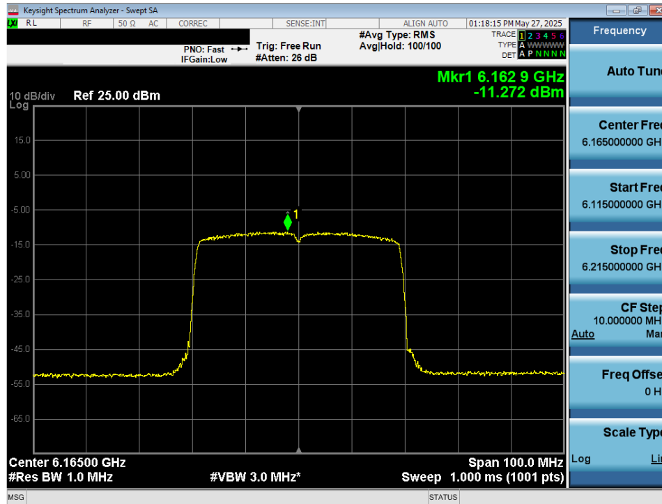
Plot 7-53. Power Spectral Density Plot MIMO ANT2 (40MHz 802.11ax/be (Full Tones) (UNII Band 5) – Ch. 43) - VLP
