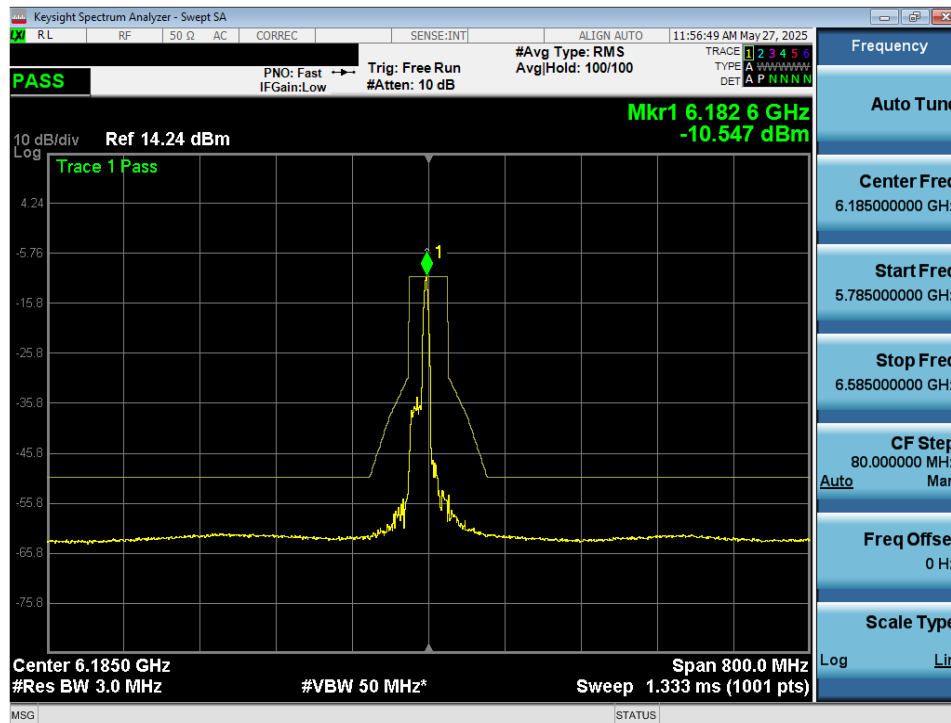
Plot 7-74. In Band Emissions Plot MIMO ANT2 (160MHz 802.11ax/be (26 Tones) (UNII Band 5) – Ch. 47) - VLP
