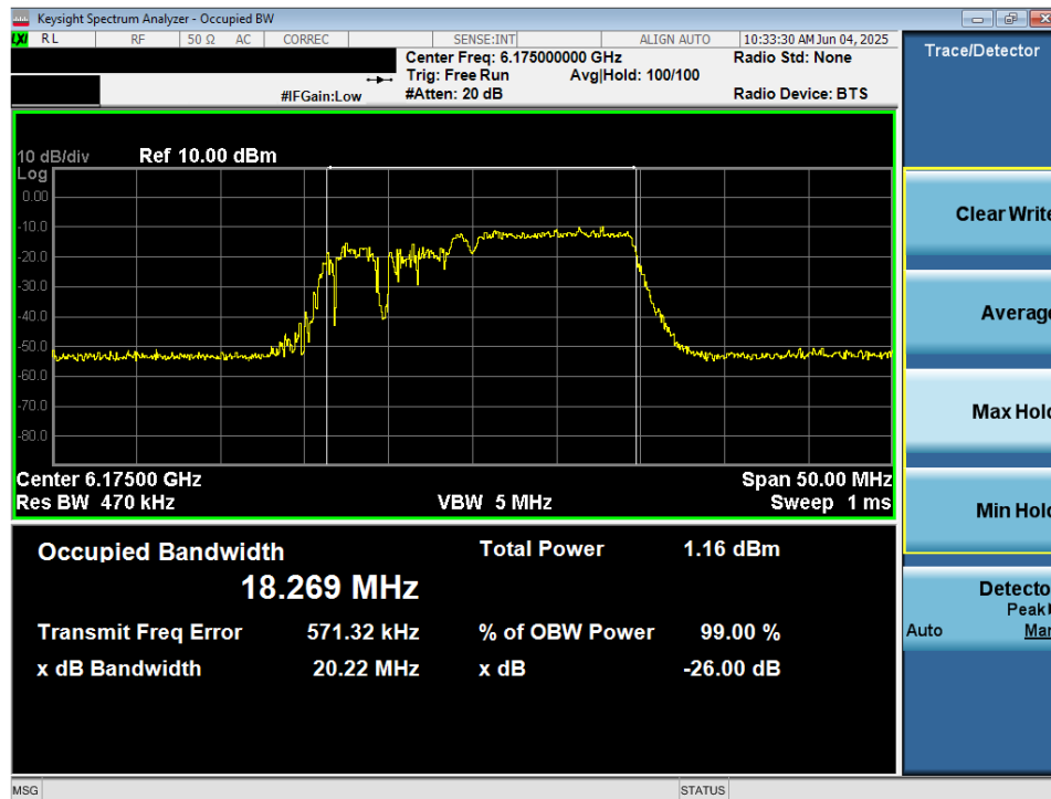
Plot 7-20. 26dB Bandwidth Plot MIMO ANT2 (20MHz 802.11be (106+26 Tones) (UNII Band 5) – Ch. 45) - VLP
