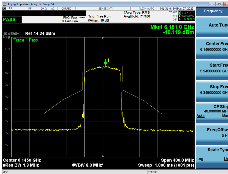
Plot 7-82. In Band Emissions Plot MIMO ANT2 (80MHz 802.11ax/be (Full Tones) (UNII Band 5) – Ch. 39) - VLP
