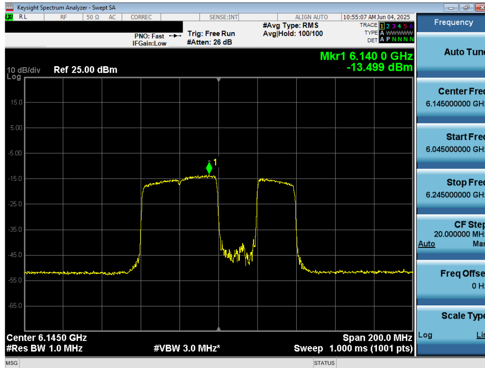
Plot 7-49. Power Spectral Density Plot MIMO ANT2 (80MHz 802.11be (484+242 Tones) (UNII Band 5) – Ch. 39) VLP
