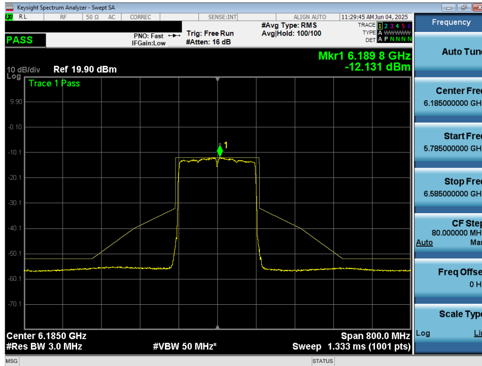
Plot 7-83. In Band Emissions Plot MIMO ANT2 (160MHz 802.11ax/be (Full Tones) (UNII Band 5) – Ch. 47) - VLP
