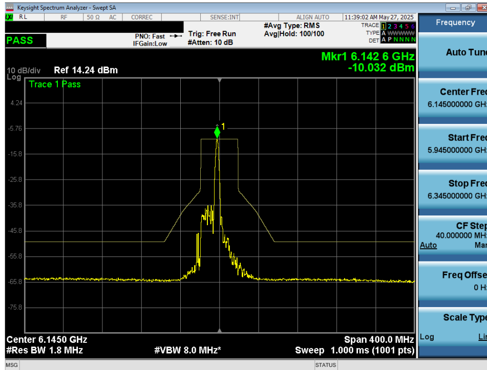
Plot 7-73. In Band Emissions Plot MIMO ANT2 (80MHz 802.11ax/be (26 Tones) (UNII Band 5) – Ch. 39) - VLP
