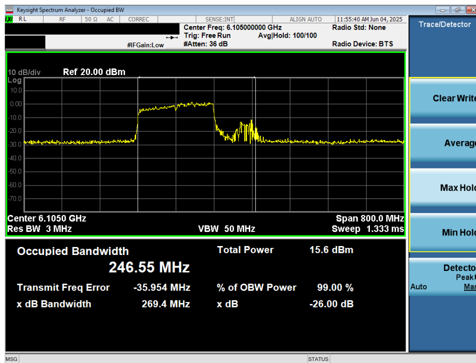
Plot 7-28. 26dB Bandwidth Plot MIMO ANT2 (320MHz 802.11be (2*996 Tones) (UNII Band 5) – Ch. 31) - VLP
