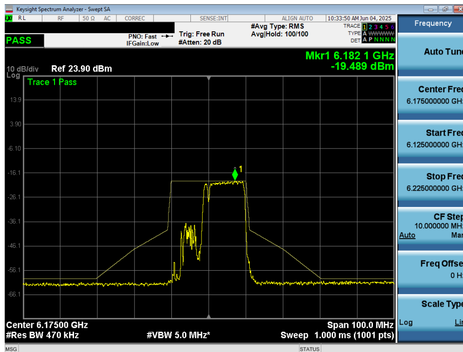
Plot 7-76. In Band Emissions Plot MIMO ANT2 (20MHz 802.11be (106+26 Tones) (UNII Band 5) – Ch. 45) - VLP
