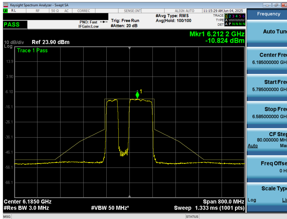
Plot 7-78. In Band Emissions Plot MIMO ANT2 (160MHz 802.11be (996+484 Tones) (UNII Band 5) – Ch. 47) VLP
