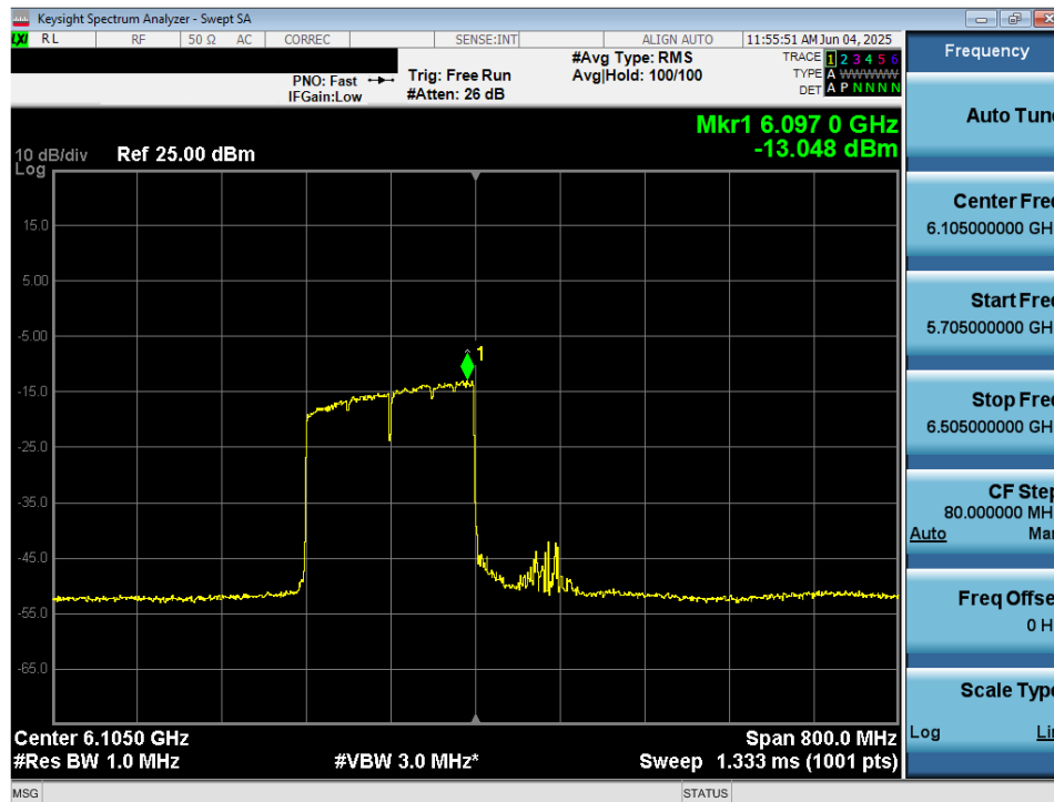
Plot 7-56. Power Spectral Density Plot MIMO ANT2 (320MHz 802.11be (2*996 Tones) (UNII Band 5) – Ch. 31) - VLP
