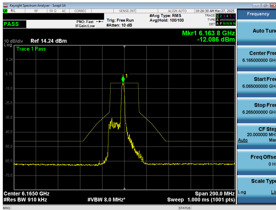
Plot 7-72. In Band Emissions Plot MIMO ANT2 (40MHz 802.11ax/be (26 Tones) (UNII Band 5) – Ch. 43) - VLP
