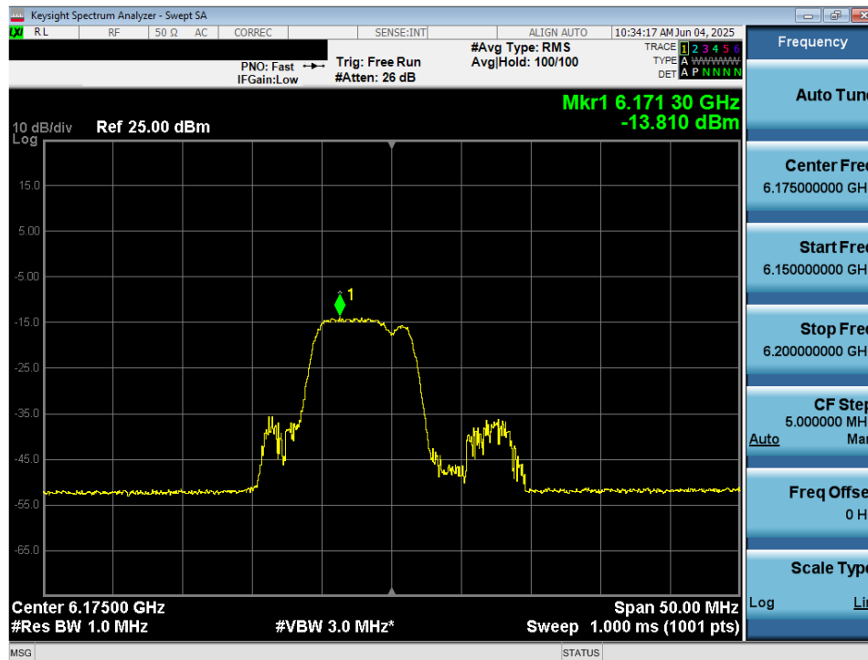
Plot 7-48. Power Spectral Density Plot MIMO ANT2 (20MHz 802.11be (52+26 Tones) (UNII Band 5) – Ch. 45) - VLP
