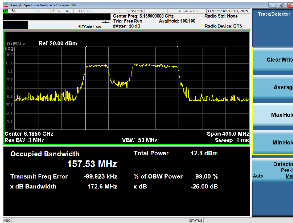
Plot 7-22. 26dB Bandwidth Plot MIMO ANT2 (160MHz 802.11be (996+484 Tones) (UNII Band 5) – Ch. 47) VLP
