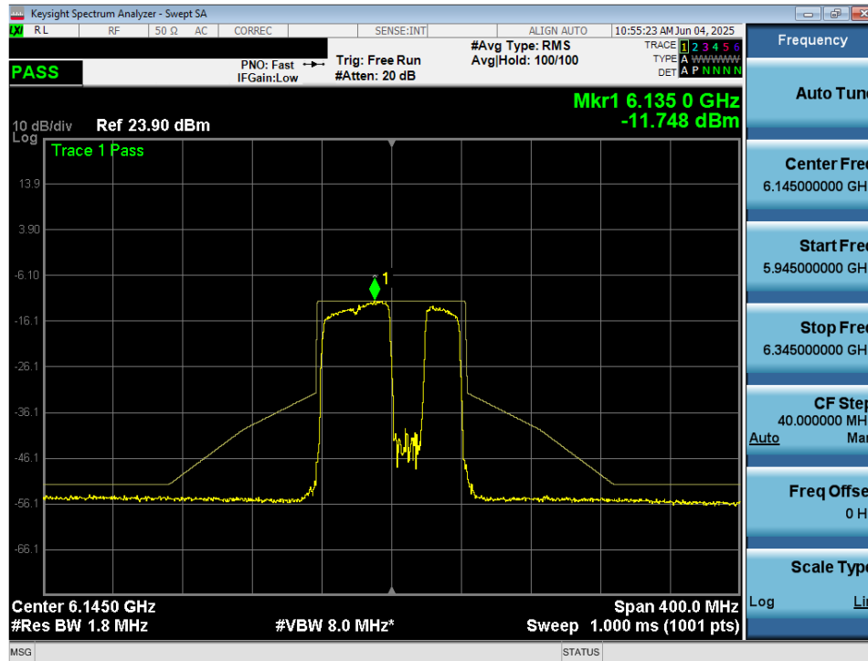
Plot 7-77. In Band Emissions Plot MIMO ANT2 (80MHz 802.11be (484+242 Tones) (UNII Band 5) – Ch. 39) VLP
