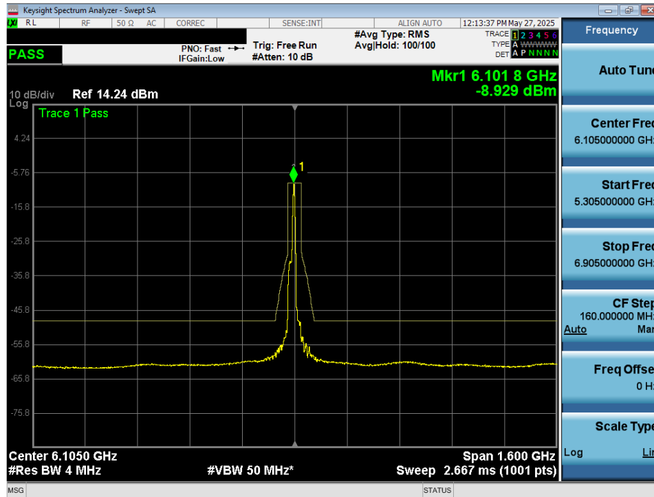
Plot 7-75. In Band Emissions Plot MIMO ANT2 (320MHz 802.11be (26 Tones) (UNII Band 5) – Ch. 31) - VLP
