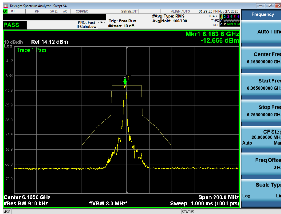
Plot 7-58. In Band Emissions Plot MIMO ANT1 (40MHz 802.11ax/be (26 Tones) (UNII Band 5) – Ch. 43) - VLP
