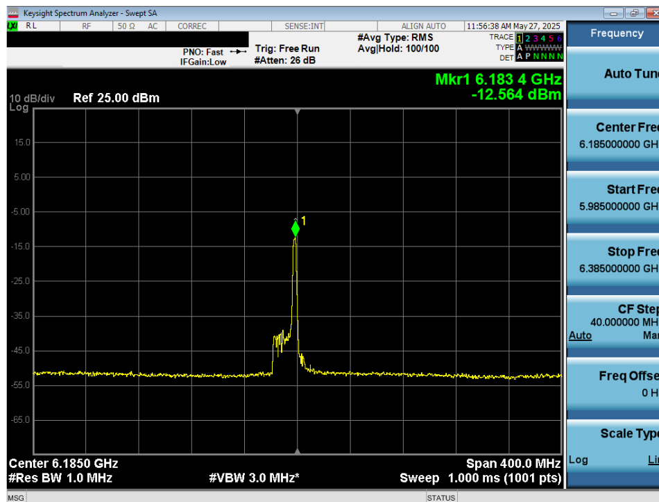
Plot 7-46. Power Spectral Density Plot MIMO ANT2 (160MHz 802.11ax/be (26 Tones) (UNII Band 5) – Ch. 47) - VLP
