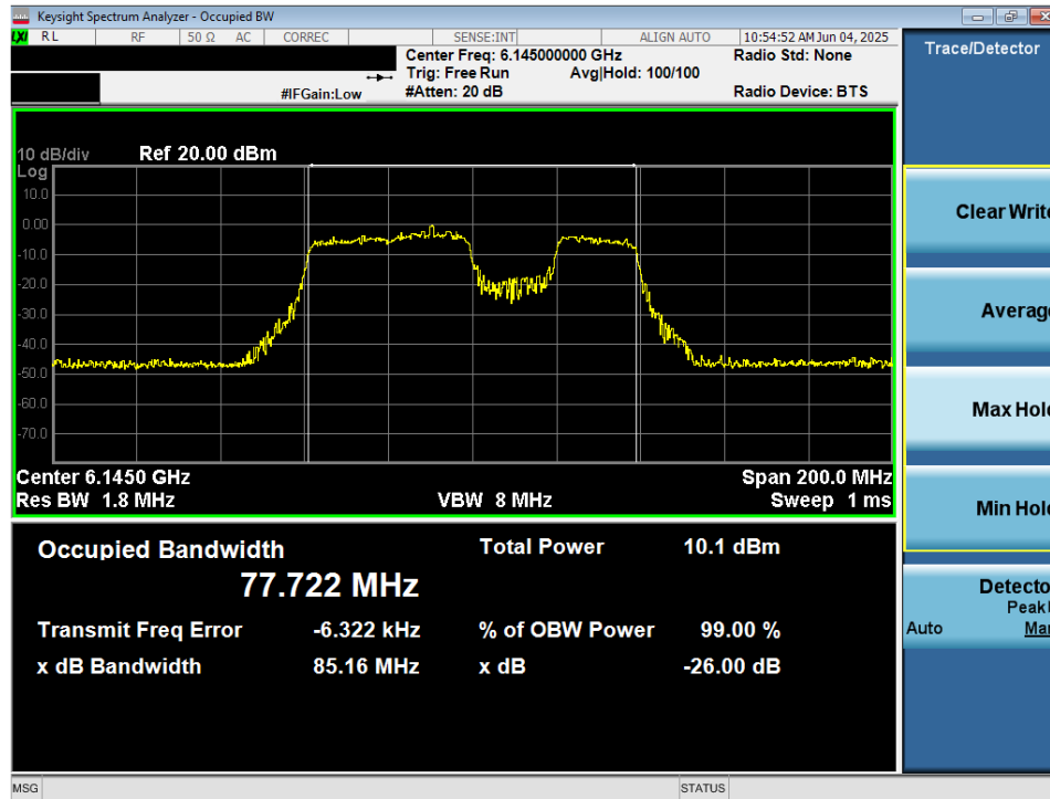
Plot 7-21. 26dB Bandwidth Plot MIMO ANT2 (80MHz 802.11be (484+242 Tones) (UNII Band 5) – Ch. 39) VLP
