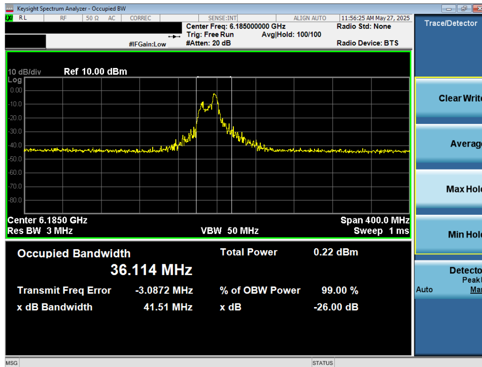
Plot 7-18. 26dB Bandwidth Plot MIMO ANT2 (160MHz 802.11ax/be (26 Tones) (UNII Band 5) – Ch. 47) - VLP
