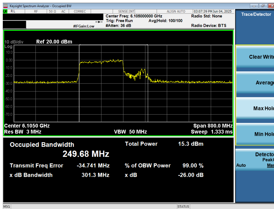
Plot 7-14. 26dB Bandwidth Plot MIMO ANT1 (320MHz 802.11be (2*996 Tones) (UNII Band 5) – Ch. 31) - VLP
