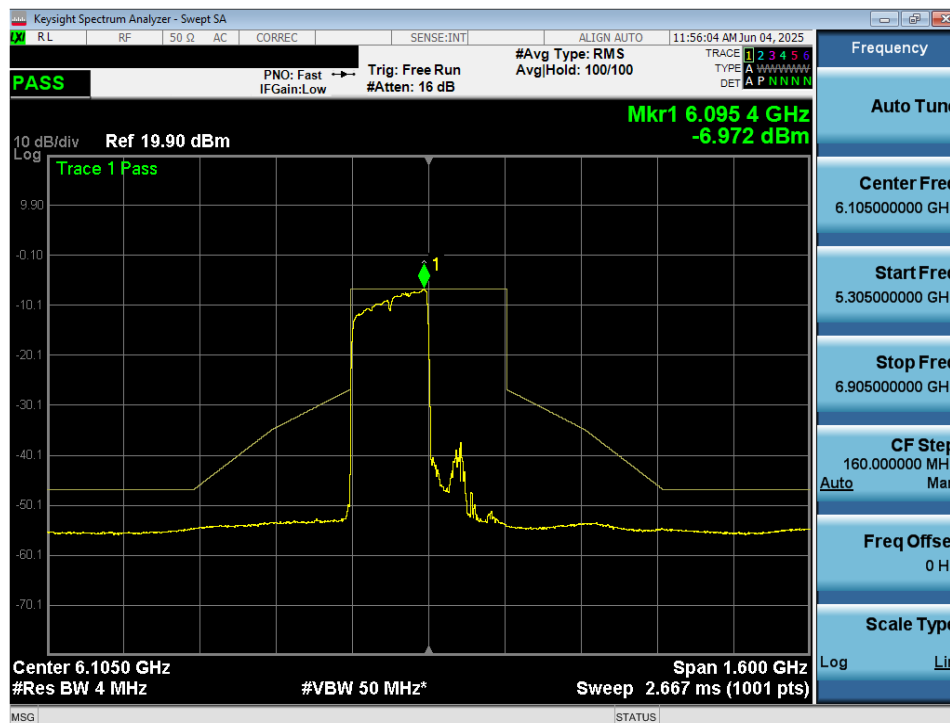
Plot 7-84. In Band Emissions Plot MIMO ANT2 (320MHz 802.11be (Full Tones) (UNII Band 5) – Ch. 31) - VLP
