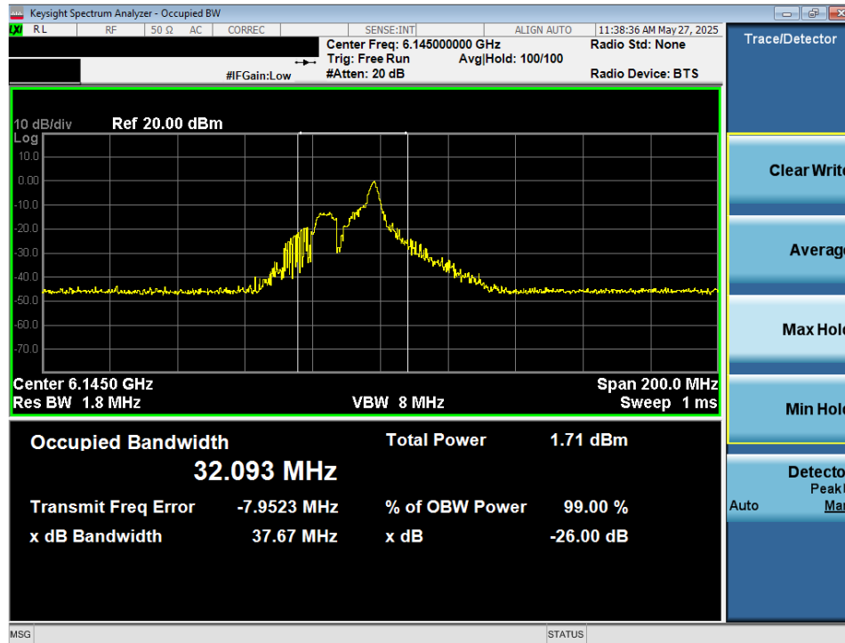
Plot 7-17. 26dB Bandwidth Plot MIMO ANT2 (80MHz 802.11ax/be (26 Tones) (UNII Band 5) – Ch. 39) - VLP
