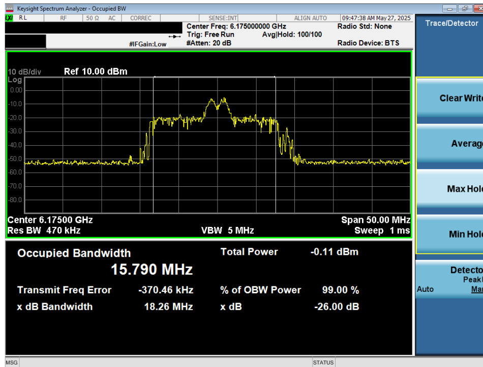
Plot 7-15. 26dB Bandwidth Plot MIMO ANT2 (20MHz 802.11ax/be (26 Tones) (UNII Band 5) – Ch. 45) - VLP
