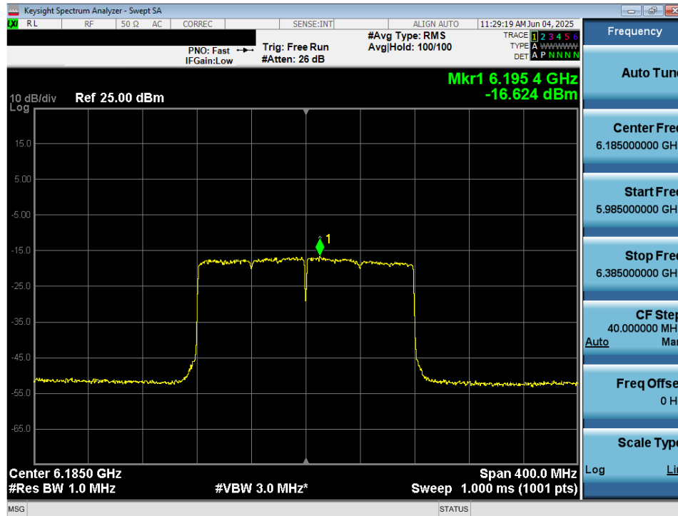
Plot 7-55. Power Spectral Density Plot MIMO ANT2 (160MHz 802.11ax/be (Full Tones) (UNII Band 5) – Ch. 47) - VLP
