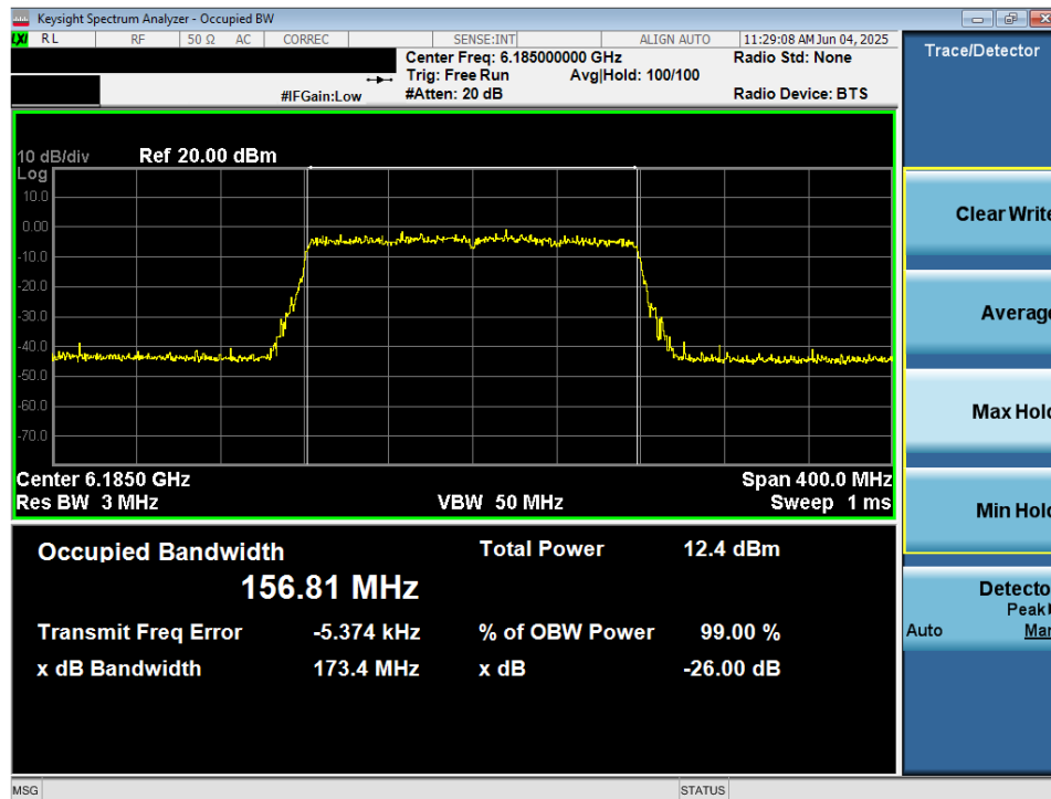
Plot 7-27. 26dB Bandwidth Plot MIMO ANT2 (160MHz 802.11ax/be (Full Tones) (UNII Band 5) – Ch. 47) - VLP
