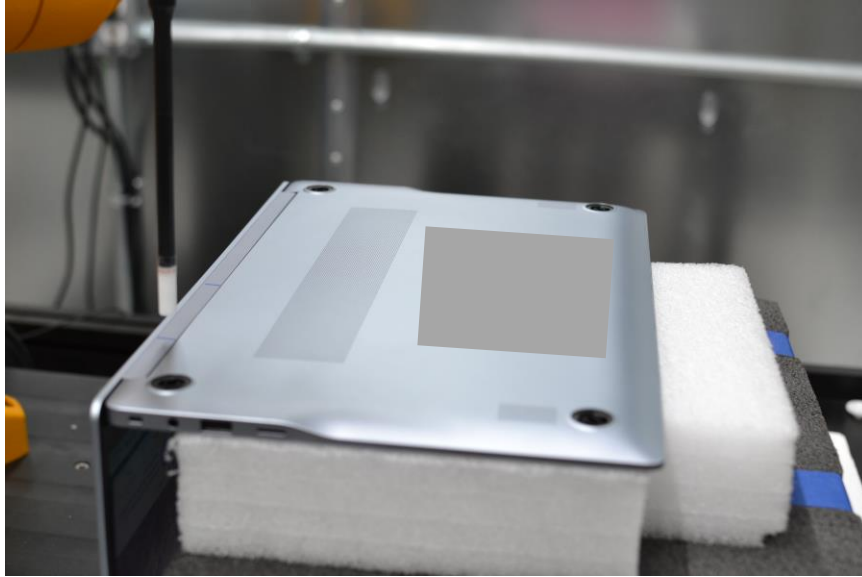
Test Setup Photo 3 - Near Field Power Density, Bottom Edge at 10.02 mm
