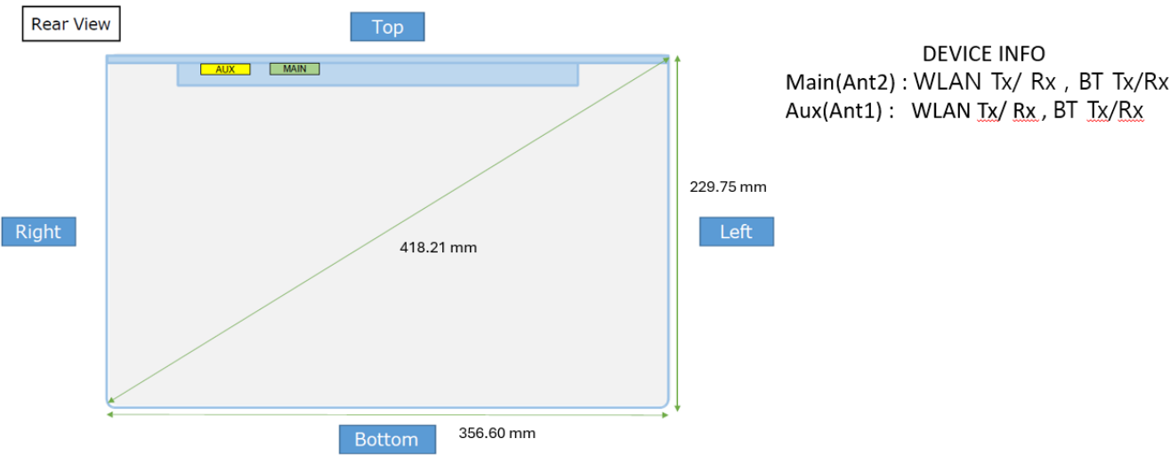
Figure H-1 DUT Antenna Locations
