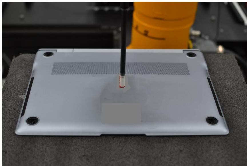
Near Field Power Density Test Setup Photo 2 – Bottom Edge at 2 mm
