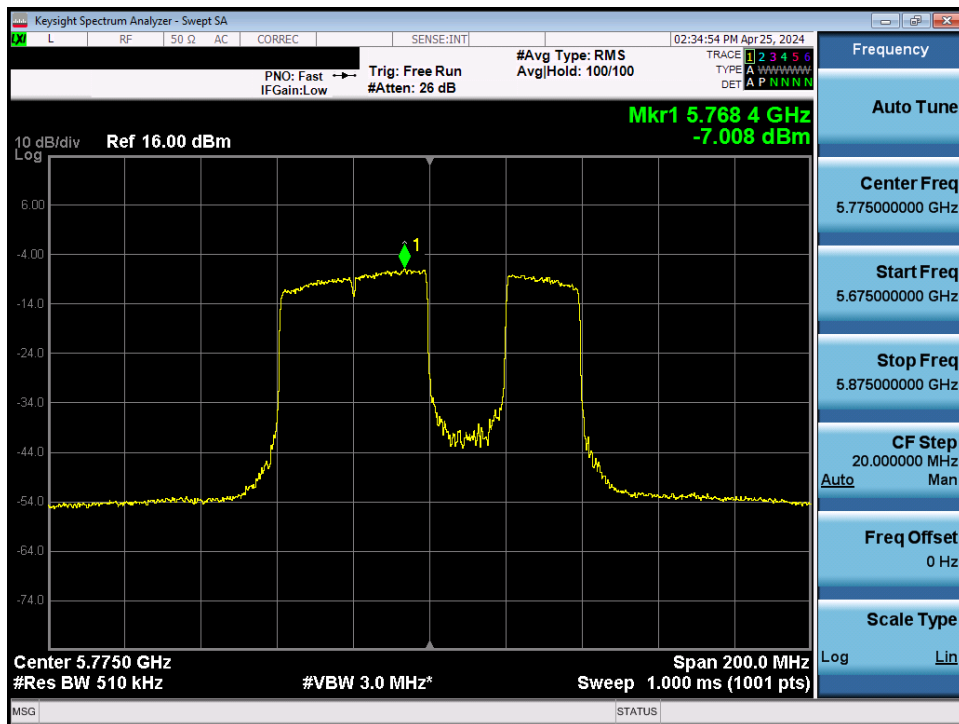
Plot 7-180. Power Spectral Density Plot MIMO ANT2 (80MHz BW 802.11be (UNII Band 3) – Ch. 155)
