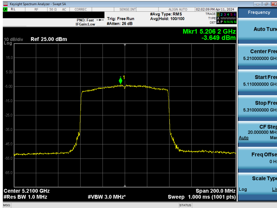
Plot 7-132. Power Spectral Density Plot MIMO ANT2 (80MHz BW 802.11ax/be (UNII Band 1) – Ch. 42)
