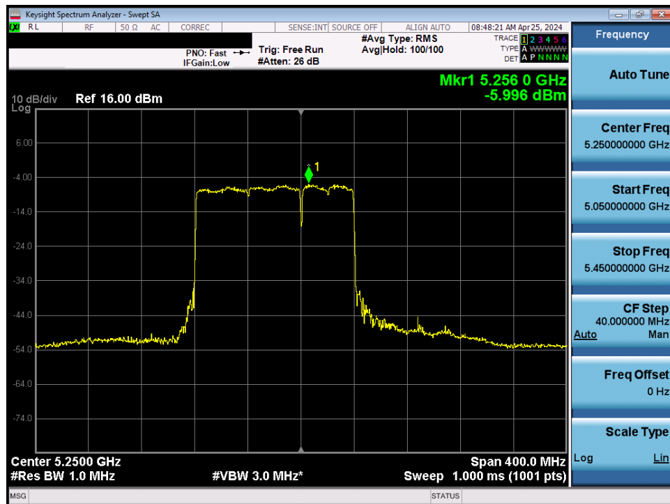
Plot 7-168. Power Spectral Density Plot MIMO ANT1 (160MHz BW 802.11be (UNII Band 1/2A) – Ch. 50)
