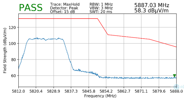
Plot 7-197. Radiated Upper Band Edge Plot MIMO (Peak – UNII Band 3)
