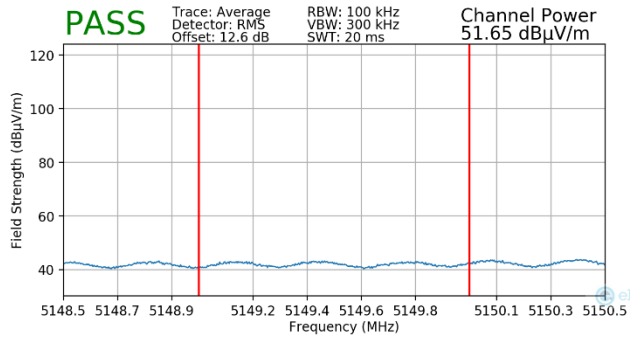
Plot 7-201. Radiated Lower Band Edge Plot MIMO (Average – UNII Band 1)
