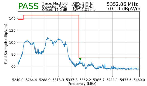
Plot 7-214. Radiated Upper Band Edge Plot MIMO (Peak – UNII Band 2A)
