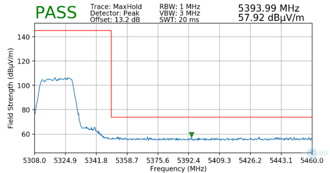
Plot 7-194. Radiated Upper Band Edge Plot MIMO (Peak – UNII Band 2A)
