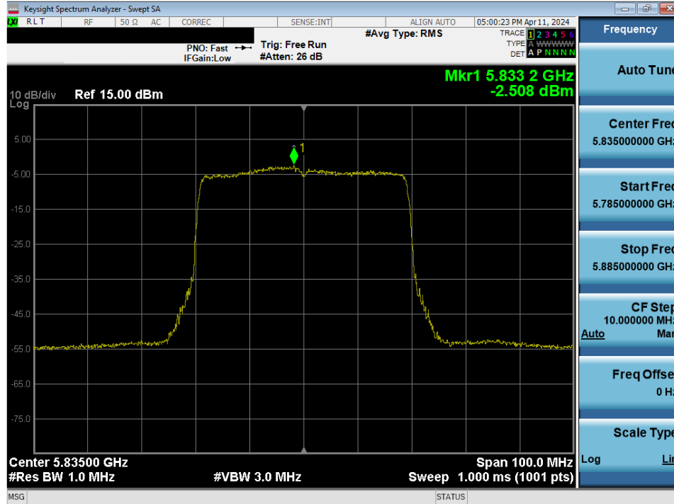
Plot 7-121. Power Spectral Density Plot MIMO ANT1 (40MHz BW 802.11ax/be (UNII Band 3/4) – Ch. 167)
