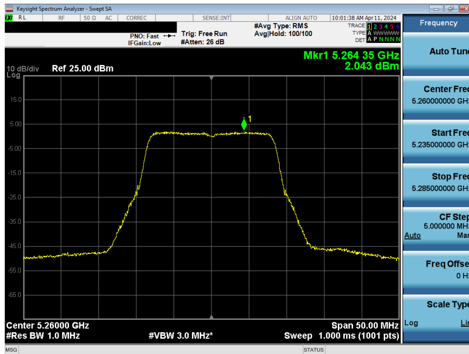
Plot 7-135. Power Spectral Density Plot MIMO ANT2 (802.11a (UNII Band 2A) – Ch. 52)
