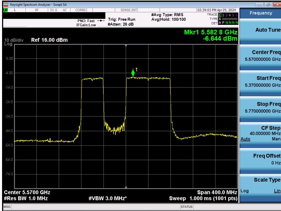
Plot 7-179. Power Spectral Density Plot MIMO ANT2 (160MHz BW 802.11be (UNII Band 2C) – Ch. 114)
