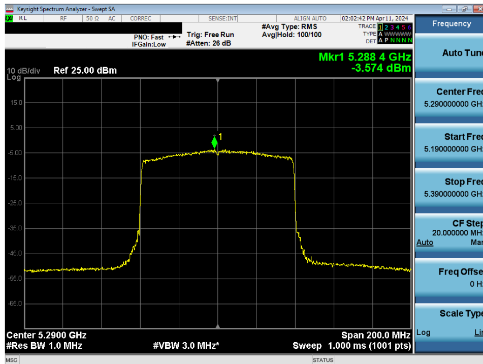
Plot 7-141. Power Spectral Density Plot MIMO ANT2 (80MHz BW 802.11ax/be (UNII Band 2A) – Ch. 58)
