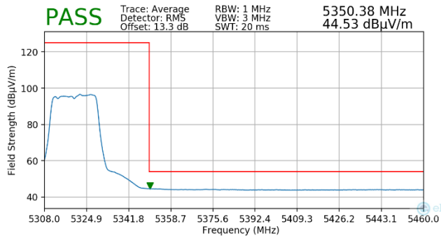
Plot 7-193. Radiated Upper Band Edge Plot MIMO (Average – UNII Band 2A)
