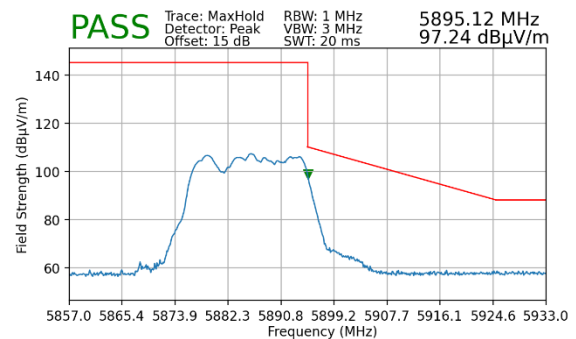
Plot 7-200. Radiated Upper Band Edge Plot MIMO (Peak – UNII Band 4)
