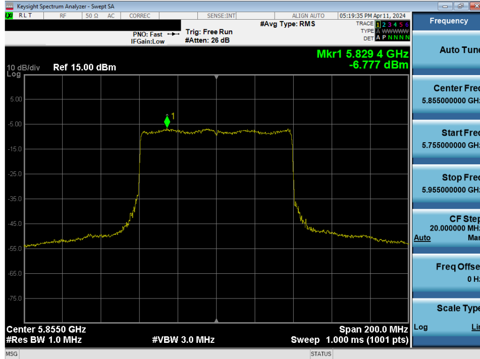
Plot 7-123. Power Spectral Density Plot MIMO ANT1 (80MHz BW 802.11ax/be (UNII Band 3/4) – Ch. 171)
