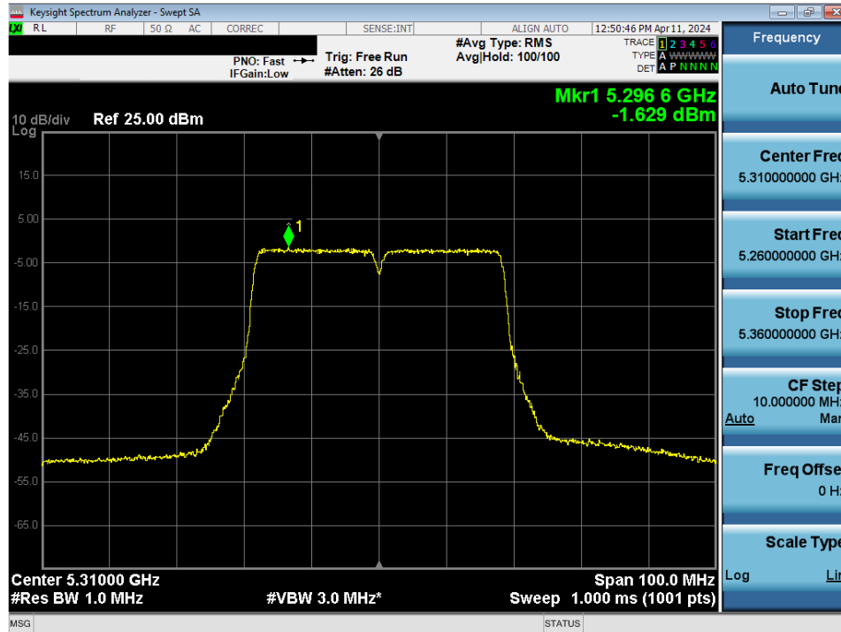
Plot 7-138. Power Spectral Density Plot MIMO ANT2 (40MHz BW 802.11n (UNII Band 2A) – Ch. 62)
