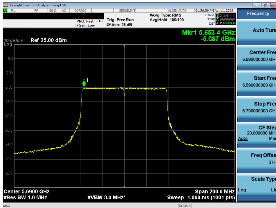
Plot 7-147. Power Spectral Density Plot MIMO ANT2 (80MHz BW 802.11ac (UNII Band 2C) – Ch. 138)
