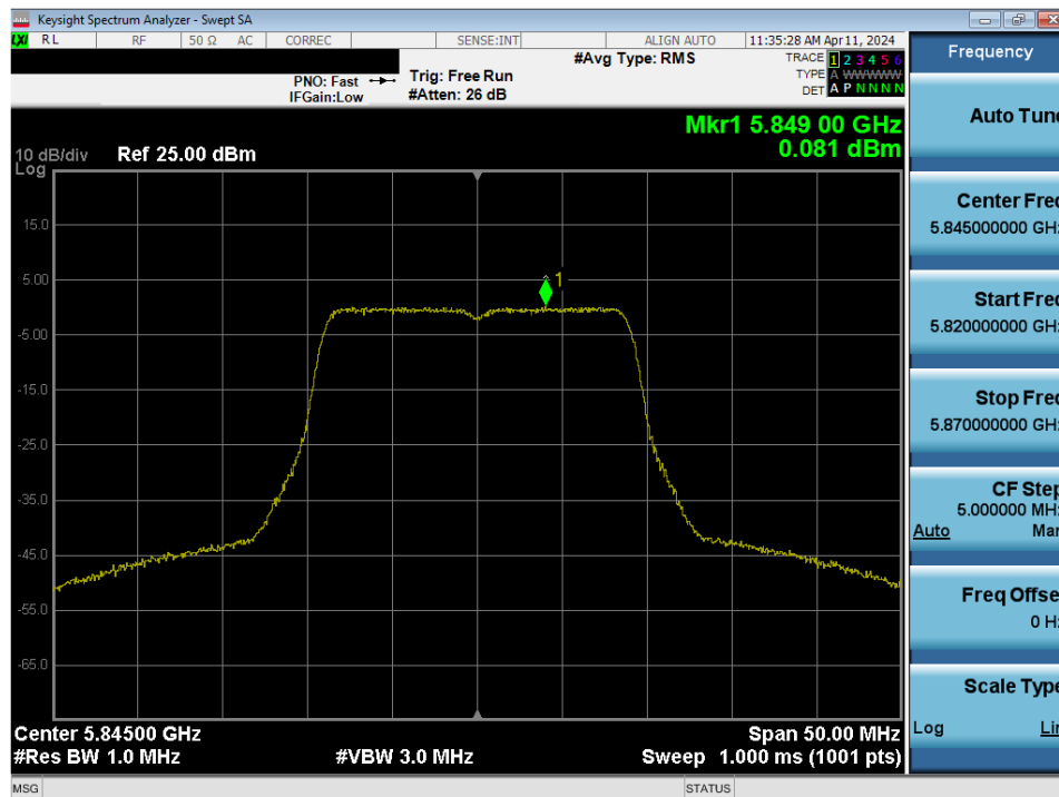
Plot 7-159. Power Spectral Density Plot MIMO ANT2 (20MHz BW 802.11n (UNII Band 3/4) – Ch. 169)
