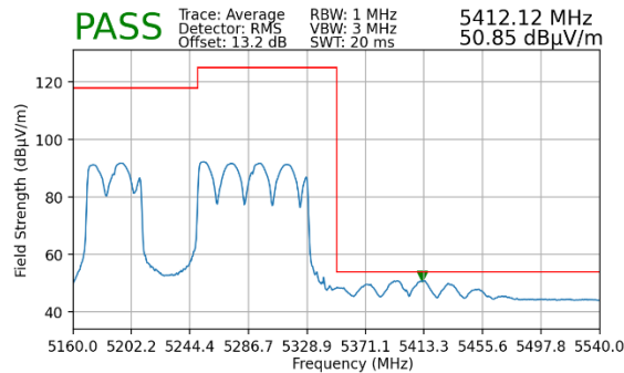
Plot 7-223. Radiated Upper Band Edge Plot MIMO (Average – UNII Band 2A)
