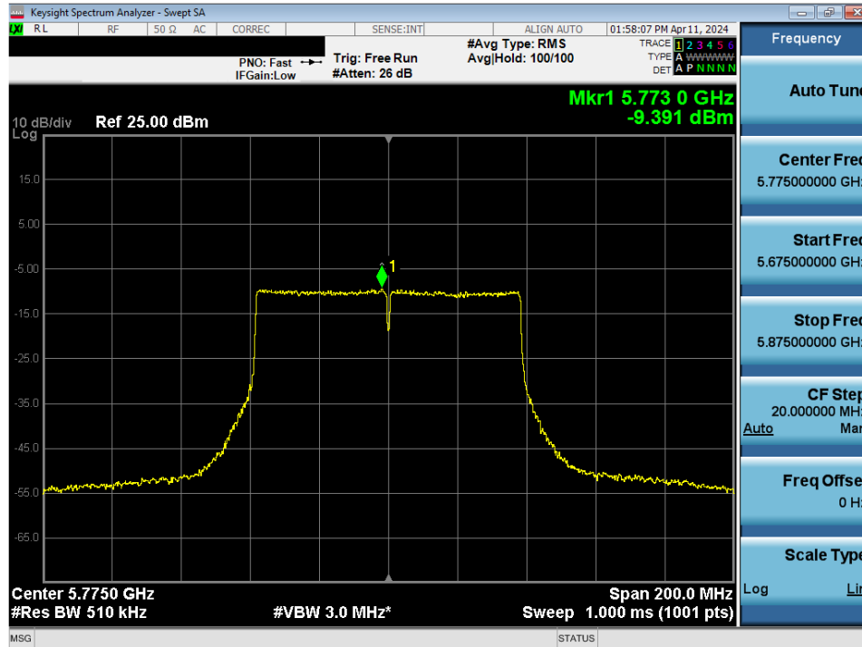
Plot 7-156. Power Spectral Density Plot MIMO ANT2 (80MHz BW 802.11ac (UNII Band 3) – Ch. 155)
