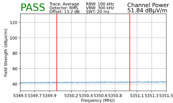
Plot 7-213. Radiated Upper Band Edge Plot MIMO (Average – UNII Band 2A)
