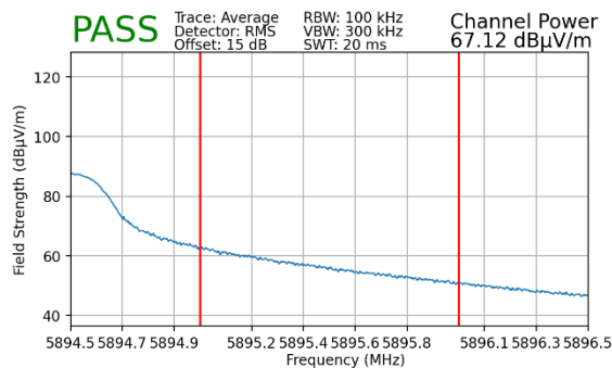
Plot 7-199. Radiated Upper Band Edge Plot MIMO (Average – UNII Band 4)
