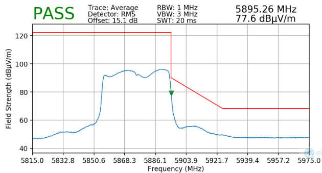
Plot 7-209. Radiated Upper Band Edge Plot MIMO (Average – UNII Band 4)
