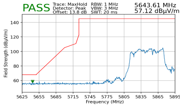
Plot 7-208. Radiated Lower Band Edge Plot MIMO (Peak – UNII Band 4)
