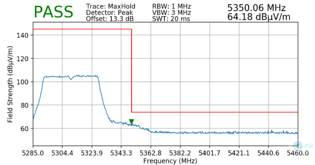
Plot 7-204. Radiated Upper Band Edge Plot MIMO (Peak – UNII Band 2A)
