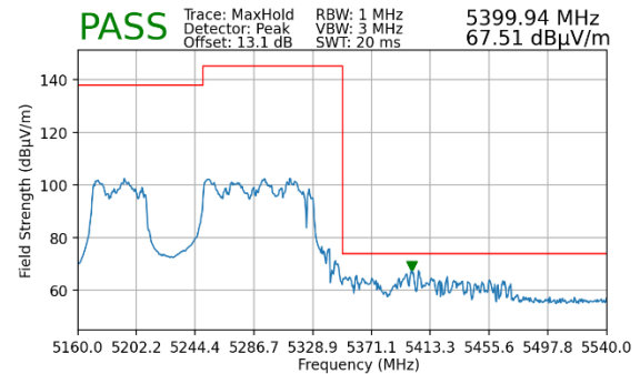
Plot 7-224. Radiated Upper Band Edge Plot MIMO (Peak – UNII Band 2A)
