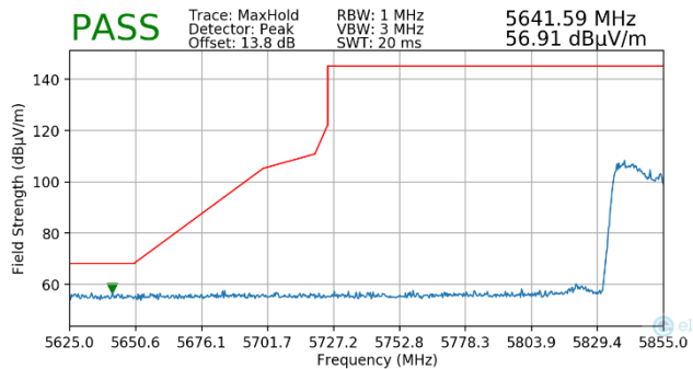
Plot 7-198. Radiated Lower Band Edge Plot MIMO (Peak – UNII Band 4)
