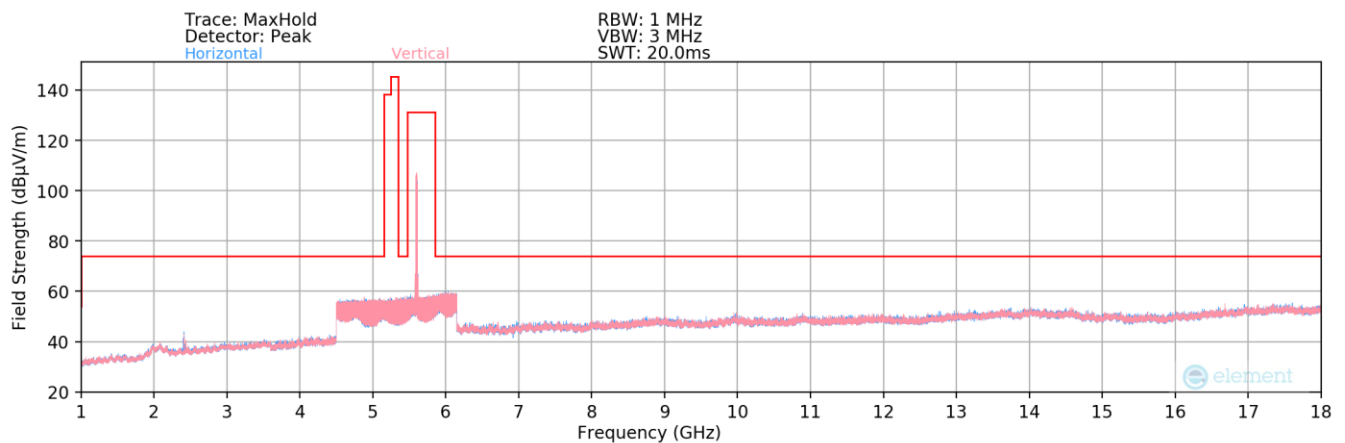
Plot 7-186. Radiated Spurious Plot above 1GHz MIMO (802.11a – UNII Band 2C Ch. 120)
