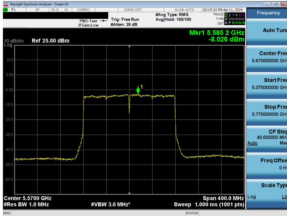
Plot 7-150. Power Spectral Density Plot MIMO ANT2 (160MHz BW 802.11ax/be (UNII Band 2C) – Ch. 114)
