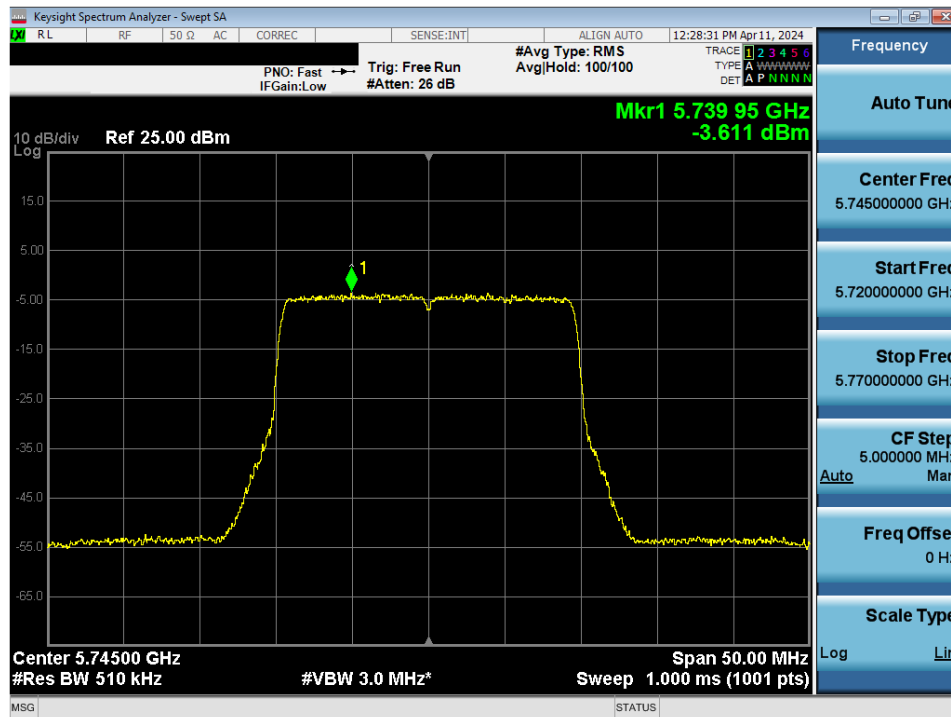
Plot 7-153. Power Spectral Density Plot MIMO ANT2 (20MHz BW 802.11ax/be (UNII Band 3) – Ch. 149)
