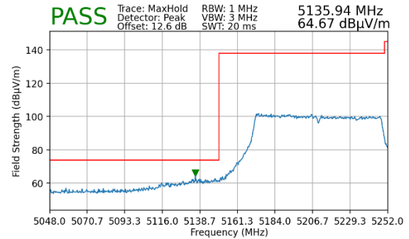
Plot 7-212. Radiated Lower Band Edge Plot MIMO (Peak – UNII Band 1)
