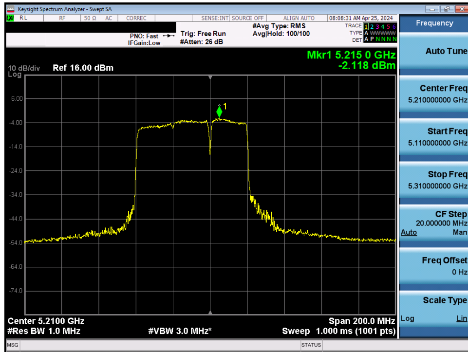
Plot 7-167. Power Spectral Density Plot MIMO ANT1 (80MHz BW 802.11be (UNII Band 1) – Ch. 42)
