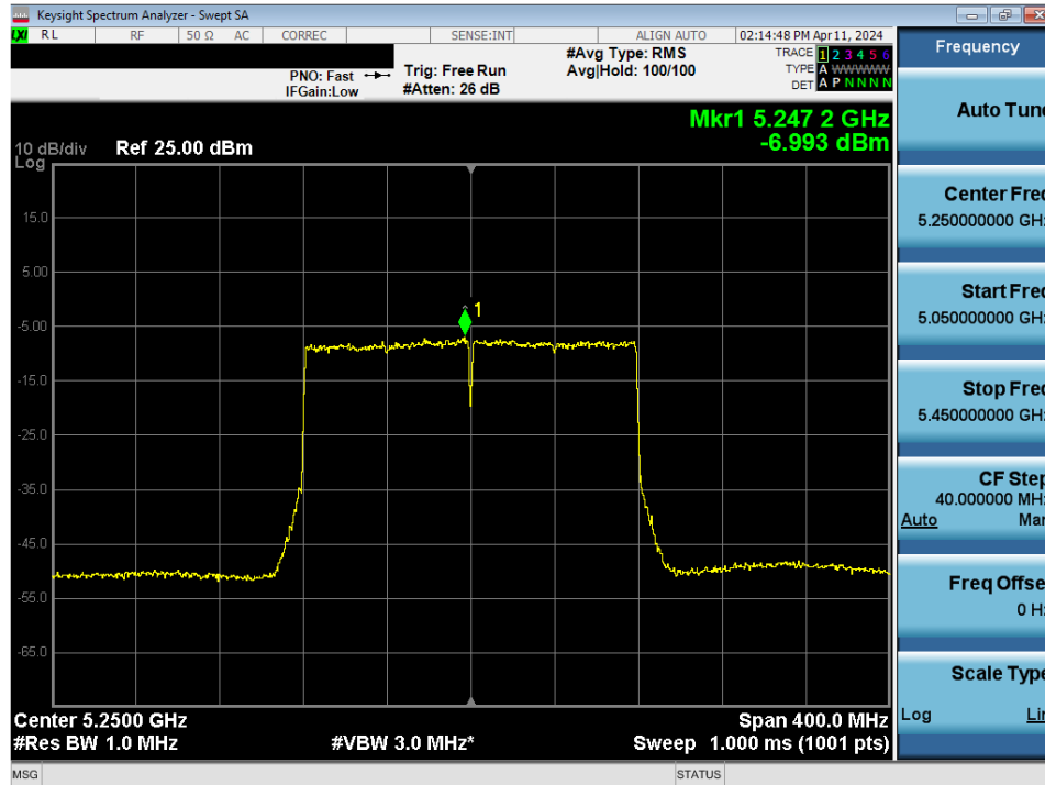
Plot 7-134. Power Spectral Density Plot MIMO ANT2 (160MHz BW 802.11ax/be (UNII Band 1/2A) – Ch. 50)
