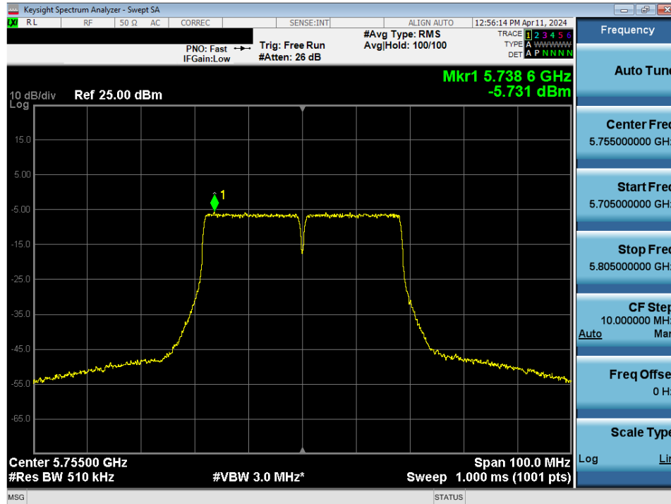
Plot 7-154. Power Spectral Density Plot MIMO ANT2 (40MHz BW 802.11n (UNII Band 3) – Ch. 151)
