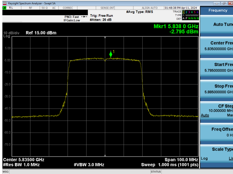
Plot 7-162. Power Spectral Density Plot MIMO ANT2 (40MHz BW 802.11ax/be (UNII Band 3/4) – Ch. 167)
