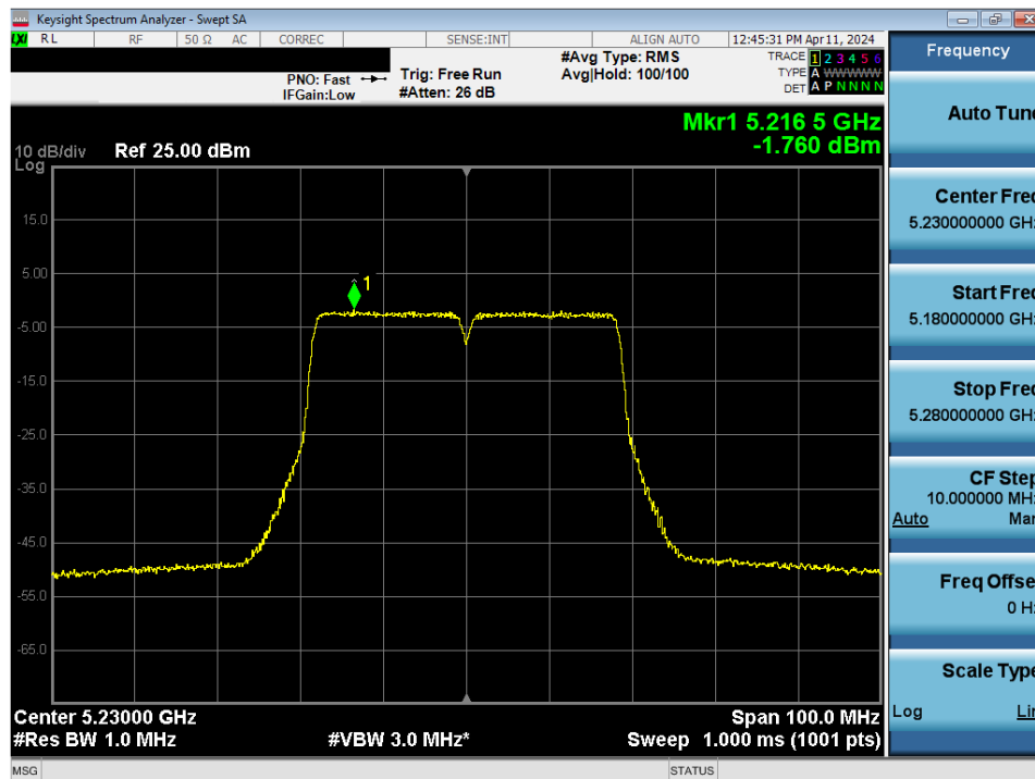
Plot 7-129. Power Spectral Density Plot MIMO ANT2 (40MHz BW 802.11n (UNII Band 1) – Ch. 46)
