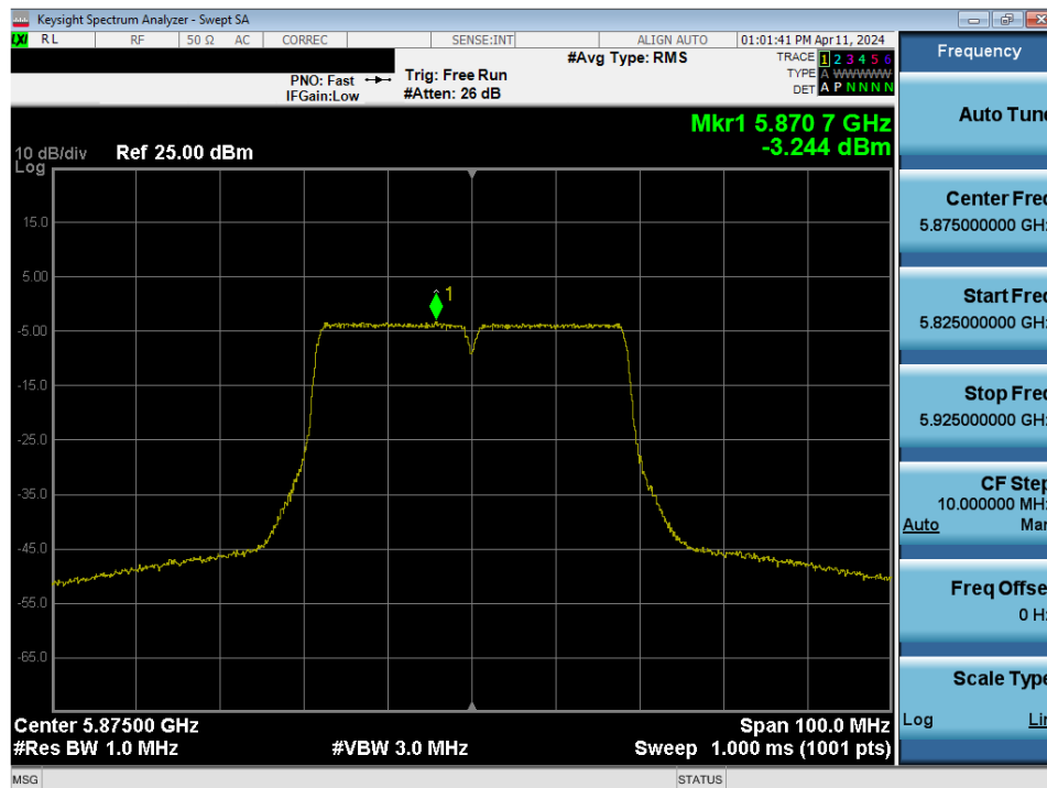
Plot 7-161. Power Spectral Density Plot MIMO ANT2 (40MHz BW 802.11n (UNII Band 4) – Ch. 175)
