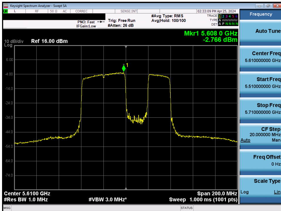
Plot 7-178. Power Spectral Density Plot MIMO ANT2 (80MHz BW 802.11be (UNII Band 2C) – Ch. 122)
