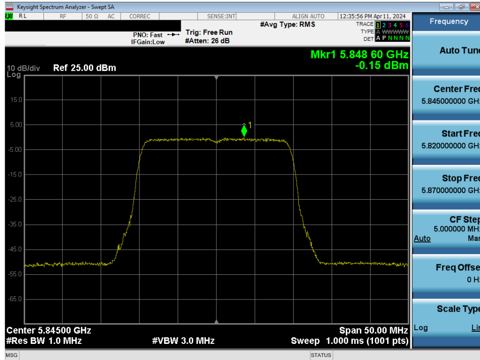
Plot 7-160. Power Spectral Density Plot MIMO ANT2 (20MHz BW 802.11ax/be (UNII Band 3/4) – Ch. 169)
