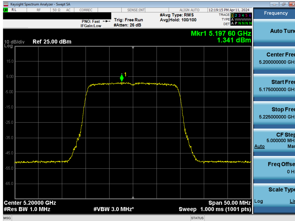
Plot 7-128. Power Spectral Density Plot MIMO ANT2 (20MHz BW 802.11ax/be (UNII Band 1) – Ch. 40)
