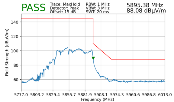
Plot 7-220. Radiated Upper Band Edge Plot MIMO (Peak – UNII Band 4)
