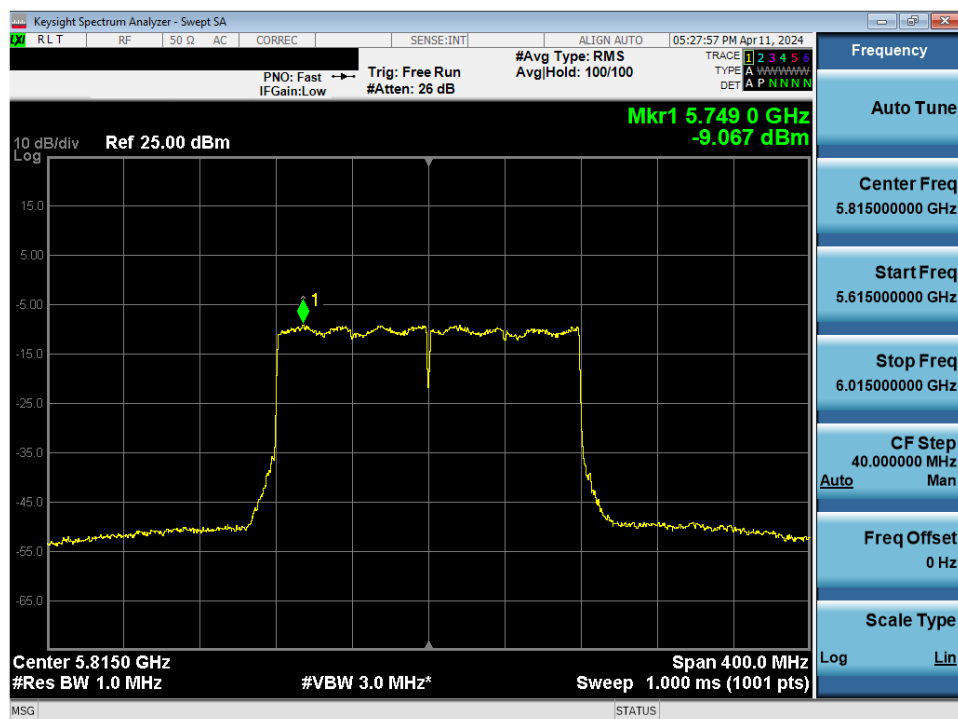
Plot 7-125. Power Spectral Density Plot MIMO ANT1 (160MHz BW 802.11ax/be (UNII Band 3/4) – Ch. 163)
