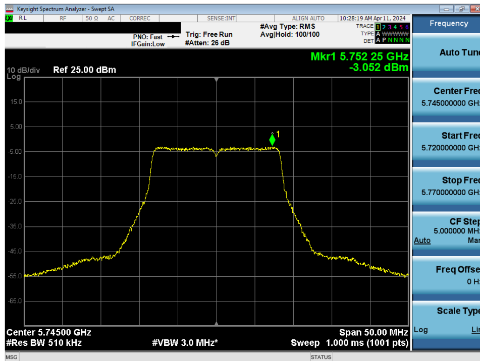
Plot 7-151. Power Spectral Density Plot MIMO ANT2 (802.11a (UNII Band 3) – Ch. 149)
