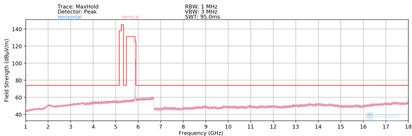
Plot 7-188. Radiated Spurious Plot above 1GHz MIMO (802.11a – UNII Band 4 Ch. 173)
