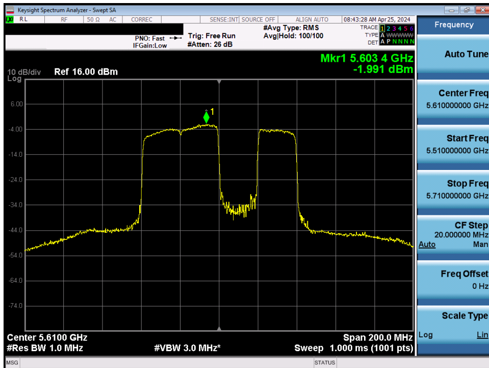
Plot 7-170. Power Spectral Density Plot MIMO ANT1 (80MHz BW 802.11be (UNII Band 2C) – Ch. 122)
