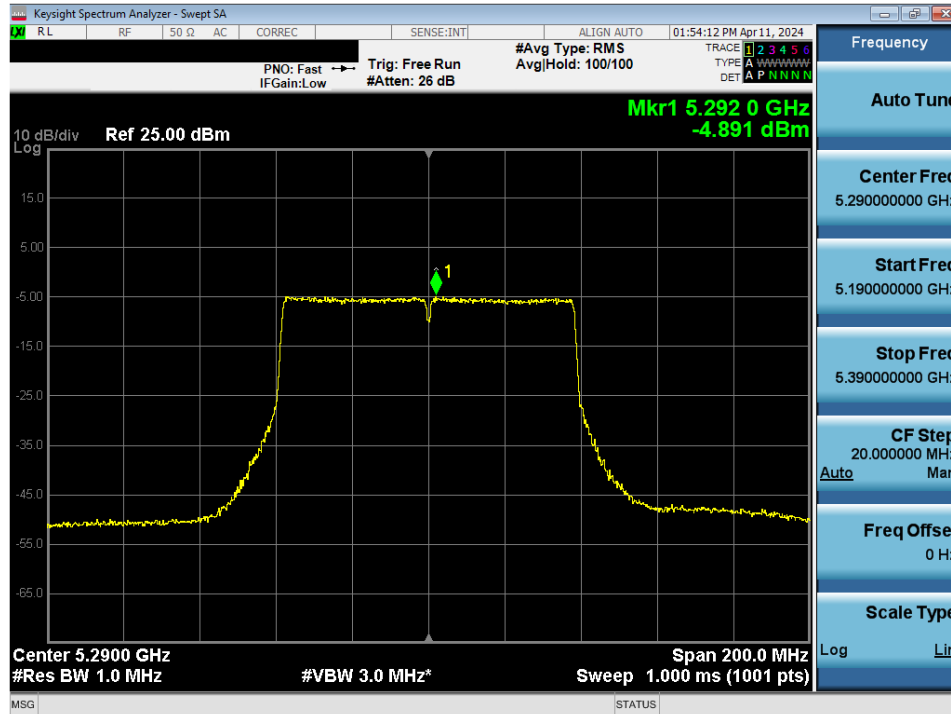
Plot 7-140. Power Spectral Density Plot MIMO ANT2 (80MHz BW 802.11ac (UNII Band 2A) – Ch. 58)
