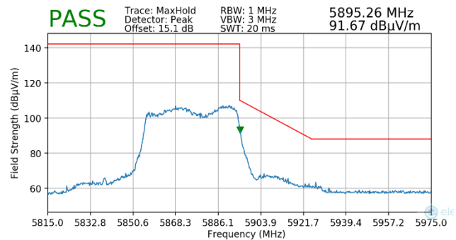
Plot 7-210. Radiated Upper Band Edge Plot MIMO (Peak – UNII Band 4)
