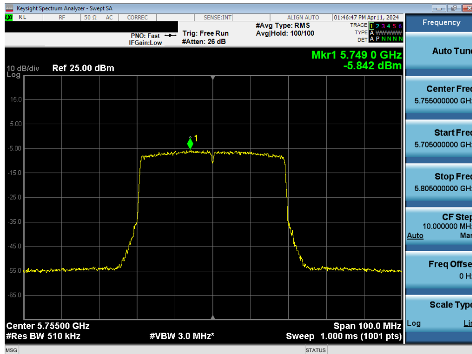
Plot 7-155. Power Spectral Density Plot MIMO ANT2 (40MHz BW 802.11ax/be (UNII Band 3) – Ch. 151)
