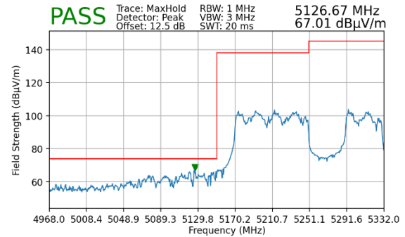
Plot 7-222. Radiated Lower Band Edge Plot MIMO (Peak – UNII Band 1)
