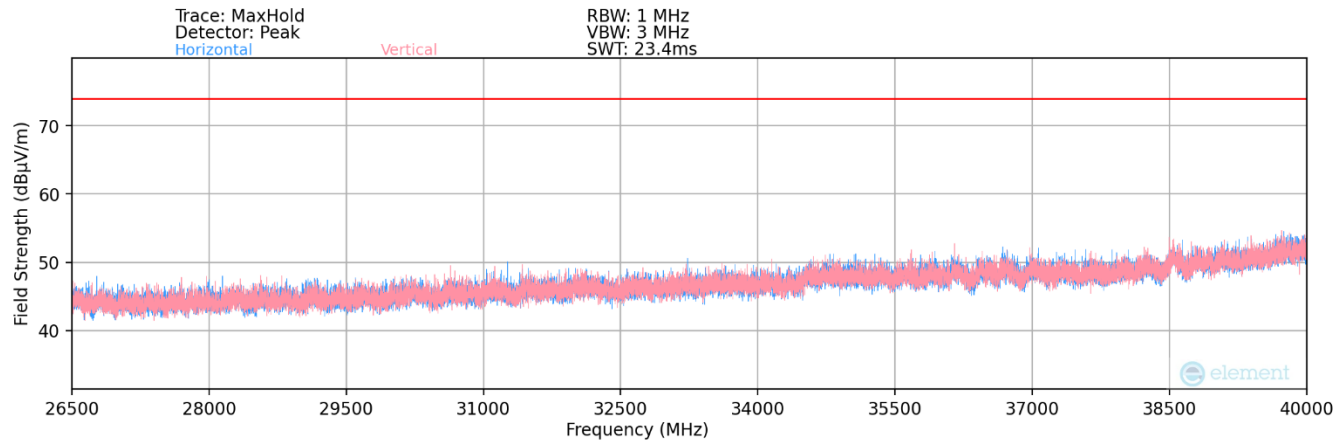
Plot 7-190. Radiated Spurious Plot 26.5GHz – 40GHz MIMO (802.11a)
