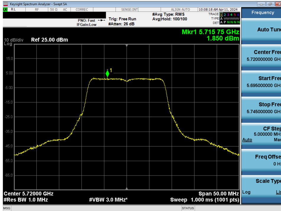
Plot 7-142. Power Spectral Density Plot MIMO ANT2 (802.11a (UNII Band 2C) – Ch. 144)
