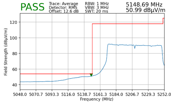
Plot 7-211. Radiated Lower Band Edge Plot MIMO (Average – UNII Band 1)
