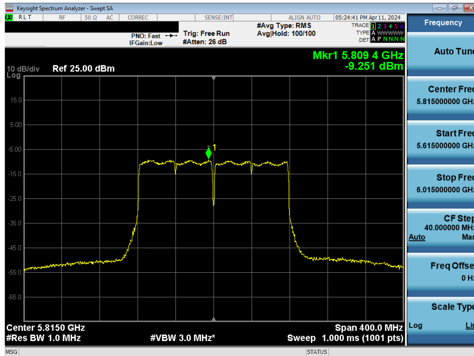
Plot 7-124. Power Spectral Density Plot MIMO ANT1 (160MHz BW 802.11ac (UNII Band 3/4) – Ch. 163)
