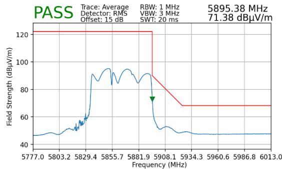
Plot 7-219. Radiated Upper Band Edge Plot MIMO (Average – UNII Band 4)
