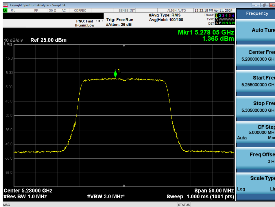
Plot 7-137. Power Spectral Density Plot MIMO ANT2 (20MHz BW 802.11ax/be (UNII Band 2A) – Ch. 56)
