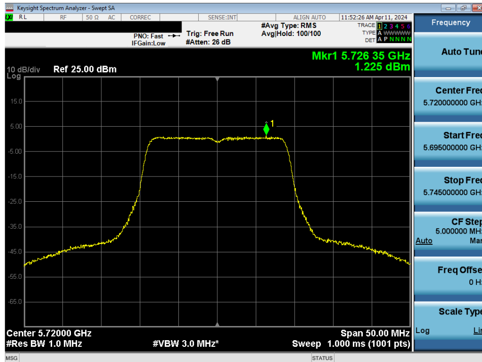
Plot 7-143. Power Spectral Density Plot MIMO ANT2 (20MHz BW 802.11n (UNII Band 2C) – Ch. 144)
