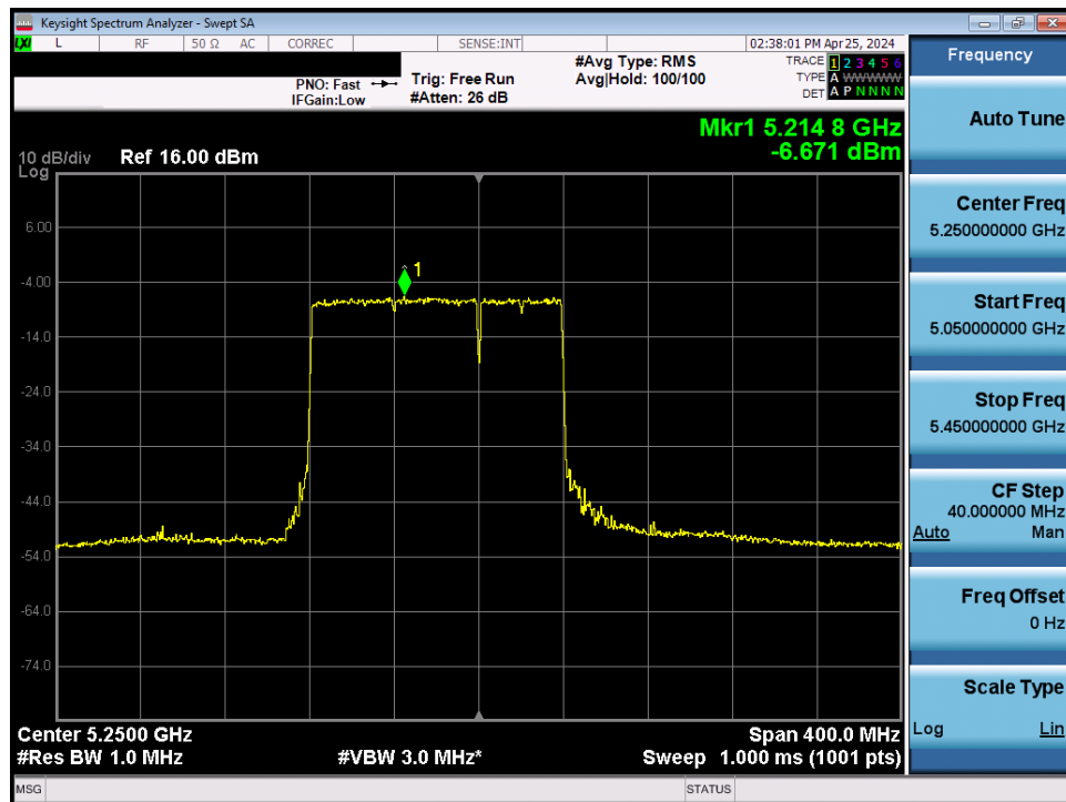
Plot 7-176. Power Spectral Density Plot MIMO ANT2 (160MHz BW 802.11be (UNII Band 1/2A) – Ch. 50)
