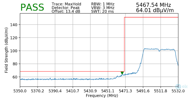
Plot 7-206. Radiated Lower Band Edge Plot MIMO (Peak – UNII Band 2C)
