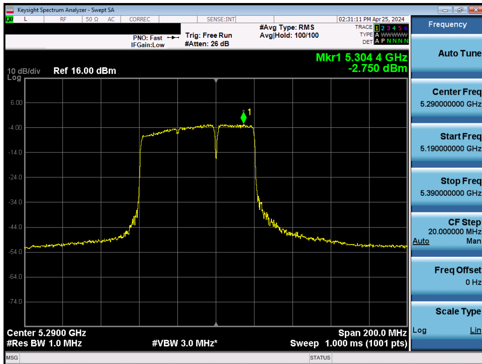
Plot 7-177. Power Spectral Density Plot MIMO ANT2 (80MHz BW 802.11be (UNII Band 2A) – Ch. 58)
