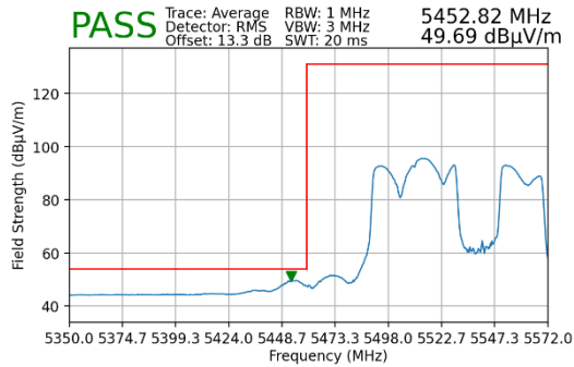
Plot 7-215. Radiated Lower Band Edge Plot MIMO (Average – UNII Band 2C)
