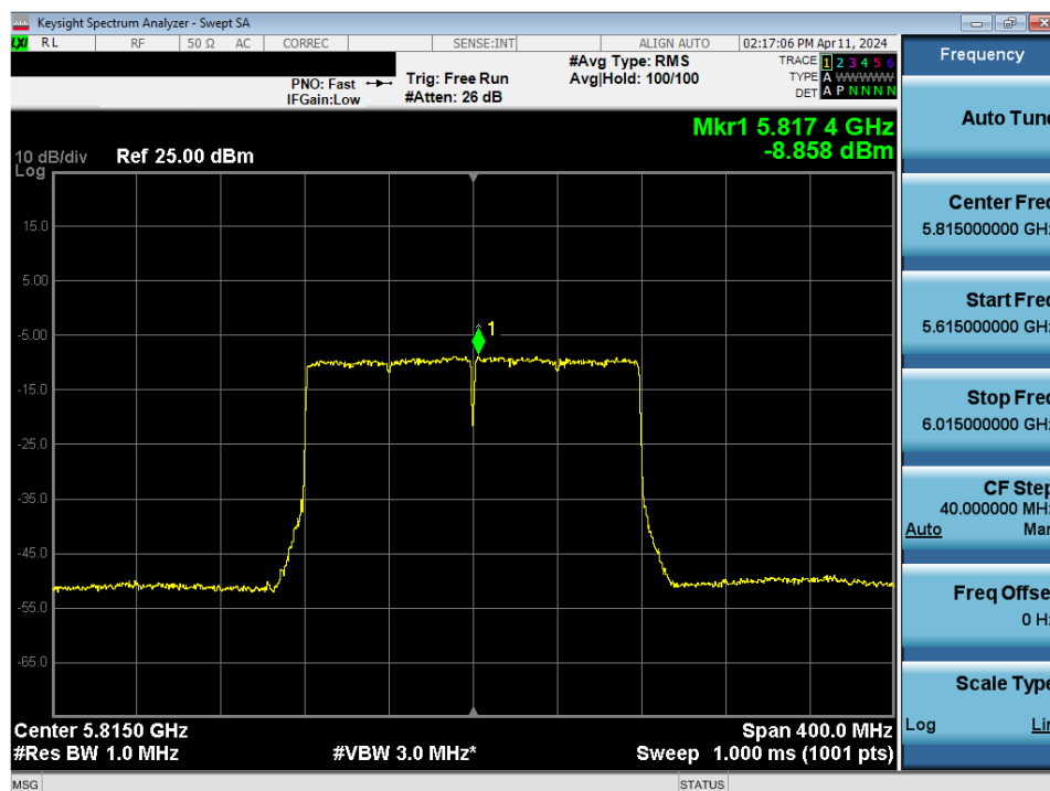
Plot 7-166. Power Spectral Density Plot MIMO ANT2 (160MHz BW 802.11ax/be (UNII Band 3/4) – Ch. 163)
