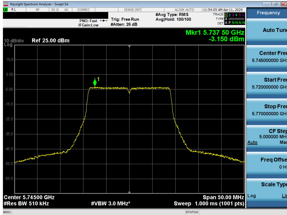
Plot 7-152. Power Spectral Density Plot MIMO ANT2 (20MHz BW 802.11n (UNII Band 3) – Ch. 149)
