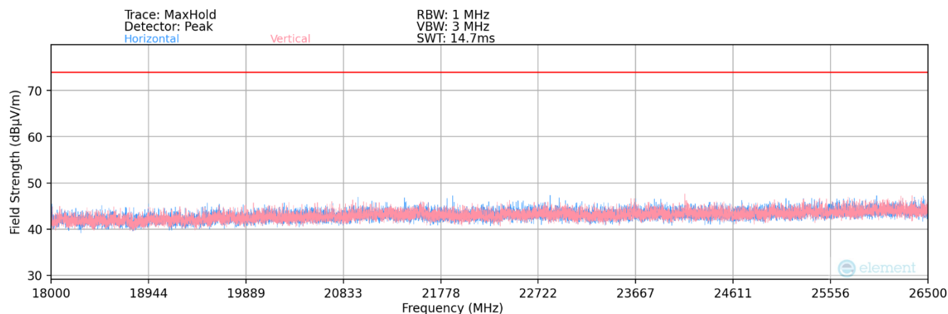
Plot 7-189. Radiated Spurious Plot 18GHz – 26.5GHz MIMO (802.11a)
