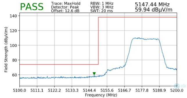
Plot 7-192. Radiated Lower Band Edge Plot MIMO (Peak – UNII Band 1)
