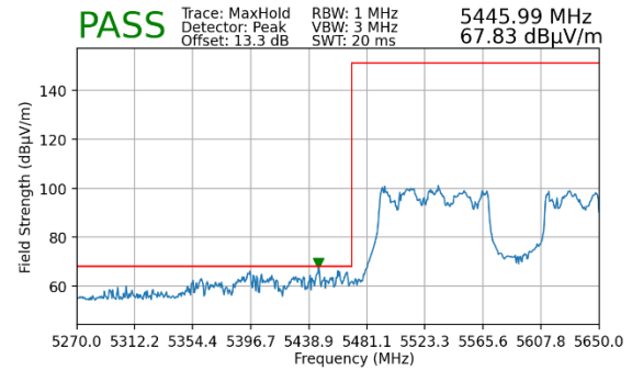
Plot 7-226. Radiated Lower Band Edge Plot MIMO (Peak – UNII Band 2C)
