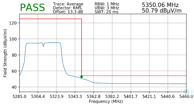
Plot 7-203. Radiated Upper Band Edge Plot MIMO (Average – UNII Band 2A)
