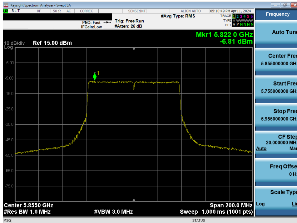
Plot 7-122. Power Spectral Density Plot MIMO ANT1 (80MHz BW 802.11ac (UNII Band 3/4) – Ch. 171)
