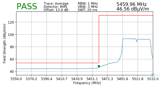
Plot 7-205. Radiated Lower Band Edge Plot MIMO (Average – UNII Band 2C)
