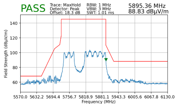
Plot 7-229. Radiated Lower Band Edge Plot MIMO (Peak – UNII Band 4)
