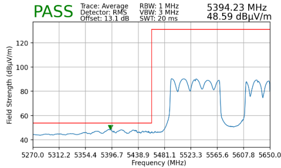
Plot 7-225. Radiated Lower Band Edge Plot MIMO (Average – UNII Band 2C)
