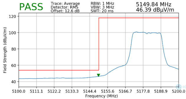
Plot 7-191. Radiated Lower Band Edge Plot MIMO (Average – UNII Band 1)
