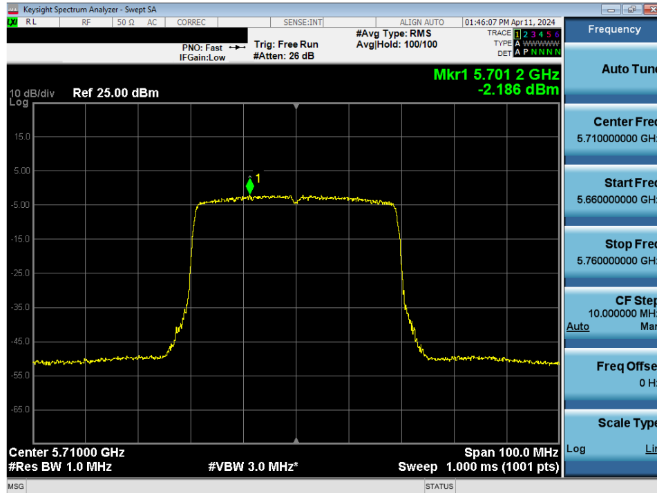
Plot 7-146. Power Spectral Density Plot MIMO ANT2 (40MHz BW 802.11ax/be (UNII Band 2C) – Ch. 142)
