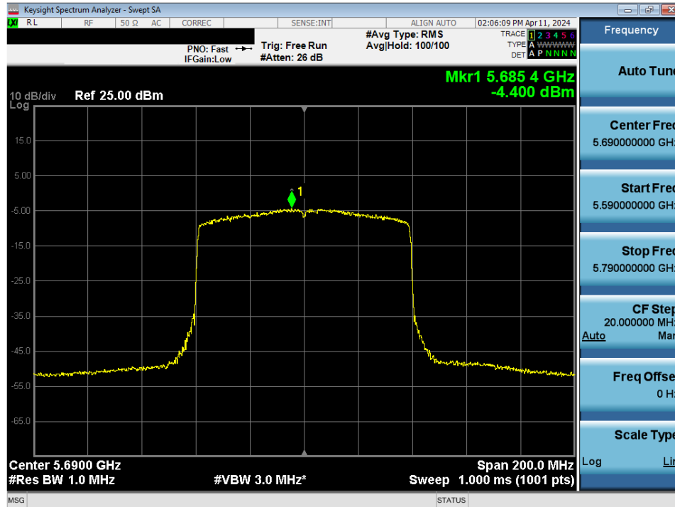
Plot 7-148. Power Spectral Density Plot MIMO ANT2 (80MHz BW 802.11ax/be (UNII Band 2C) – Ch. 138)
