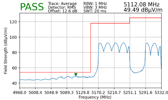
Plot 7-221. Radiated Lower Band Edge Plot MIMO (Average – UNII Band 1)
