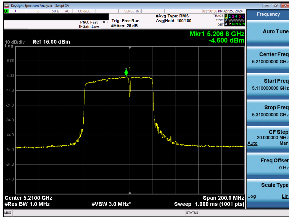
Plot 7-175. Power Spectral Density Plot MIMO ANT2 (80MHz BW 802.11be (UNII Band 1) – Ch. 42)
