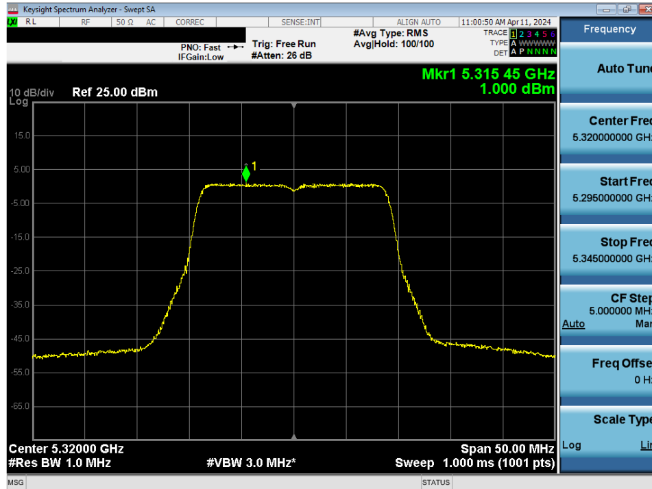
Plot 7-136. Power Spectral Density Plot MIMO ANT2 (20MHz BW 802.11n (UNII Band 2A) – Ch. 64)
