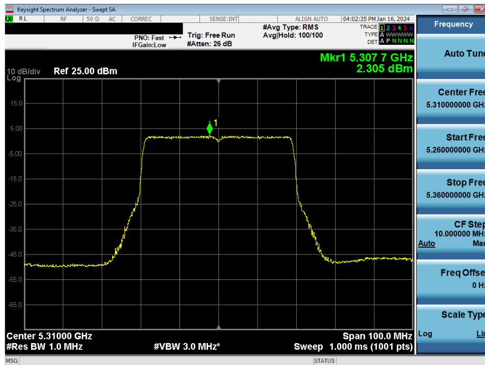
Plot 7-139. Power Spectral Density Plot MIMO ANT2 (40MHz BW 802.11ax/be (UNII Band 2A) – Ch. 62)
