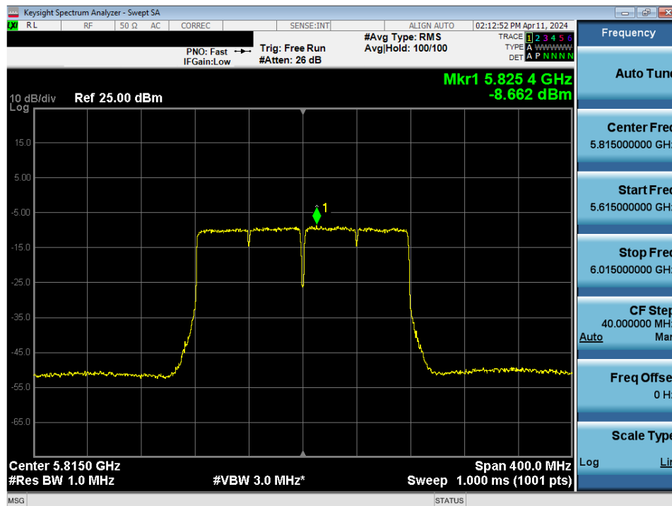
Plot 7-165. Power Spectral Density Plot MIMO ANT2 (160MHz BW 802.11ac (UNII Band 3/4) – Ch. 163)
