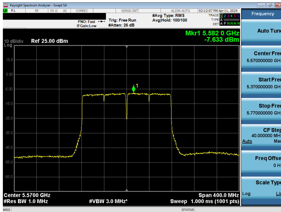
Plot 7-149. Power Spectral Density Plot MIMO ANT2 (160MHz BW 802.11ac (UNII Band 2C) – Ch. 114)
