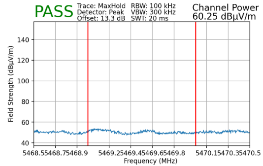
Plot 7-216. Radiated Lower Band Edge Plot MIMO (Peak – UNII Band 2C)
