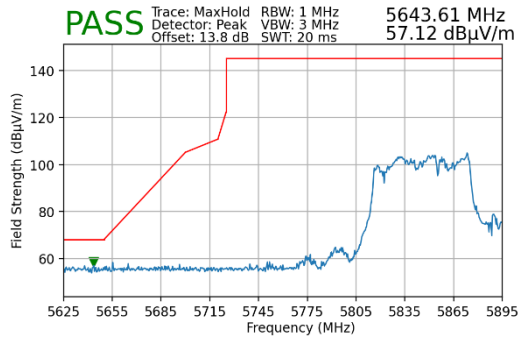
Plot 7-218. Radiated Lower Band Edge Plot MIMO (Peak – UNII Band 4)
