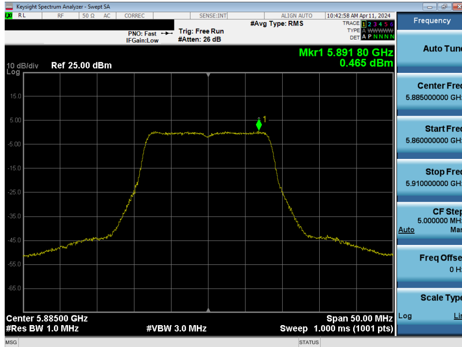
Plot 7-158. Power Spectral Density Plot MIMO ANT2 (20MHz BW 802.11a (UNII Band 4) – Ch. 177)
