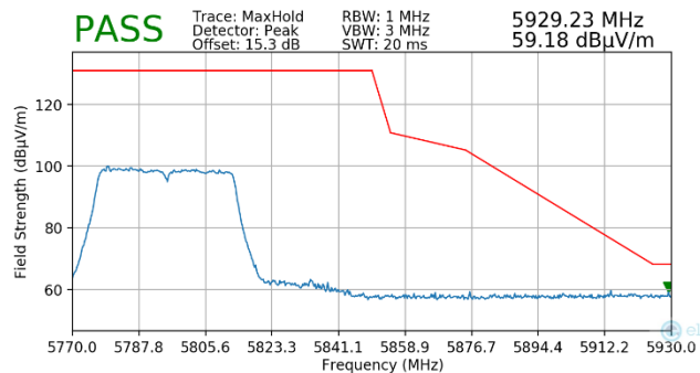
Plot 7-207. Radiated Upper Band Edge Plot MIMO (Peak – UNII Band 3)
