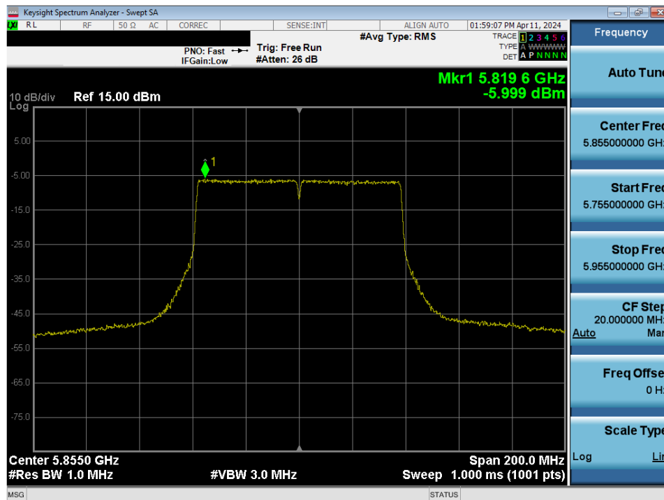
Plot 7-163. Power Spectral Density Plot MIMO ANT2 (80MHz BW 802.11ac (UNII Band 3/4) – Ch. 171)
