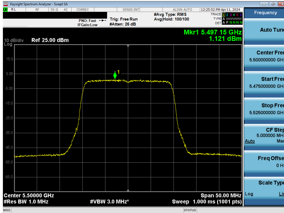
Plot 7-144. Power Spectral Density Plot MIMO ANT2 (20MHz BW 802.11ax/be (UNII Band 2C) – Ch. 100)
