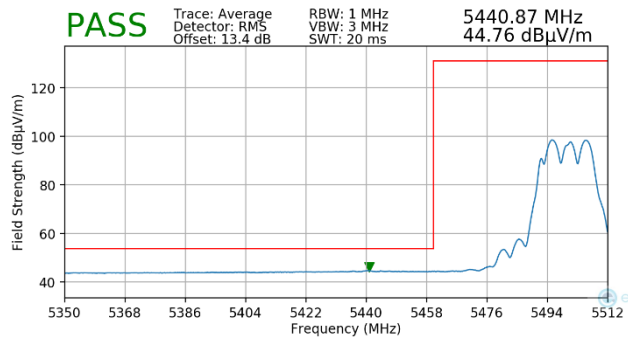
Plot 7-195. Radiated Lower Band Edge Plot MIMO (Average – UNII Band 2C)
