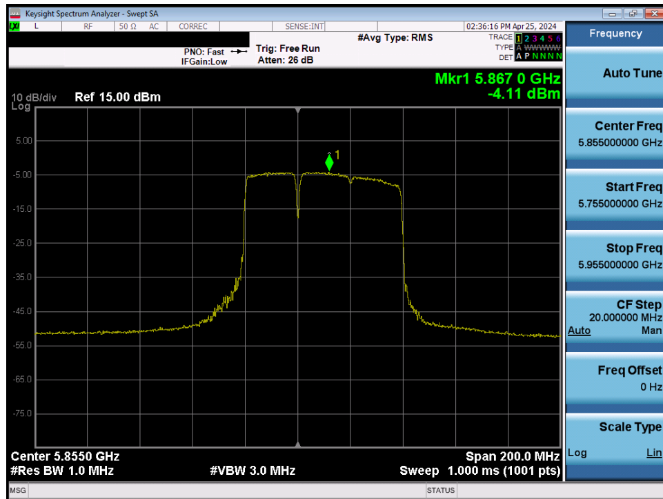
Plot 7-181. Power Spectral Density Plot MIMO ANT2 (80MHz BW 802.11be (UNII Band 3/4) – Ch. 171)
