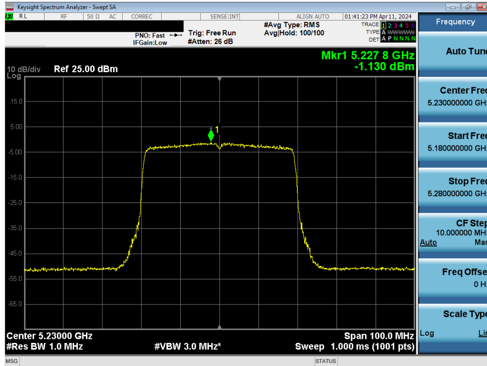
Plot 7-130. Power Spectral Density Plot MIMO ANT2 (40MHz BW 802.11ax/be (UNII Band 1) – Ch. 46)
