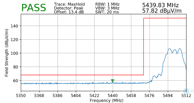
Plot 7-196. Radiated Lower Band Edge Plot MIMO (Peak – UNII Band 2C)
