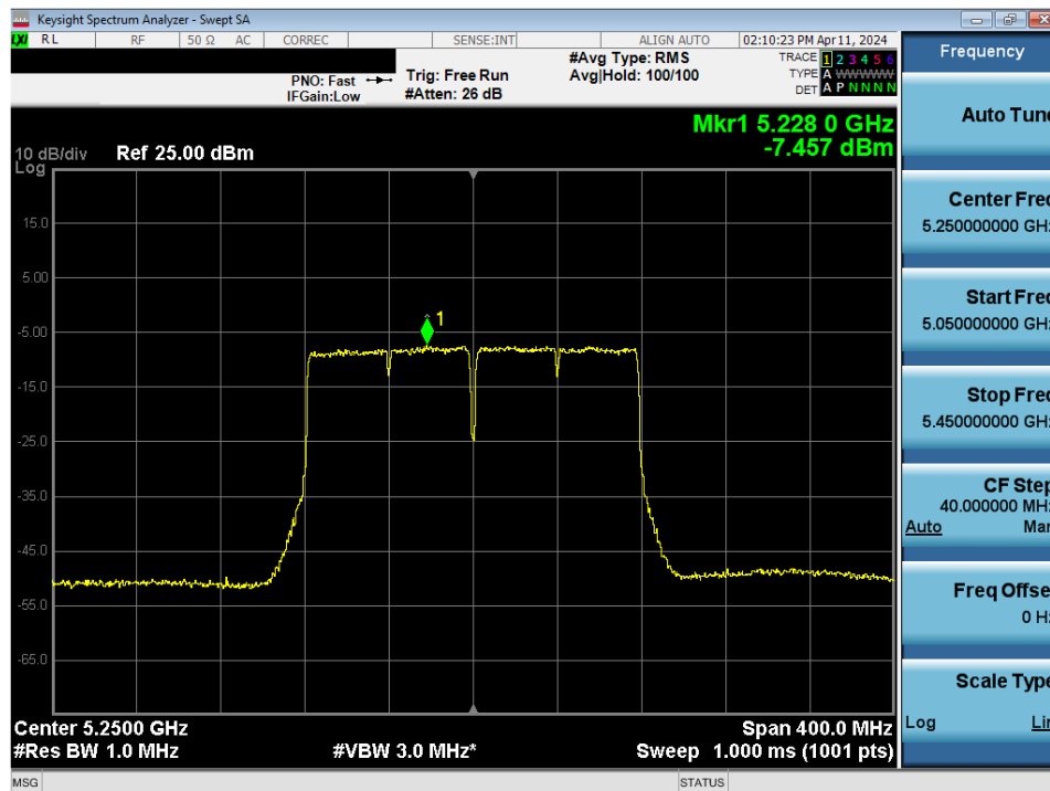
Plot 7-133. Power Spectral Density Plot MIMO ANT2 (160MHz BW 802.11ac (UNII Band 1/2A) – Ch. 50)
