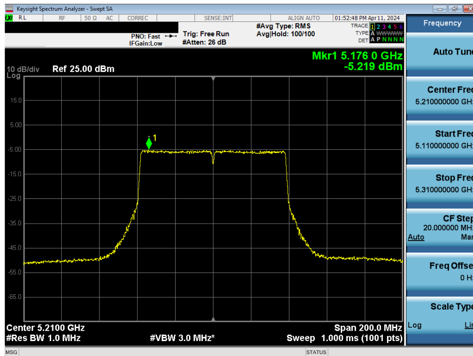
Plot 7-131. Power Spectral Density Plot MIMO ANT2 (80MHz BW 802.11ac (UNII Band 1) – Ch. 42)
