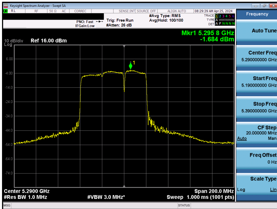
Plot 7-169. Power Spectral Density Plot MIMO ANT1 (80MHz BW 802.11be (UNII Band 2A) – Ch. 58)
