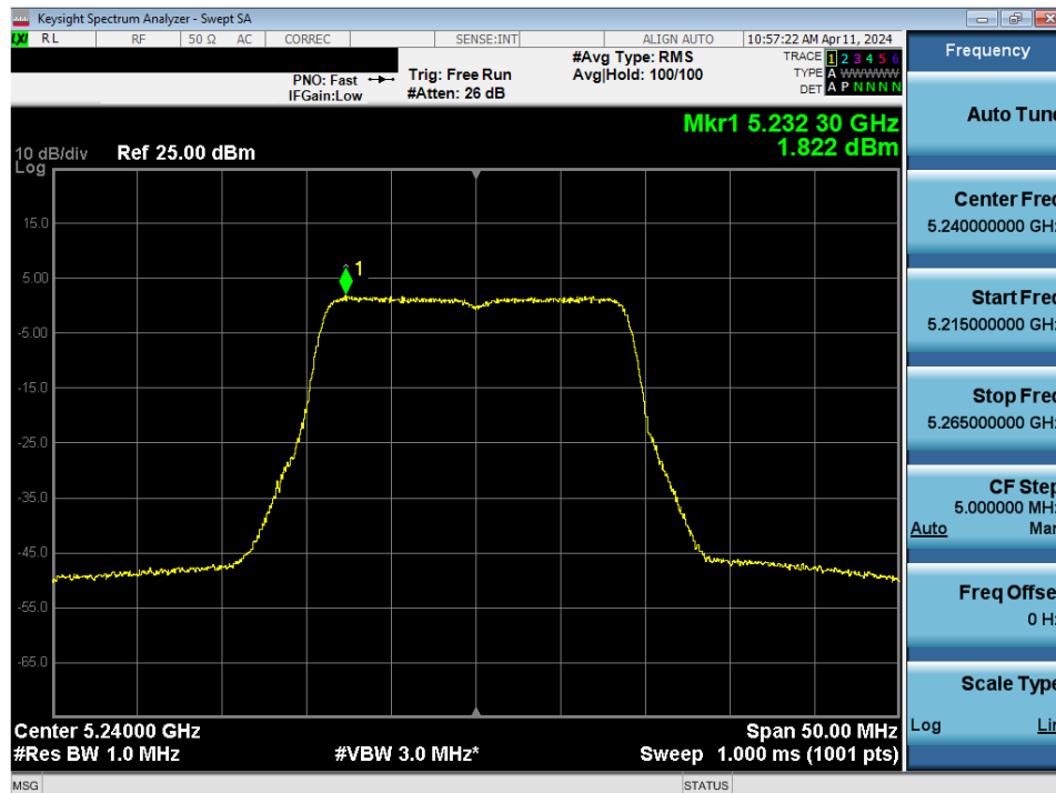
Plot 7-127. Power Spectral Density Plot MIMO ANT2 (20MHz BW 802.11n (UNII Band 1) – Ch. 48)
