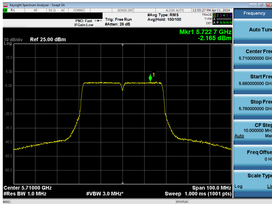
Plot 7-145. Power Spectral Density Plot MIMO ANT2 (40MHz BW 802.11n (UNII Band 2C) – Ch. 142)
