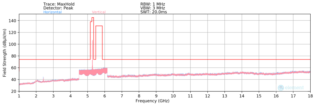
Plot 7-185. Radiated Spurious Plot above 1GHz MIMO (802.11a – UNII Band 2A Ch. 56)
