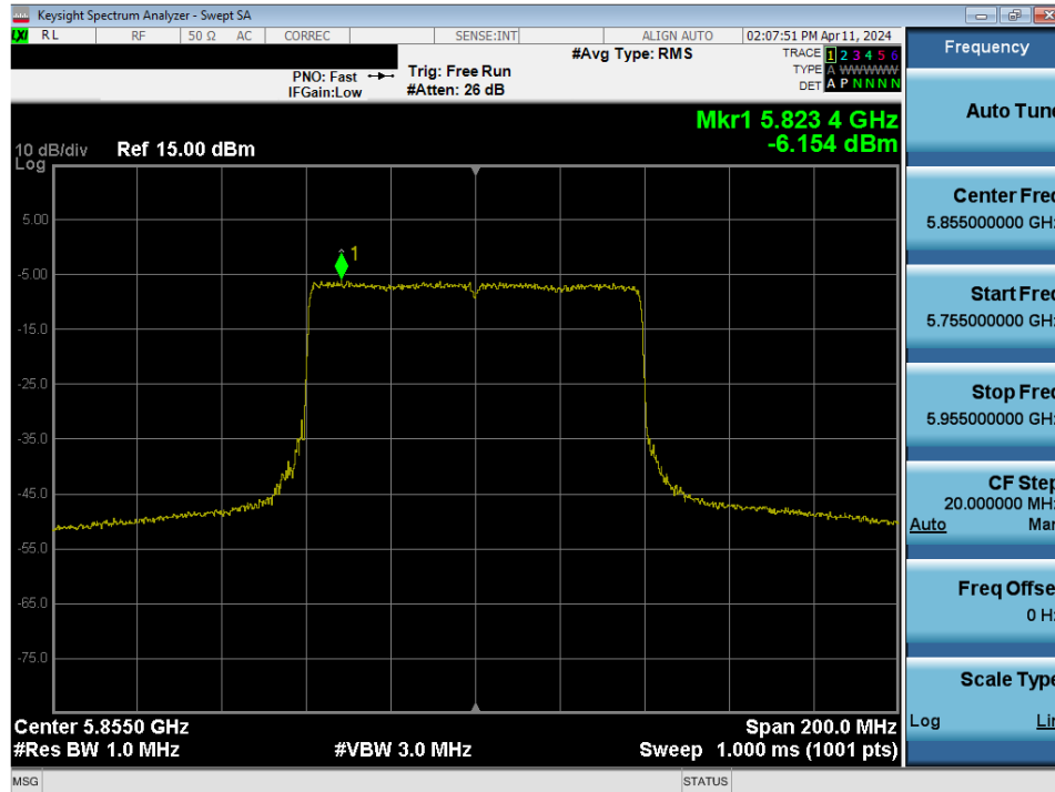
Plot 7-164. Power Spectral Density Plot MIMO ANT2 (80MHz BW 802.11ax/be (UNII Band 3/4) – Ch. 171)
