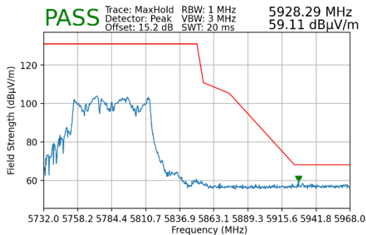
Plot 7-217. Radiated Upper Band Edge Plot MIMO (Peak – UNII Band 3)
