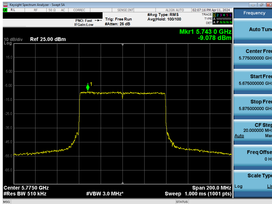
Plot 7-157. Power Spectral Density Plot MIMO ANT2 (80MHz BW 802.11ax/be (UNII Band 3) – Ch. 155)
