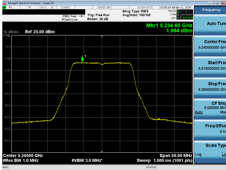
Plot 7-126. Power Spectral Density Plot MIMO ANT2 (802.11a (UNII Band 1) – Ch. 48)
