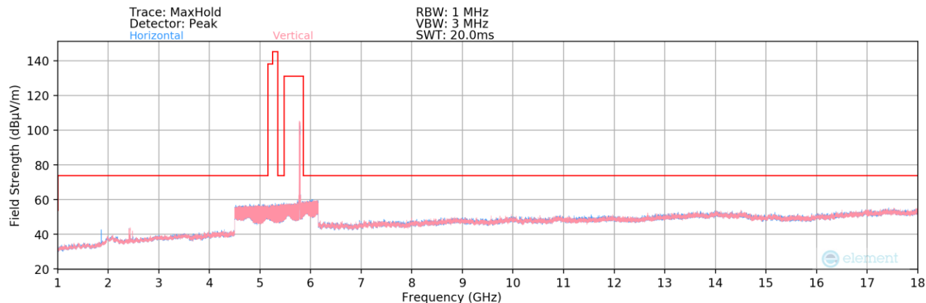
Plot 7-187. Radiated Spurious Plot above 1GHz MIMO (802.11a – UNII Band 3 Ch. 157)
