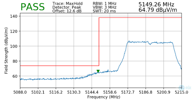
Plot 7-202. Radiated Lower Band Edge Plot MIMO (Peak – UNII Band 1)
