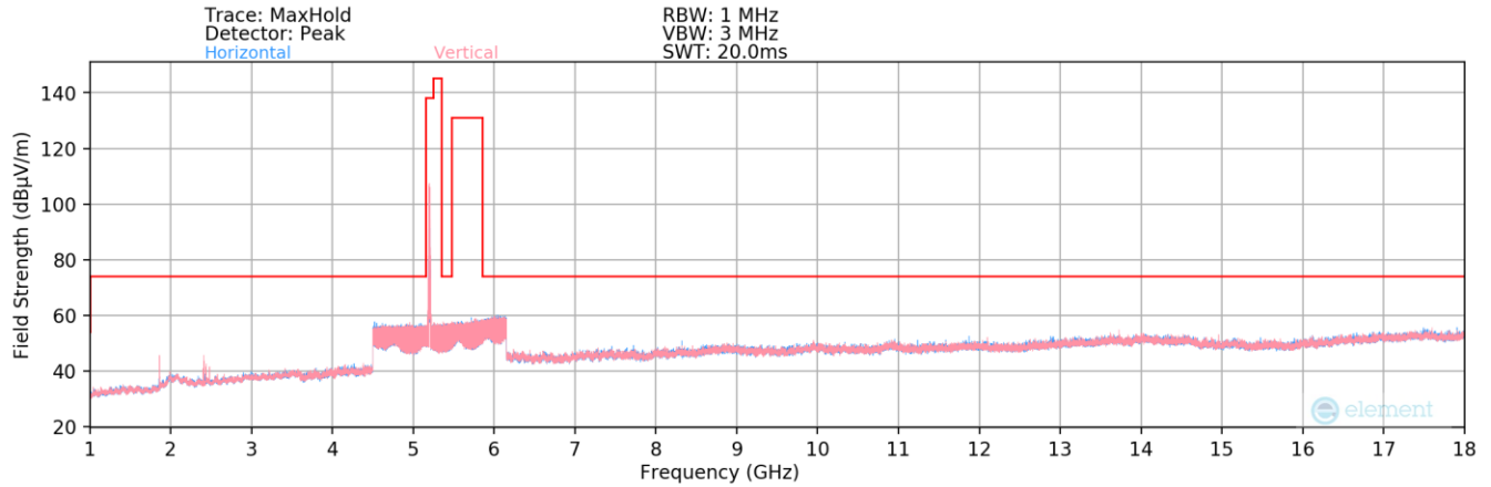
Plot 7-184. Radiated Spurious Plot above 1GHz MIMO (802.11a – UNII Band 1 Ch. 40)
