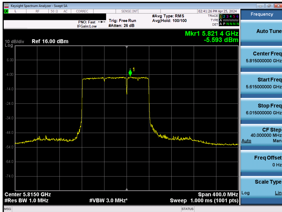
Plot 7-182. Power Spectral Density Plot MIMO ANT2 (160MHz BW 802.11be (UNII Band 3/4) – Ch. 163)
