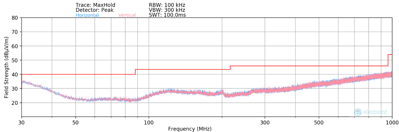
Plot 7-183. Radiated Spurious Plot below 1GHz MIMO (802.11a)
